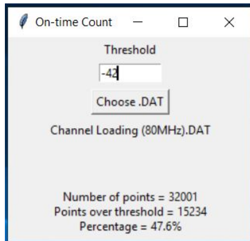
Figure 9-2. Band 2C - Channel Loading Calculation (80MHz)
