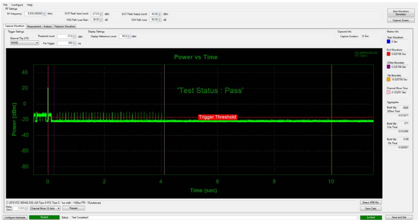
Figure 9-3. 5530MHz - Channel Move/ Closing Transmission Time - (80 MHz)
