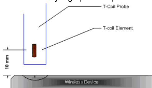
Figure 4-10 Measurement Distance
