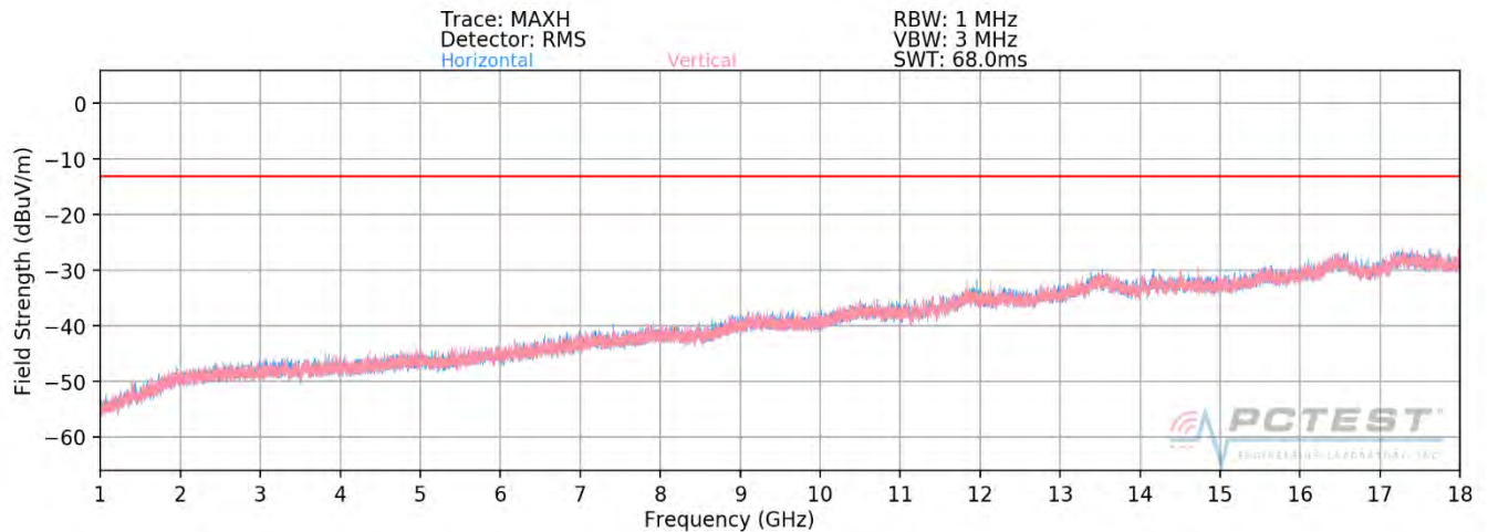
Plot 7-52. J Dipole Radiated Spurious Plot 1-18 GHz (1CC QPSK Mid Channel V Beam)
