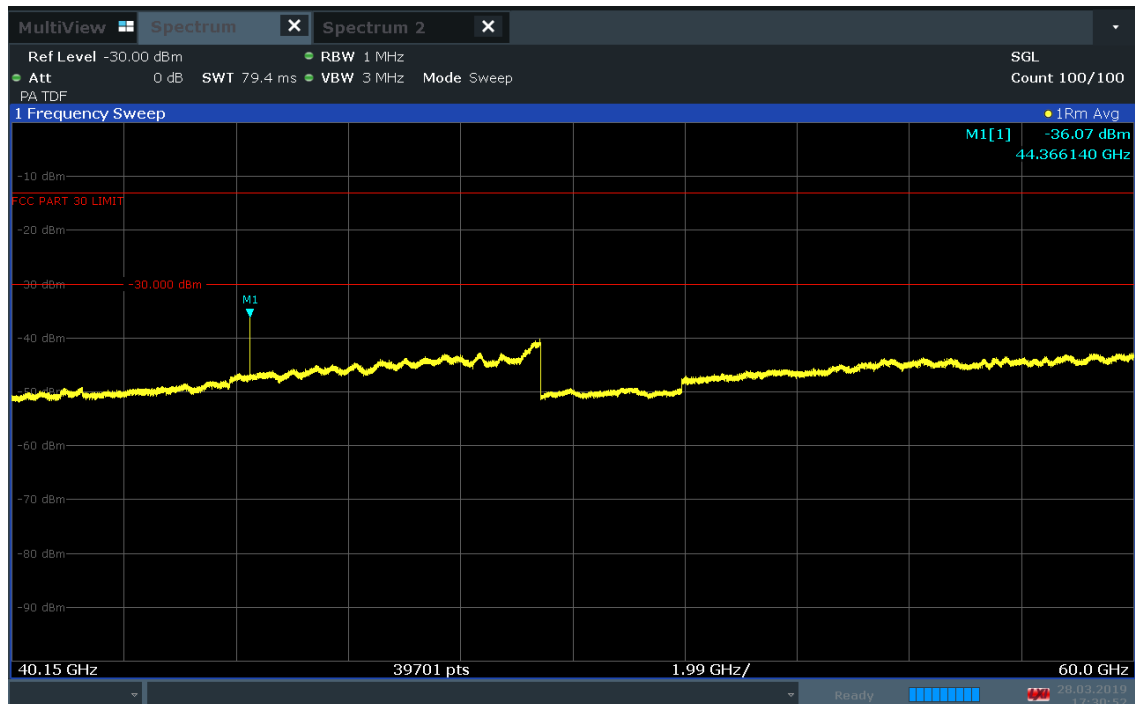
Plot 7-100. J Patch Radiated Spurious Plot 40.15-60 GHz (1CC QPSK Mid Channel H Beam)
