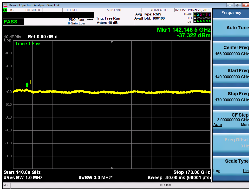
Plot 7-77. J Dipole Radiated Spurious Plot 140-170 GHz (1CC QPSK Low Channel H Beam)
