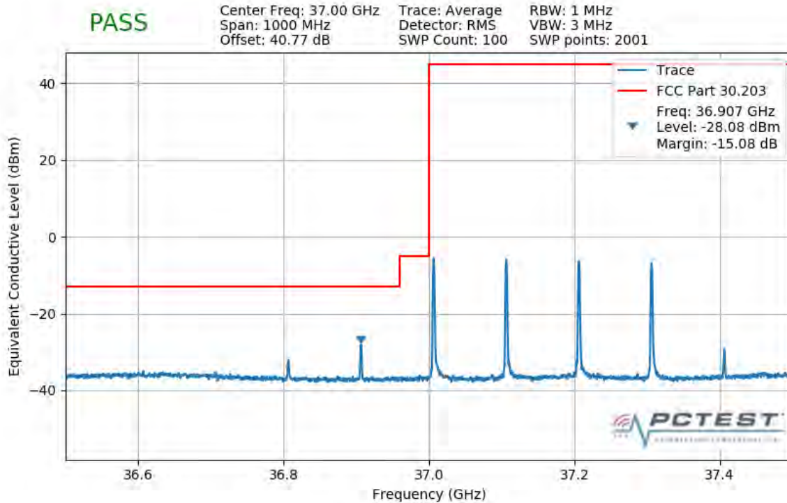
Plot 7-414. Lower Band Edge Plot (4CC 400MHz QPSK 1 RB)
