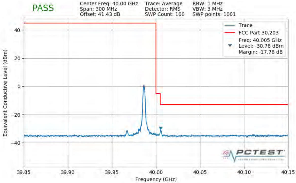
Plot 7-419. Upper Band Edge Plot (1CC 50MHz 16QAM 1 RB)
