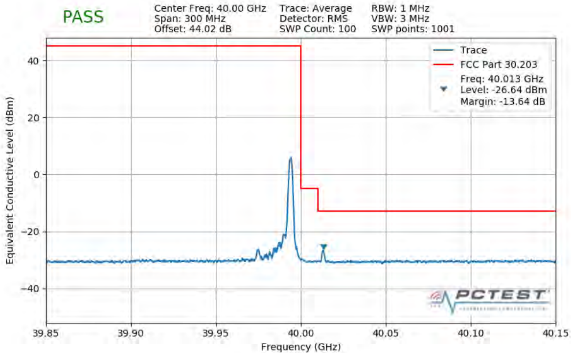
Plot 7-488. Upper Band Edge Plot (1CC 100MHz 64QAM 1 RB)
