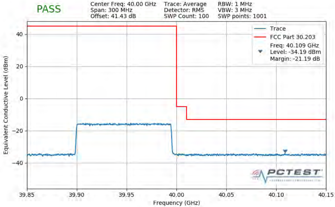
Plot 7-421. Upper Band Edge Plot (1CC 100MHz QPSK Full RB)
