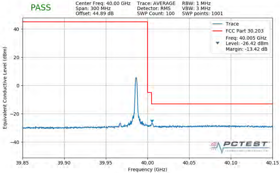
Plot 7-355. Upper Band Edge Plot (1CC 50MHz 16QAM 1 RB)
