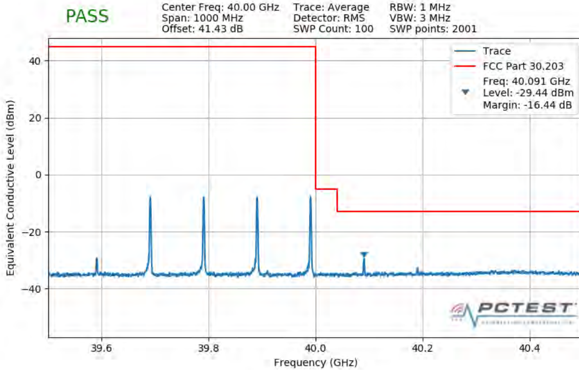
Plot 7-431. Upper Band Edge Plot (4CC 400MHz 16QAM 1 RB)
