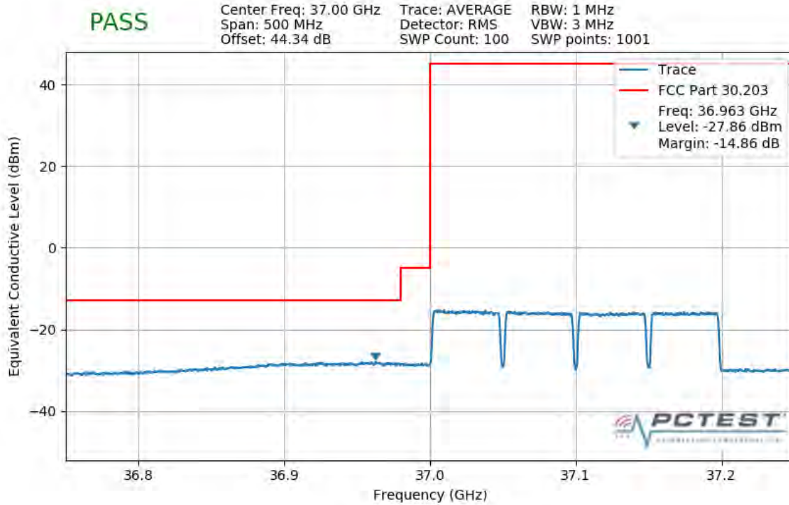
Plot 7-377. Lower Band Edge Plot (4CC 200MHz QPSK Full RB)
