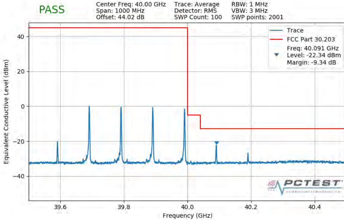
Plot 7-463. Upper Band Edge Plot (4CC 400MHz 16QAM 1 RB)
