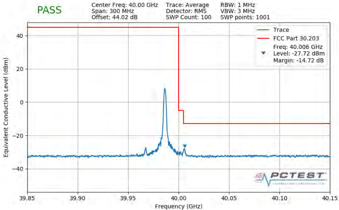
Plot 7-450. Upper Band Edge Plot (1CC 50MHz QPSK 1 RB)
