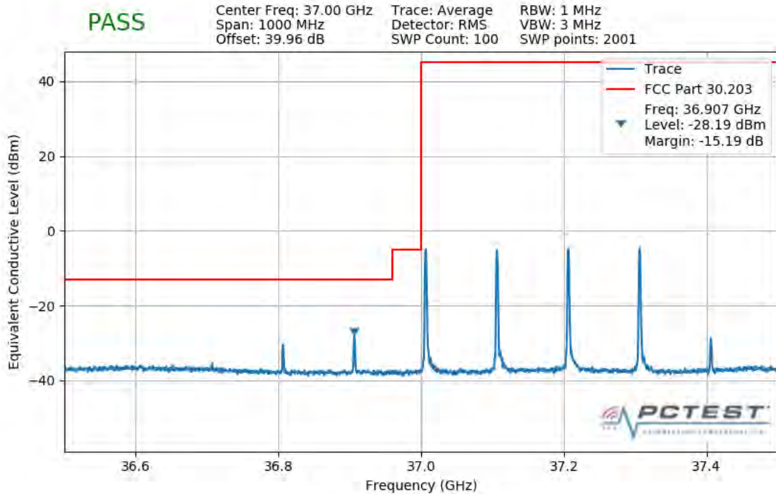
Plot 7-510. Lower Band Edge Plot (4CC 400MHz QPSK 1 RB)
