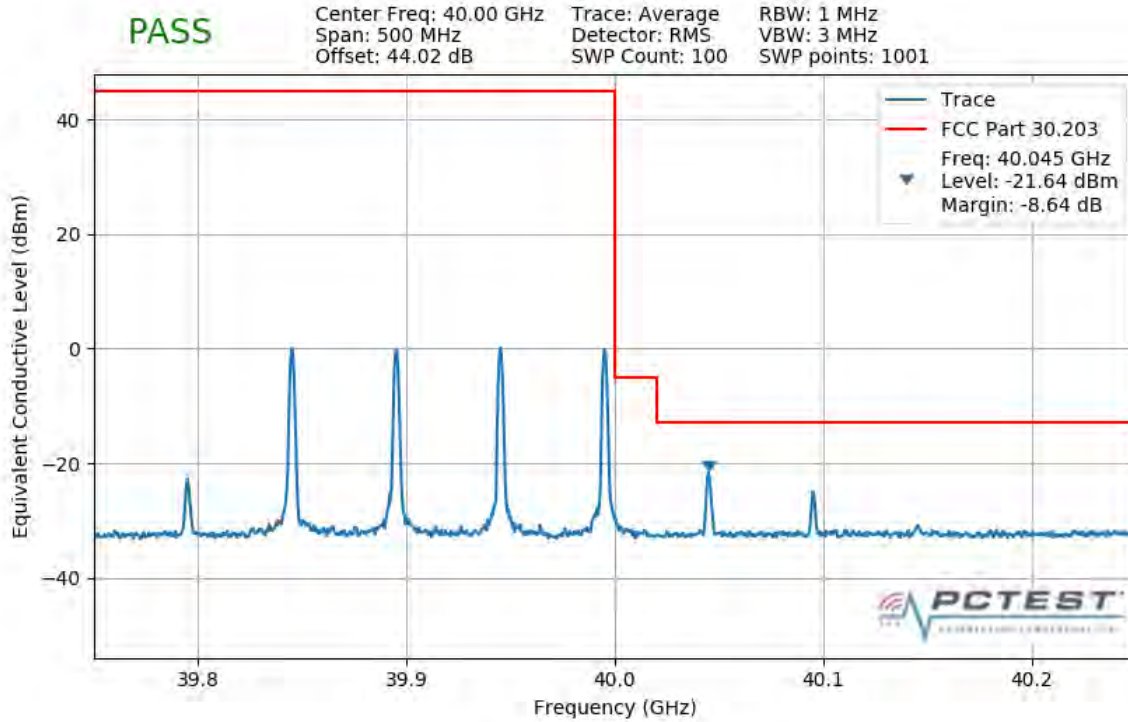
Plot 7-459. Upper Band Edge Plot (4CC 200MHz 16QAM 1 RB)
