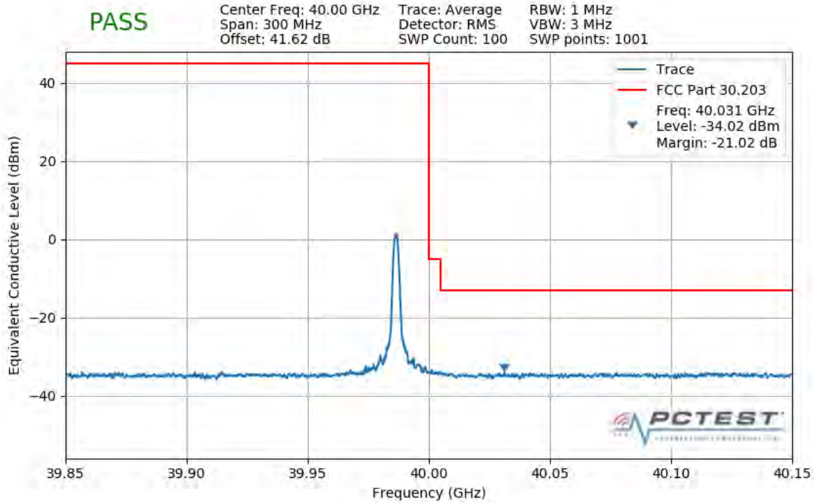
Plot 7-515. Upper Band Edge Plot (1CC 50MHz 16QAM 1 RB)
