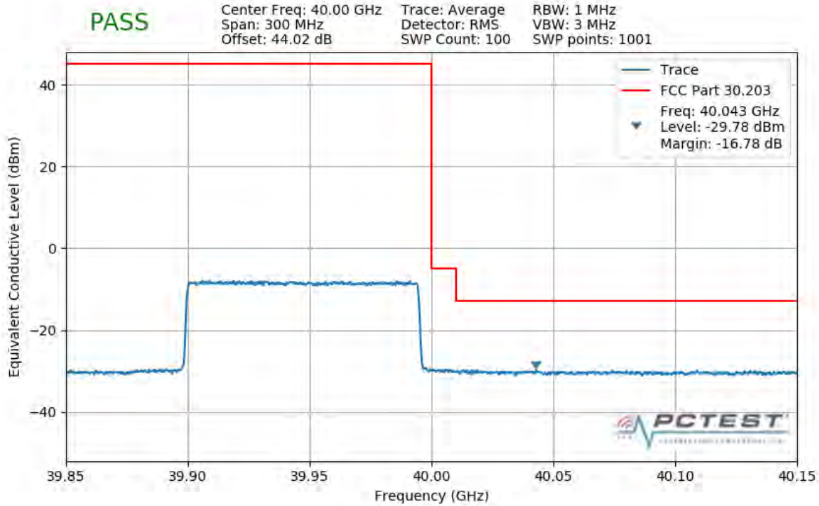
Plot 7-485. Upper Band Edge Plot (1CC 100MHz QPSK Full RB)
