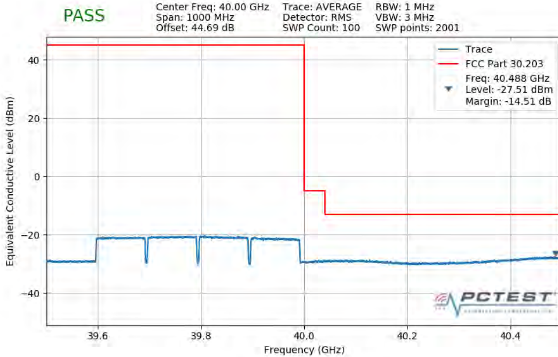
Plot 7-365. Upper Band Edge Plot (4CC 400MHz QPSK Full RB)
