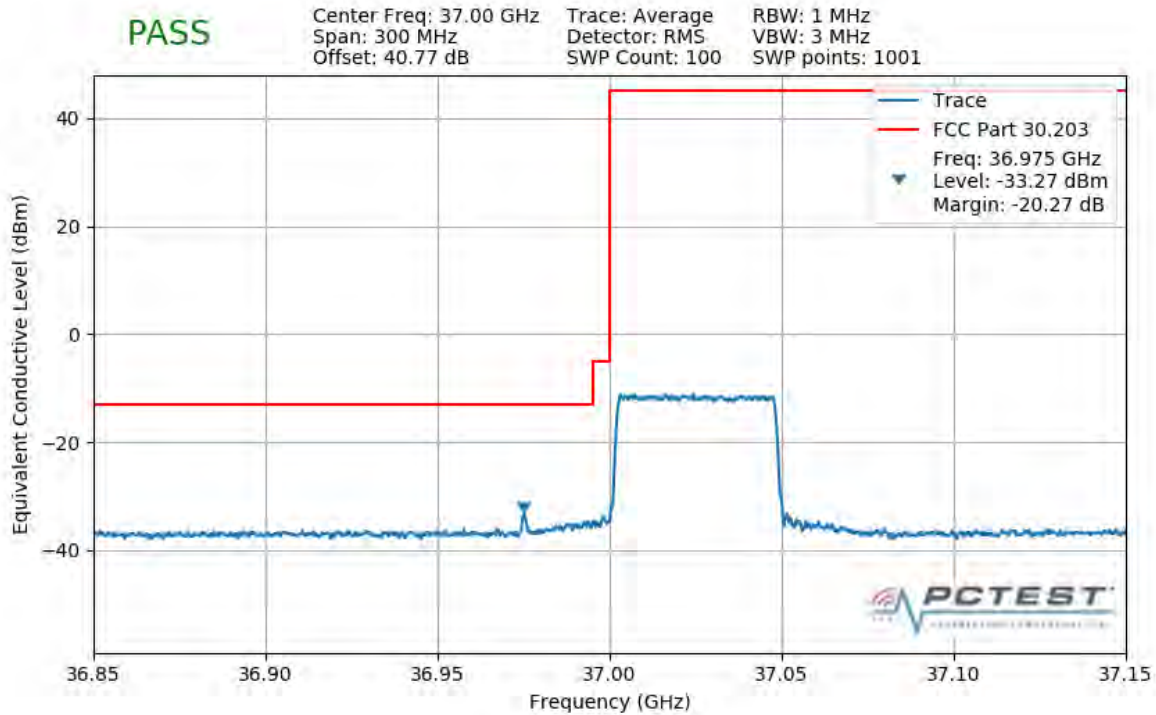
Plot 7-401. Lower Band Edge Plot (1CC 50MHz QPSK Full RB)
