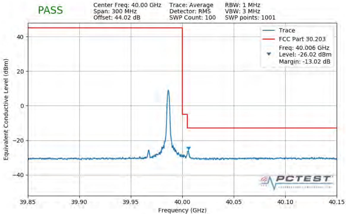
Plot 7-482. Upper Band Edge Plot (1CC 50MHz QPSK 1 RB)
