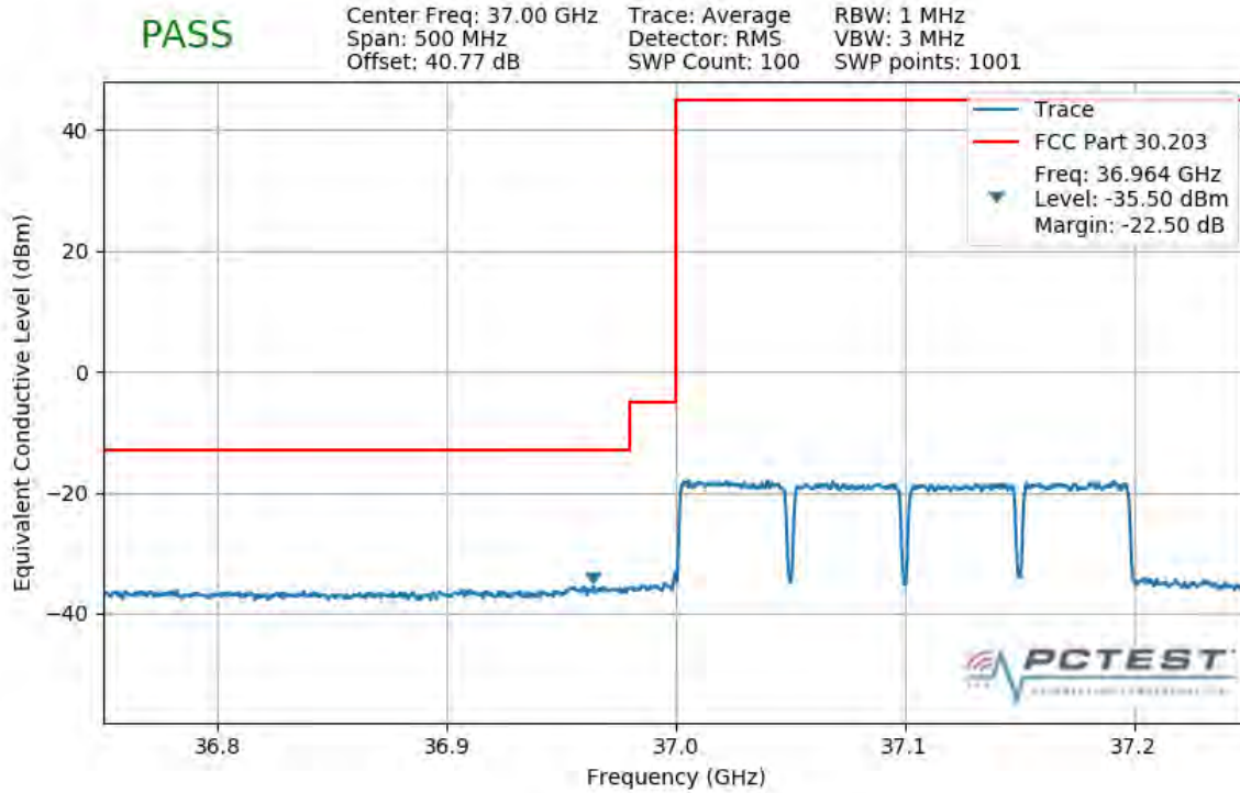
Plot 7-409. Lower Band Edge Plot (4CC 200MHz QPSK Full RB)
