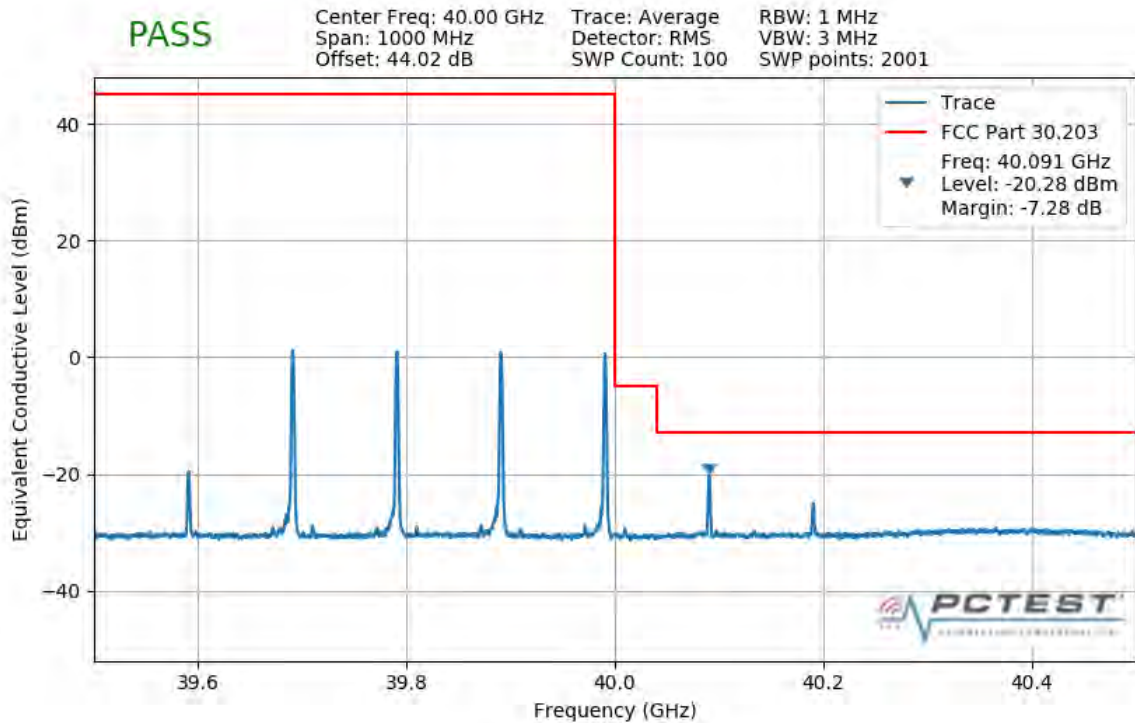
Plot 7-494. Upper Band Edge Plot (4CC 400MHz QPSK 1 RB)
