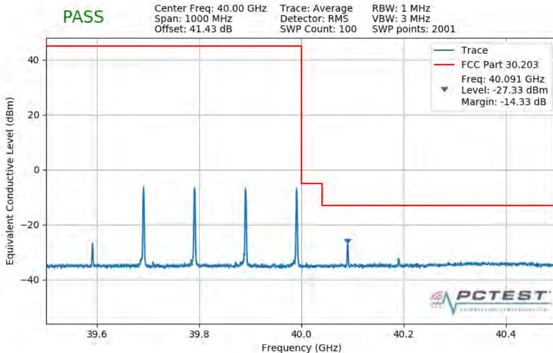
Plot 7-430. Upper Band Edge Plot (4CC 400MHz QPSK 1 RB)
