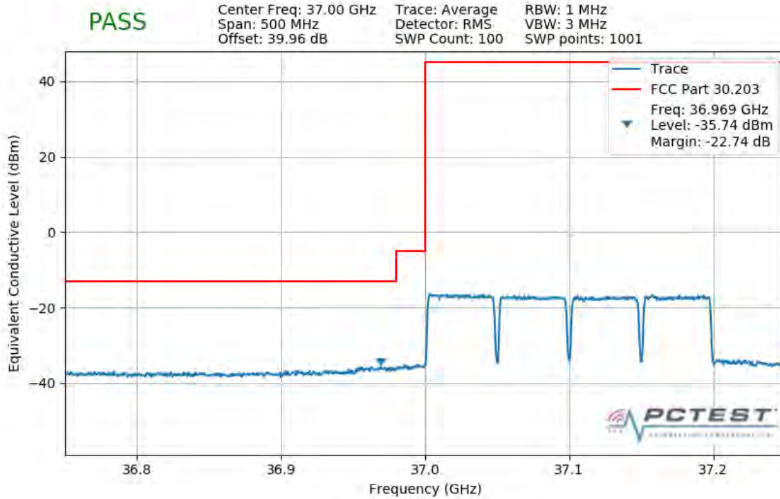
Plot 7-505. Lower Band Edge Plot (4CC 200MHz QPSK Full RB)
