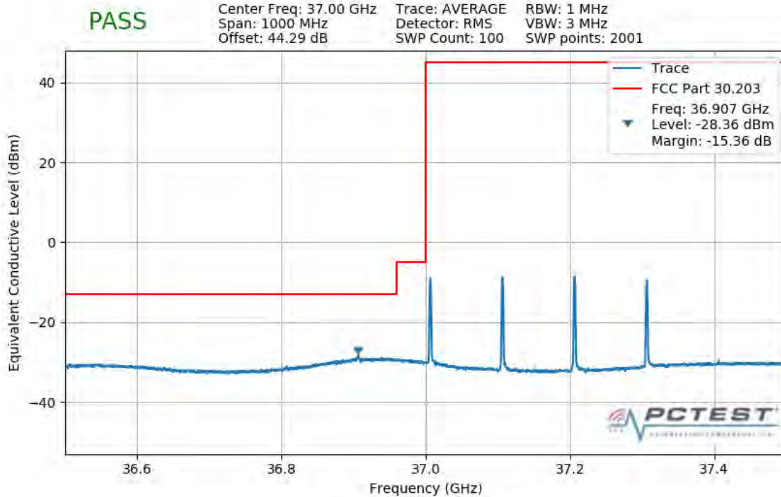
Plot 7-352. Lower Band Edge Plot (4CC 400MHz 64QAM 1 RB)
