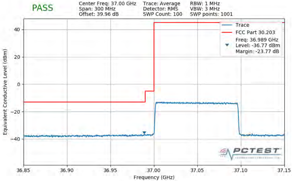
Plot 7-501. Lower Band Edge Plot (1CC 100MHz QPSK Full RB)
