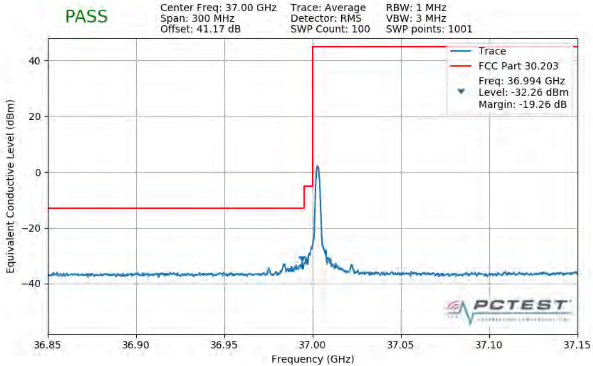
Plot 7-436. Lower Band Edge Plot (1CC 50MHz 64QAM 1 RB)
