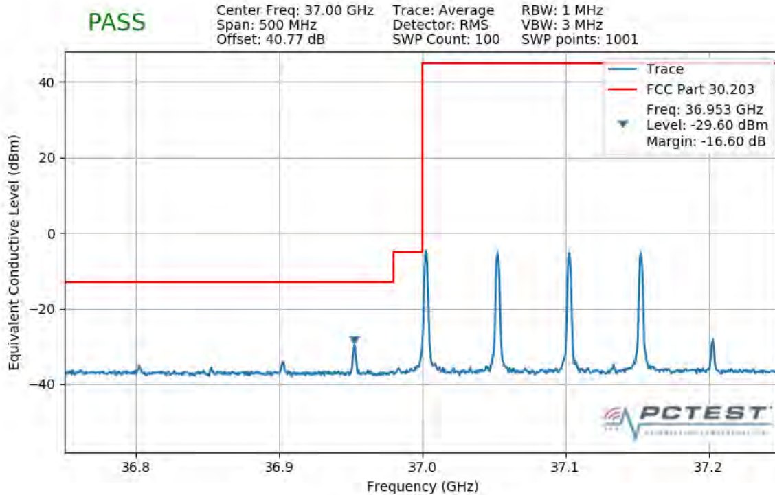
Plot 7-410. Lower Band Edge Plot (4CC 200MHz QPSK 1 RB)
