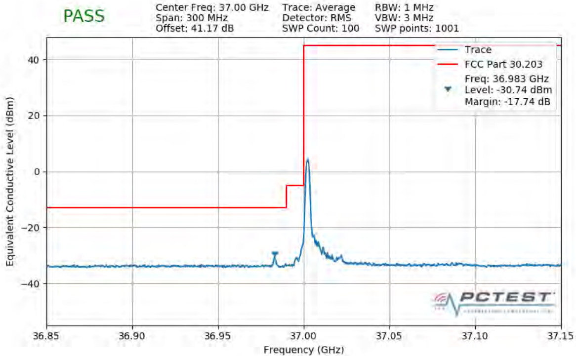
Plot 7-472. Lower Band Edge Plot (1CC 100MHz 64QAM 1 RB)
