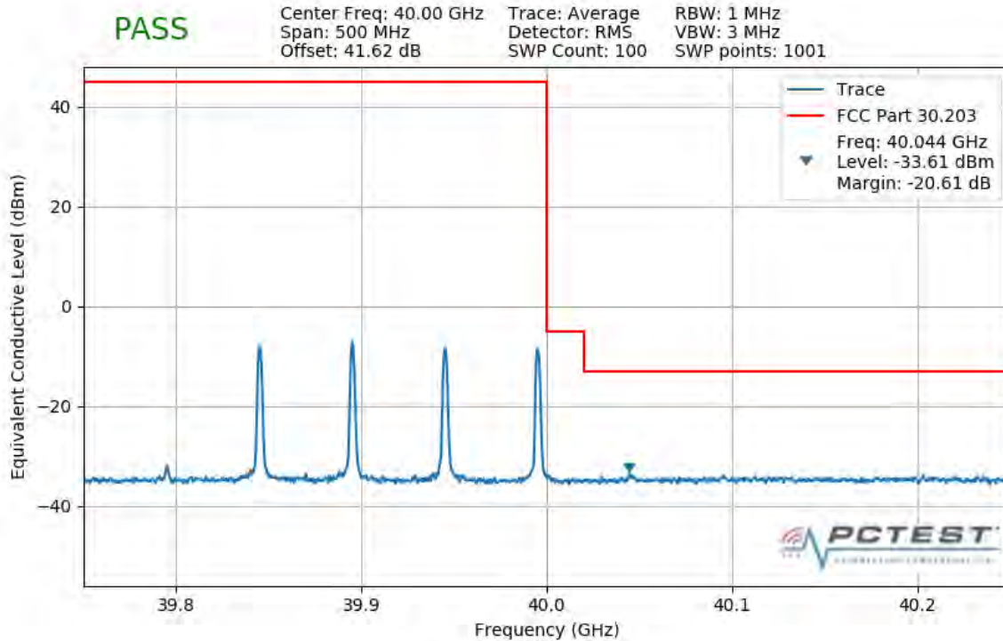
Plot 7-524. Upper Band Edge Plot (4CC 200MHz 64QAM 1 RB)
