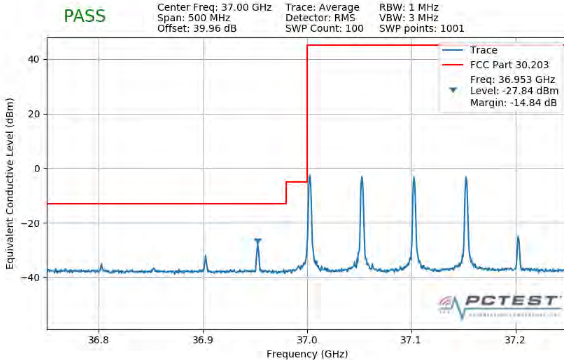
Plot 7-506. Lower Band Edge Plot (4CC 200MHz QPSK 1 RB)
