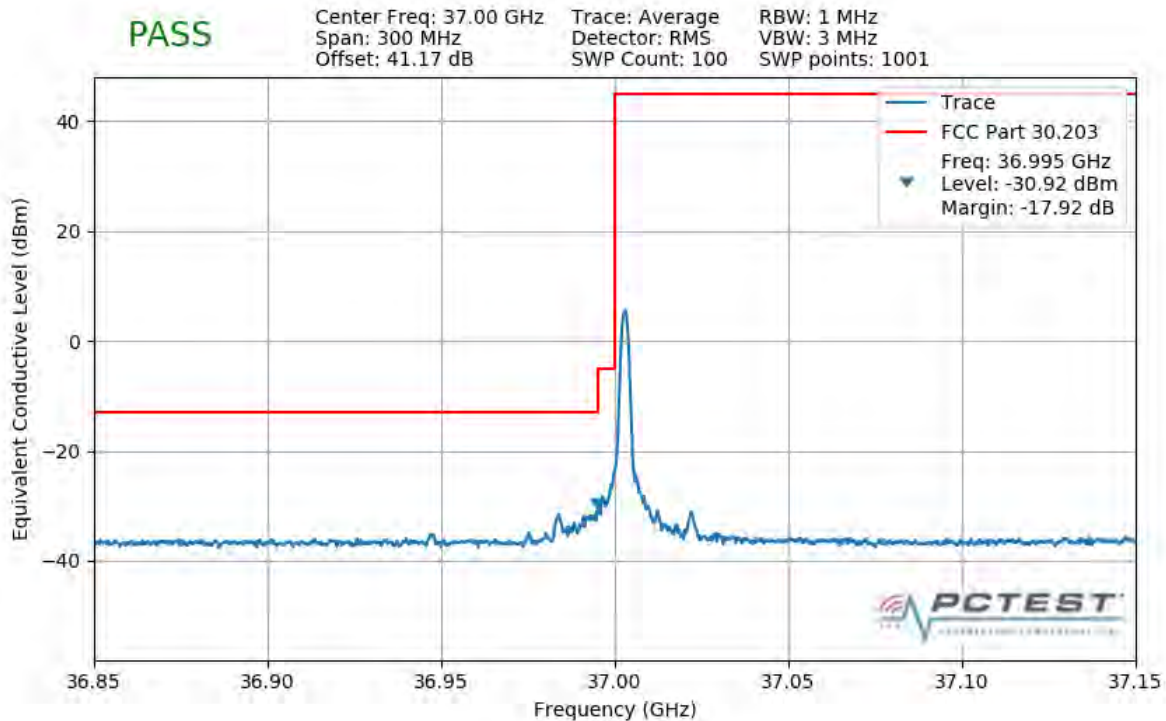
Plot 7-434. Lower Band Edge Plot (1CC 50MHz QPSK 1 RB)
