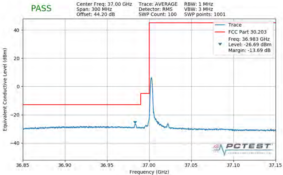
Plot 7-374. Lower Band Edge Plot (1CC 100MHz QPSK 1 RB)
