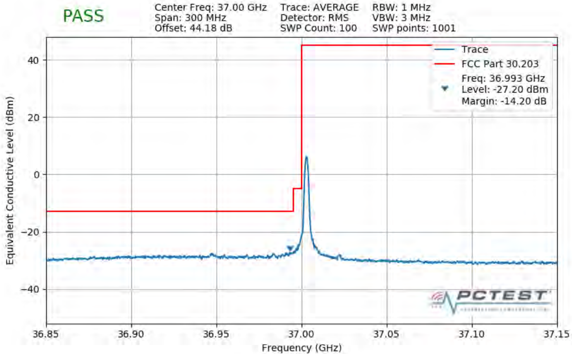
Plot 7-371. Lower Band Edge Plot (1CC 50MHz 16QAM 1 RB)
