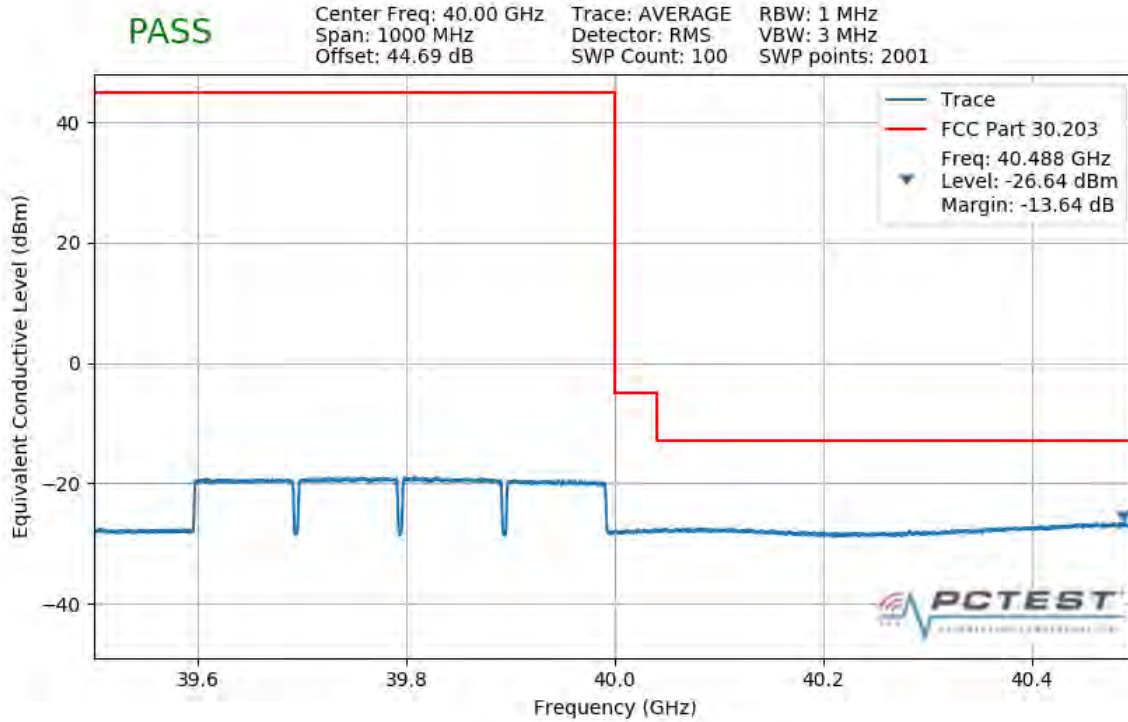
Plot 7-397. Upper Band Edge Plot (4CC 400MHz QPSK Full RB)
