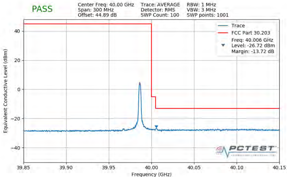
Plot 7-388. Upper Band Edge Plot (1CC 50MHz 64QAM 1 RB)
