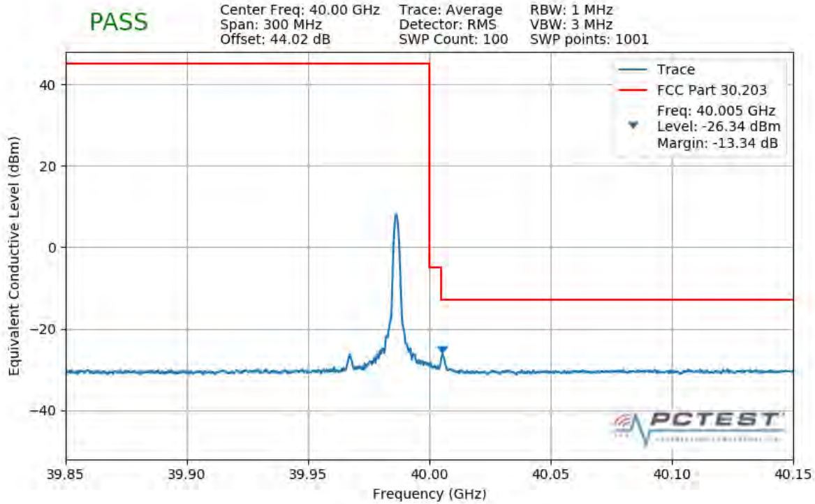
Plot 7-483. Upper Band Edge Plot (1CC 50MHz 16QAM 1 RB)
