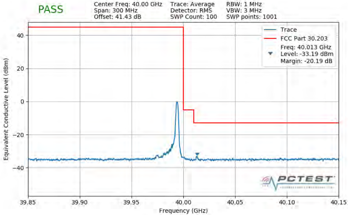
Plot 7-423. Upper Band Edge Plot (1CC 100MHz 16QAM 1 RB)
