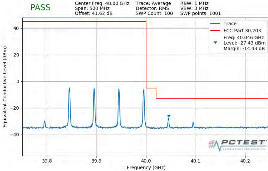
Plot 7-523. Upper Band Edge Plot (4CC 200MHz 16QAM 1 RB)
