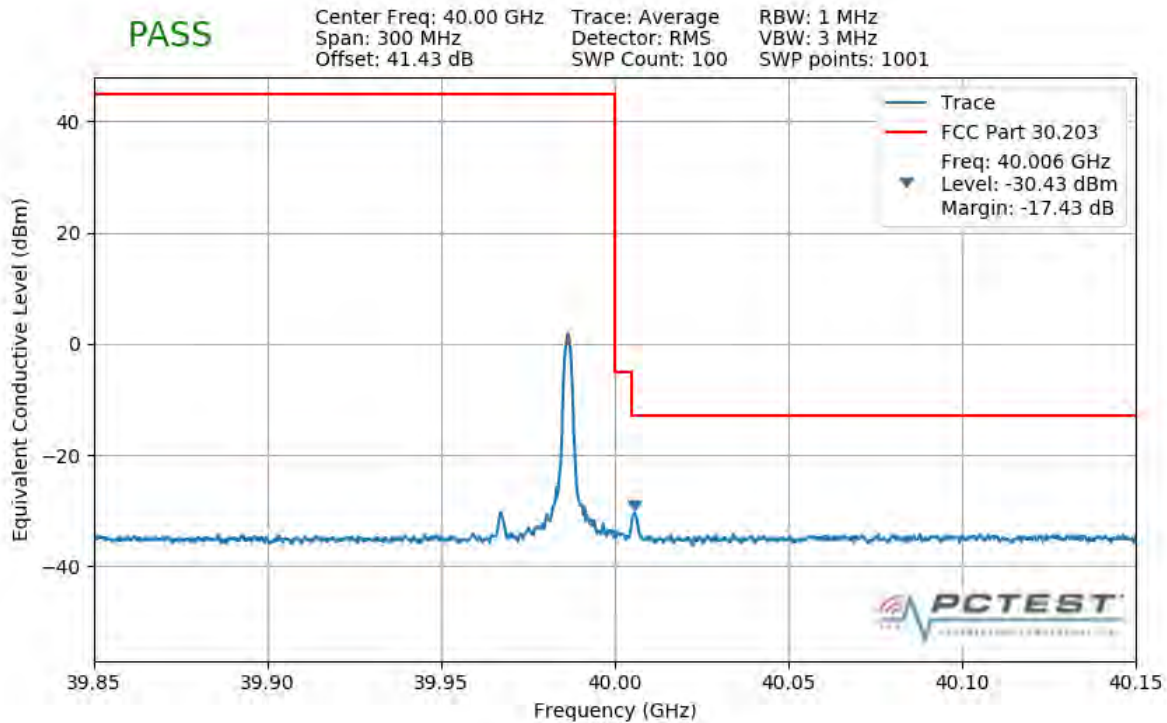
Plot 7-418. Upper Band Edge Plot (1CC 50MHz QPSK 1 RB)
