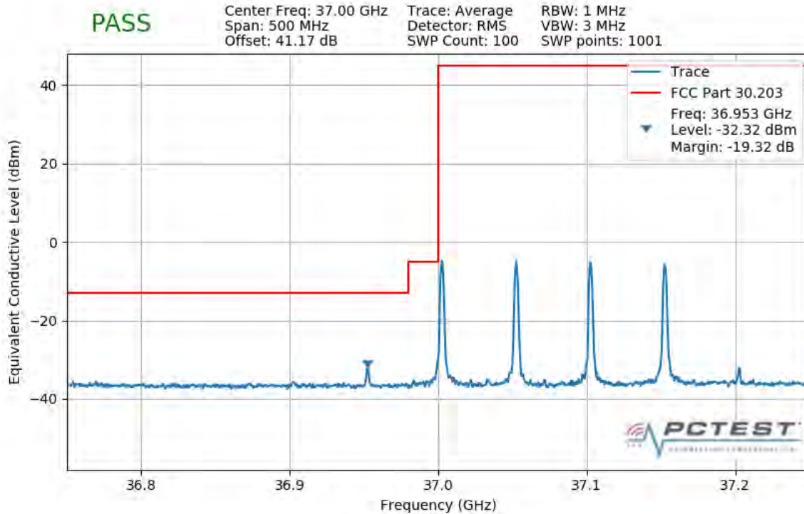
Plot 7-444. Lower Band Edge Plot (4CC 200MHz 64QAM 1 RB)
