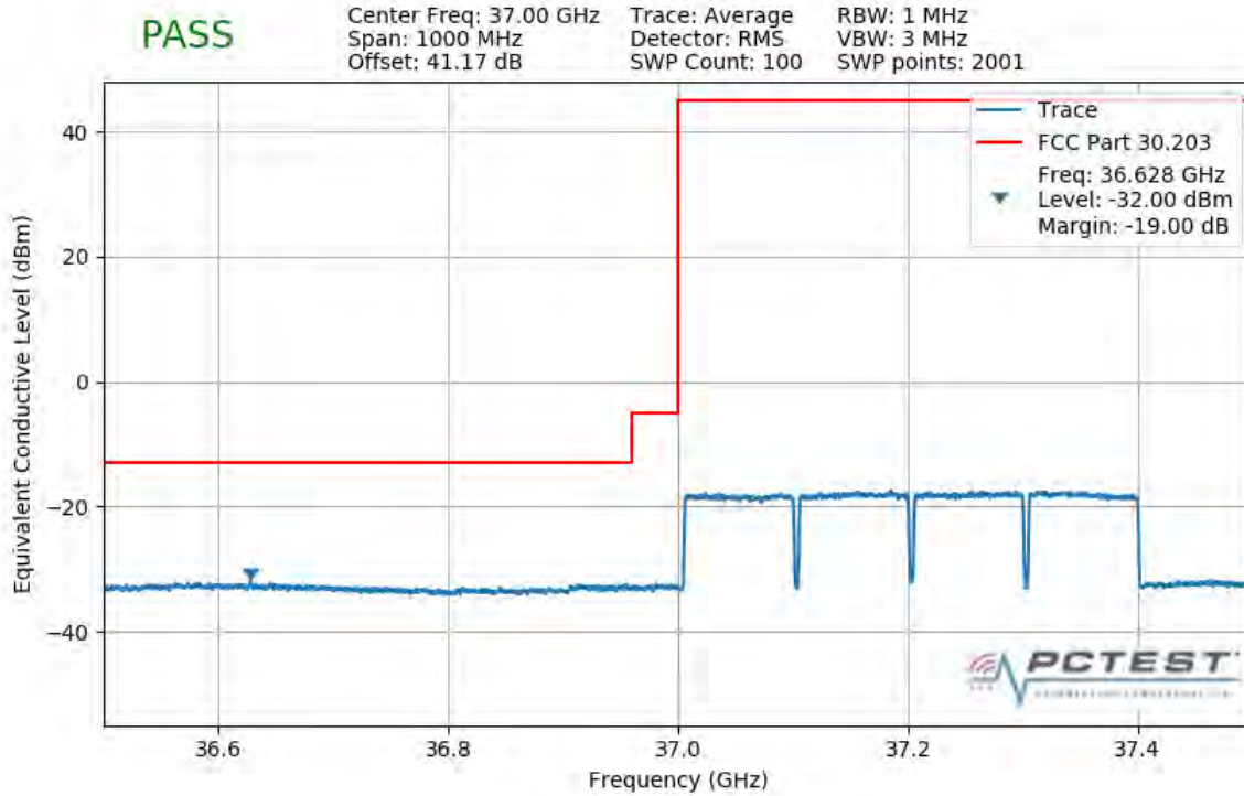
Plot 7-477. Lower Band Edge Plot (4CC 400MHz QPSK Full RB)
