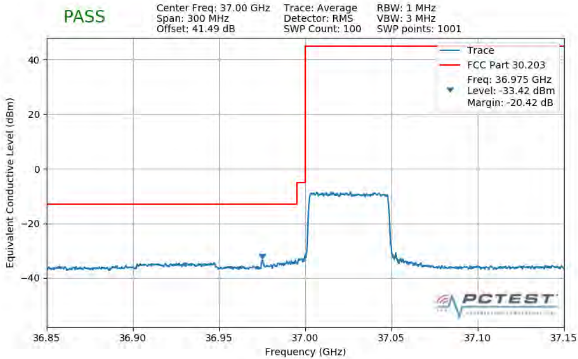
Plot 7-529. Lower Band Edge Plot (1CC 50MHz QPSK Full RB)
