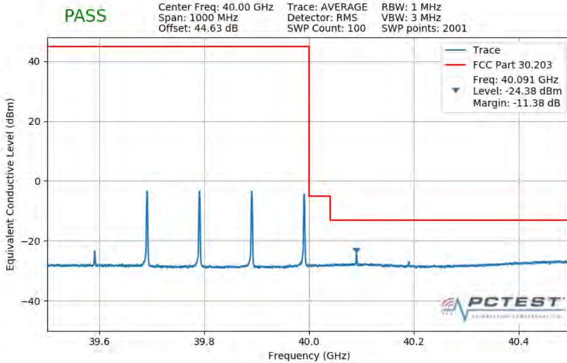
Plot 7-399. Upper Band Edge Plot (4CC 400MHz 16QAM 1 RB)
