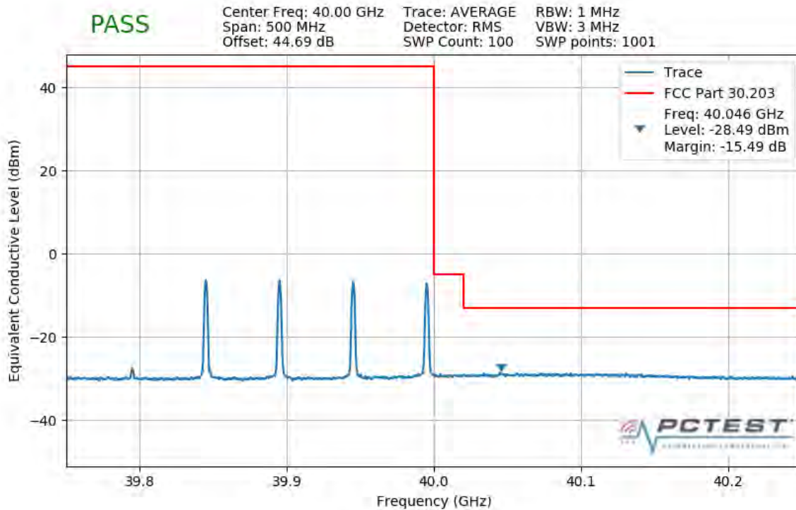
Plot 7-364. Upper Band Edge Plot (4CC 200MHz 64QAM 1 RB)
