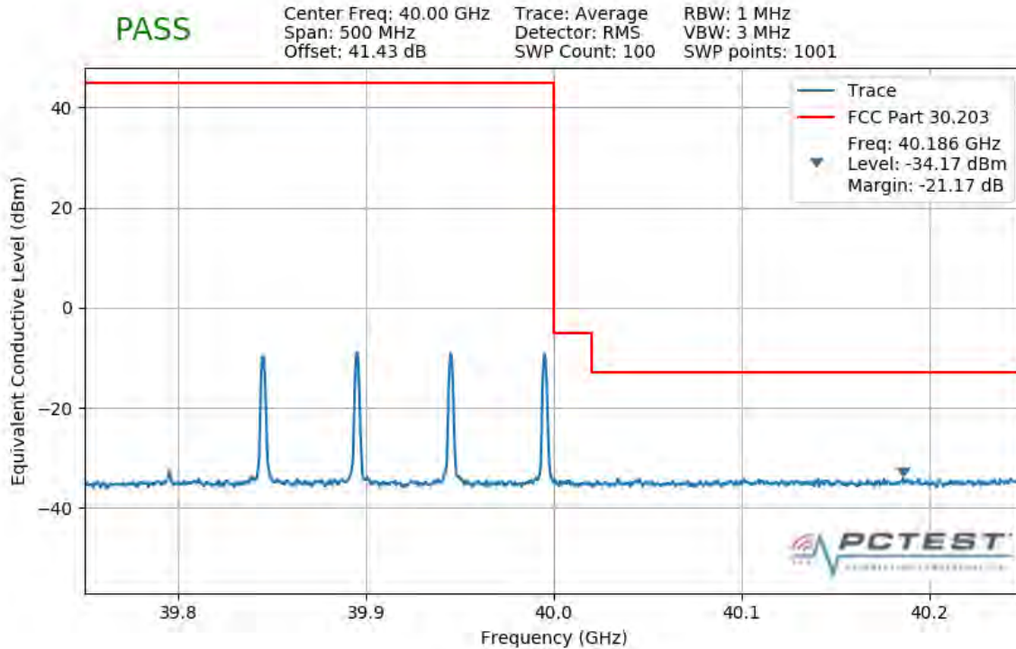
Plot 7-428. Upper Band Edge Plot (4CC 200MHz 64QAM 1 RB)
