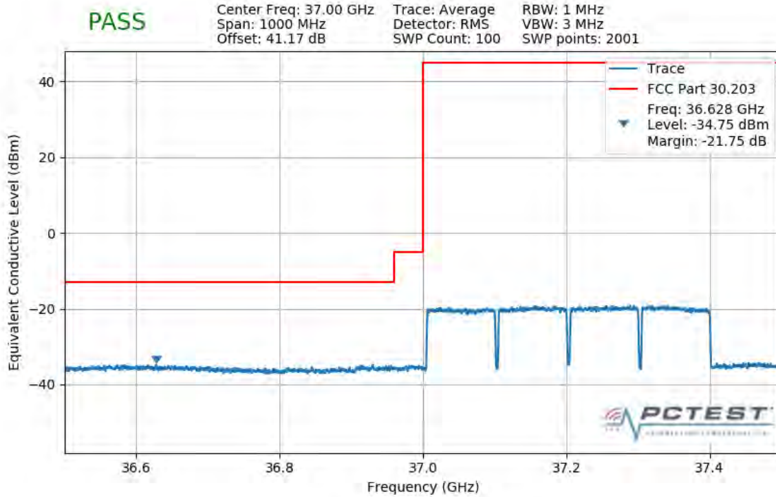
Plot 7-445. Lower Band Edge Plot (4CC 400MHz QPSK Full RB)
