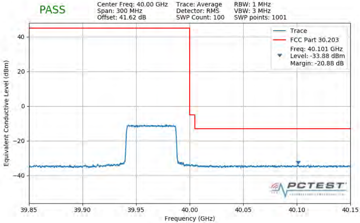
Plot 7-513. Upper Band Edge Plot (1CC 50MHz QPSK Full RB)
