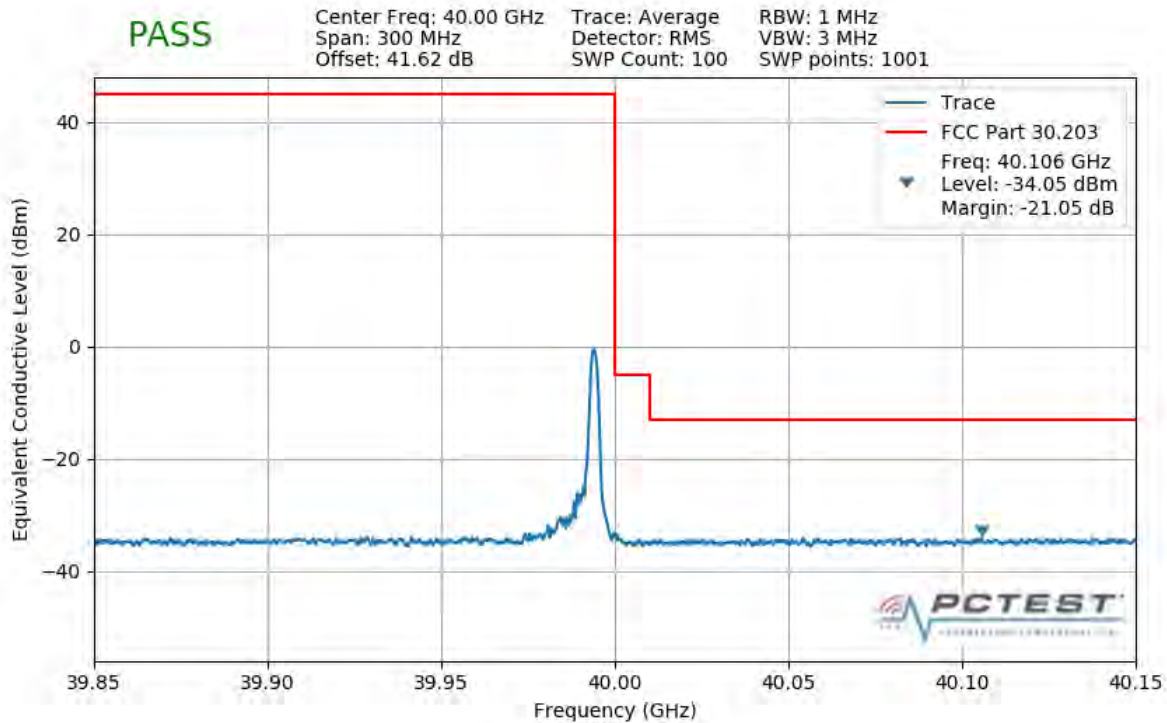
Plot 7-520. Upper Band Edge Plot (1CC 100MHz 64QAM 1 RB)
