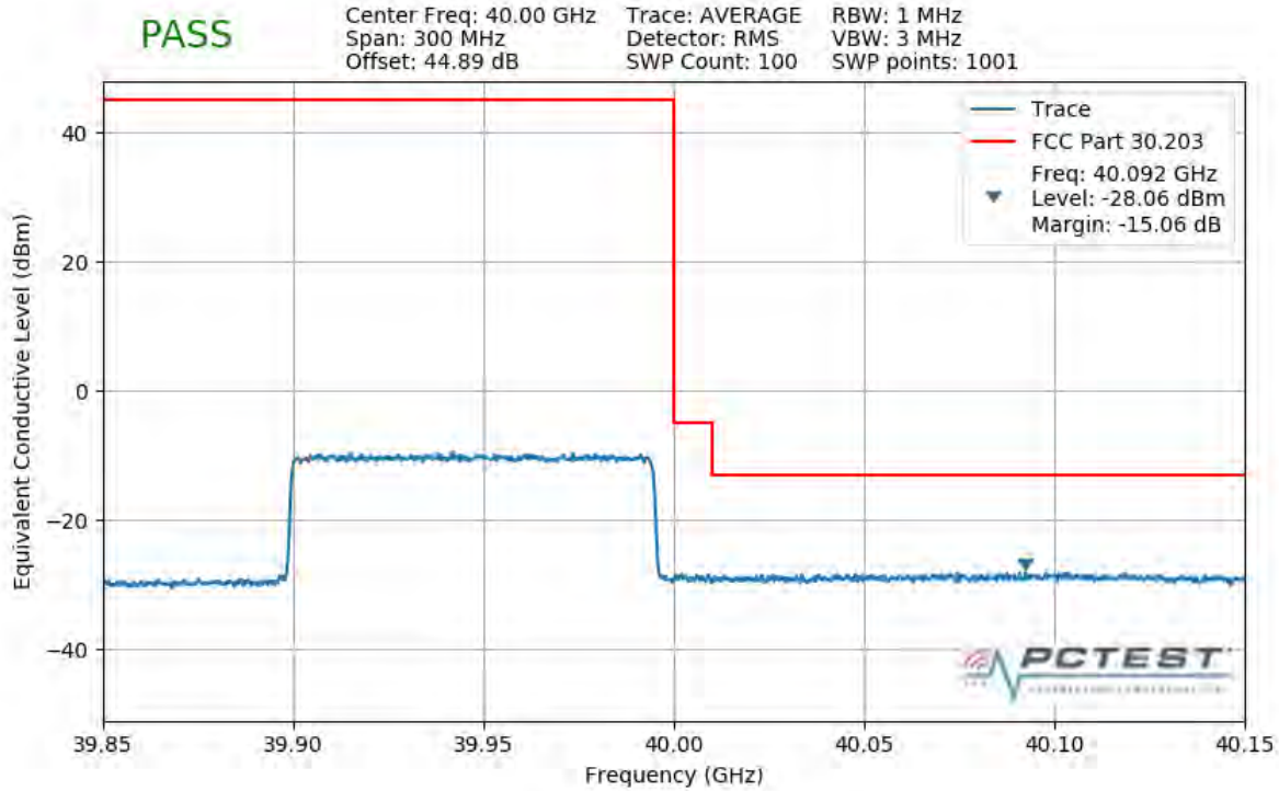
Plot 7-357. Upper Band Edge Plot (1CC 100MHz QPSK Full RB)
