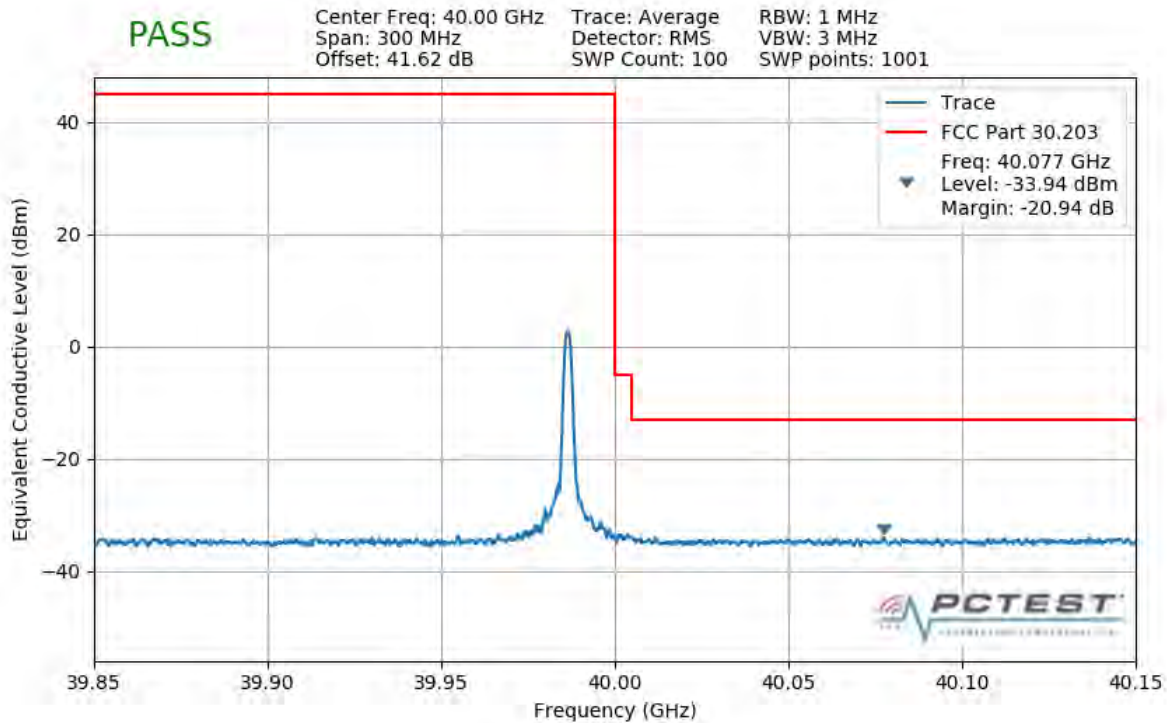
Plot 7-514. Upper Band Edge Plot (1CC 50MHz QPSK 1 RB)
