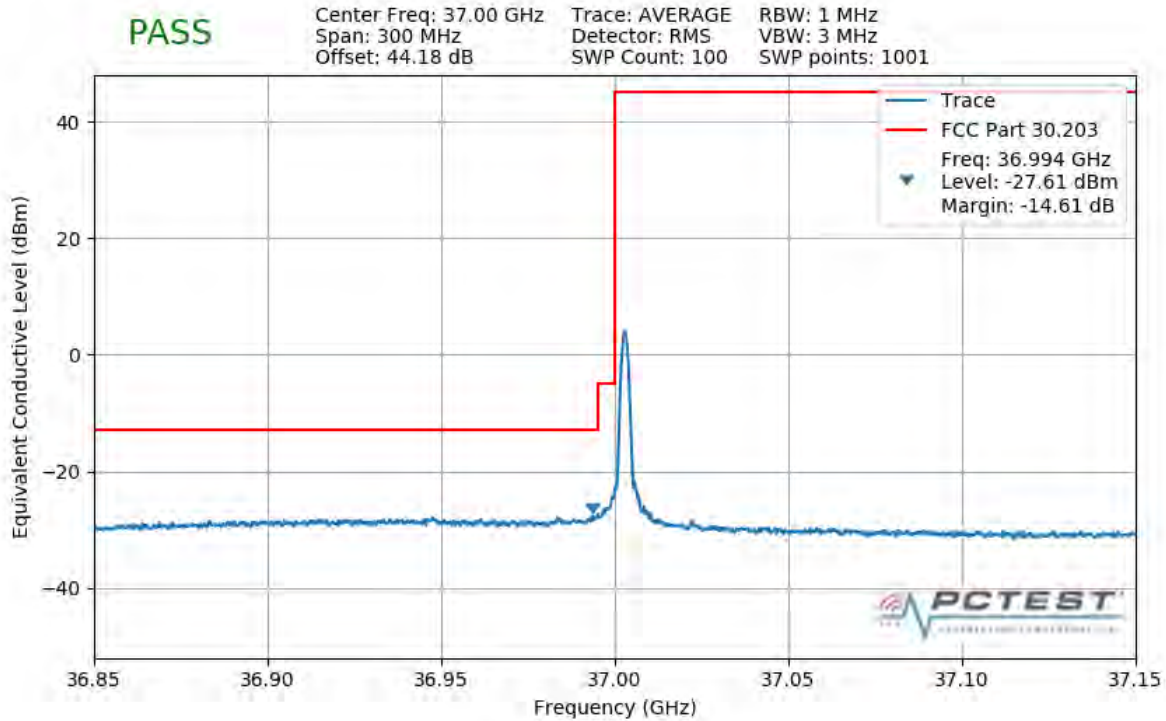
Plot 7-372. Lower Band Edge Plot (1CC 50MHz 64QAM 1 RB)
