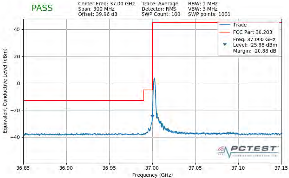
Plot 7-502. Lower Band Edge Plot (1CC 100MHz QPSK 1 RB)
