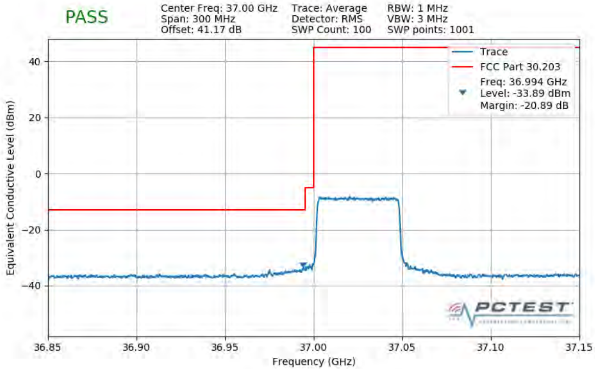
Plot 7-433. Lower Band Edge Plot (1CC 50MHz QPSK Full RB)
