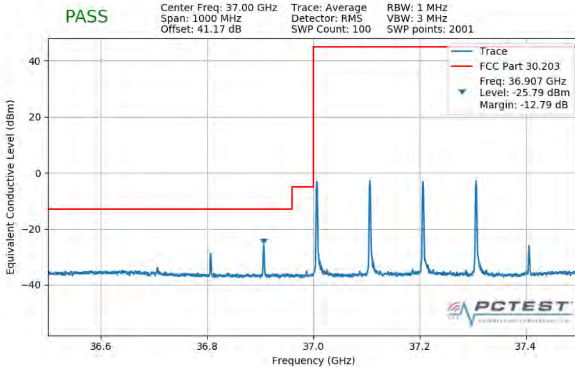
Plot 7-446. Lower Band Edge Plot (4CC 400MHz QPSK 1 RB)
