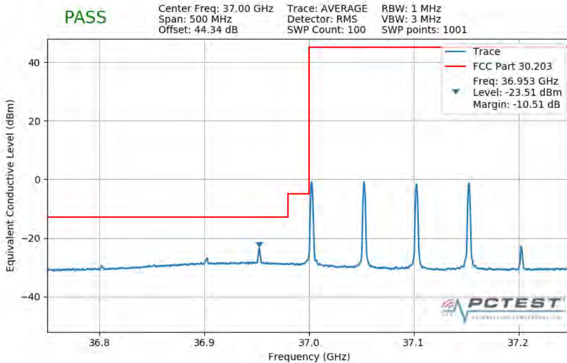
Plot 7-378. Lower Band Edge Plot (4CC 200MHz QPSK 1 RB)
