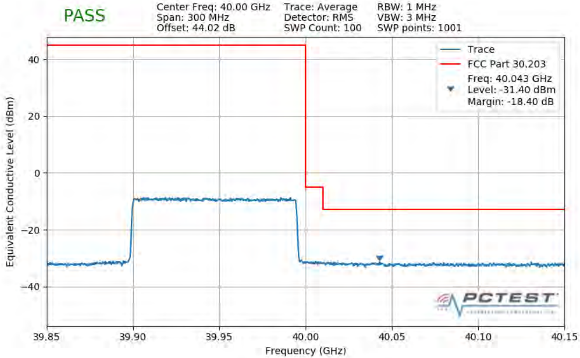
Plot 7-453. Upper Band Edge Plot (1CC 100MHz QPSK Full RB)
