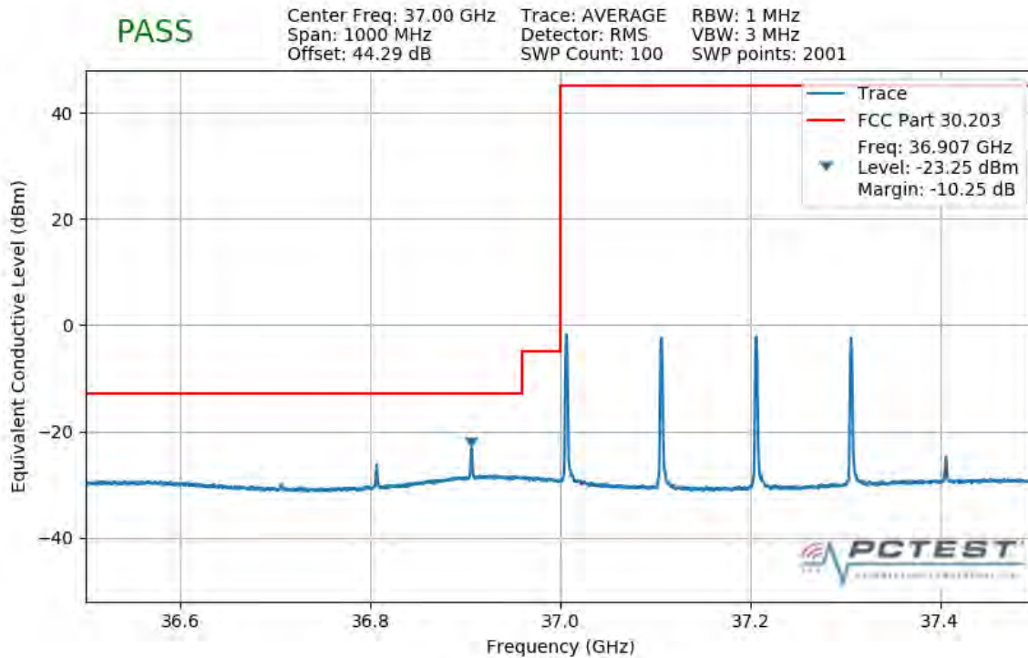
Plot 7-382. Lower Band Edge Plot (4CC 400MHz QPSK 1 RB)
