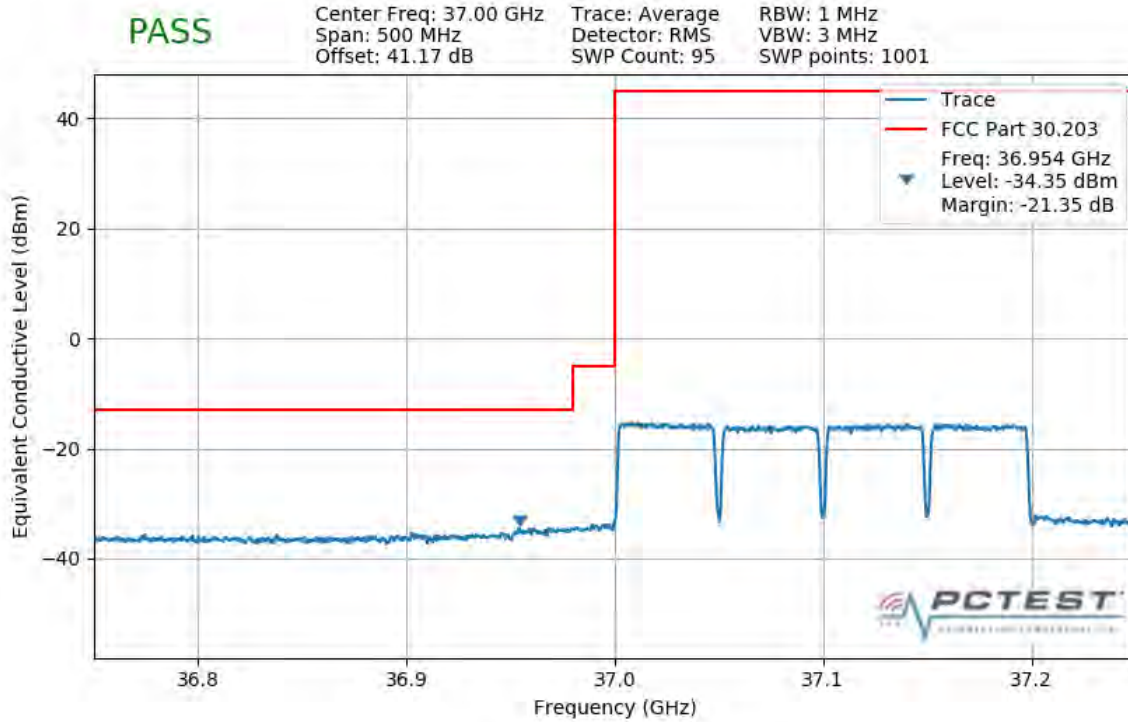
Plot 7-441. Lower Band Edge Plot (4CC 200MHz QPSK Full RB)
