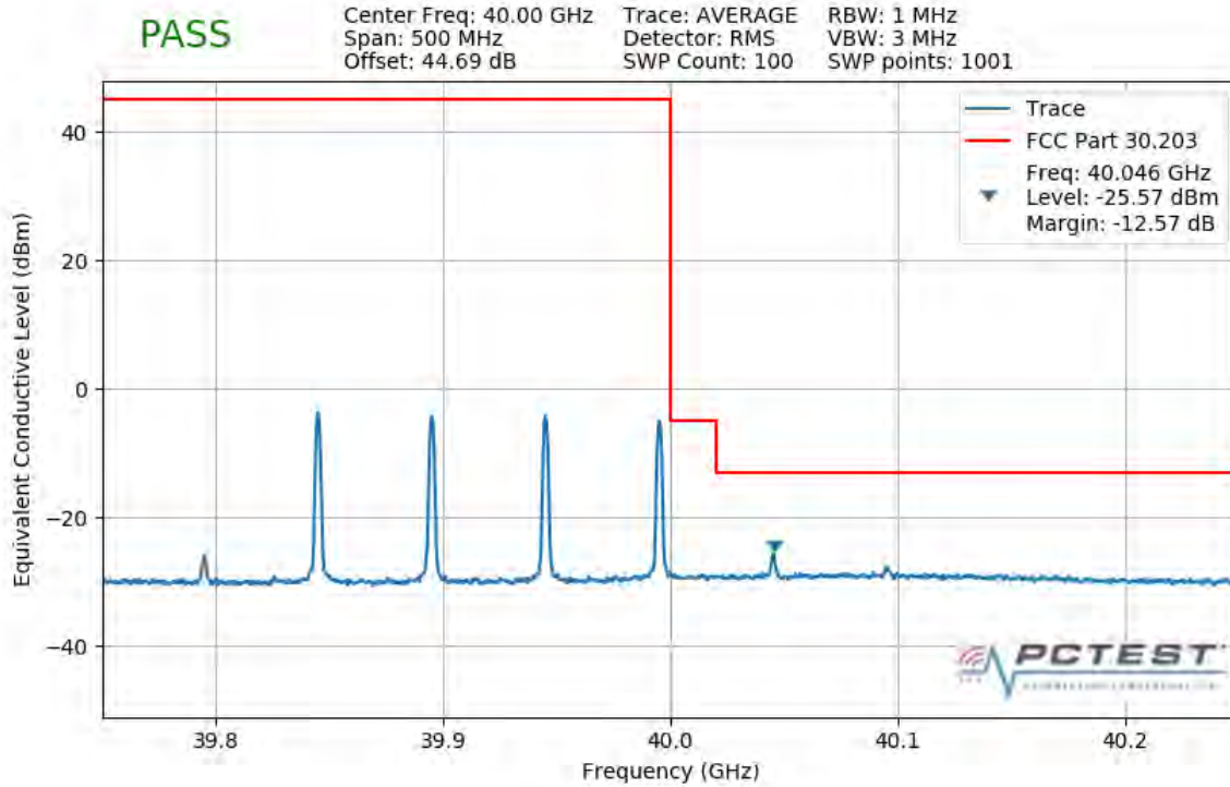
Plot 7-363. Upper Band Edge Plot (4CC 200MHz 16QAM 1 RB)
