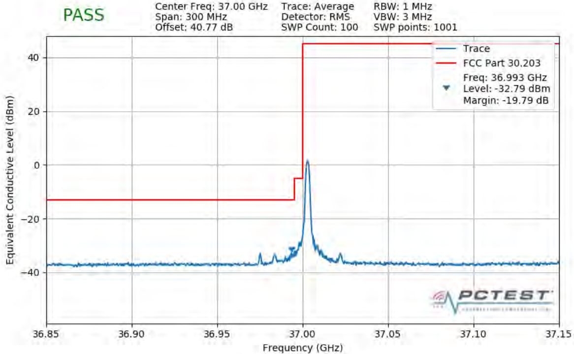
Plot 7-403. Lower Band Edge Plot (1CC 50MHz 16QAM 1 RB)
