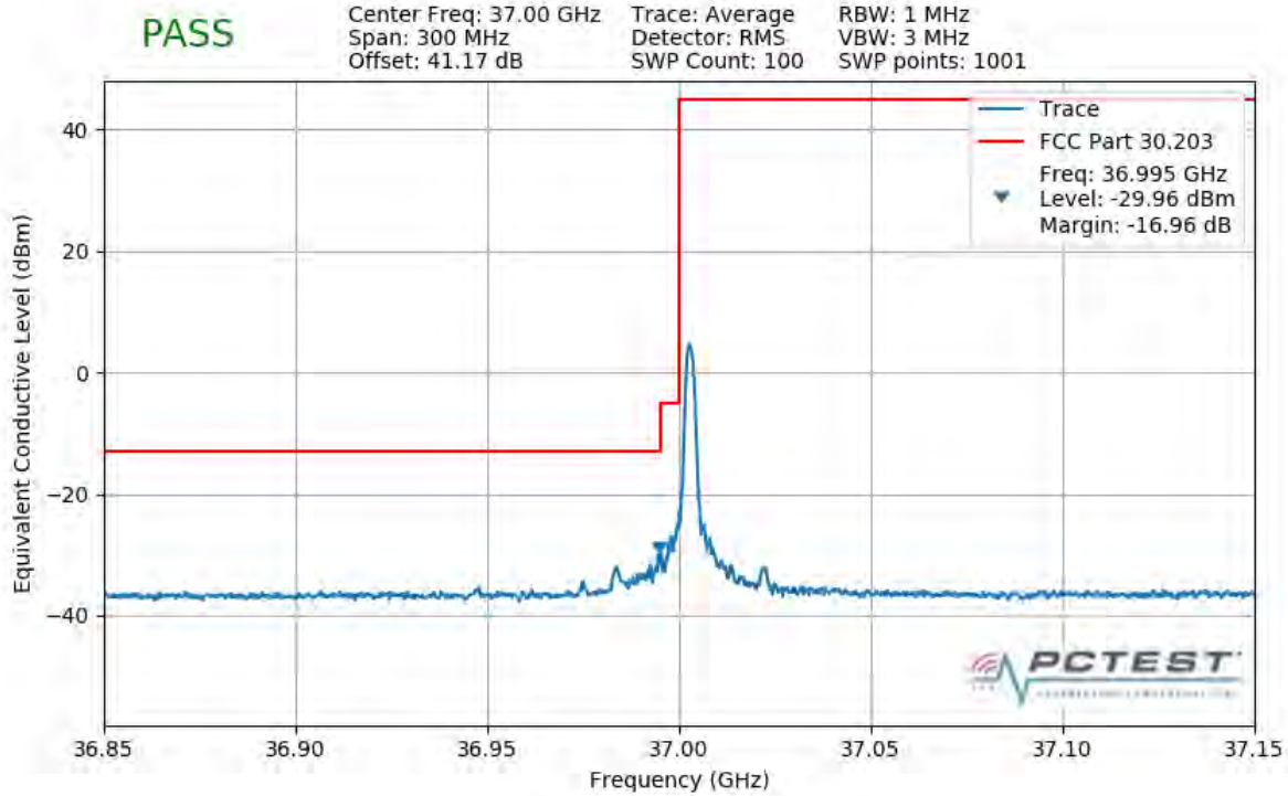
Plot 7-435. Lower Band Edge Plot (1CC 50MHz 16QAM 1 RB)
