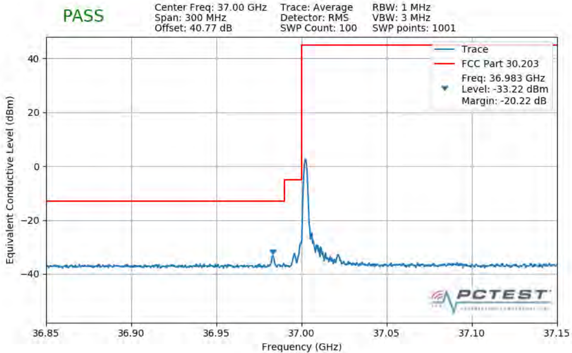
Plot 7-406. Lower Band Edge Plot (1CC 100MHz QPSK 1 RB)
