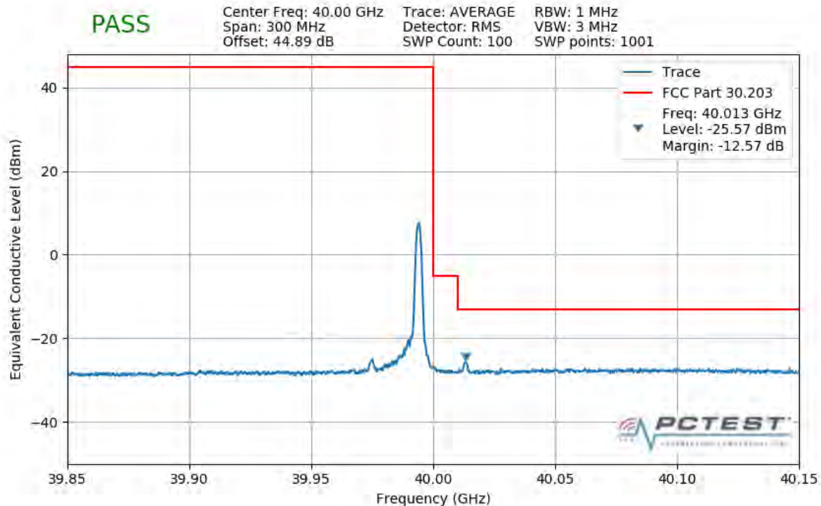
Plot 7-390. Upper Band Edge Plot (1CC 100MHz QPSK 1 RB)
