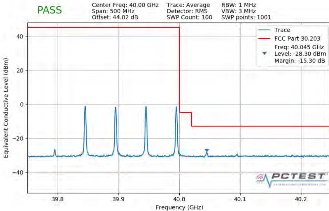
Plot 7-492. Upper Band Edge Plot (4CC 200MHz 64QAM 1 RB)
