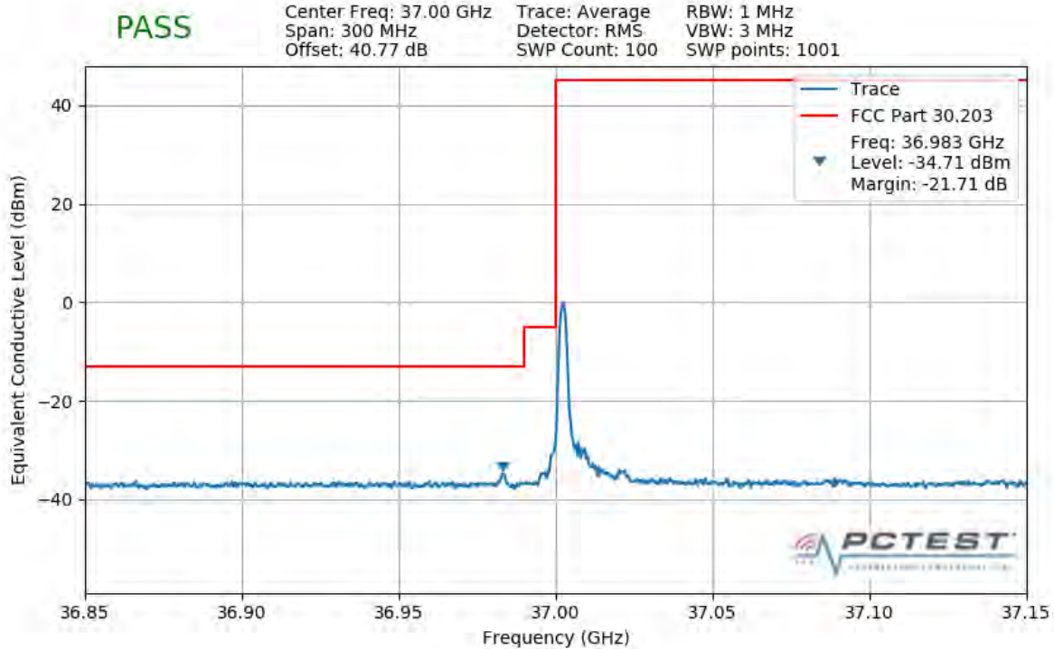
Plot 7-408. Lower Band Edge Plot (1CC 100MHz 64QAM 1 RB)
