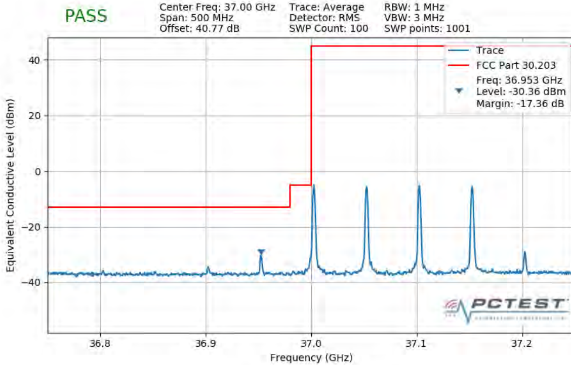
Plot 7-411. Lower Band Edge Plot (4CC 200MHz 16QAM 1 RB)
