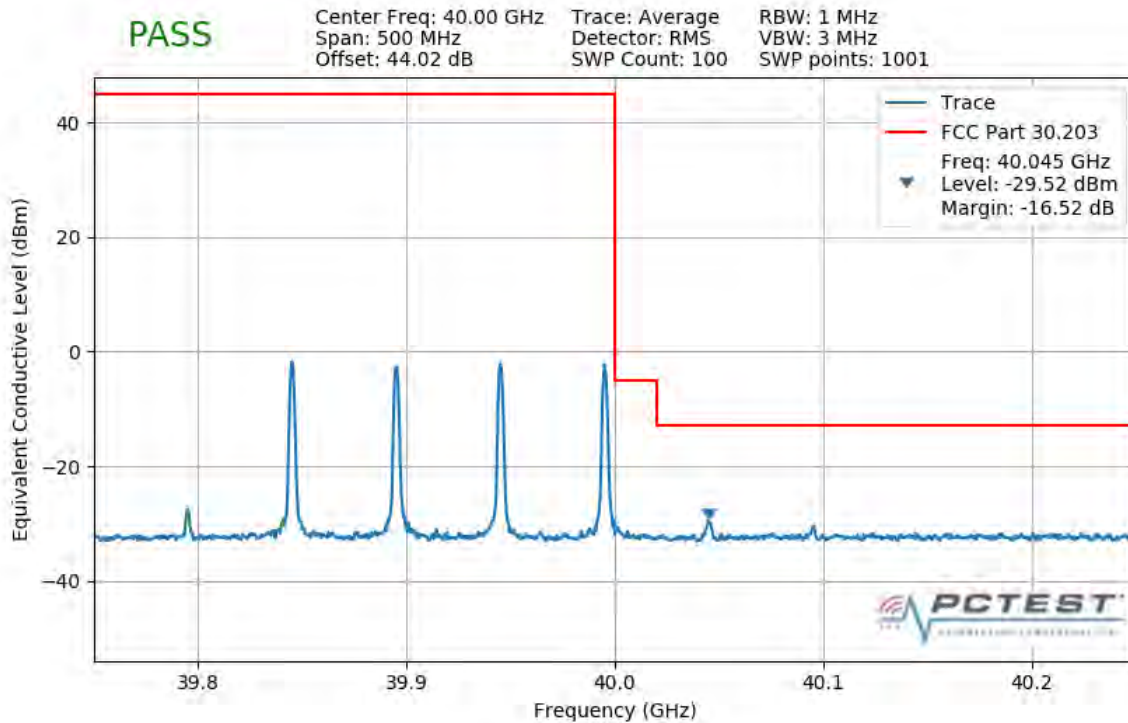
Plot 7-460. Upper Band Edge Plot (4CC 200MHz 64QAM 1 RB)
