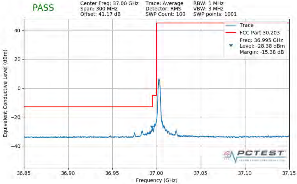
Plot 7-467. Lower Band Edge Plot (1CC 50MHz 16QAM 1 RB)
