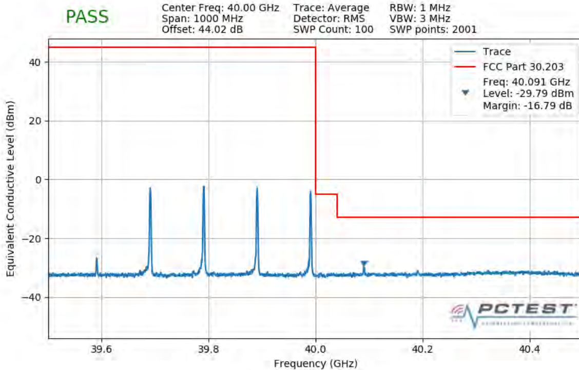
Plot 7-464. Upper Band Edge Plot (4CC 400MHz 64QAM 1 RB)
