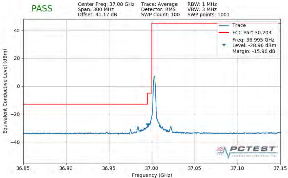
Plot 7-466. Lower Band Edge Plot (1CC 50MHz QPSK 1 RB)
