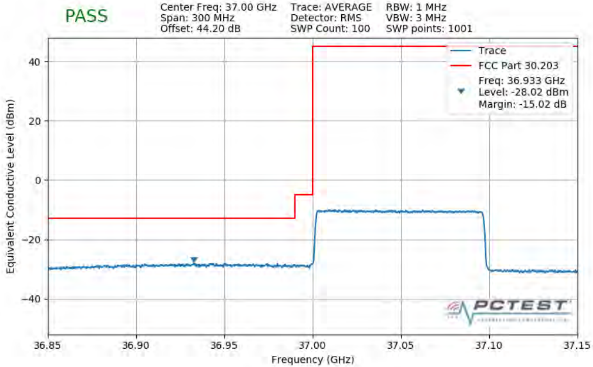
Plot 7-373. Lower Band Edge Plot (1CC 100MHz QPSK Full RB)
