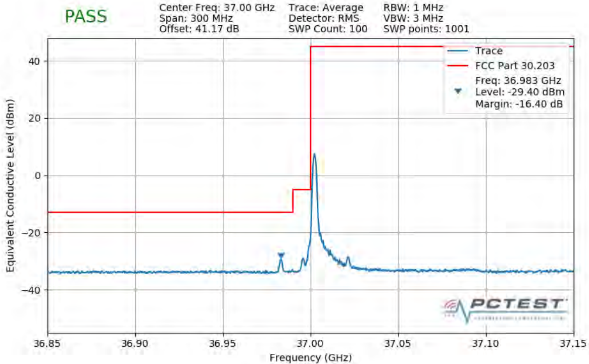
Plot 7-470. Lower Band Edge Plot (1CC 100MHz QPSK 1 RB)
