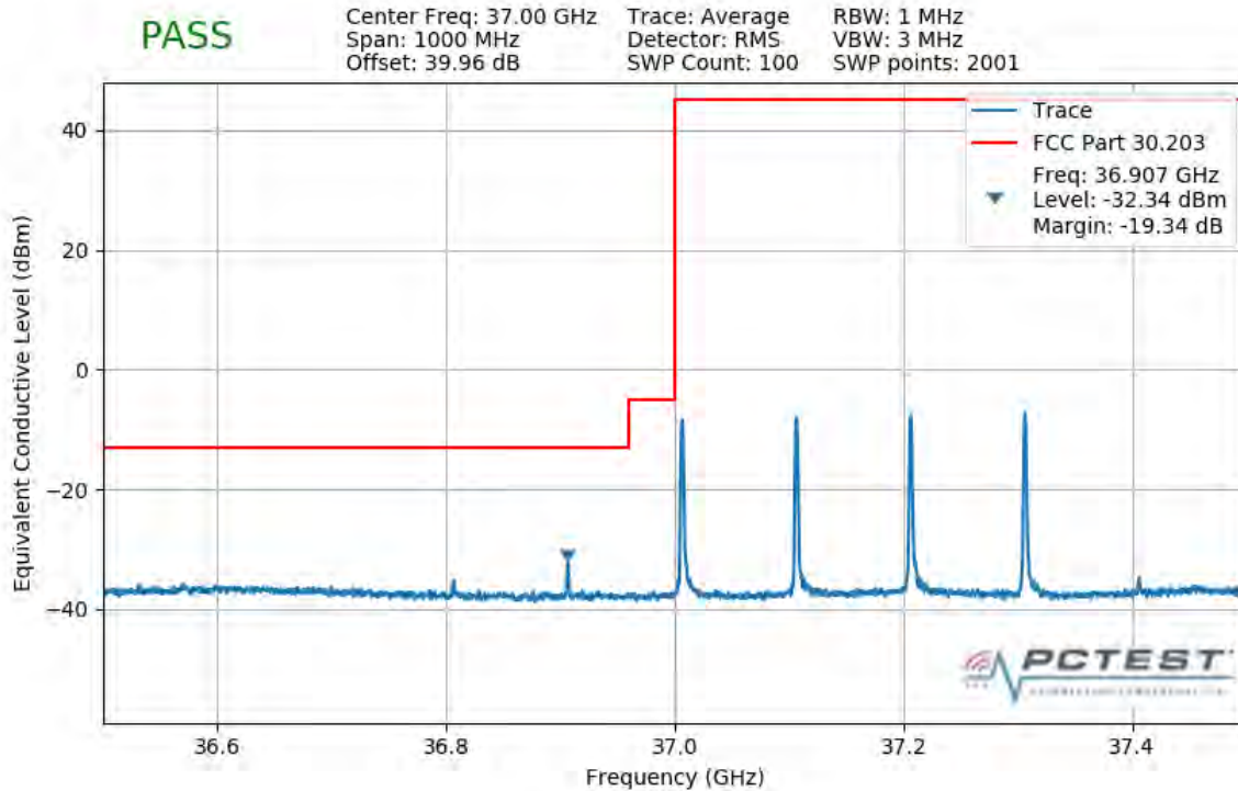
Plot 7-512. Lower Band Edge Plot (4CC 400MHz 64QAM 1 RB)
