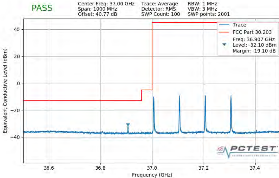
Plot 7-416. Lower Band Edge Plot (4CC 400MHz 64QAM 1 RB)
