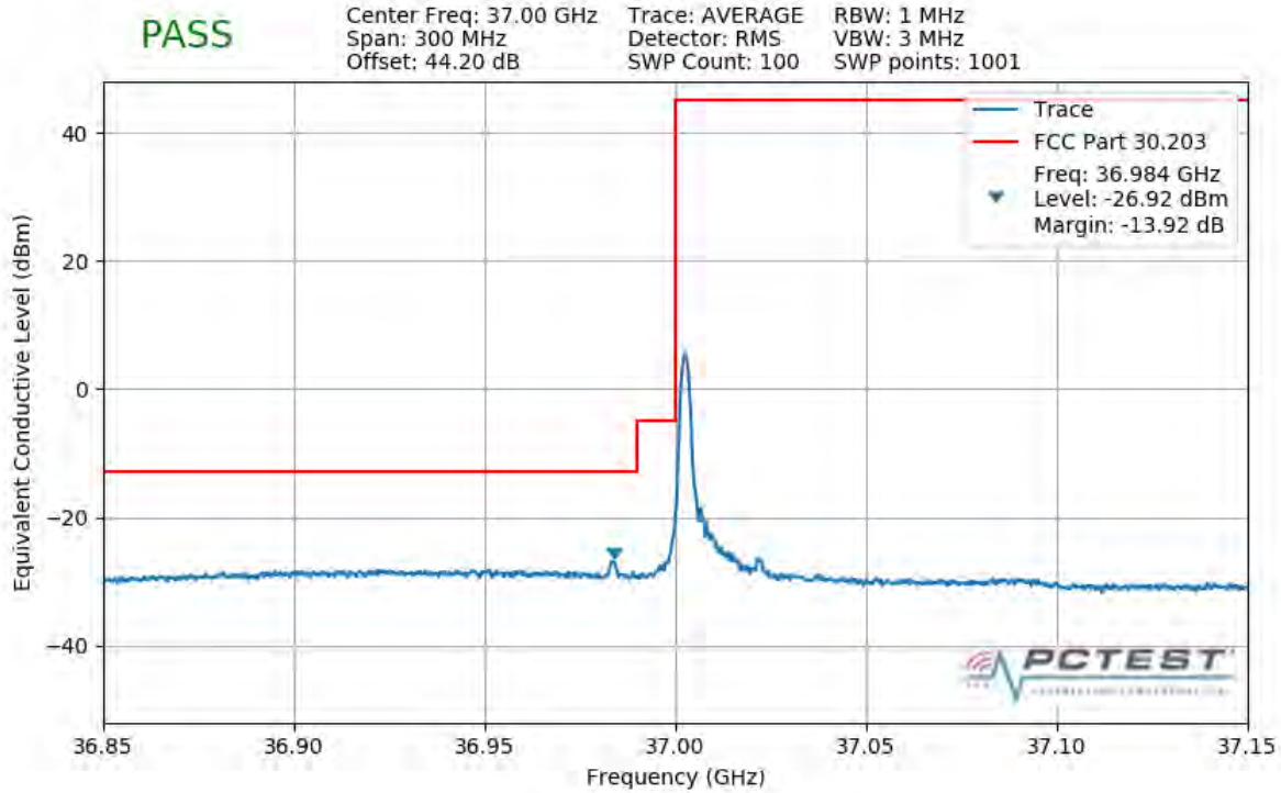
Plot 7-375. Lower Band Edge Plot (1CC 100MHz 16QAM 1 RB)
