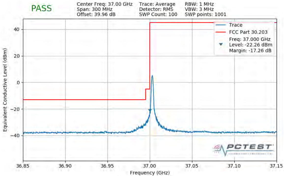
Plot 7-498. Lower Band Edge Plot (1CC 50MHz QPSK 1 RB)
