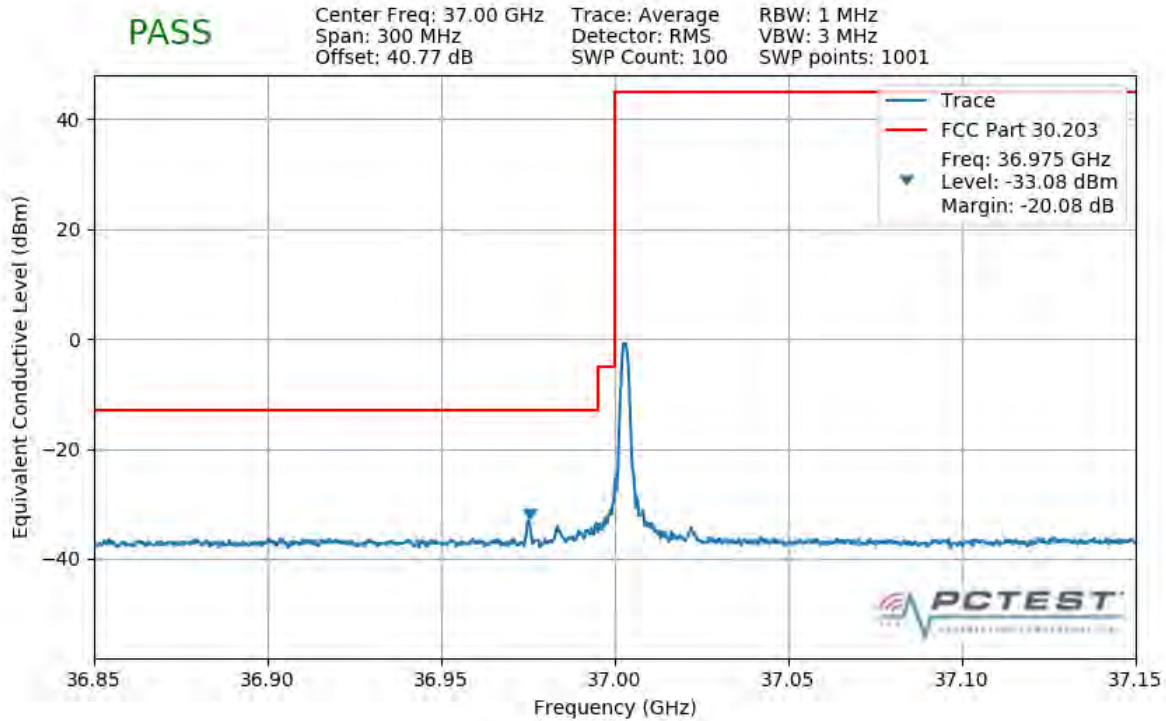
Plot 7-404. Lower Band Edge Plot (1CC 50MHz 64QAM 1 RB)
