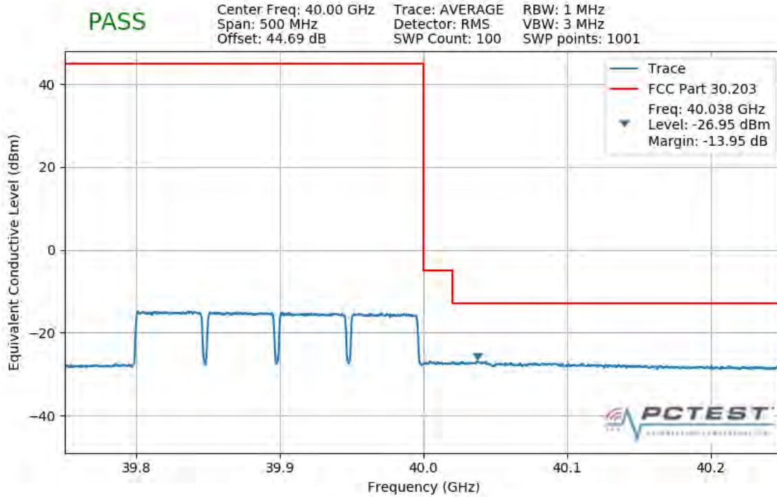
Plot 7-393. Upper Band Edge Plot (4CC 200MHz QPSK Full RB)
