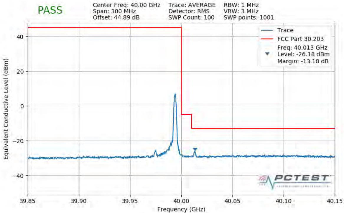
Plot 7-358. Upper Band Edge Plot (1CC 100MHz QPSK 1 RB)
