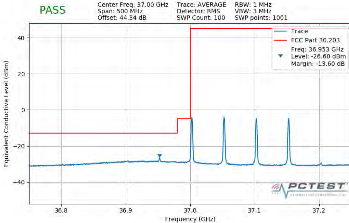
Plot 7-380. Lower Band Edge Plot (4CC 200MHz 64QAM 1 RB)
