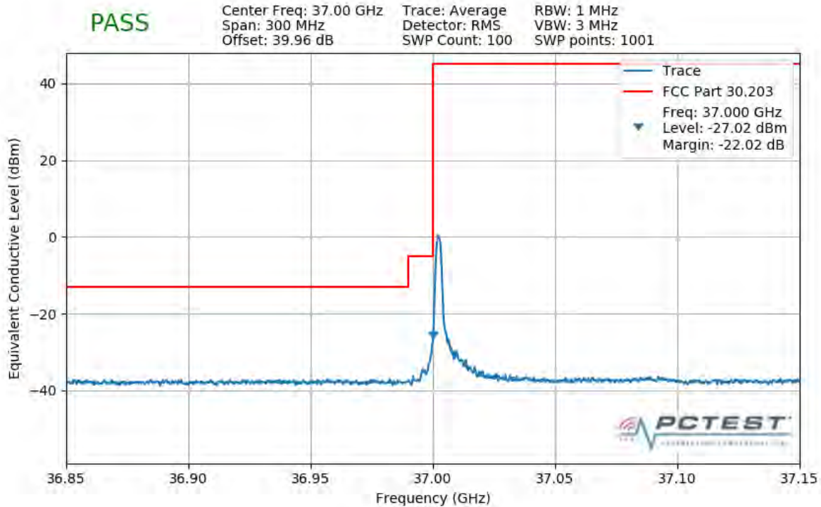
Plot 7-504. Lower Band Edge Plot (1CC 100MHz 64QAM 1 RB)
