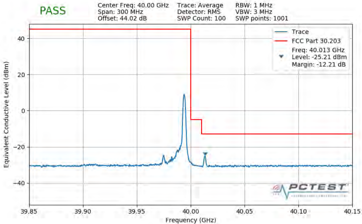
Plot 7-486. Upper Band Edge Plot (1CC 100MHz QPSK 1 RB)
