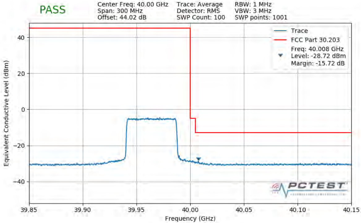
Plot 7-481. Upper Band Edge Plot (1CC 50MHz QPSK Full RB)
