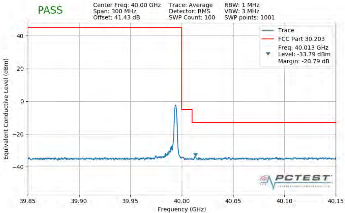
Plot 7-424. Upper Band Edge Plot (1CC 100MHz 64QAM 1 RB)
