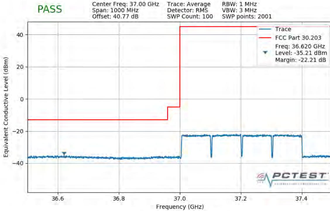
Plot 7-413. Lower Band Edge Plot (4CC 400MHz QPSK Full RB)
