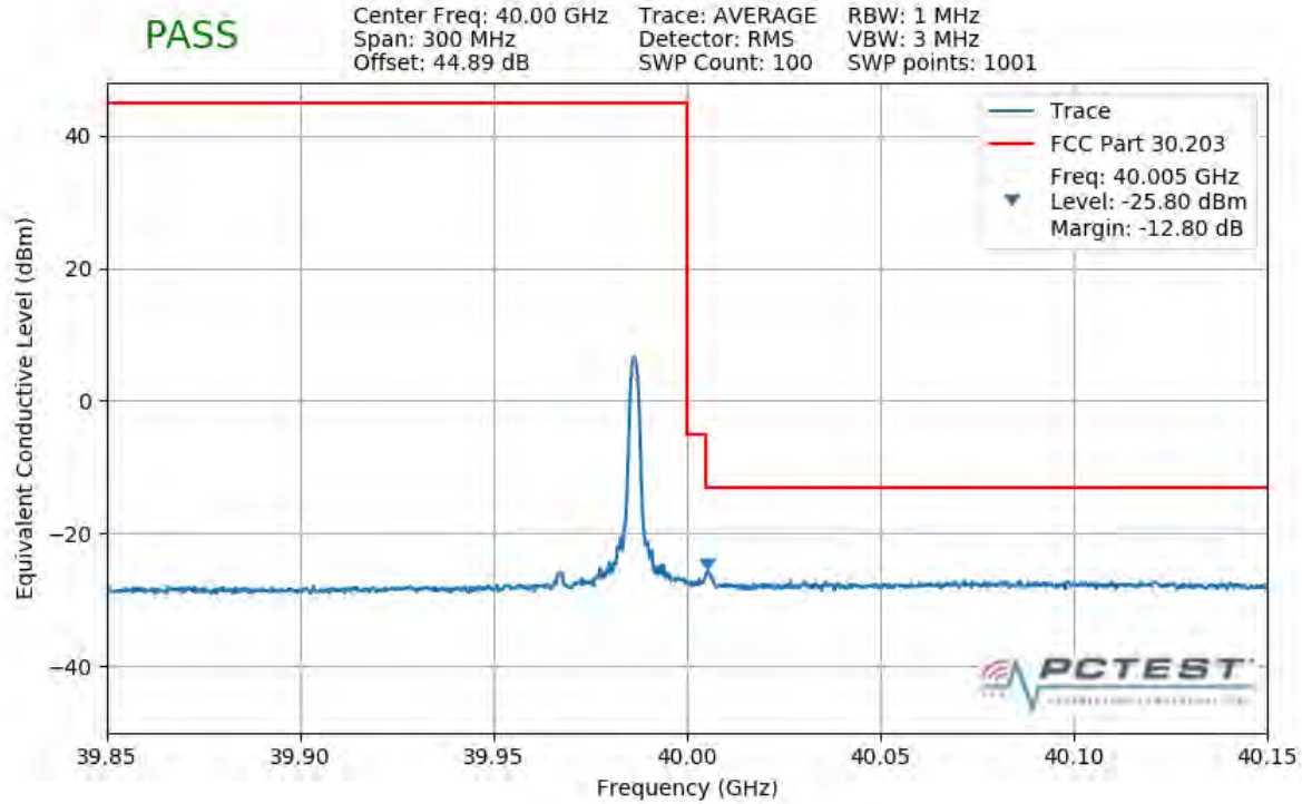
Plot 7-387. Upper Band Edge Plot (1CC 50MHz 16QAM 1 RB)
