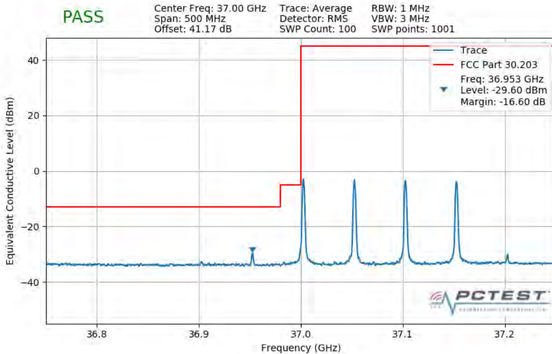
Plot 7-476. Lower Band Edge Plot (4CC 200MHz 64QAM 1 RB)
