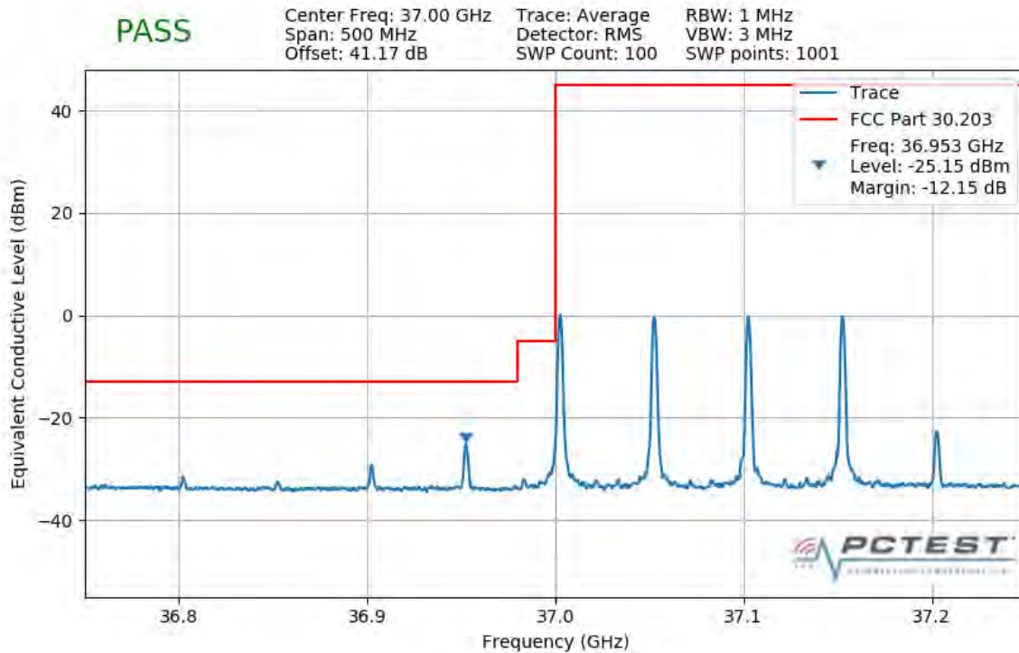
Plot 7-474. Lower Band Edge Plot (4CC 200MHz QPSK 1 RB)
