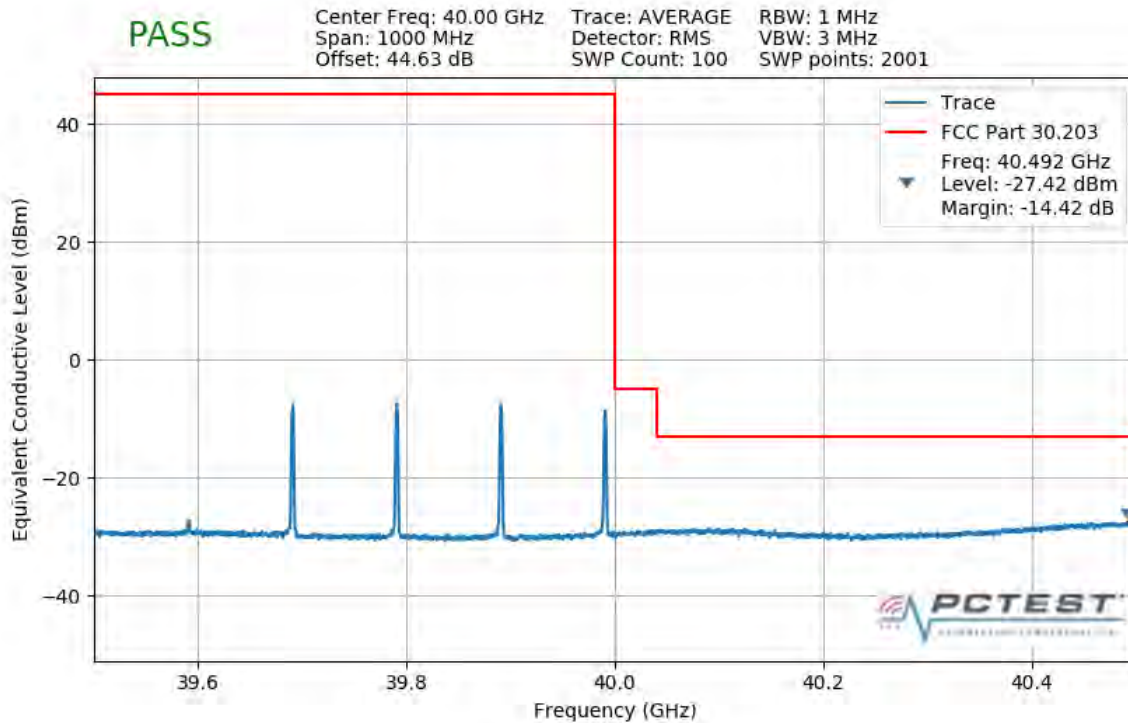
Plot 7-368. Upper Band Edge Plot (4CC 400MHz 64QAM 1 RB)
