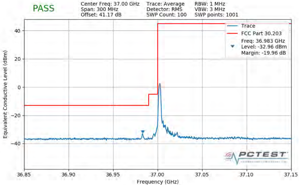
Plot 7-440. Lower Band Edge Plot (1CC 100MHz 64QAM 1 RB)
