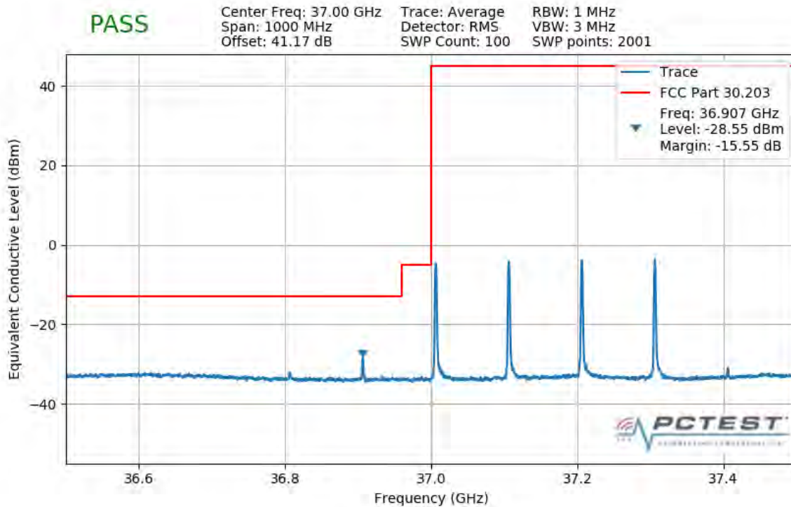
Plot 7-480. Lower Band Edge Plot (4CC 400MHz 64QAM 1 RB)
