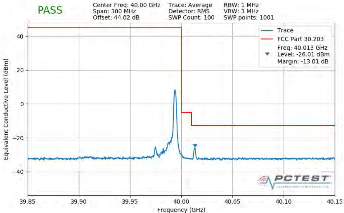
Plot 7-454. Upper Band Edge Plot (1CC 100MHz QPSK 1 RB)
