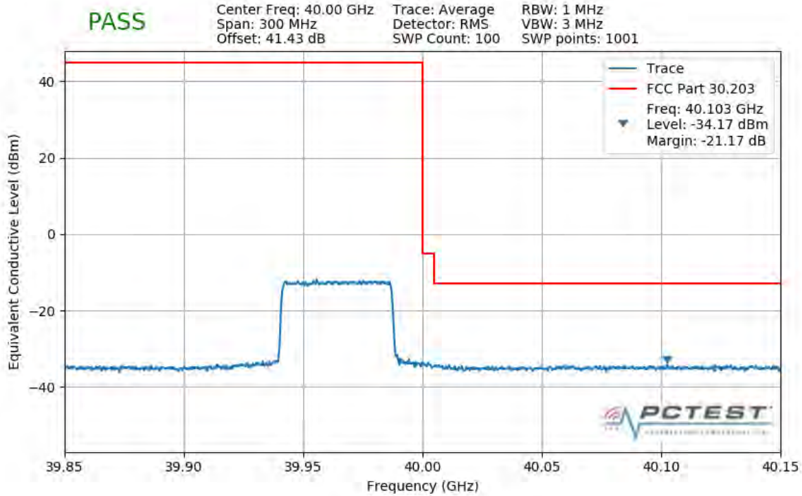
Plot 7-417. Upper Band Edge Plot (1CC 50MHz QPSK Full RB)
