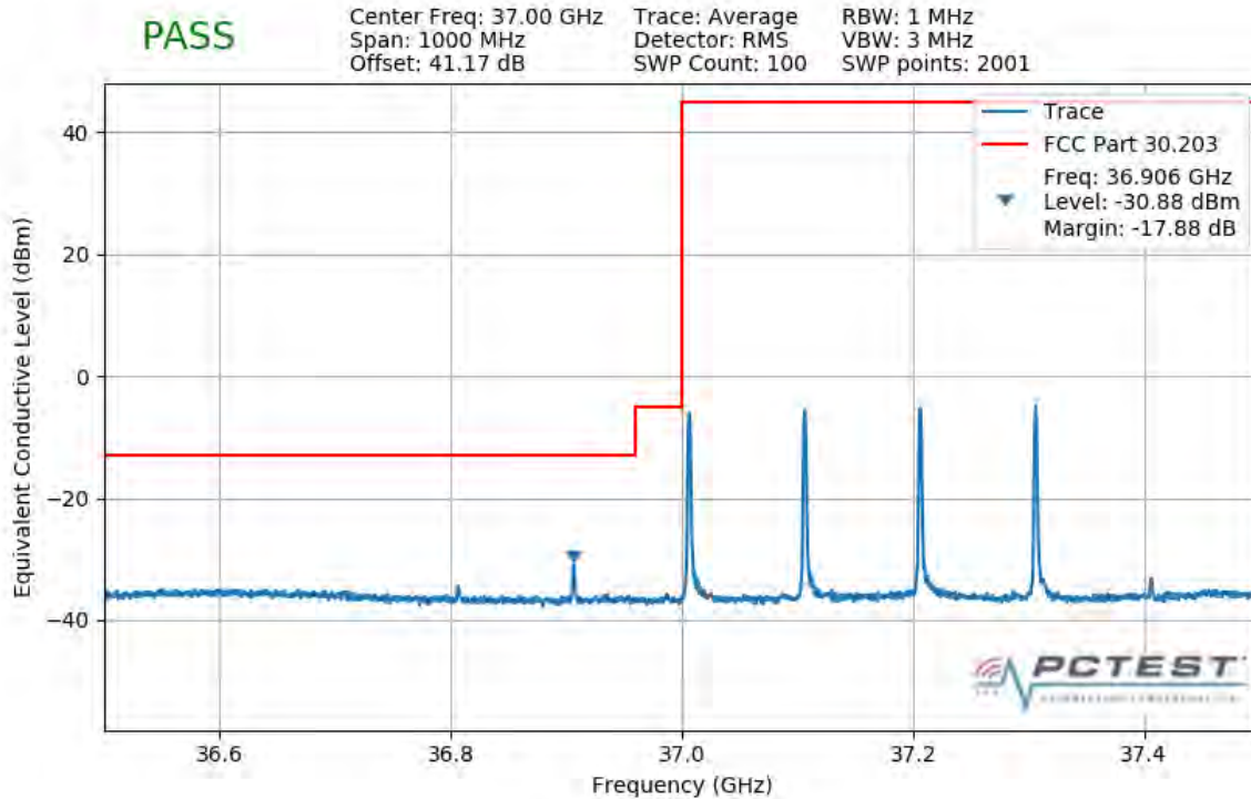
Plot 7-448. Lower Band Edge Plot (4CC 400MHz 64QAM 1 RB)
