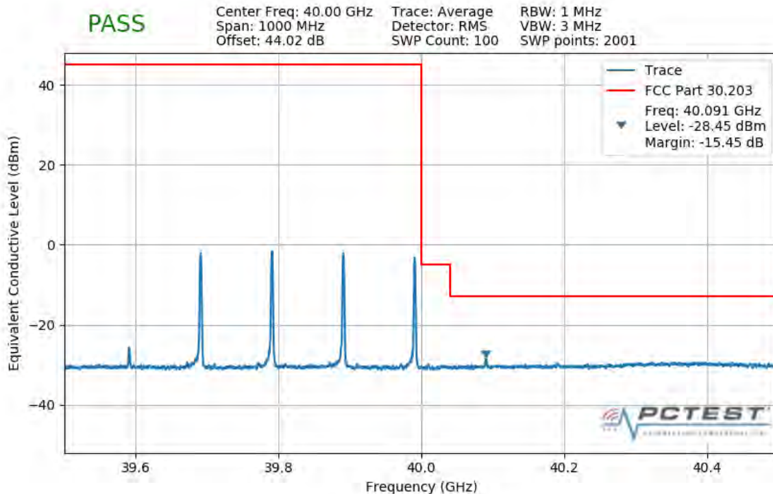
Plot 7-496. Upper Band Edge Plot (4CC 400MHz 64QAM 1 RB)
