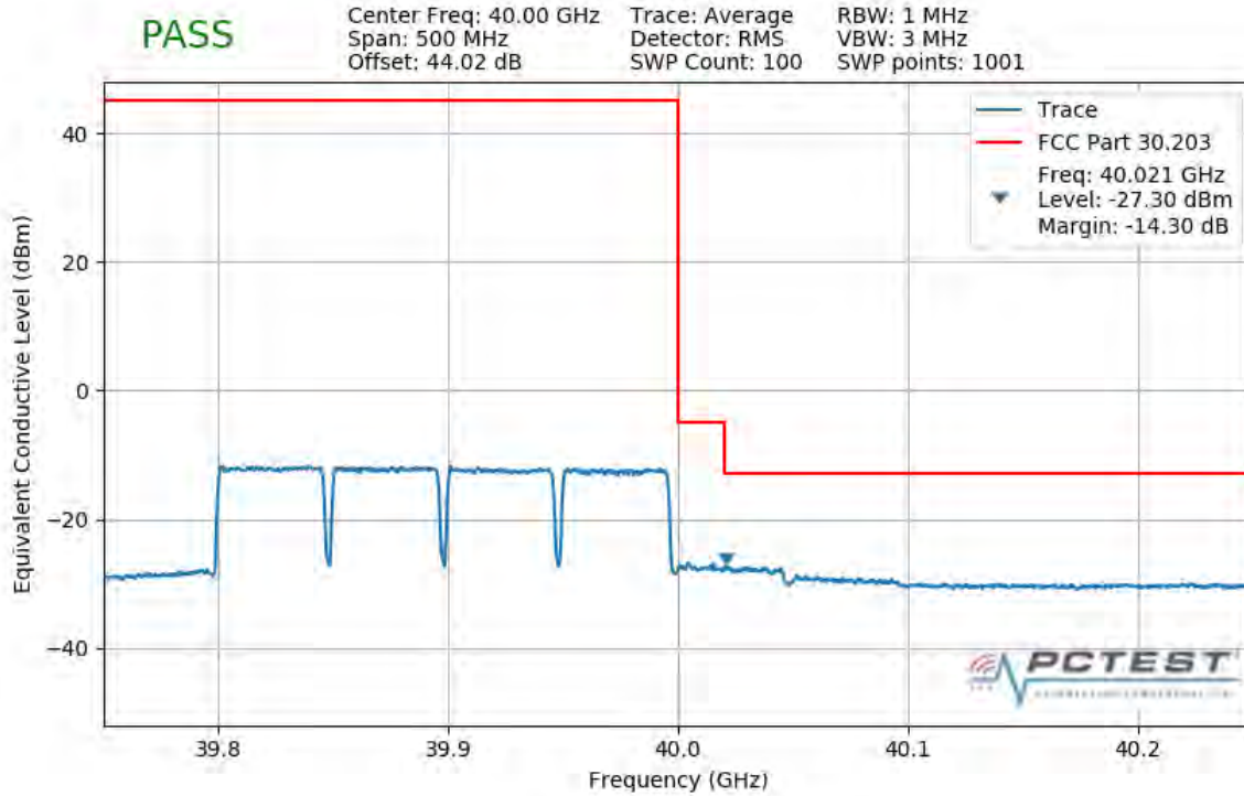
Plot 7-489. Upper Band Edge Plot (4CC 200MHz QPSK Full RB)
