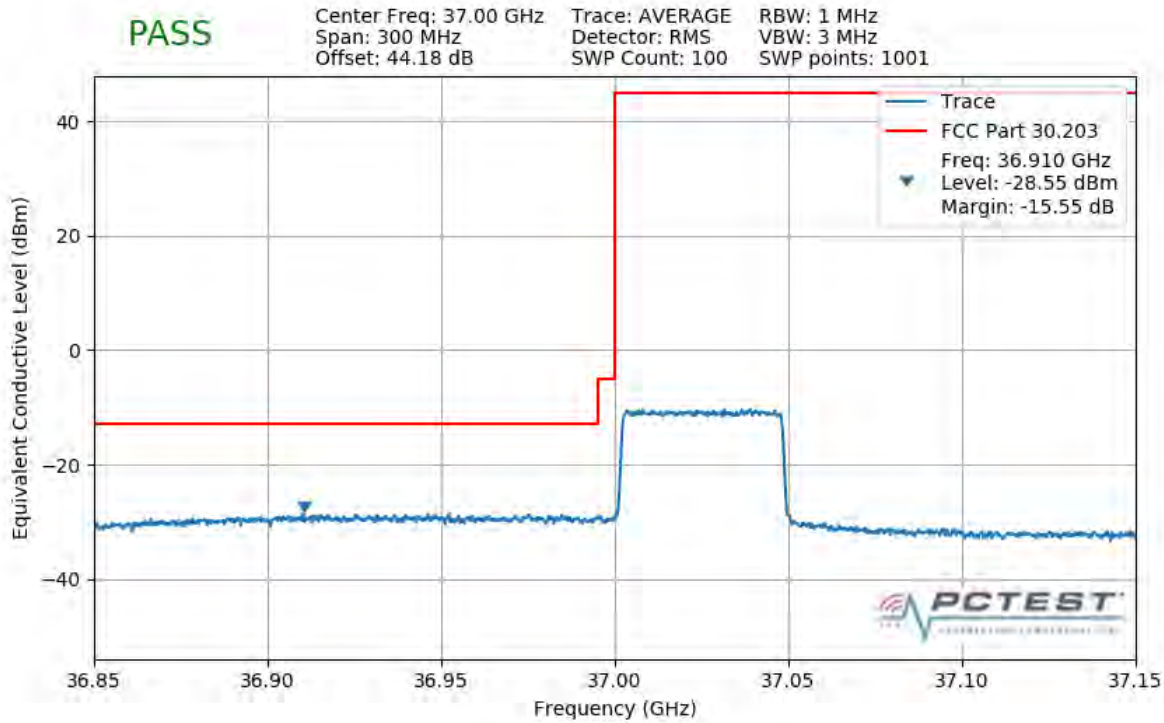
Plot 7-337. Lower Band Edge Plot (1CC 50MHz QPSK Full RB)
