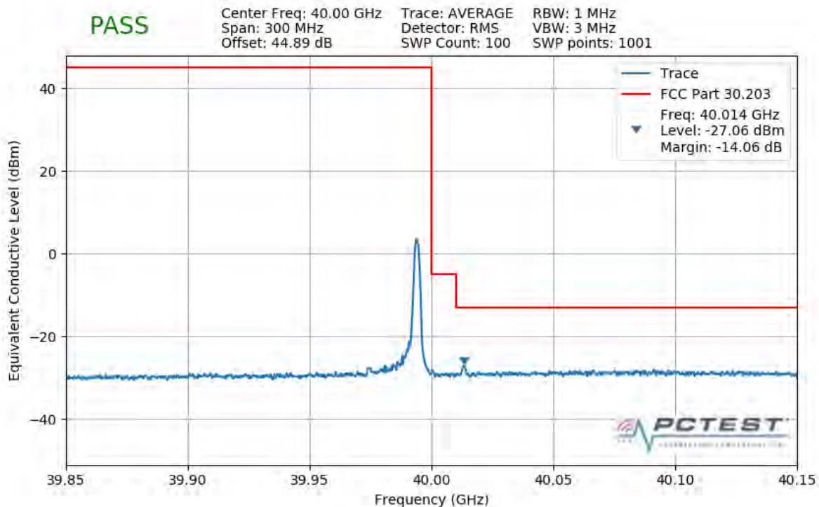
Plot 7-360. Upper Band Edge Plot (1CC 100MHz 64QAM 1 RB)
