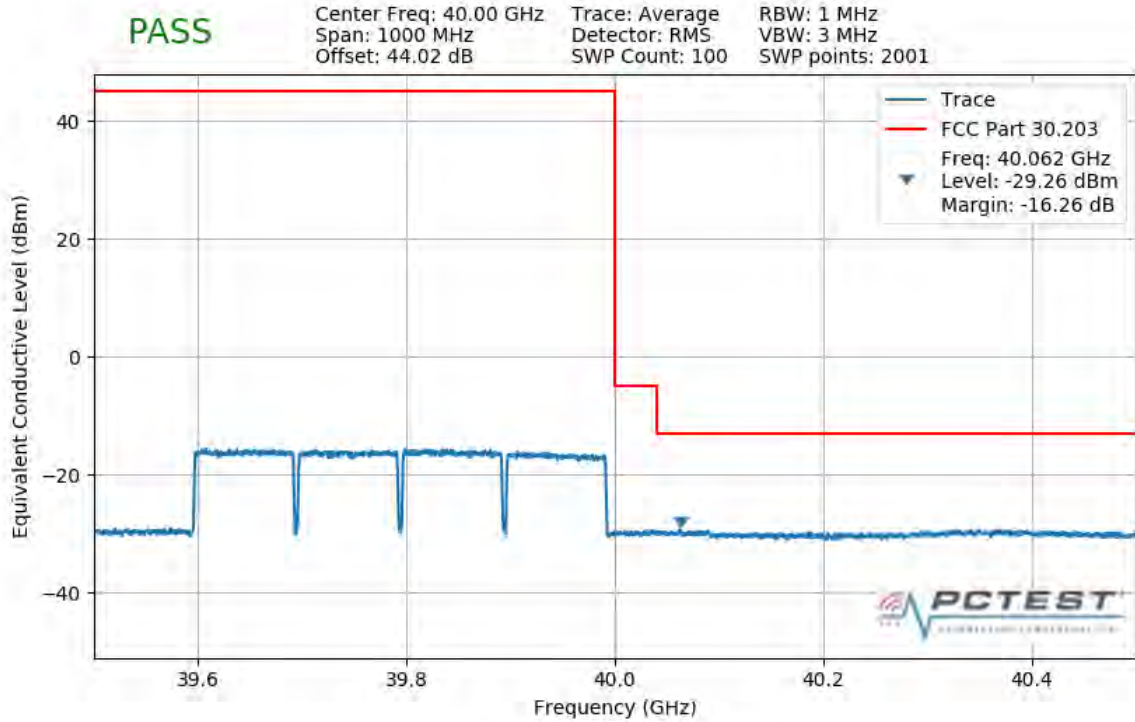
Plot 7-493. Upper Band Edge Plot (4CC 400MHz QPSK Full RB)
