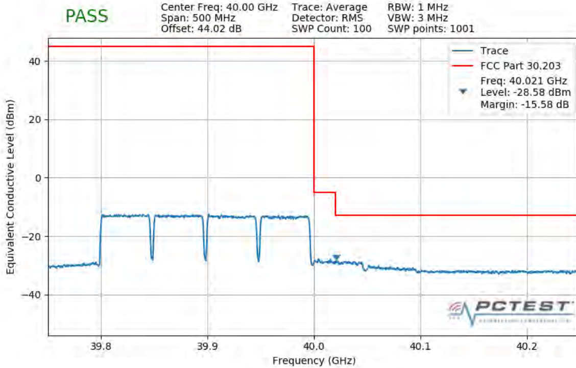
Plot 7-457. Upper Band Edge Plot (4CC 200MHz QPSK Full RB)
