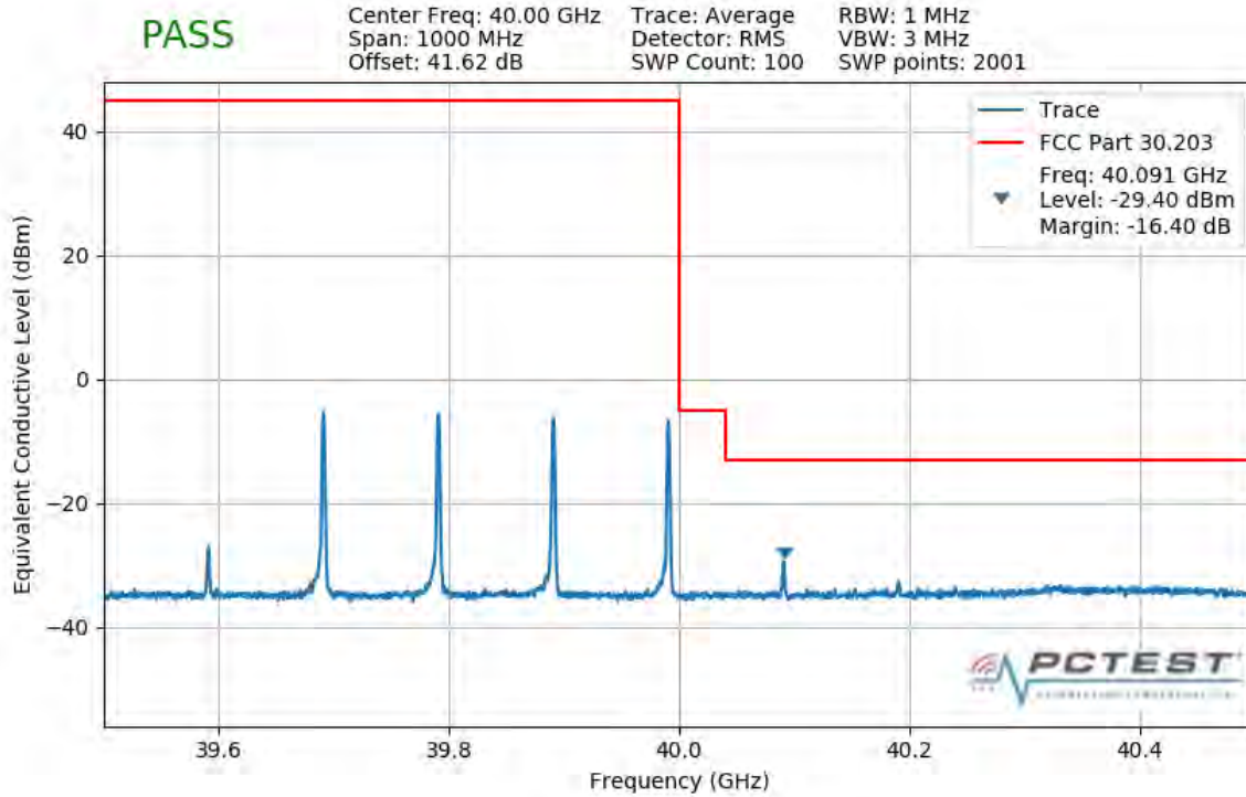
Plot 7-527. Upper Band Edge Plot (4CC 400MHz 16QAM 1 RB)
