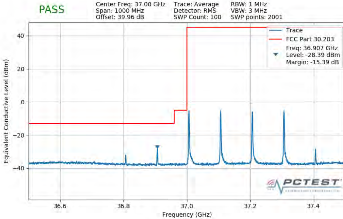
Plot 7-511. Lower Band Edge Plot (4CC 400MHz 16QAM 1 RB)
