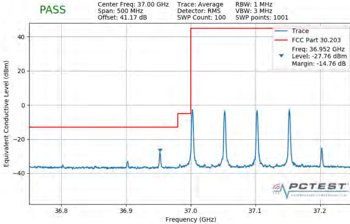
Plot 7-443. Lower Band Edge Plot (4CC 200MHz 16QAM 1 RB)
