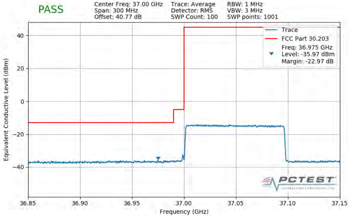
Plot 7-405. Lower Band Edge Plot (1CC 100MHz QPSK Full RB)
