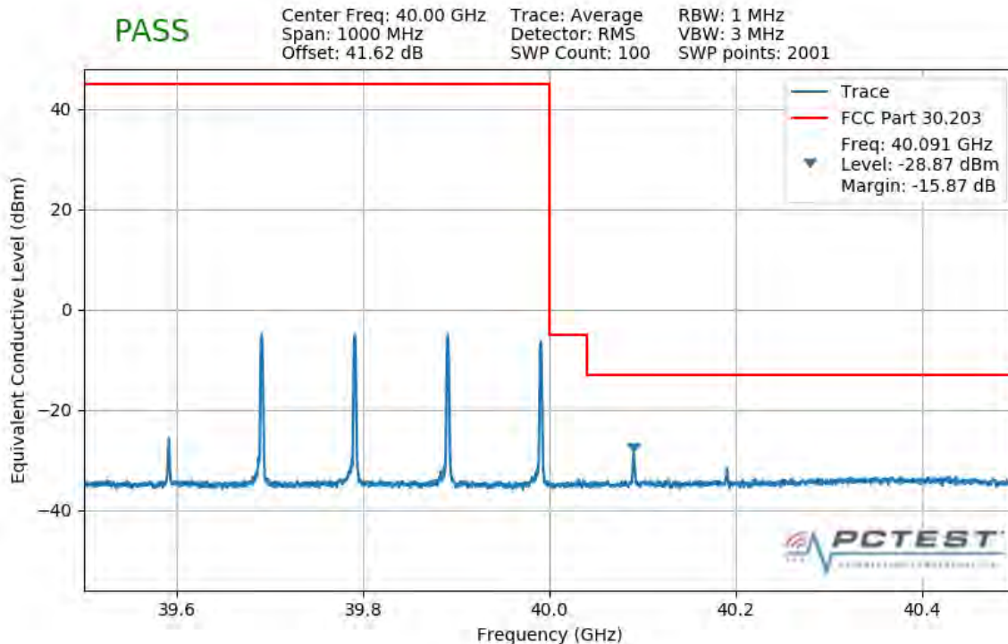
Plot 7-526. Upper Band Edge Plot (4CC 400MHz QPSK 1 RB)
