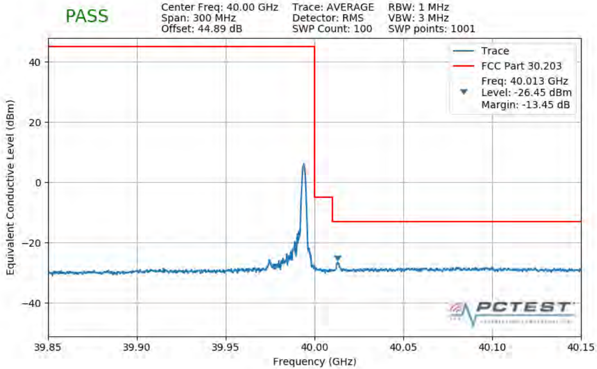
Plot 7-359. Upper Band Edge Plot (1CC 100MHz 16QAM 1 RB)
