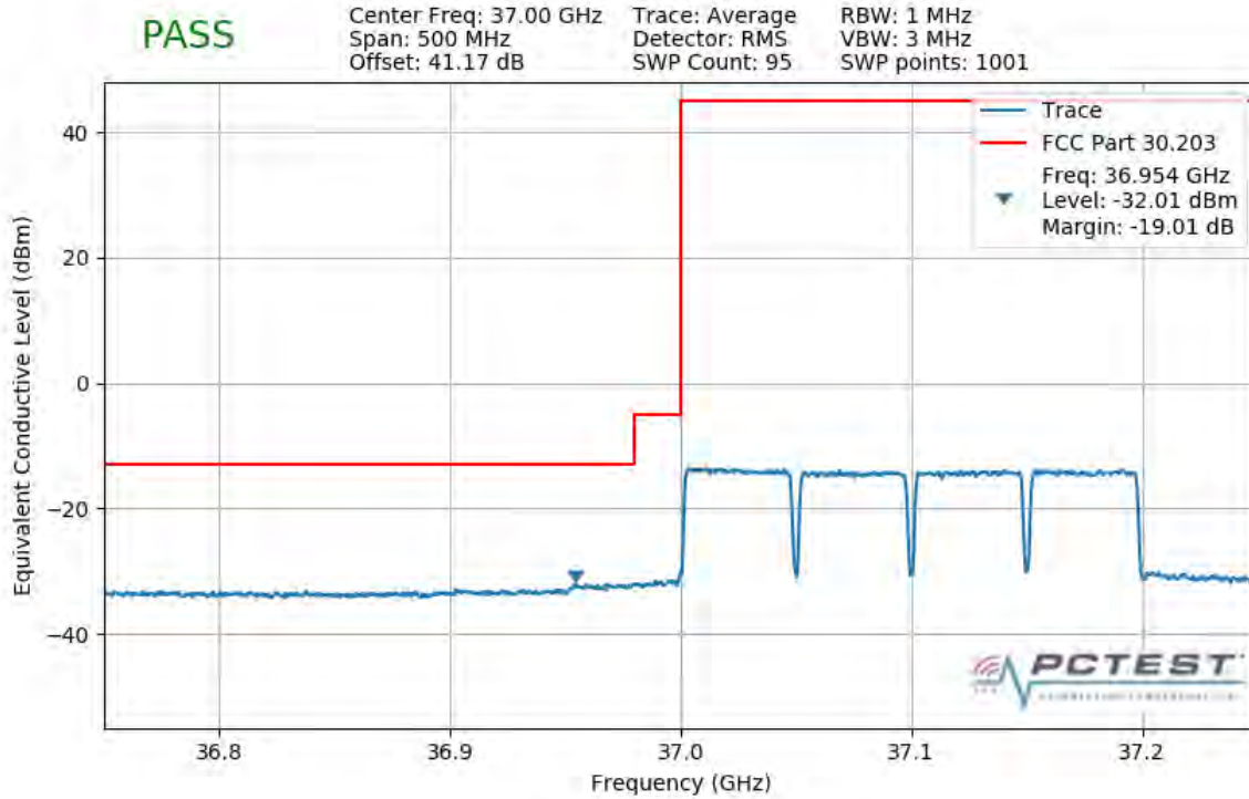
Plot 7-473. Lower Band Edge Plot (4CC 200MHz QPSK Full RB)
