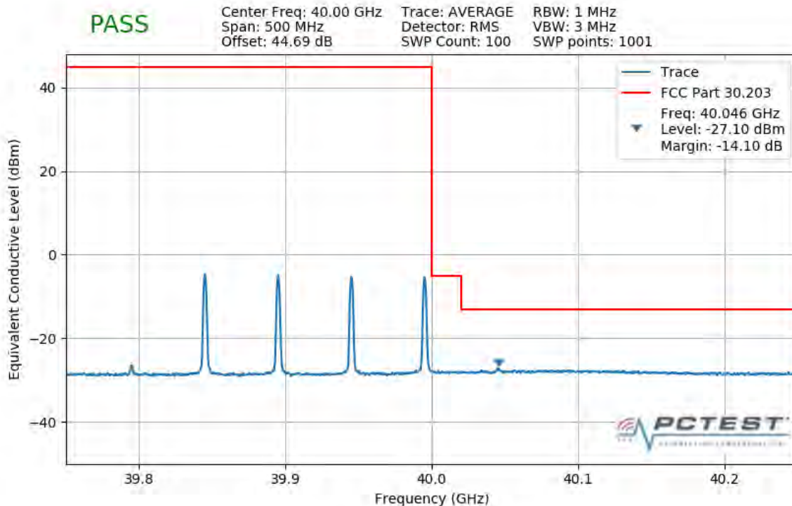
Plot 7-396. Upper Band Edge Plot (4CC 200MHz 64QAM 1 RB)
