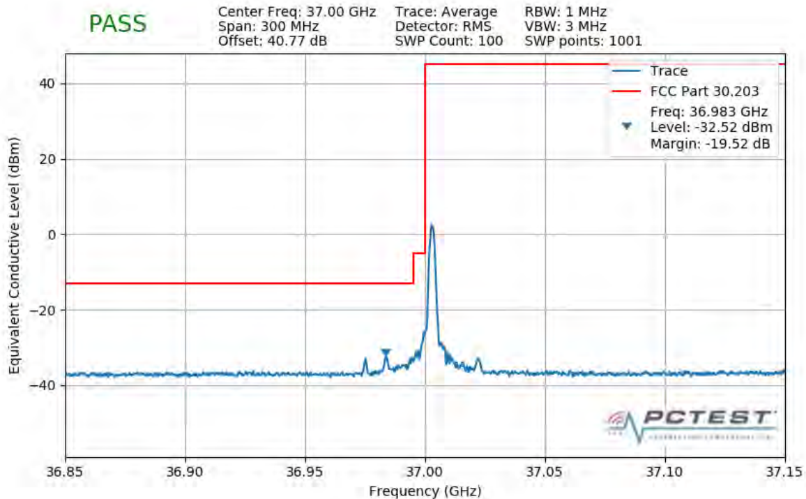
Plot 7-402. Lower Band Edge Plot (1CC 50MHz QPSK 1 RB)
