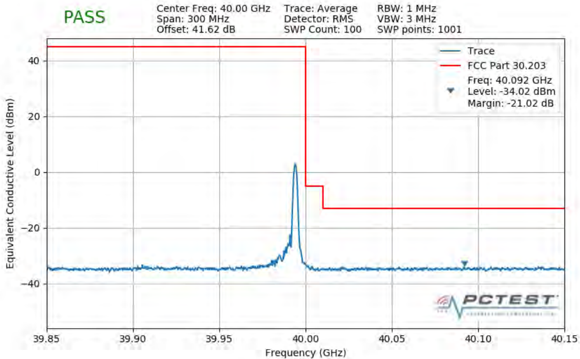
Plot 7-518. Upper Band Edge Plot (1CC 100MHz QPSK 1 RB)
