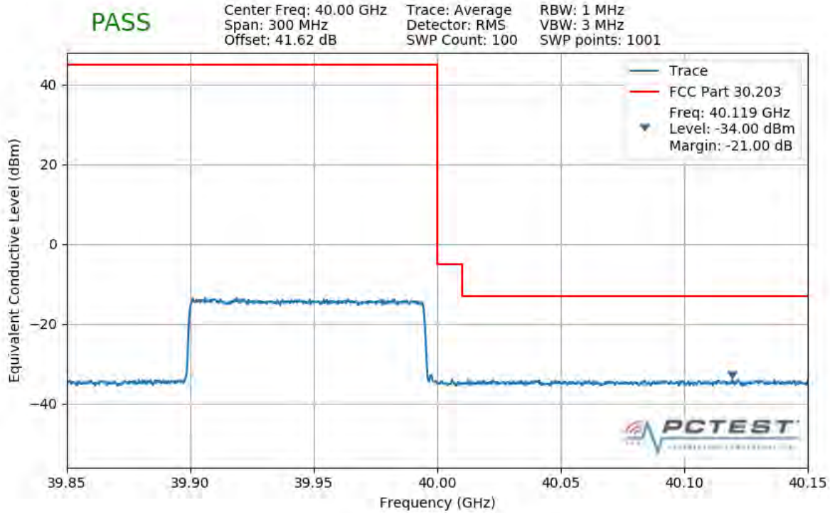
Plot 7-517. Upper Band Edge Plot (1CC 100MHz QPSK Full RB)
