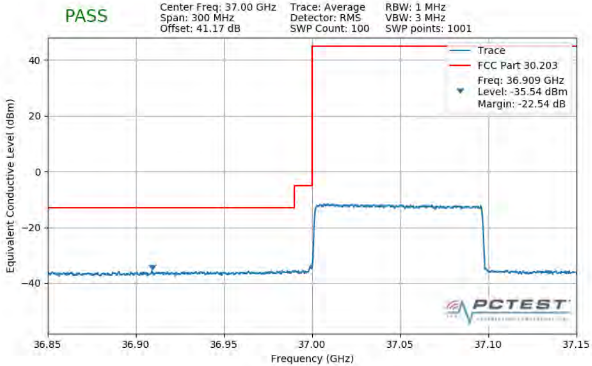
Plot 7-437. Lower Band Edge Plot (1CC 100MHz QPSK Full RB)
