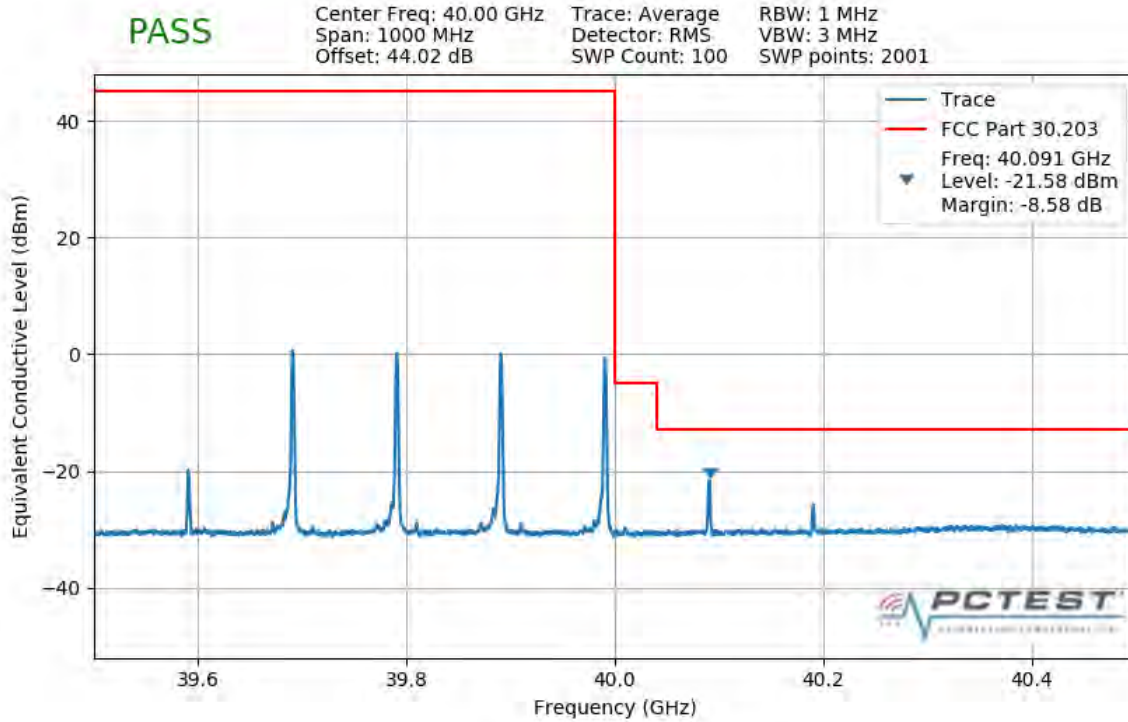
Plot 7-495. Upper Band Edge Plot (4CC 400MHz 16QAM 1 RB)
