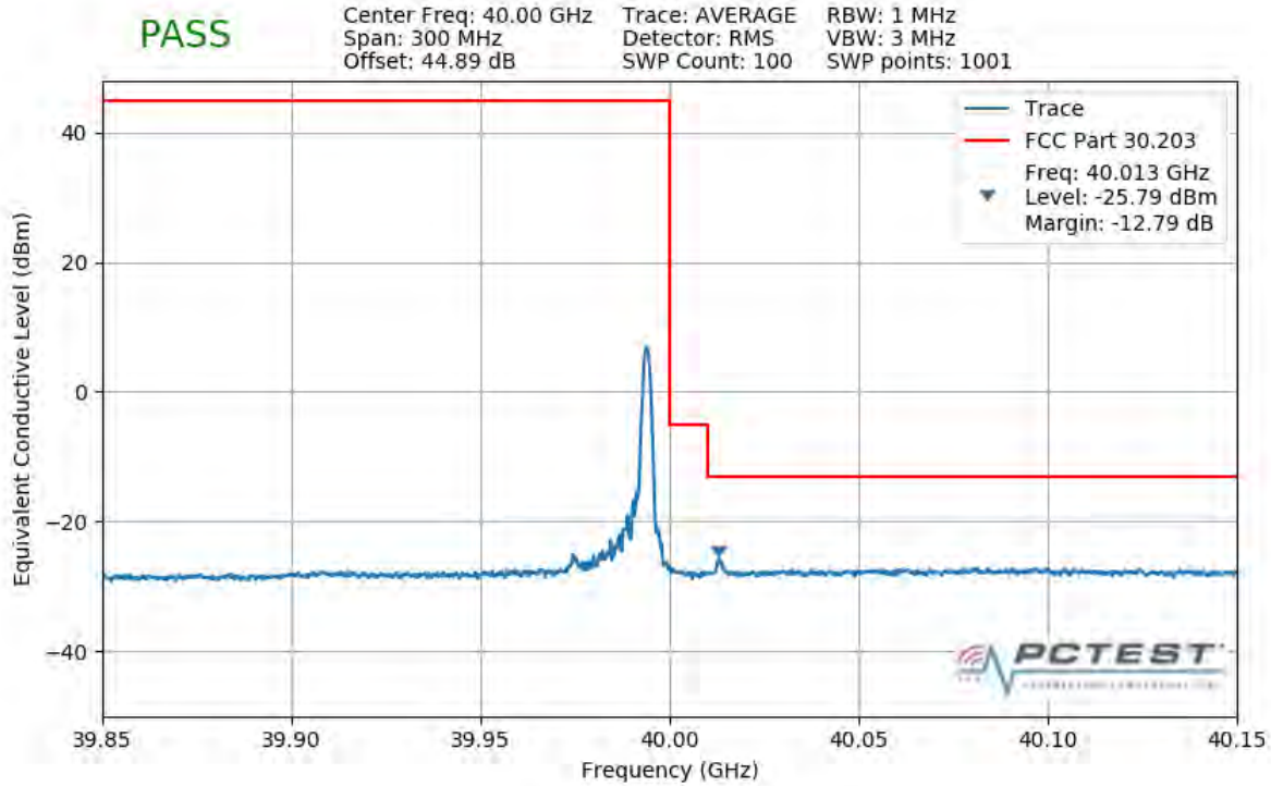
Plot 7-391. Upper Band Edge Plot (1CC 100MHz 16QAM 1 RB)
