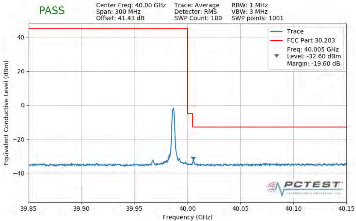
Plot 7-420. Upper Band Edge Plot (1CC 50MHz 64QAM 1 RB)
