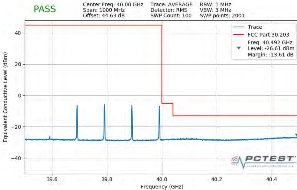
Plot 7-400. Upper Band Edge Plot (4CC 400MHz 64QAM 1 RB)
