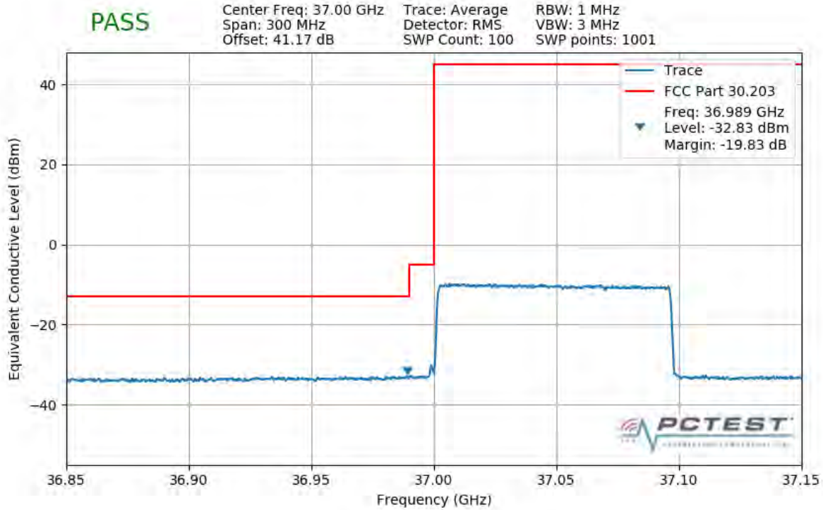
Plot 7-469. Lower Band Edge Plot (1CC 100MHz QPSK Full RB)
