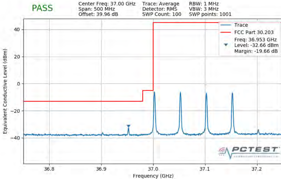
Plot 7-508. Lower Band Edge Plot (4CC 200MHz 64QAM 1 RB)
