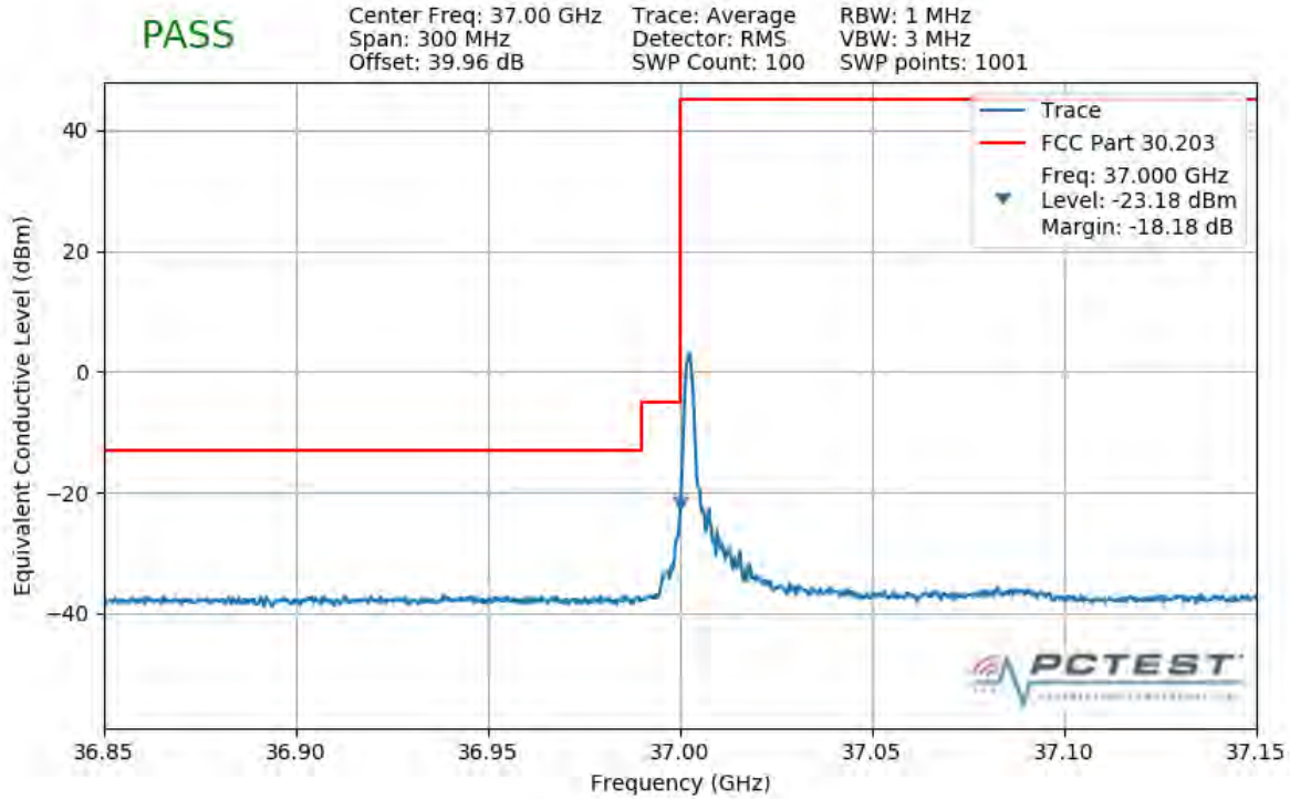
Plot 7-503. Lower Band Edge Plot (1CC 100MHz 16QAM 1 RB)
