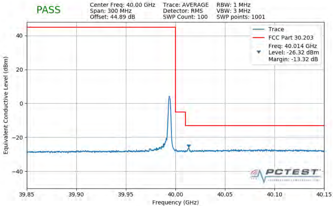
Plot 7-392. Upper Band Edge Plot (1CC 100MHz 64QAM 1 RB)
