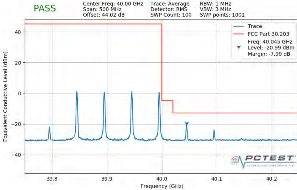
Plot 7-491. Upper Band Edge Plot (4CC 200MHz 16QAM 1 RB)
