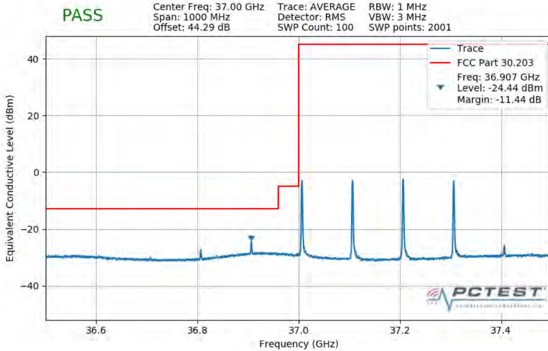
Plot 7-383. Lower Band Edge Plot (4CC 400MHz 16QAM 1 RB)
