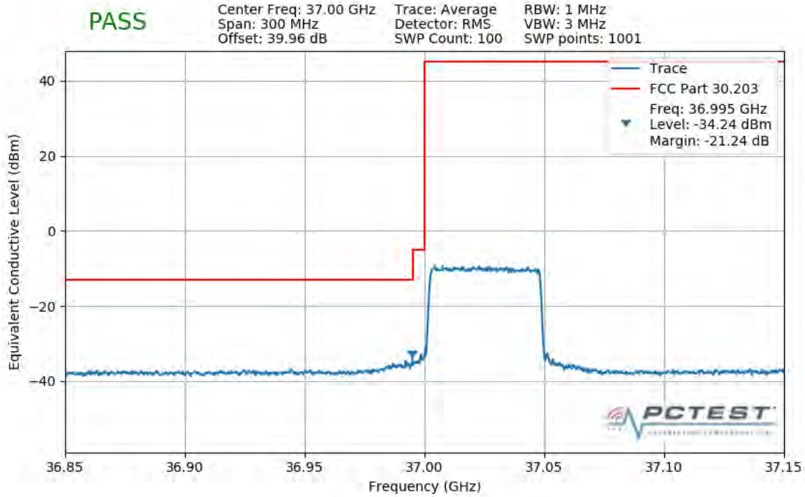
Plot 7-497. Lower Band Edge Plot (1CC 50MHz QPSK Full RB)
