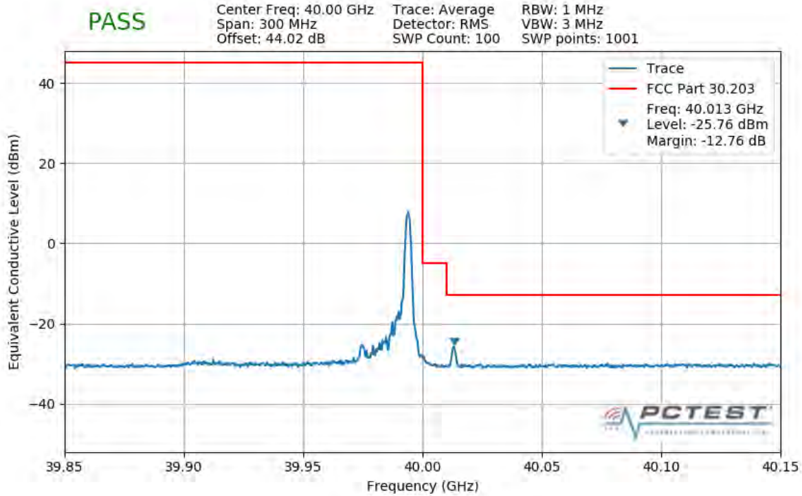
Plot 7-487. Upper Band Edge Plot (1CC 100MHz 16QAM 1 RB)
