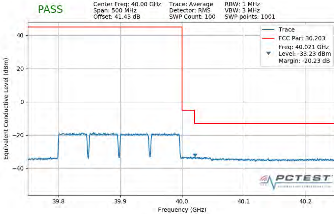
Plot 7-425. Upper Band Edge Plot (4CC 200MHz QPSK Full RB)
