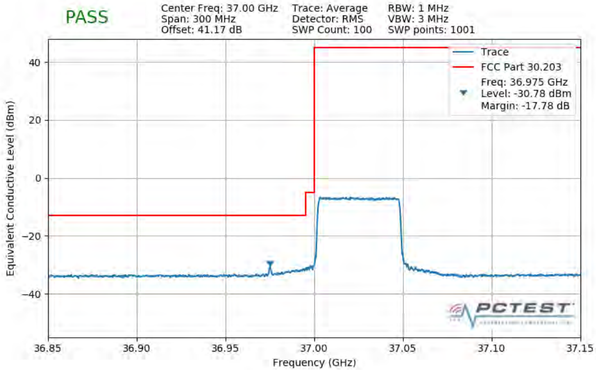
Plot 7-465. Lower Band Edge Plot (1CC 50MHz QPSK Full RB)
