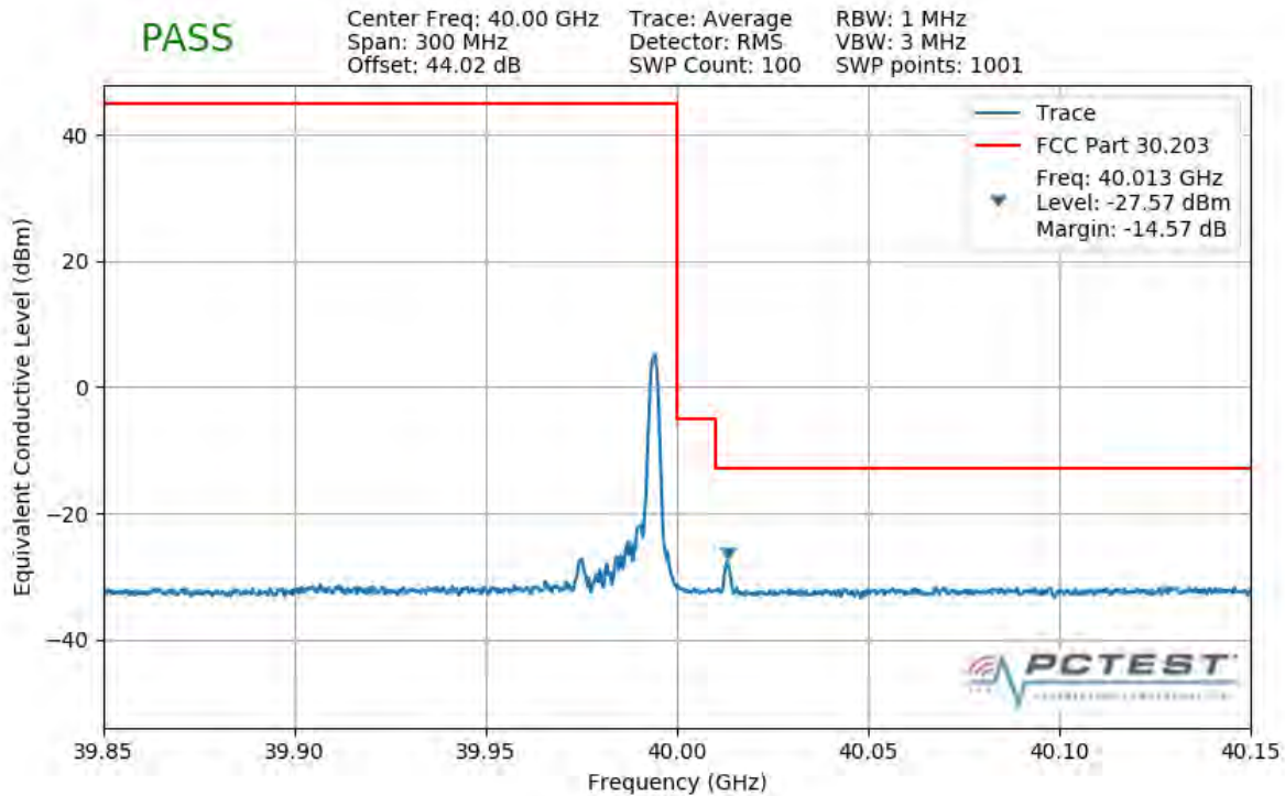
Plot 7-456. Upper Band Edge Plot (1CC 100MHz 64QAM 1 RB)
