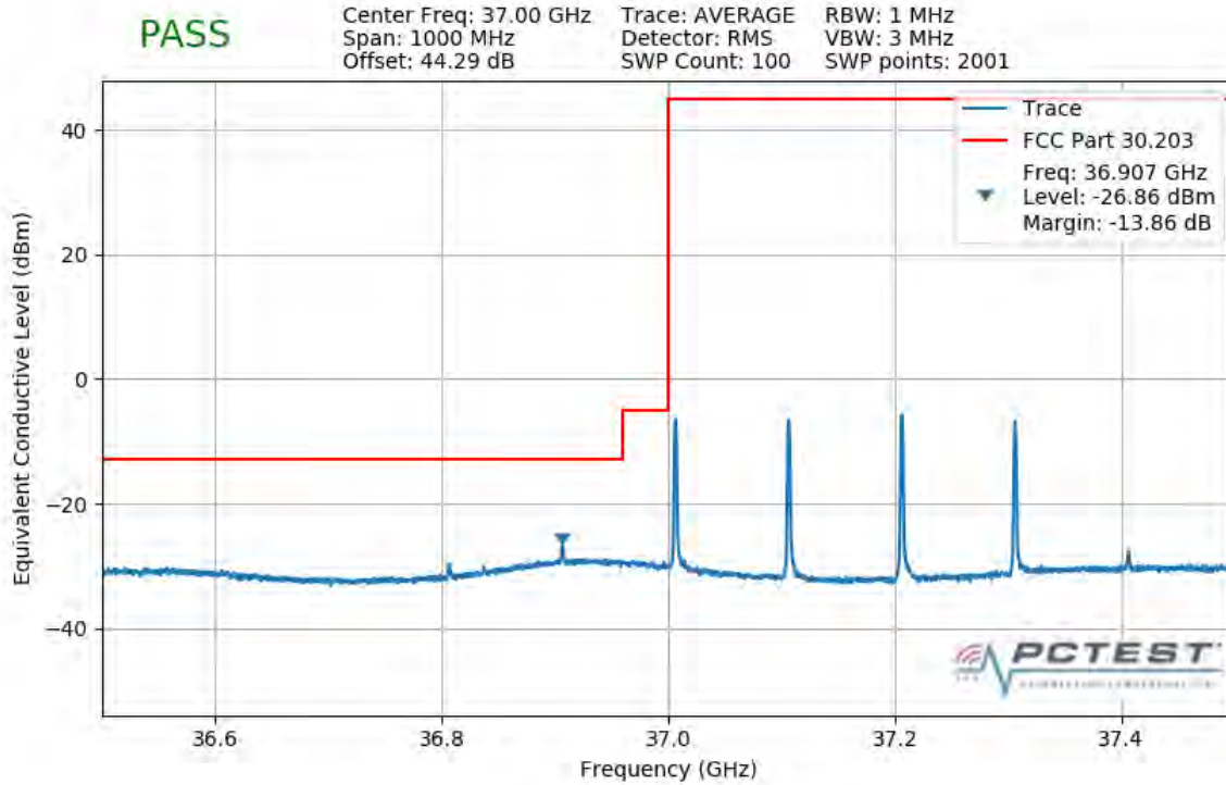
Plot 7-351. Lower Band Edge Plot (4CC 400MHz 16QAM 1 RB)
