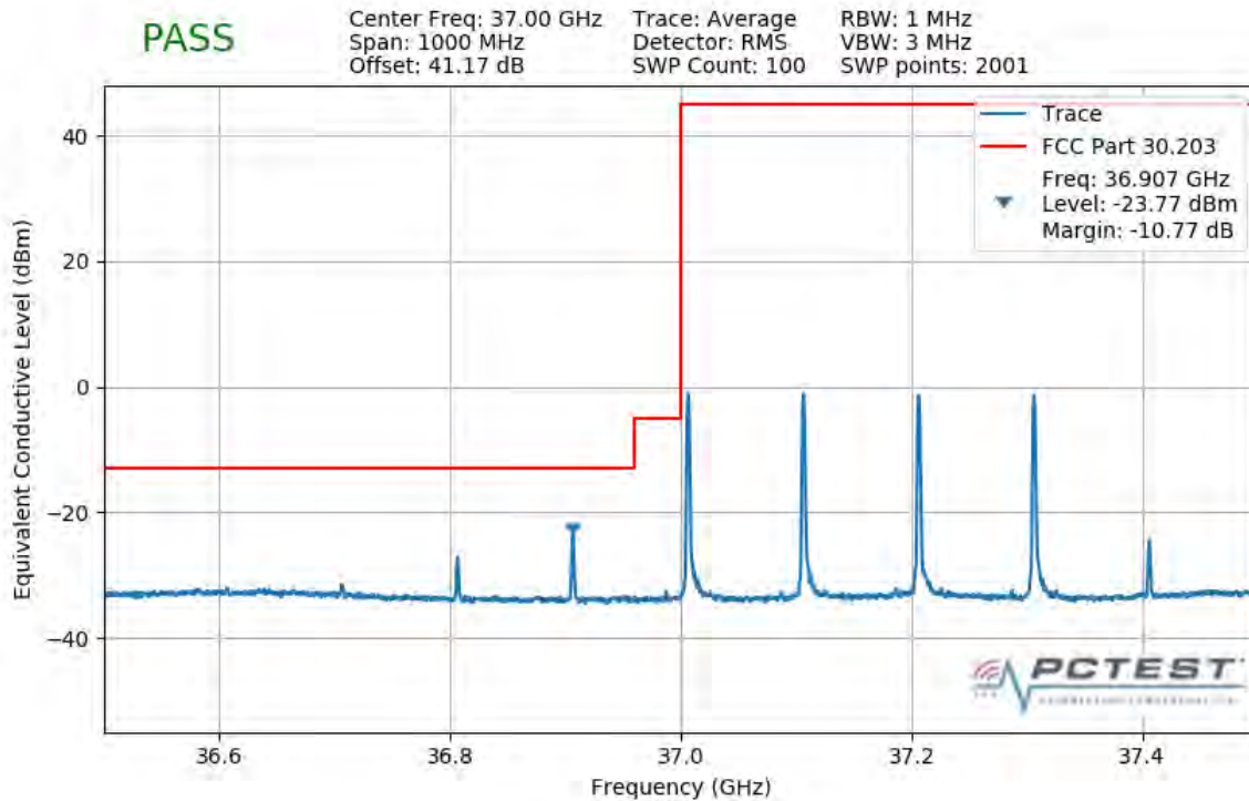
Plot 7-478. Lower Band Edge Plot (4CC 400MHz QPSK 1 RB)
