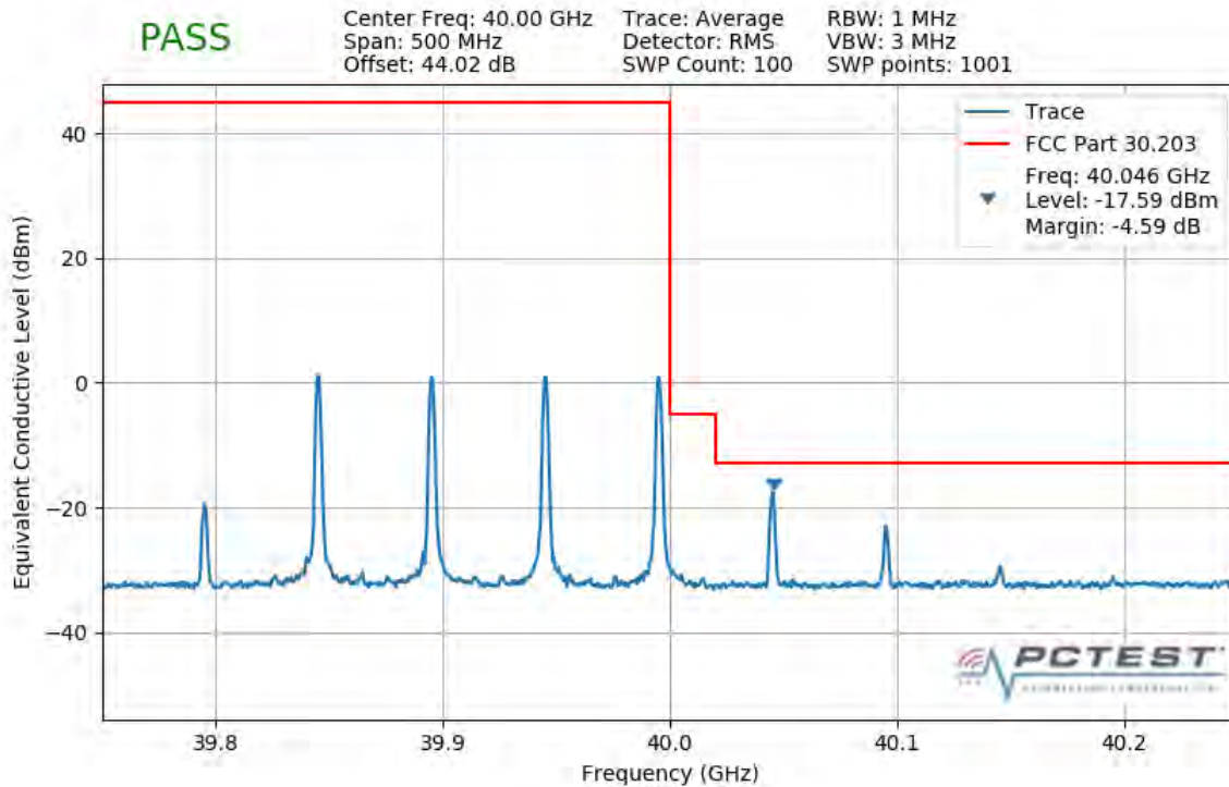
Plot 7-458. Upper Band Edge Plot (4CC 200MHz QPSK 1 RB)
