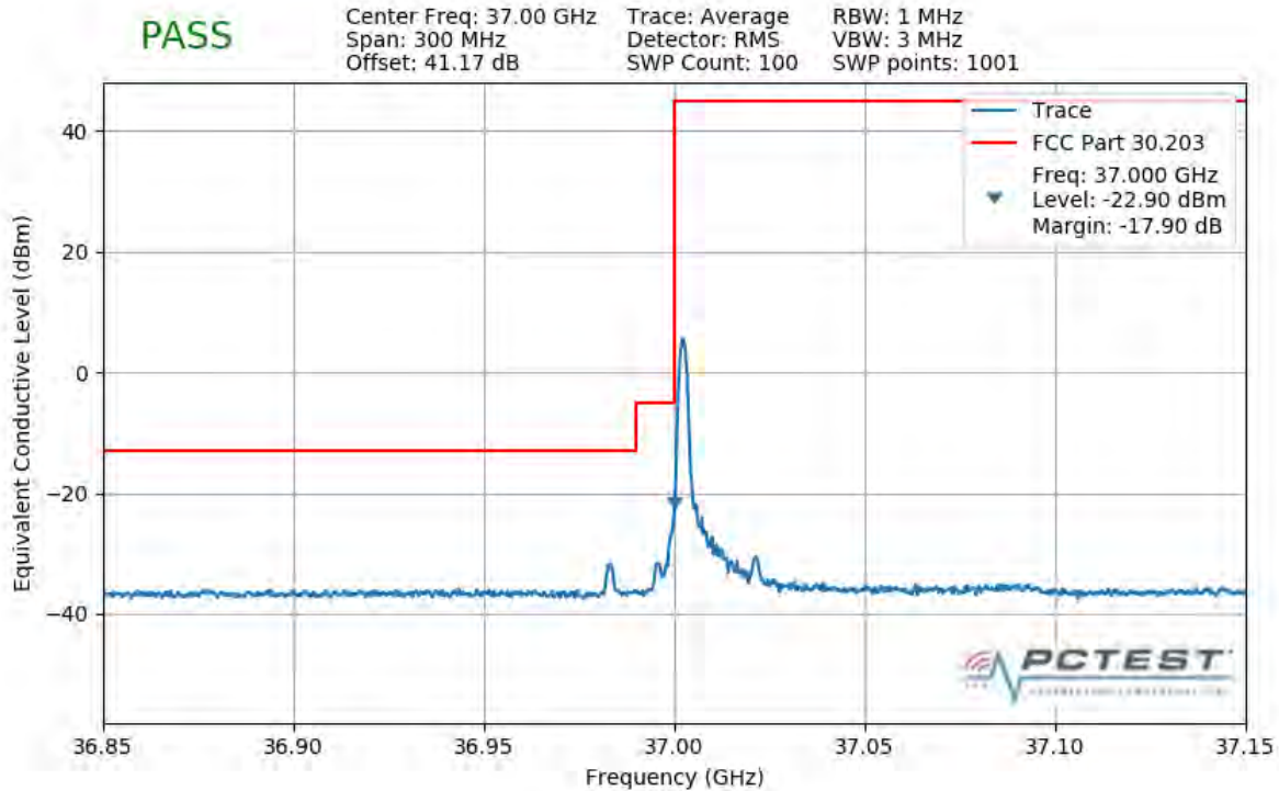
Plot 7-438. Lower Band Edge Plot (1CC 100MHz QPSK 1 RB)
