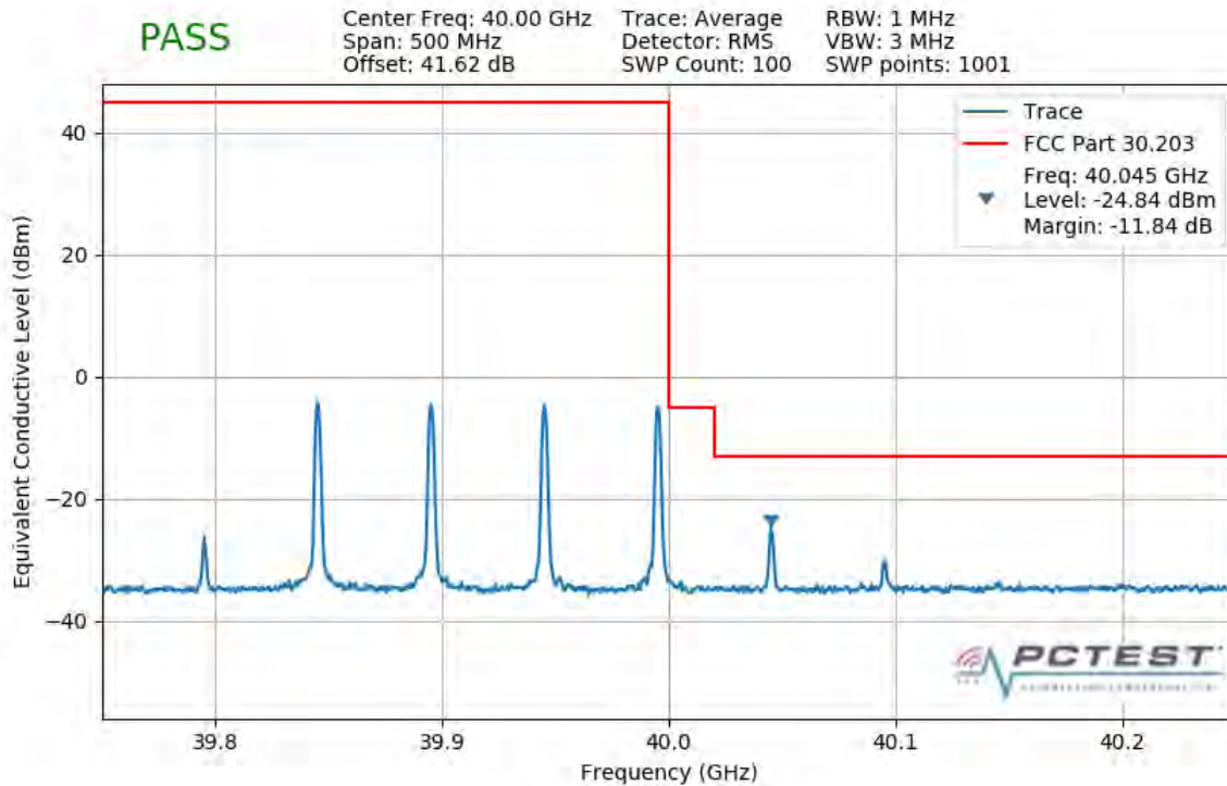
Plot 7-522. Upper Band Edge Plot (4CC 200MHz QPSK 1 RB)
