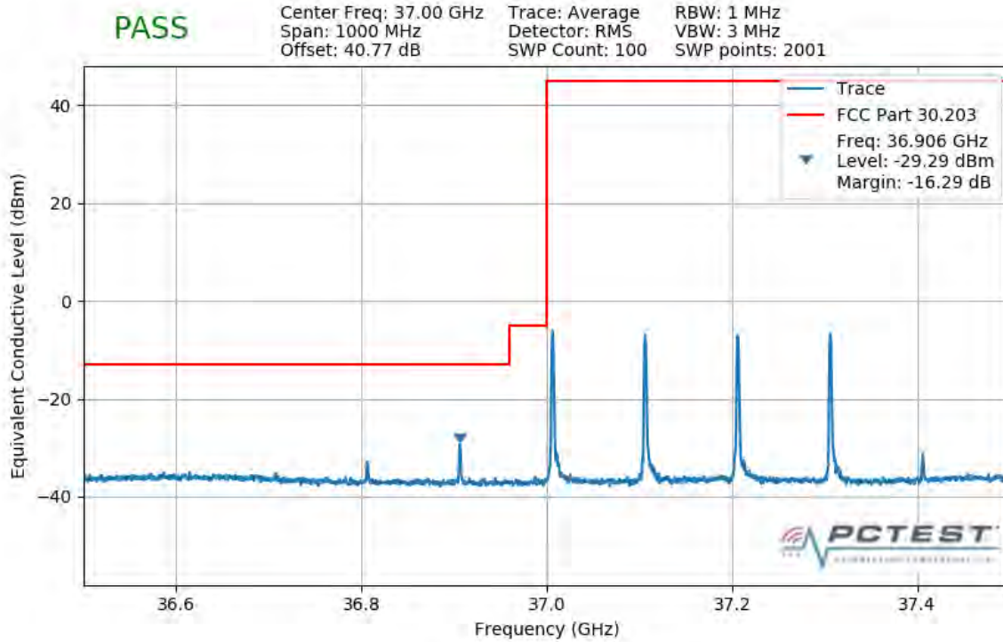
Plot 7-415. Lower Band Edge Plot (4CC 400MHz 16QAM 1 RB)
