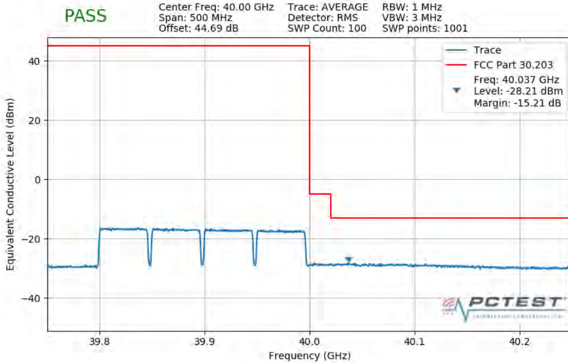
Plot 7-361. Upper Band Edge Plot (4CC 200MHz QPSK Full RB)
