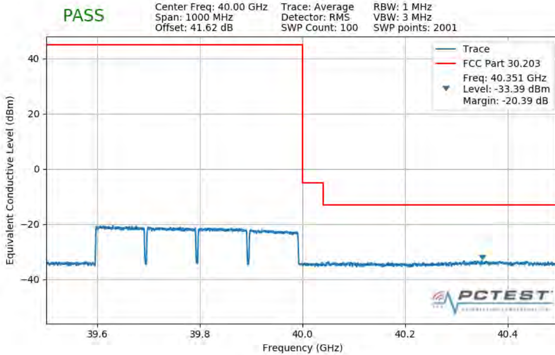
Plot 7-525. Upper Band Edge Plot (4CC 400MHz QPSK Full RB)
