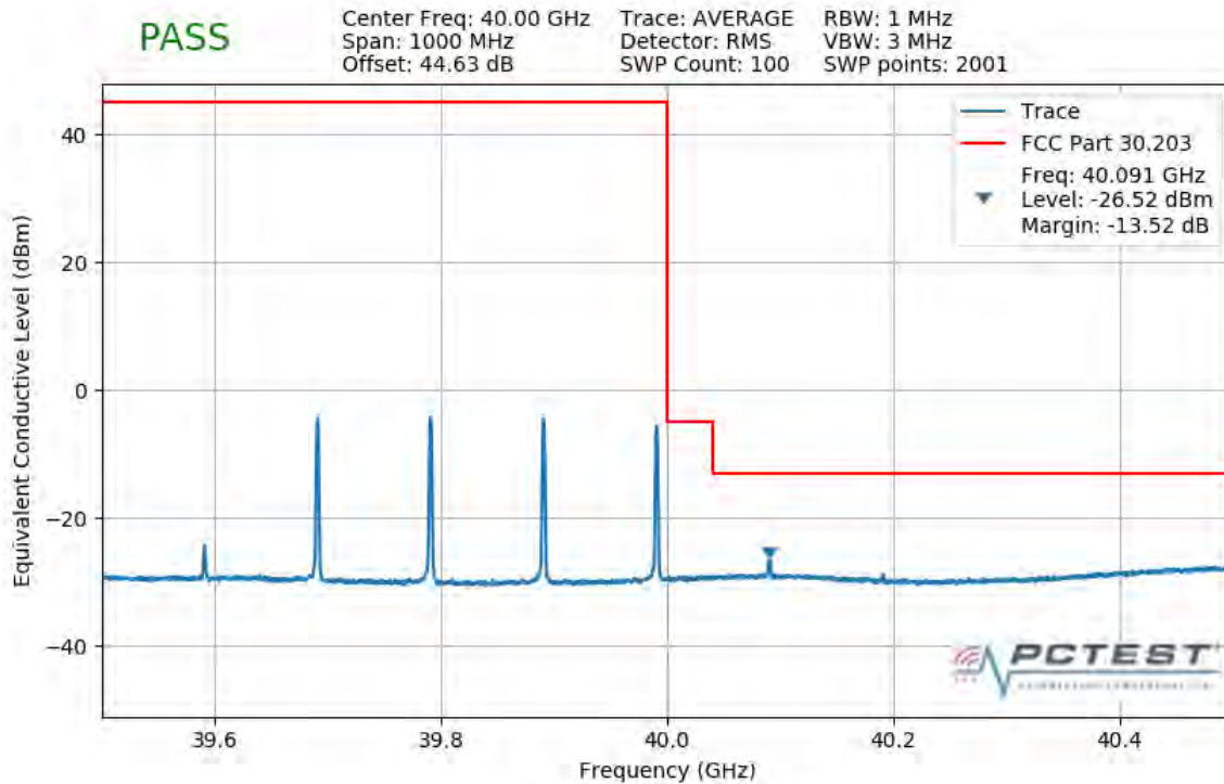
Plot 7-366. Upper Band Edge Plot (4CC 400MHz QPSK 1 RB)
