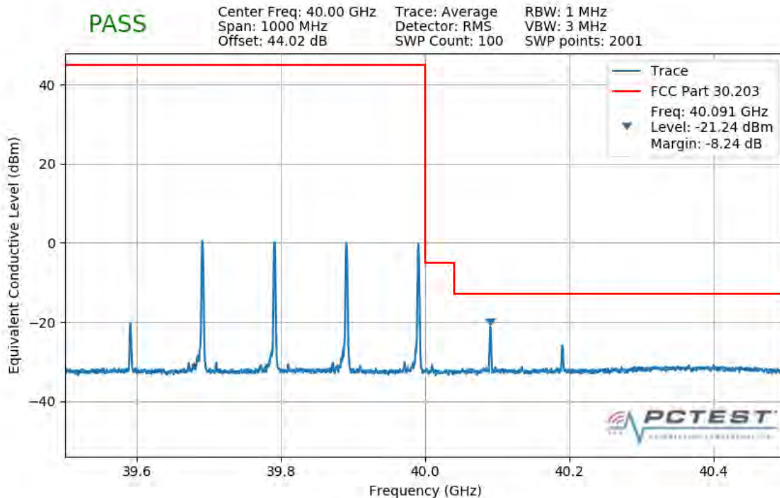
Plot 7-462. Upper Band Edge Plot (4CC 400MHz QPSK 1 RB)
