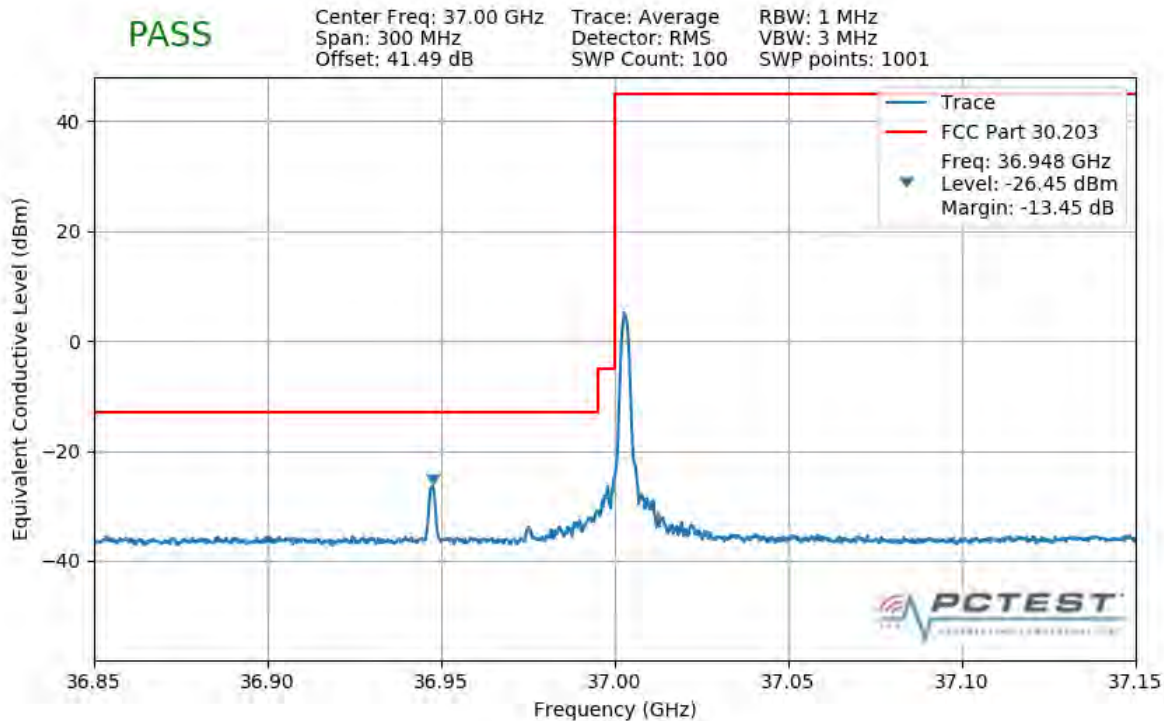
Plot 7-530. Lower Band Edge Plot (1CC 50MHz QPSK 1 RB)
