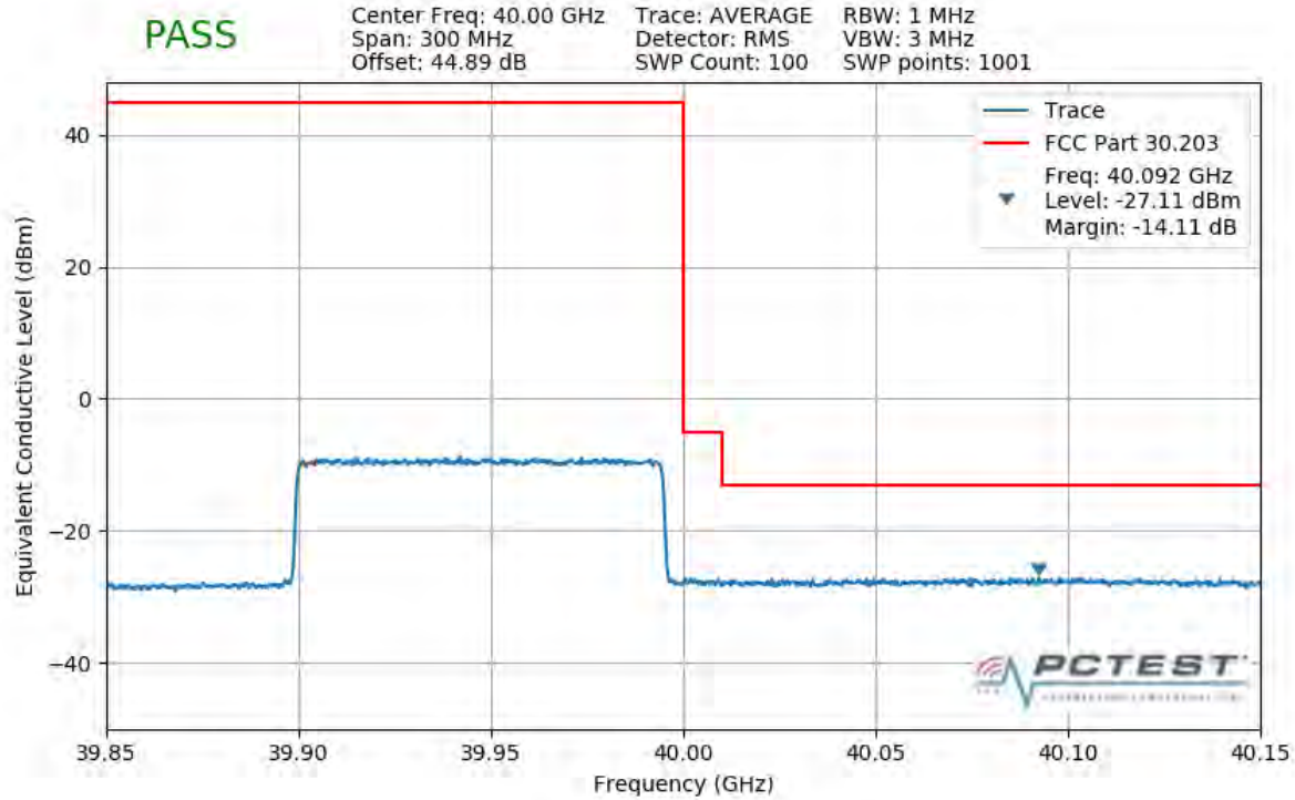
Plot 7-389. Upper Band Edge Plot (1CC 100MHz QPSK Full RB)
