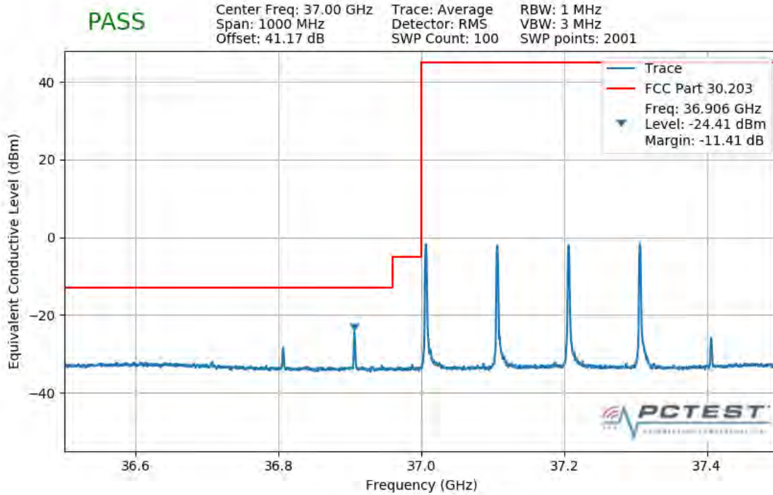
Plot 7-479. Lower Band Edge Plot (4CC 400MHz 16QAM 1 RB)
