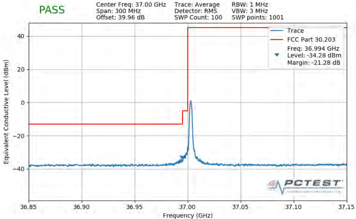
Plot 7-500. Lower Band Edge Plot (1CC 50MHz 64QAM 1 RB)
