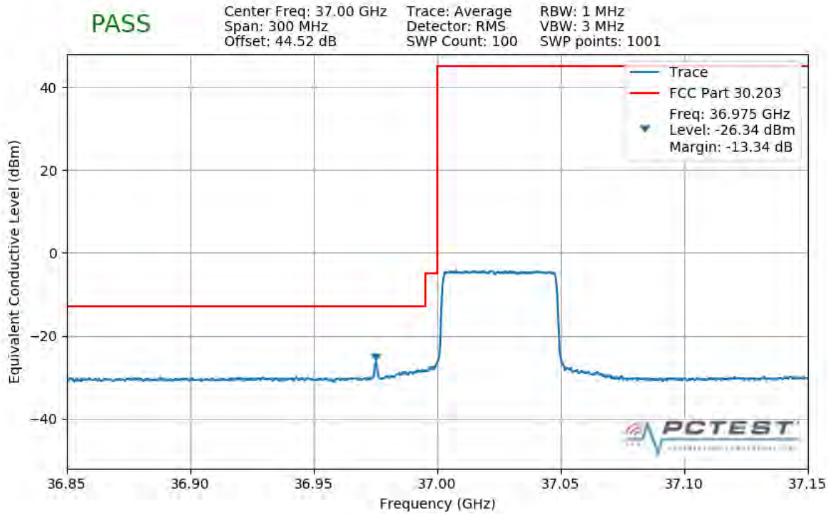
Plot 7-273. Lower Band Edge Plot (1CC 50MHz QPSK Full RB)
