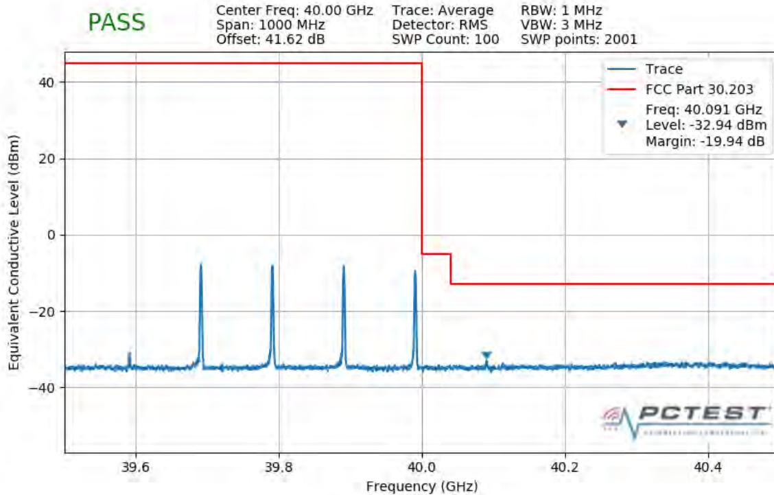
Plot 7-528. Upper Band Edge Plot (4CC 400MHz 64QAM 1 RB)
