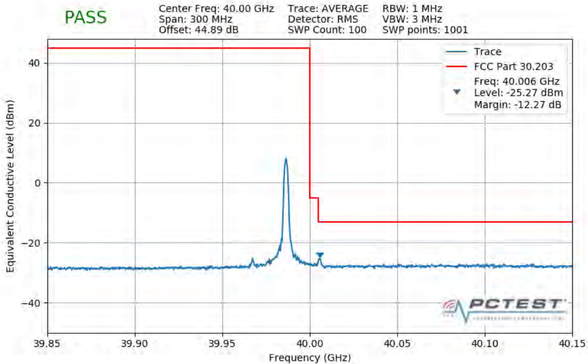
Plot 7-386. Upper Band Edge Plot (1CC 50MHz QPSK 1 RB)
