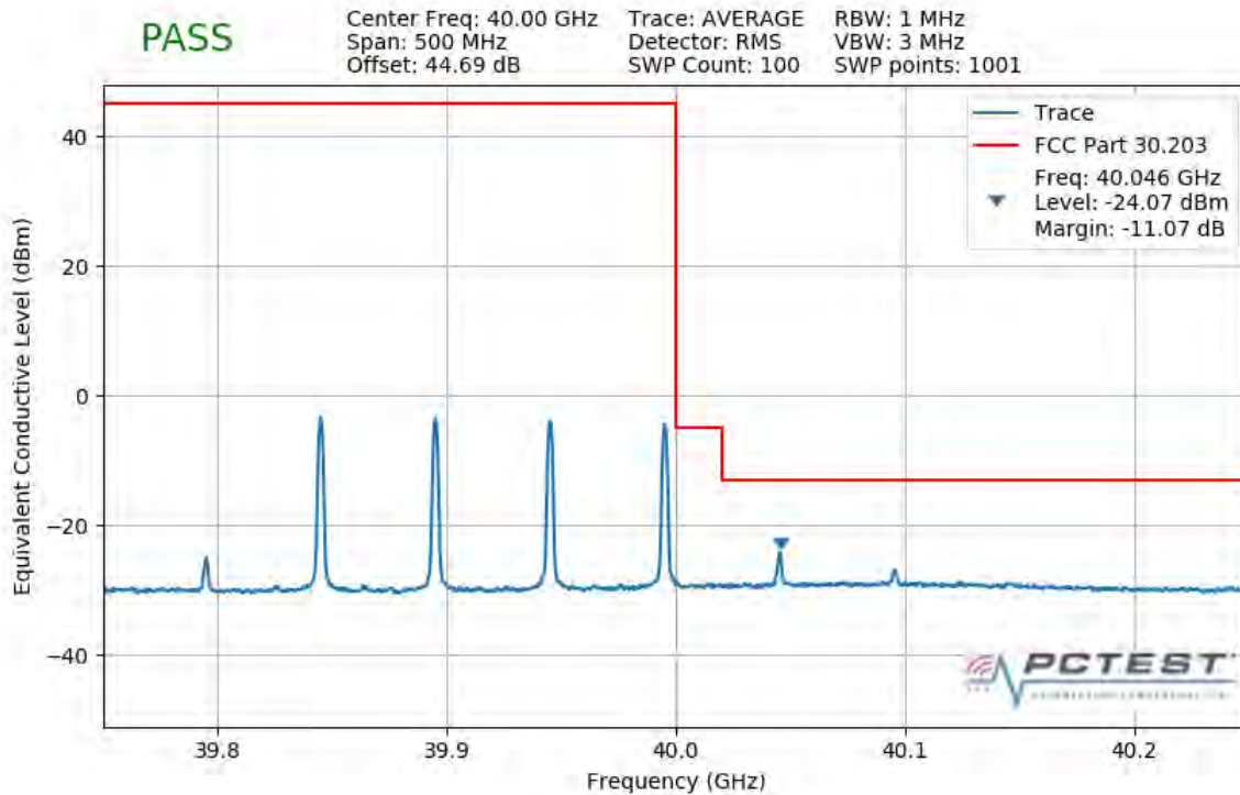
Plot 7-362. Upper Band Edge Plot (4CC 200MHz QPSK 1 RB)
