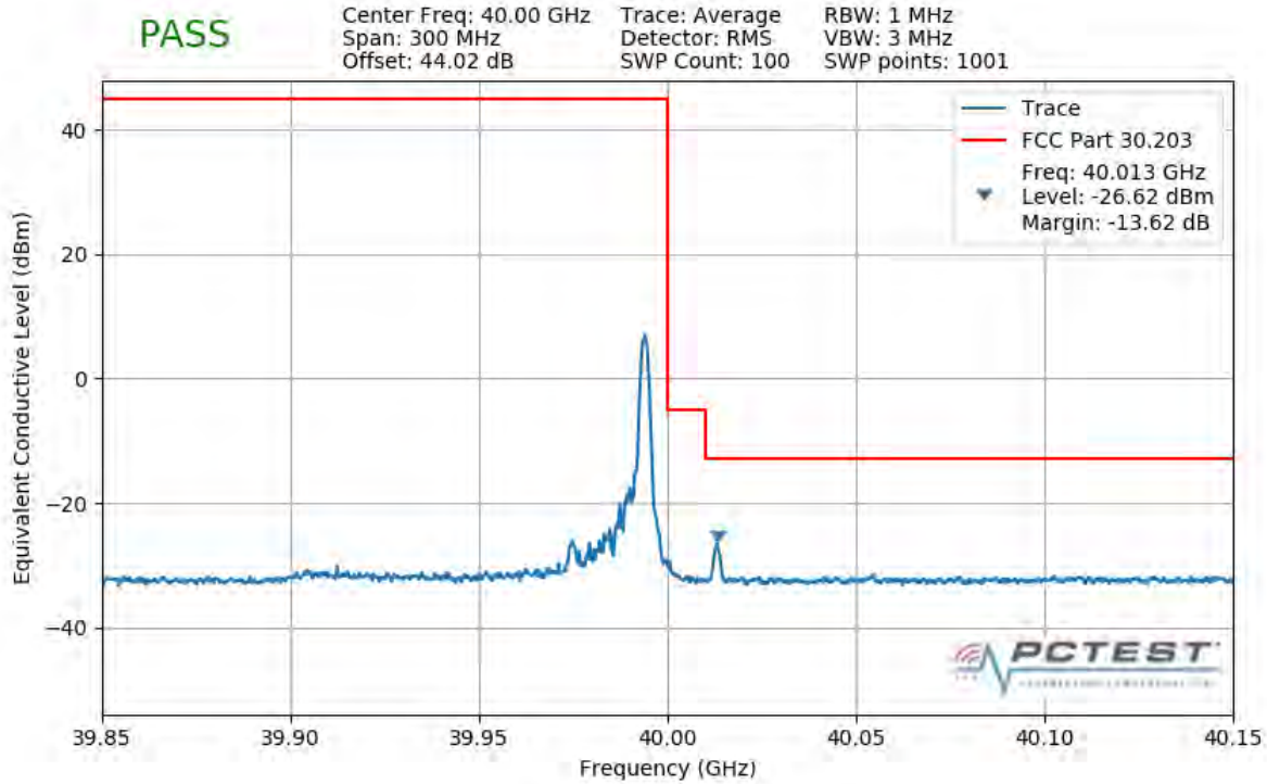
Plot 7-455. Upper Band Edge Plot (1CC 100MHz 16QAM 1 RB)
