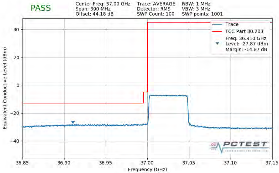
Plot 7-369. Lower Band Edge Plot (1CC 50MHz QPSK Full RB)
