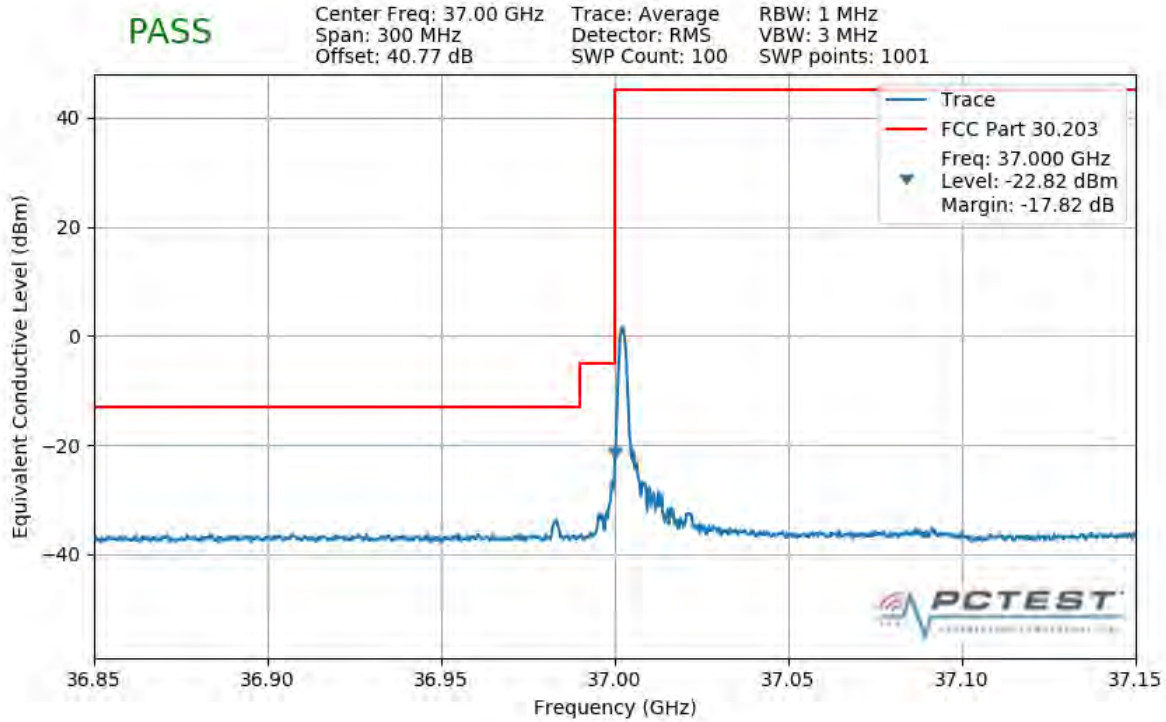
Plot 7-407. Lower Band Edge Plot (1CC 100MHz 16QAM 1 RB)
