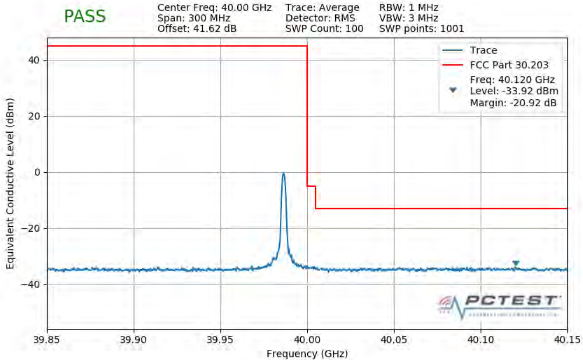
Plot 7-516. Upper Band Edge Plot (1CC 50MHz 64QAM 1 RB)
