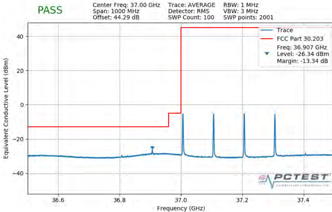
Plot 7-384. Lower Band Edge Plot (4CC 400MHz 64QAM 1 RB)
