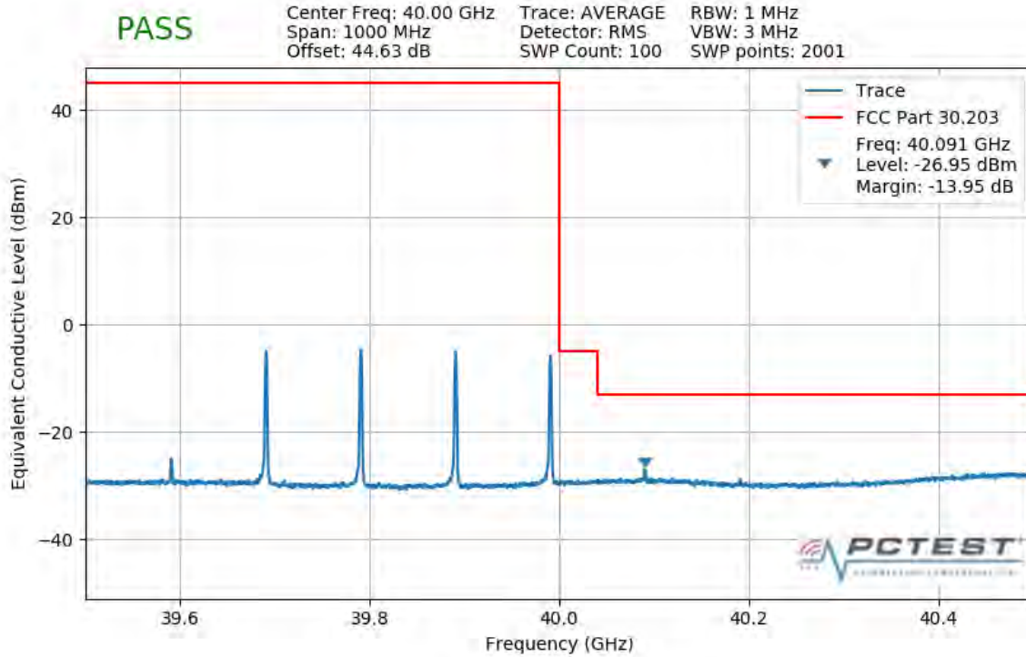
Plot 7-367. Upper Band Edge Plot (4CC 400MHz 16QAM 1 RB)
