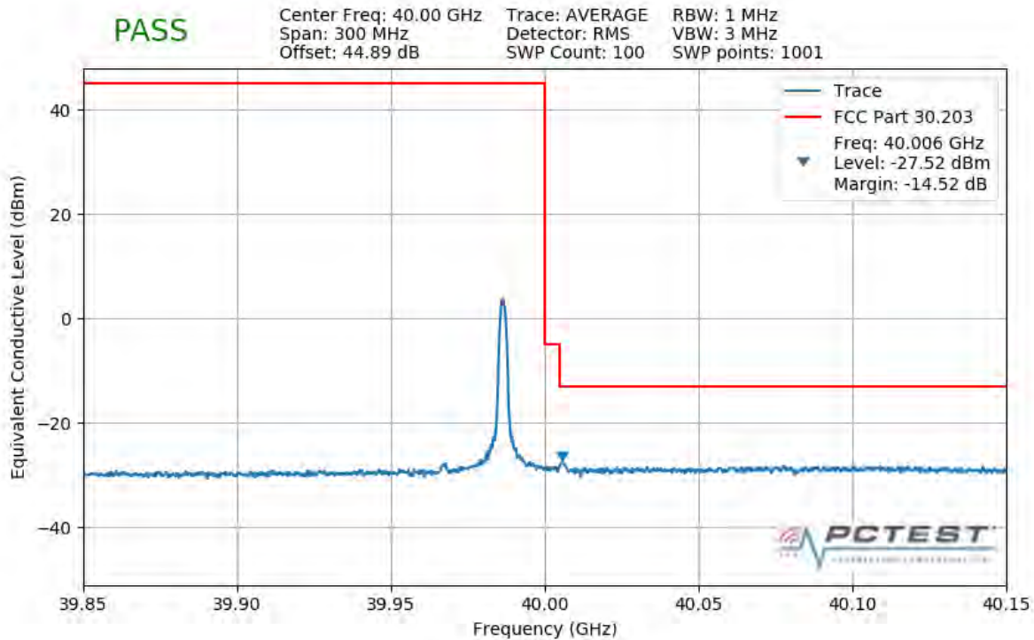
Plot 7-356. Upper Band Edge Plot (1CC 50MHz 64QAM 1 RB)
