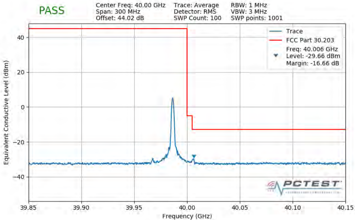
Plot 7-452. Upper Band Edge Plot (1CC 50MHz 64QAM 1 RB)
