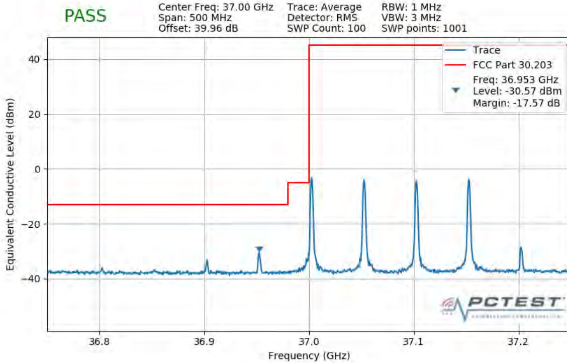
Plot 7-507. Lower Band Edge Plot (4CC 200MHz 16QAM 1 RB)
