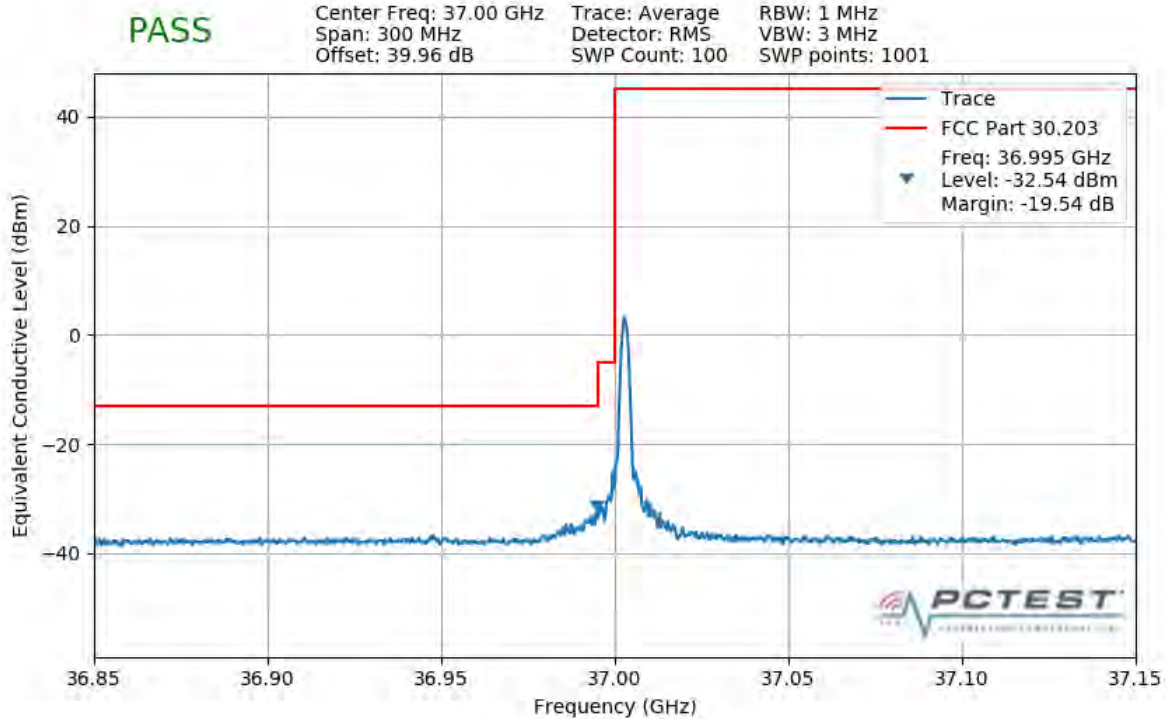
Plot 7-499. Lower Band Edge Plot (1CC 50MHz 16QAM 1 RB)
