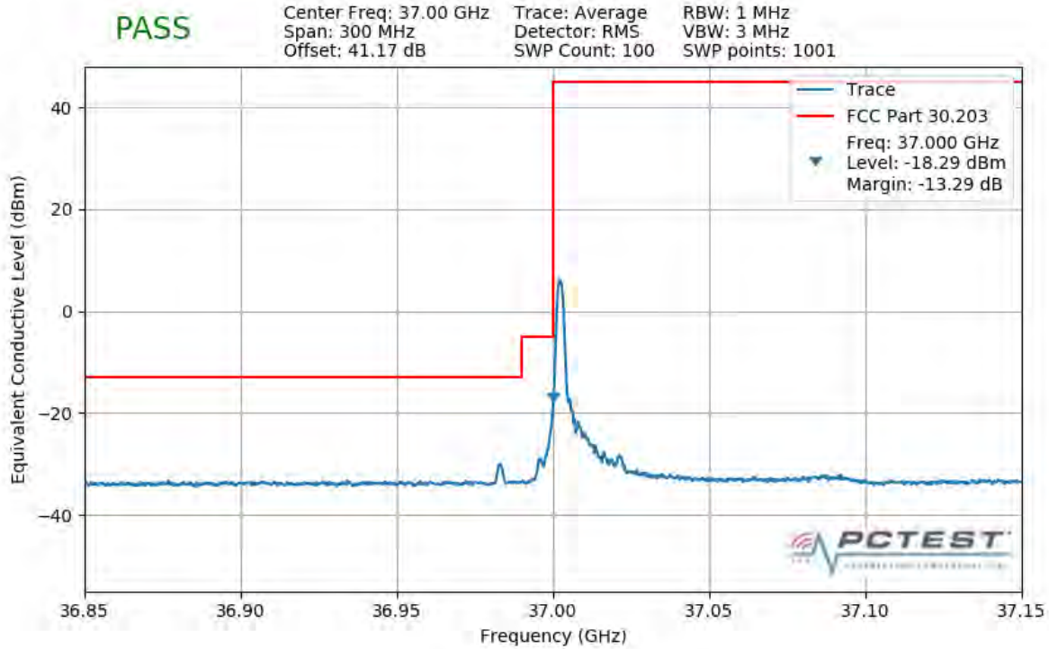
Plot 7-471. Lower Band Edge Plot (1CC 100MHz 16QAM 1 RB)
