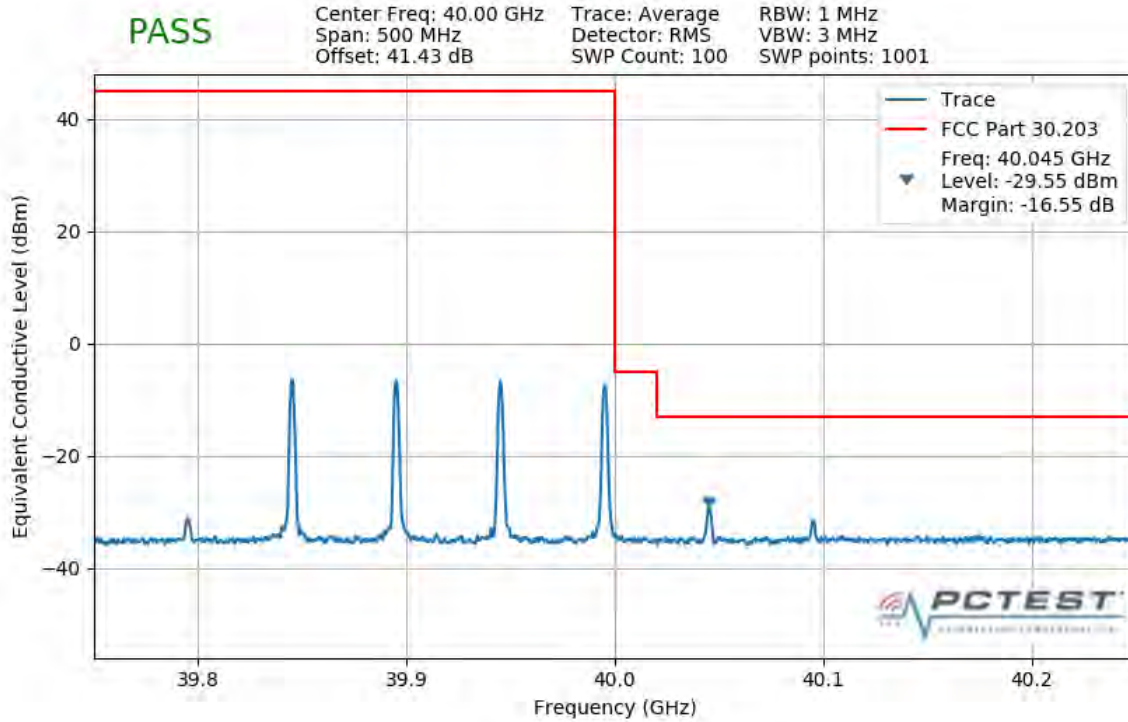
Plot 7-427. Upper Band Edge Plot (4CC 200MHz 16QAM 1 RB)
