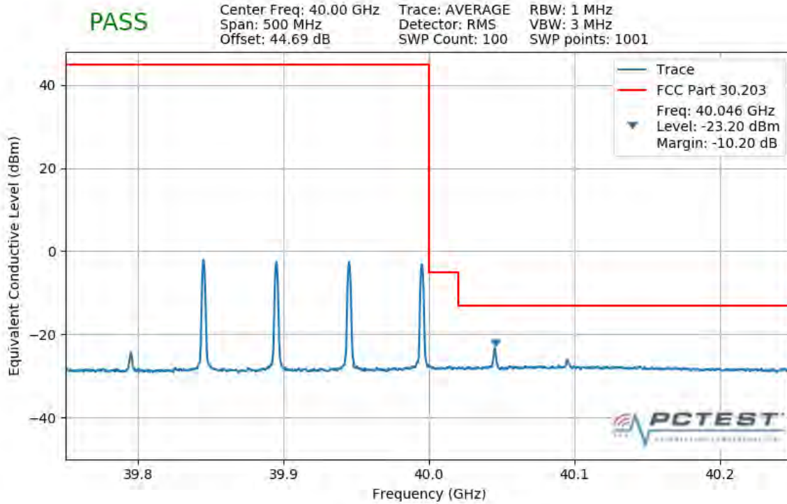
Plot 7-395. Upper Band Edge Plot (4CC 200MHz 16QAM 1 RB)
