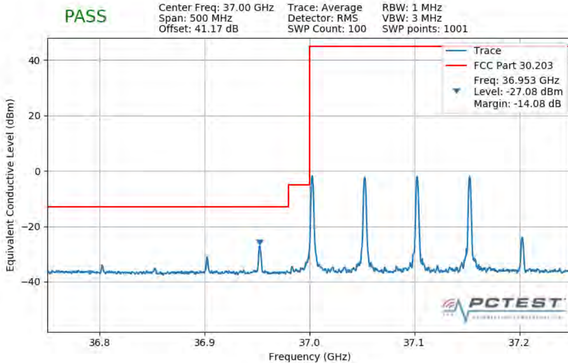
Plot 7-442. Lower Band Edge Plot (4CC 200MHz QPSK 1 RB)
