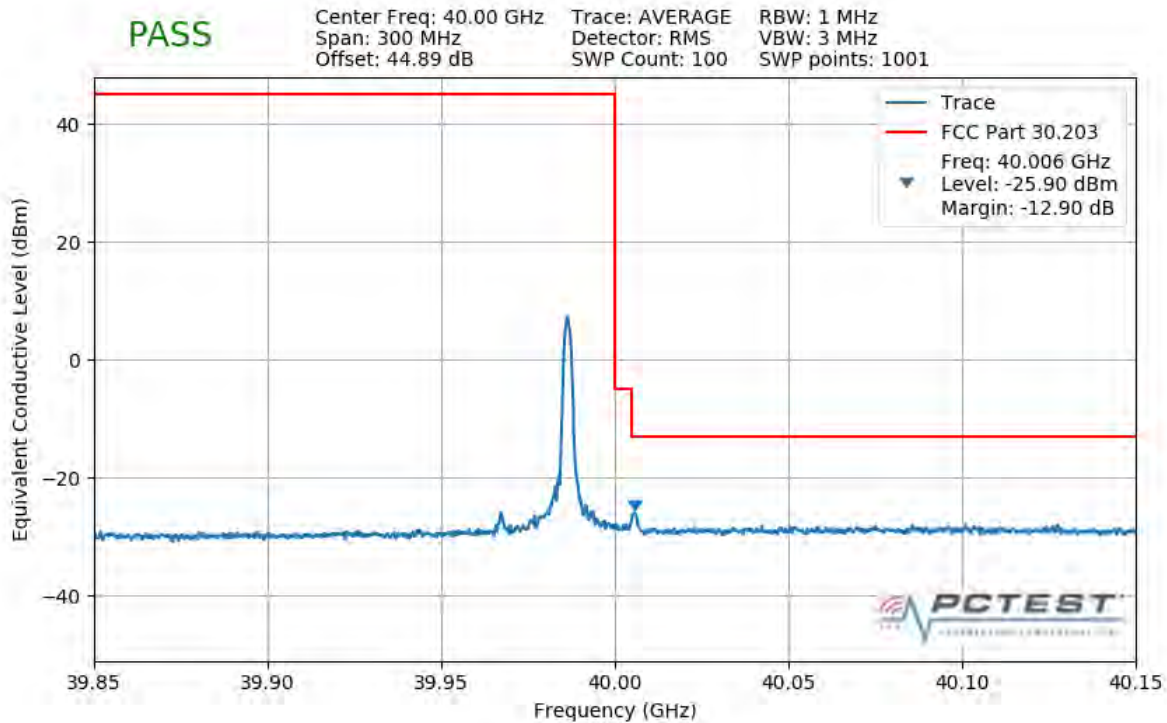
Plot 7-354. Upper Band Edge Plot (1CC 50MHz QPSK 1 RB)
