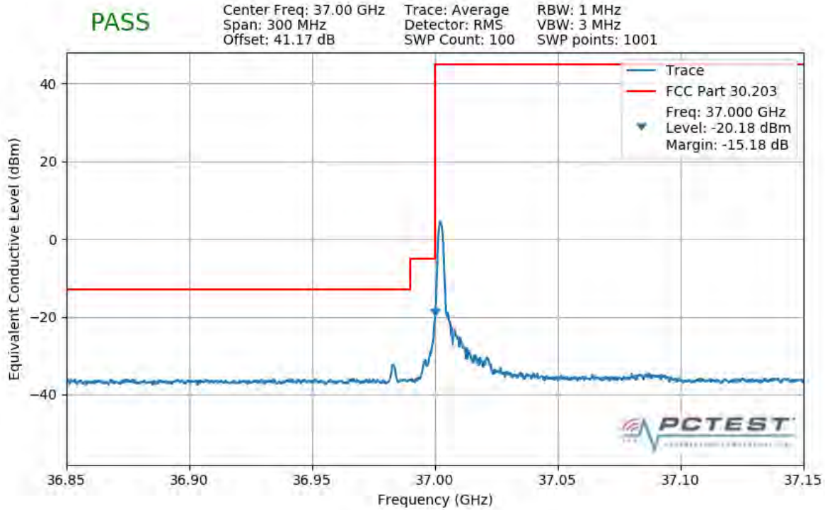
Plot 7-439. Lower Band Edge Plot (1CC 100MHz 16QAM 1 RB)
