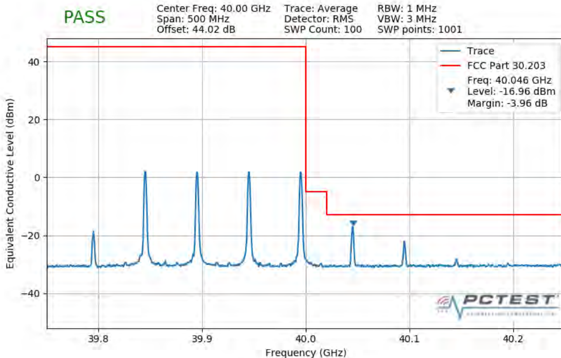
Plot 7-490. Upper Band Edge Plot (4CC 200MHz QPSK 1 RB)
