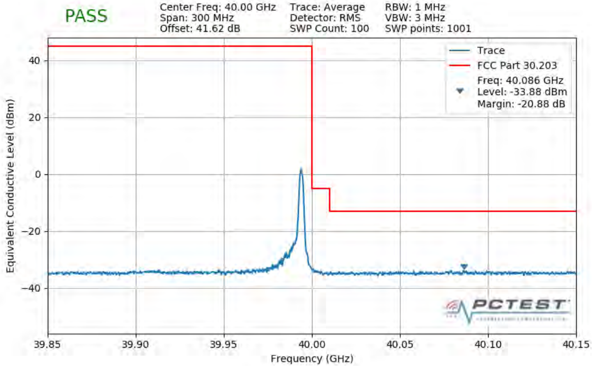
Plot 7-519. Upper Band Edge Plot (1CC 100MHz 16QAM 1 RB)
