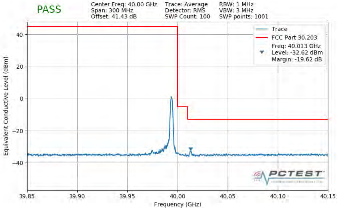
Plot 7-422. Upper Band Edge Plot (1CC 100MHz QPSK 1 RB)
