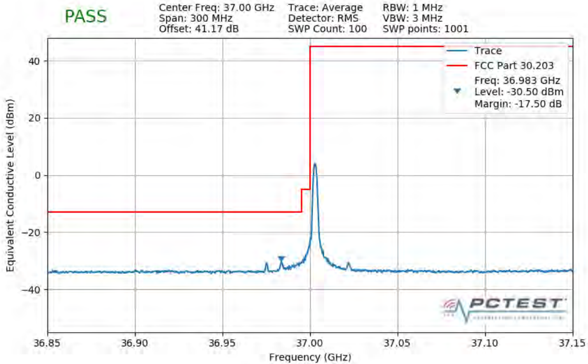
Plot 7-468. Lower Band Edge Plot (1CC 50MHz 64QAM 1 RB)
