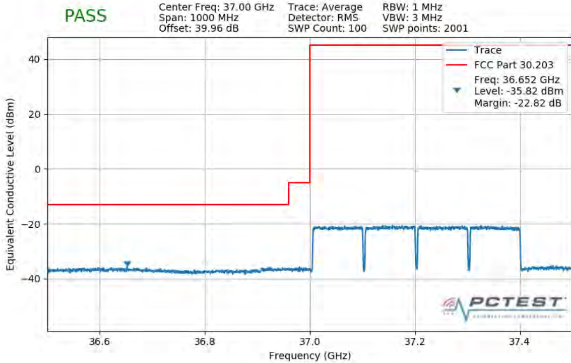
Plot 7-509. Lower Band Edge Plot (4CC 400MHz QPSK Full RB)
