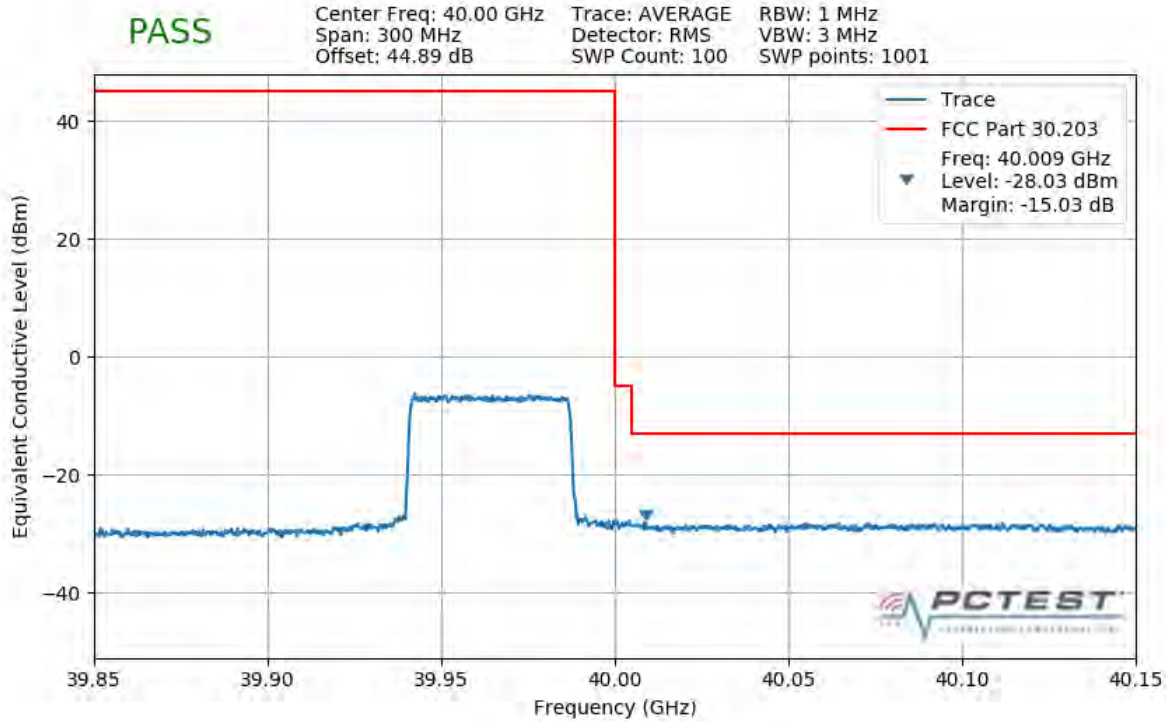
Plot 7-353. Upper Band Edge Plot (1CC 50MHz QPSK Full RB)
