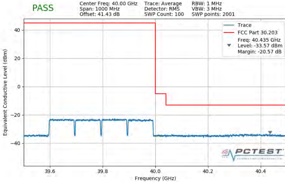
Plot 7-429. Upper Band Edge Plot (4CC 400MHz QPSK Full RB)
