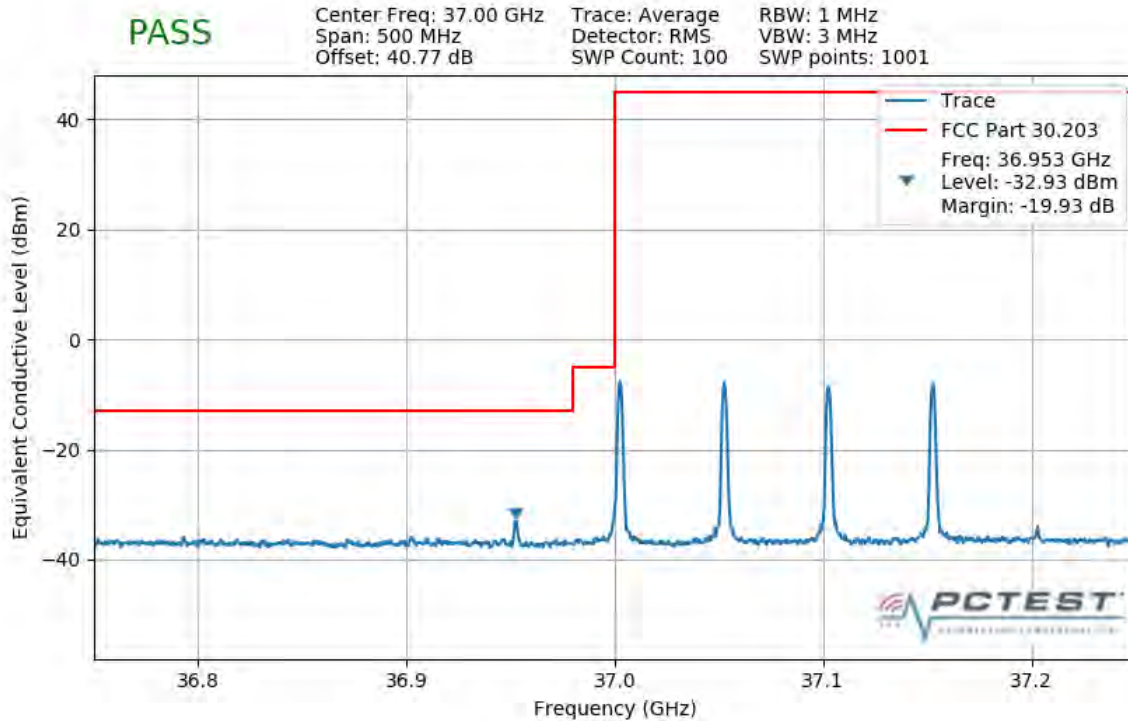
Plot 7-412. Lower Band Edge Plot (4CC 200MHz 64QAM 1 RB)
