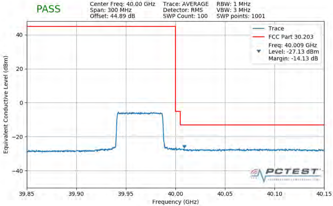
Plot 7-385. Upper Band Edge Plot (1CC 50MHz QPSK Full RB)
