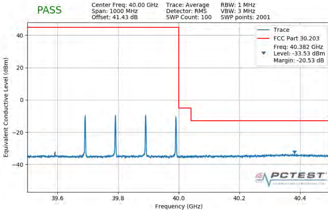
Plot 7-432. Upper Band Edge Plot (4CC 400MHz 64QAM 1 RB)
