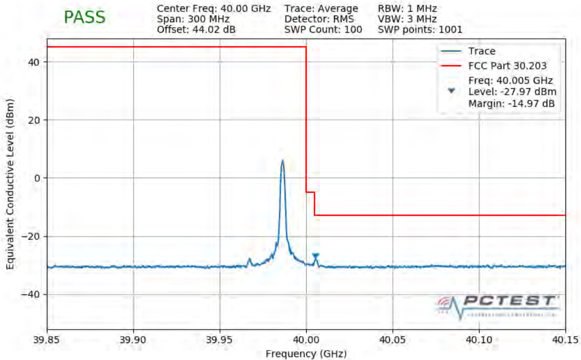
Plot 7-484. Upper Band Edge Plot (1CC 50MHz 64QAM 1 RB)
