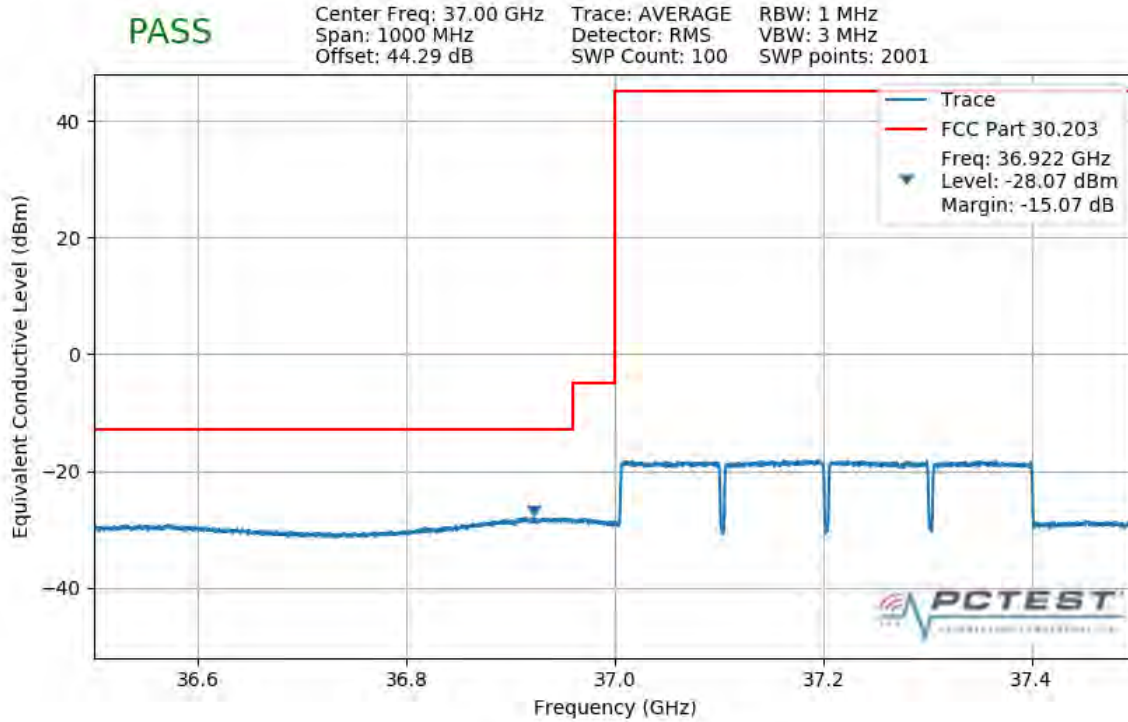
Plot 7-381. Lower Band Edge Plot (4CC 400MHz QPSK Full RB)
