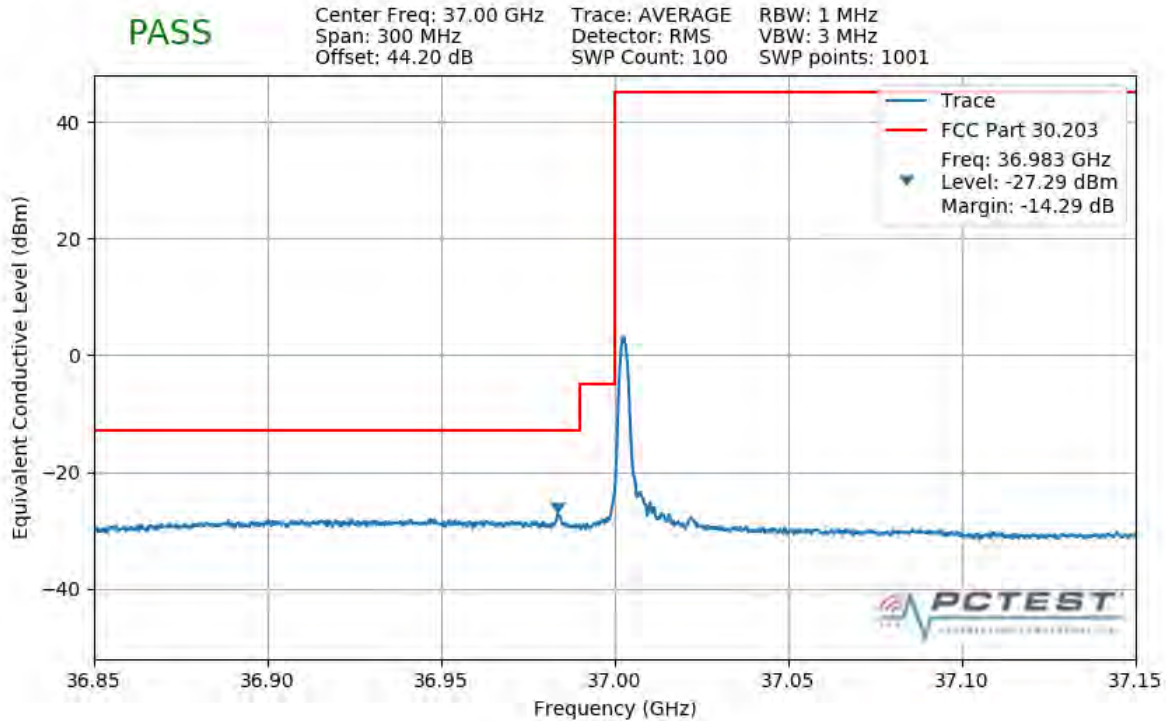
Plot 7-376. Lower Band Edge Plot (1CC 100MHz 64QAM 1 RB)
