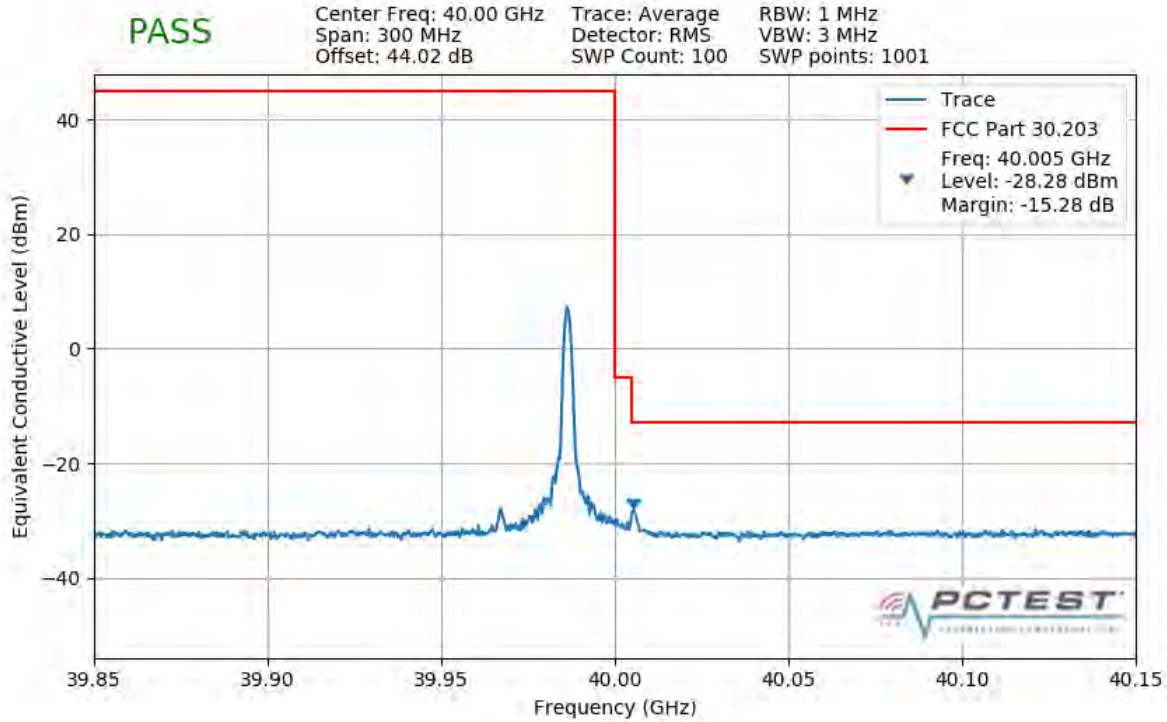
Plot 7-451. Upper Band Edge Plot (1CC 50MHz 16QAM 1 RB)
