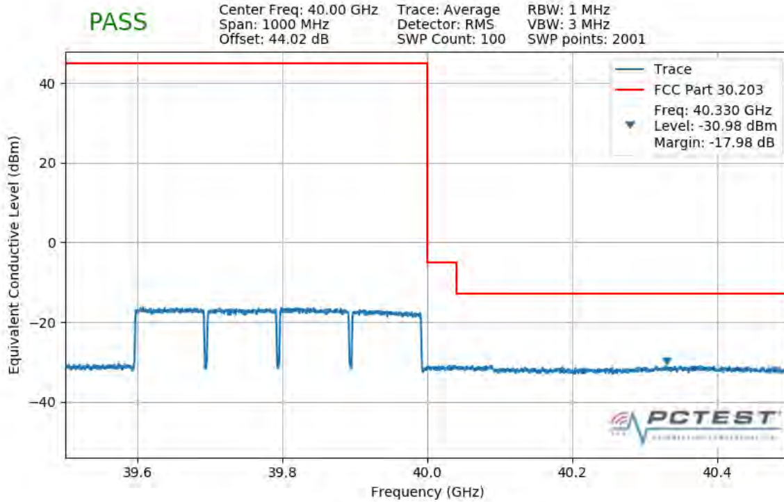
Plot 7-461. Upper Band Edge Plot (4CC 400MHz QPSK Full RB)
