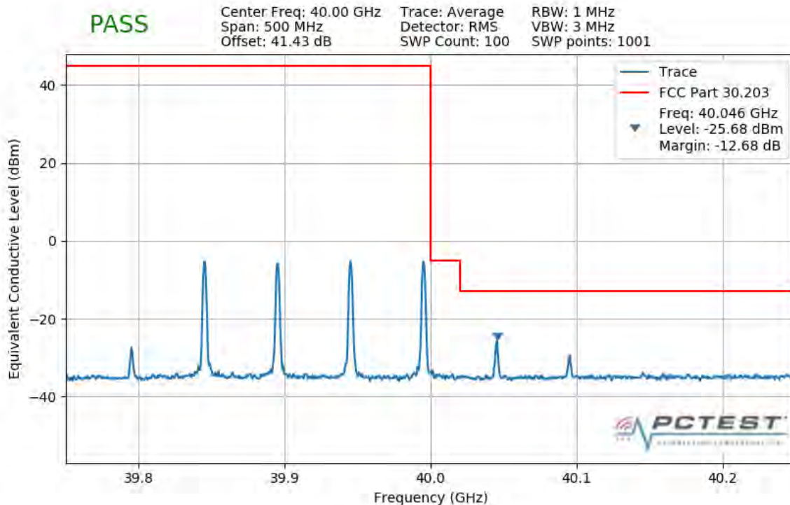
Plot 7-426. Upper Band Edge Plot (4CC 200MHz QPSK 1 RB)
