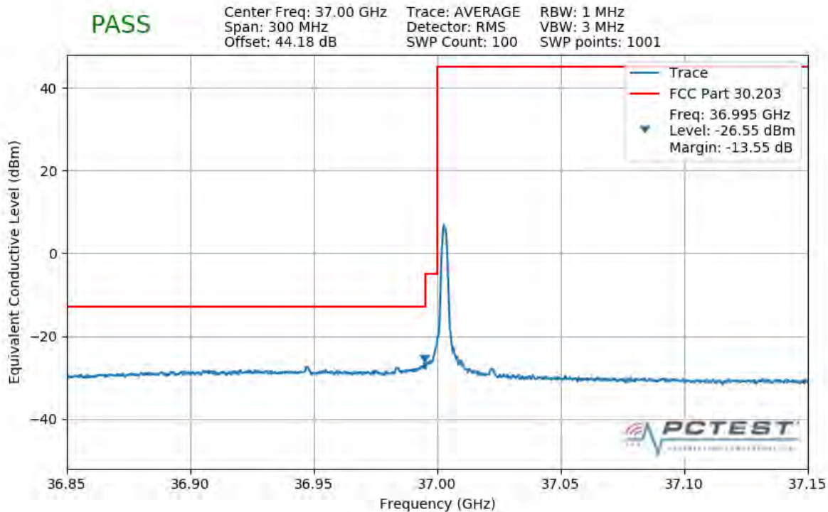
Plot 7-370. Lower Band Edge Plot (1CC 50MHz QPSK 1 RB)
