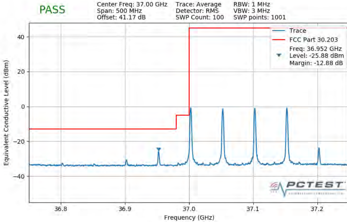
Plot 7-475. Lower Band Edge Plot (4CC 200MHz 16QAM 1 RB)
