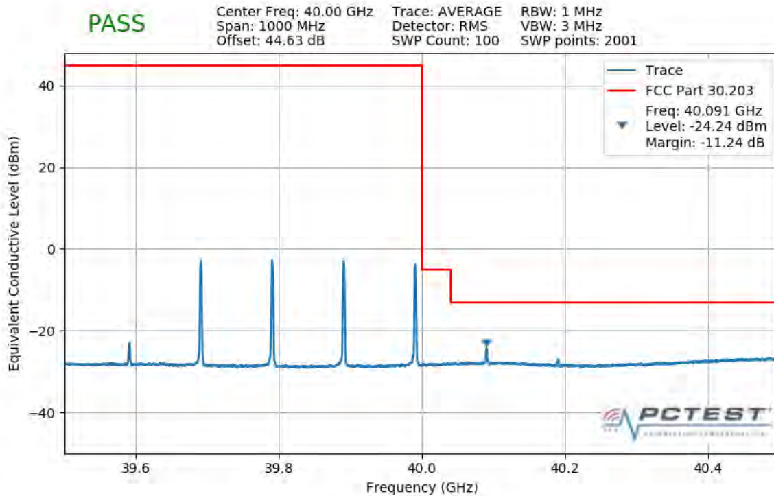
Plot 7-398. Upper Band Edge Plot (4CC 400MHz QPSK 1 RB)
