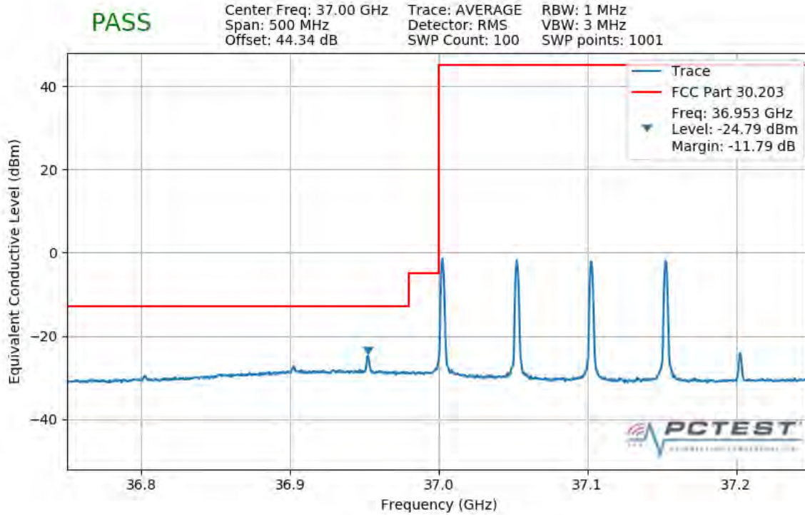
Plot 7-379. Lower Band Edge Plot (4CC 200MHz 16QAM 1 RB)
