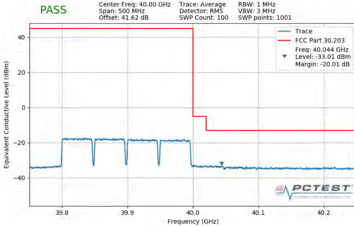
Plot 7-521. Upper Band Edge Plot (4CC 200MHz QPSK Full RB)
