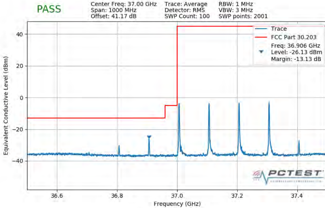
Plot 7-447. Lower Band Edge Plot (4CC 400MHz 16QAM 1 RB)
