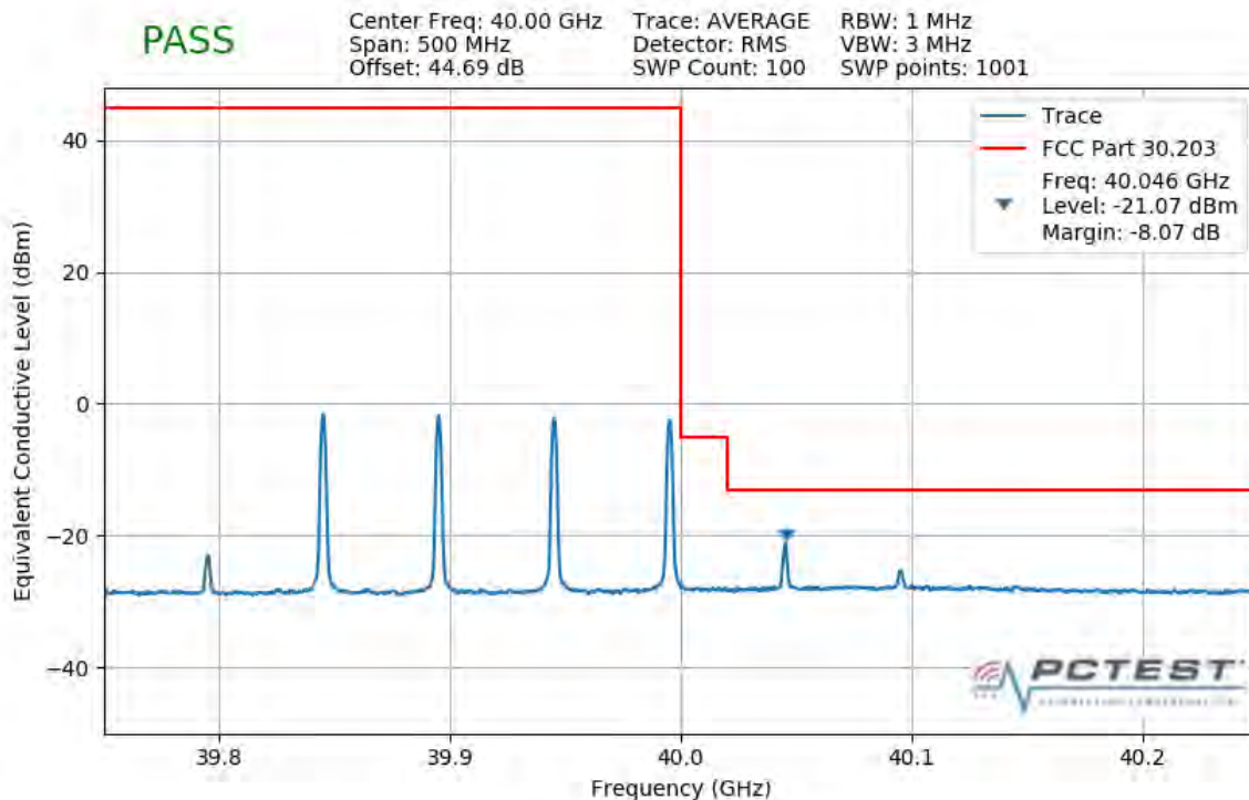
Plot 7-394. Upper Band Edge Plot (4CC 200MHz QPSK 1 RB)
