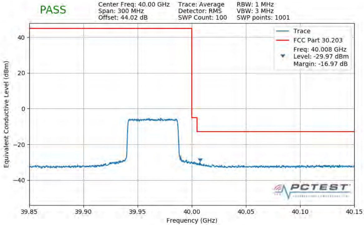
Plot 7-449. Upper Band Edge Plot (1CC 50MHz QPSK Full RB)
