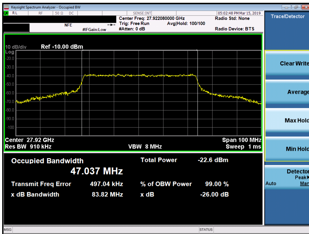
Plot 7-1. Occupied Bandwidth Plot (1CC – 50MHz - QPSK - Mid Channel)
