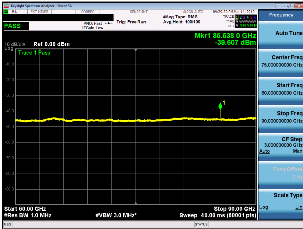
Plot 7-73. J Dipole Radiated Spurious Plot 60-90 GHz (1CC 16QAM High Channel H Beam)
