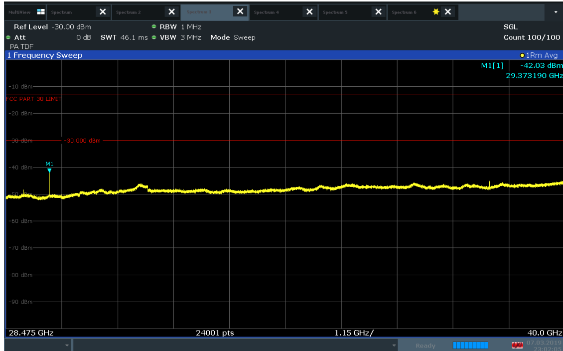
Plot 7-61. J Dipole Radiated Spurious Plot 28.475-40 GHz (1CC 16QAM High Channel H Beam)
