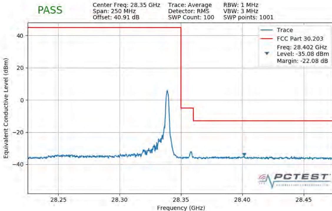
Plot 7-336. Upper Band Edge Plot (1CC 100MHz 64QAM 1 RB)
