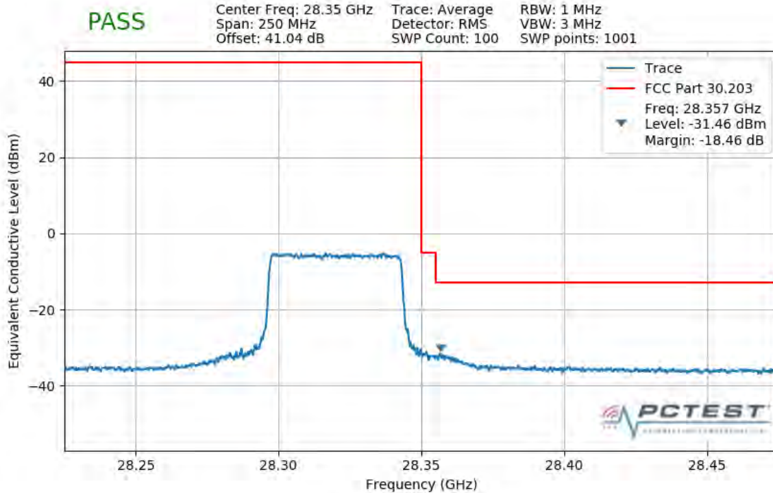
Plot 7-297. Upper Band Edge Plot (1CC 50MHz QPSK Full RB)
