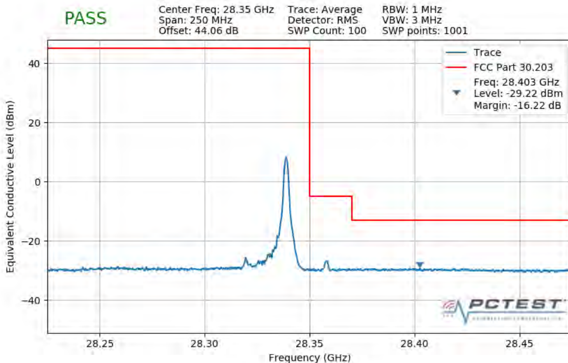
Plot 7-270. Upper Band Edge Plot (1CC 100MHz QPSK 1 RB)
