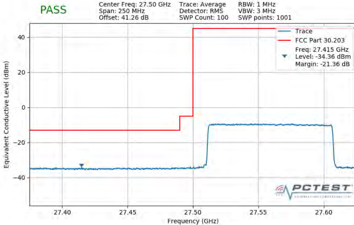
Plot 7-317. Lower Band Edge Plot (1CC 100MHz QPSK Full RB)
