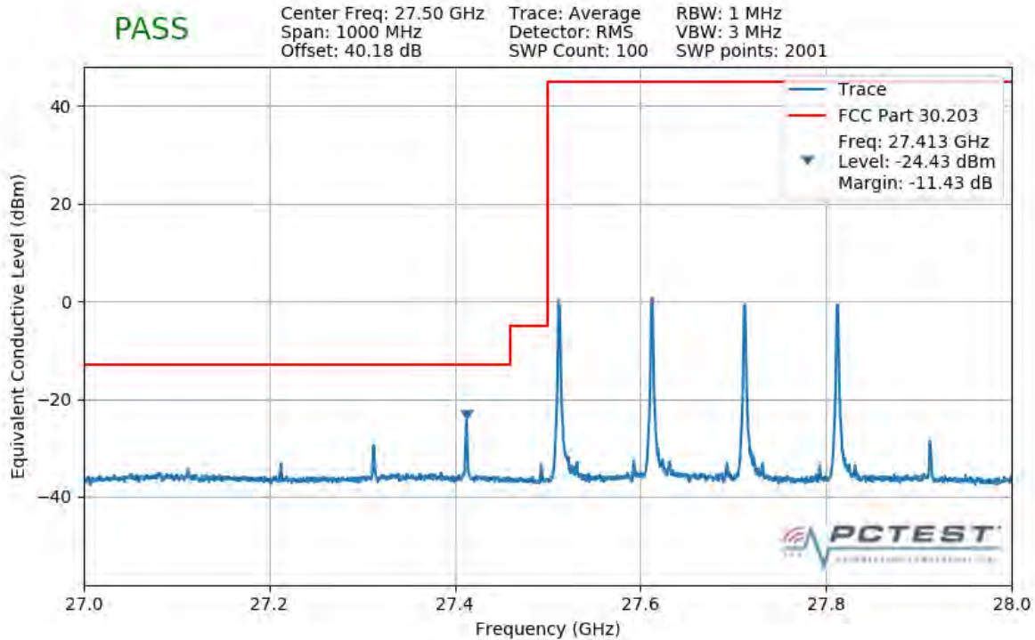
Plot 7-294. Lower Band Edge Plot (4CC 400MHz QPSK 1 RB)
