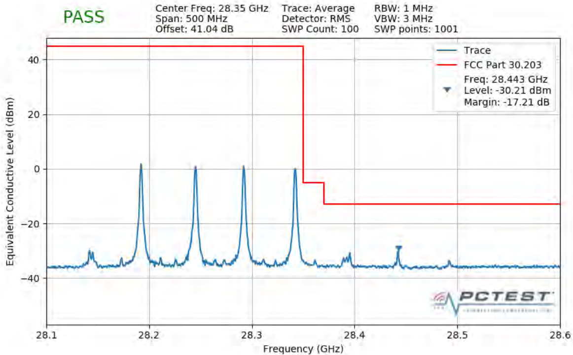
Plot 7-306. Upper Band Edge Plot (4CC 200MHz QPSK 1 RB)
