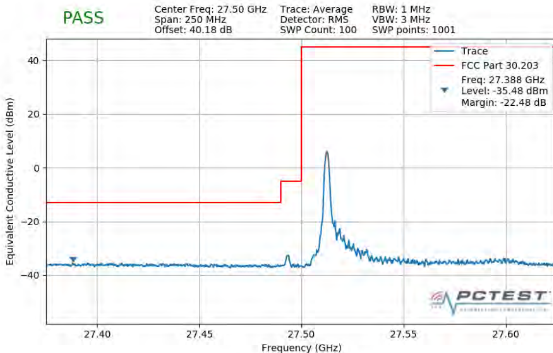
Plot 7-288. Lower Band Edge Plot (1CC 100MHz 64QAM 1 RB)
