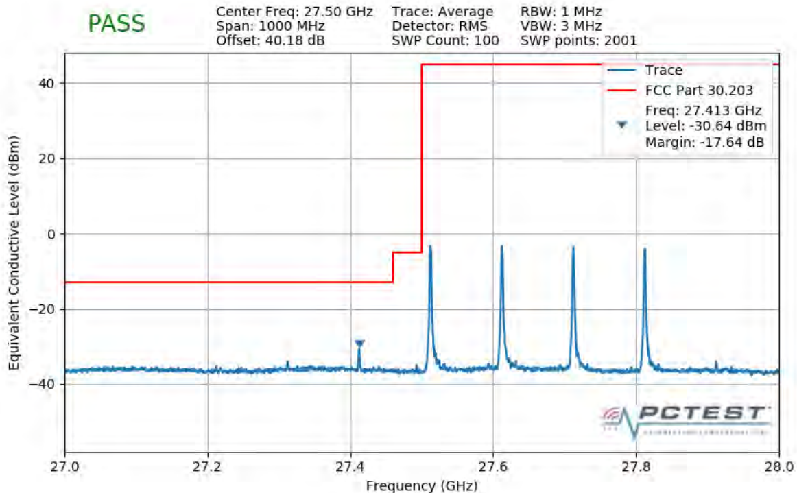
Plot 7-296. Lower Band Edge Plot (4CC 400MHz 64QAM 1 RB)
