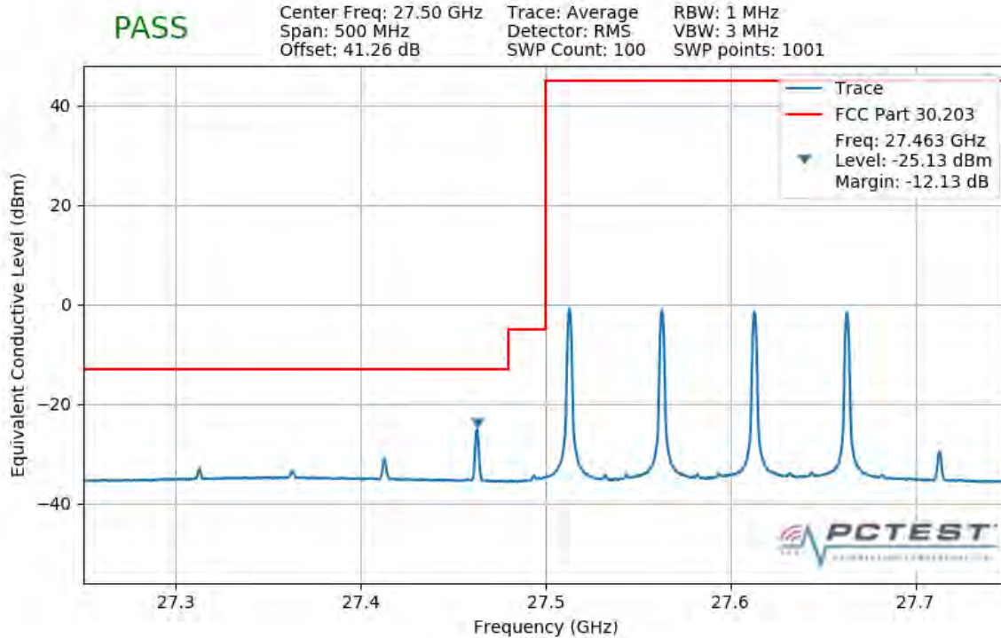
Plot 7-323. Lower Band Edge Plot (4CC 200MHz 16QAM 1 RB)
