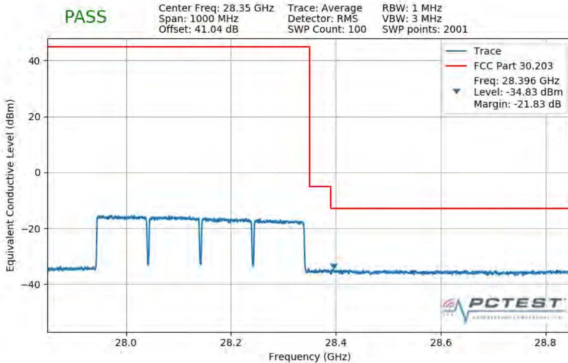
Plot 7-309. Upper Band Edge Plot (4CC 400MHz QPSK Full RB)
