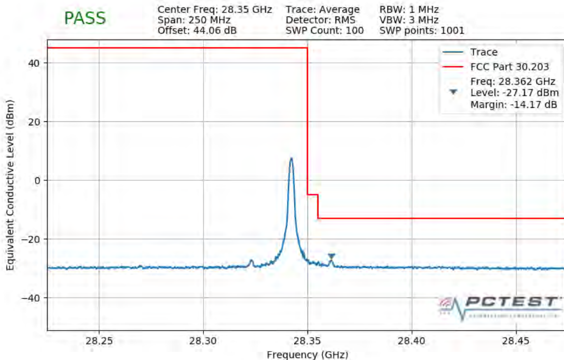
Plot 7-266. Upper Band Edge Plot (1CC 50MHz QPSK 1 RB)
