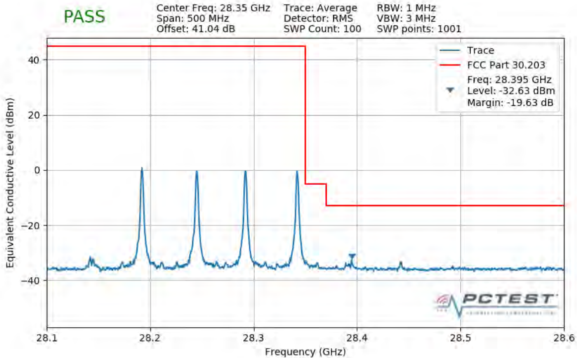
Plot 7-307. Upper Band Edge Plot (4CC 200MHz 16QAM 1 RB)
