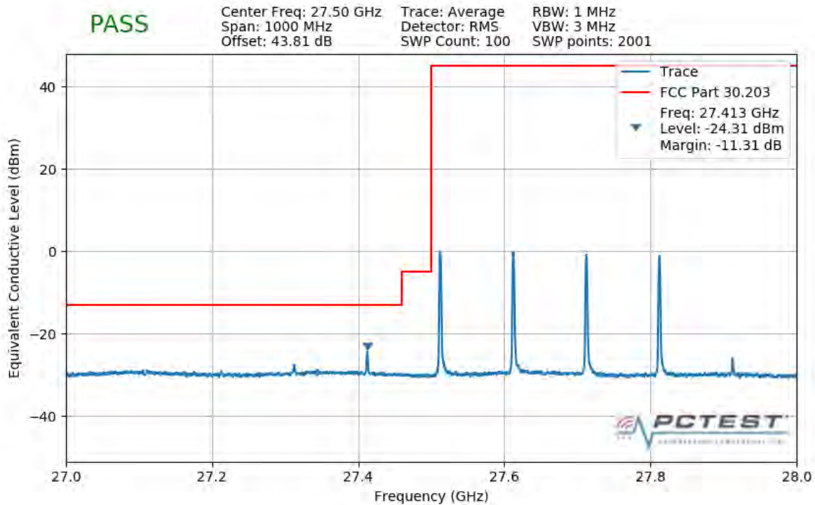
Plot 7-262. Lower Band Edge Plot (4CC 400MHz QPSK 1 RB)
