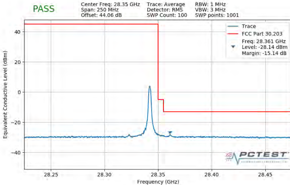
Plot 7-268. Upper Band Edge Plot (1CC 50MHz 64QAM 1 RB)
