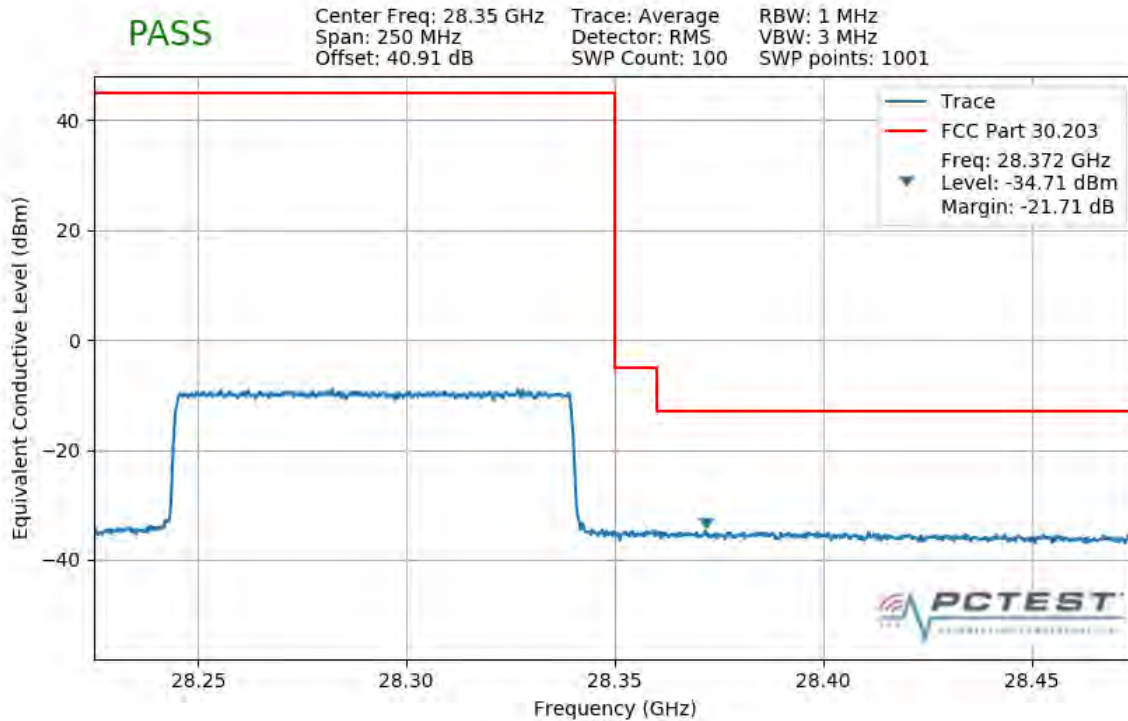
Plot 7-333. Upper Band Edge Plot (1CC 100MHz QPSK Full RB)
