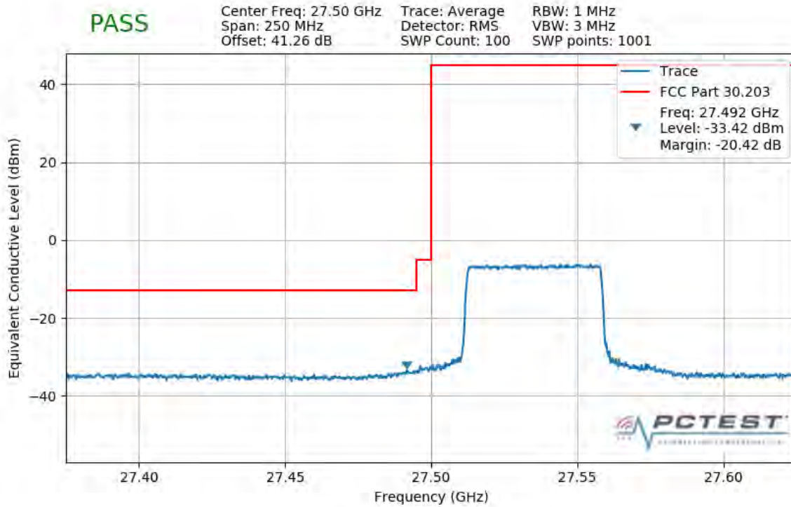
Plot 7-313. Lower Band Edge Plot (1CC 50MHz QPSK Full RB)
