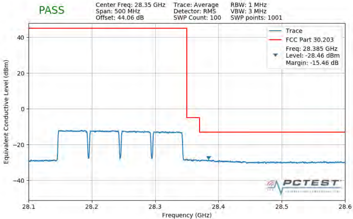
Plot 7-273. Upper Band Edge Plot (4CC 200MHz QPSK Full RB)
