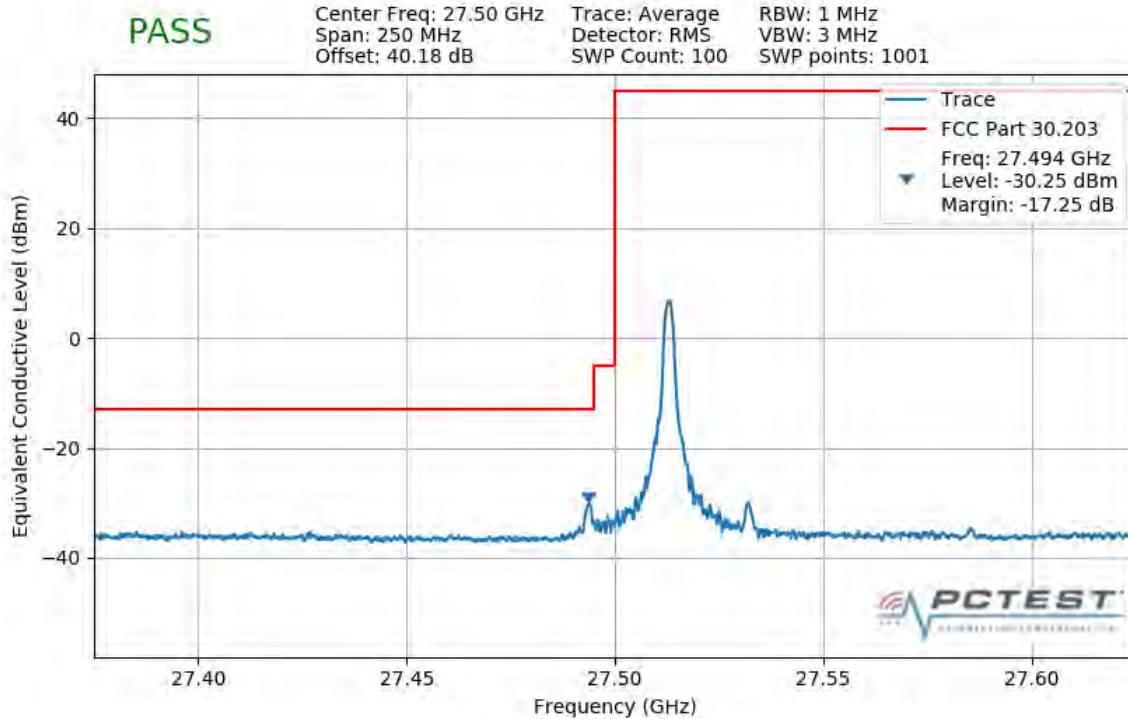
Plot 7-284. Lower Band Edge Plot (1CC 50MHz 64QAM 1 RB)
