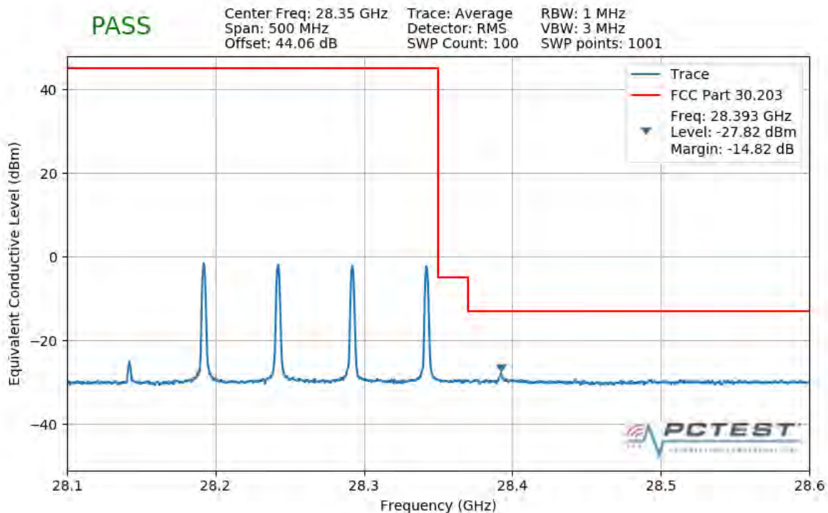
Plot 7-276. Upper Band Edge Plot (4CC 200MHz 64QAM 1 RB)
