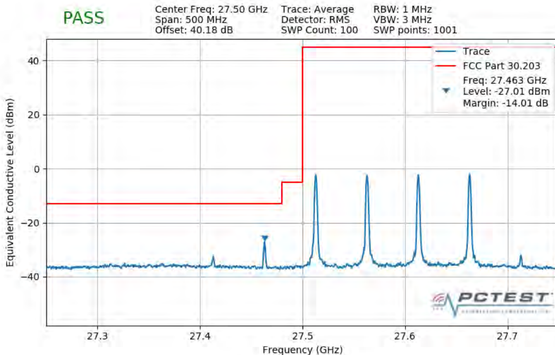
Plot 7-292. Lower Band Edge Plot (4CC 200MHz 64QAM 1 RB)
