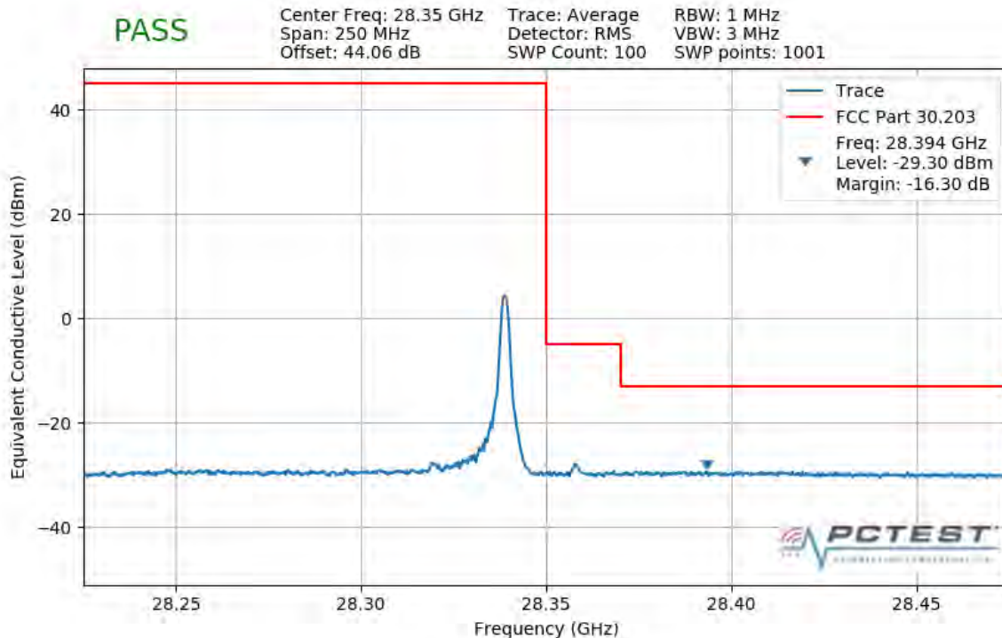
Plot 7-272. Upper Band Edge Plot (1CC 100MHz 64QAM 1 RB)
