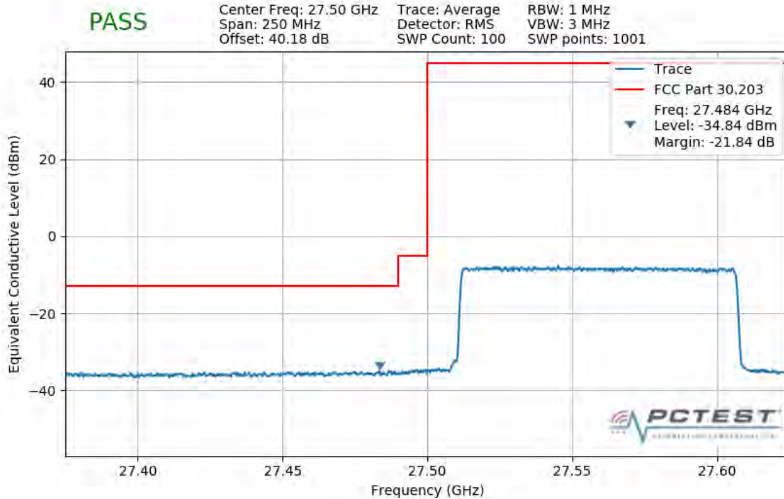
Plot 7-285. Lower Band Edge Plot (1CC 100MHz QPSK Full RB)
