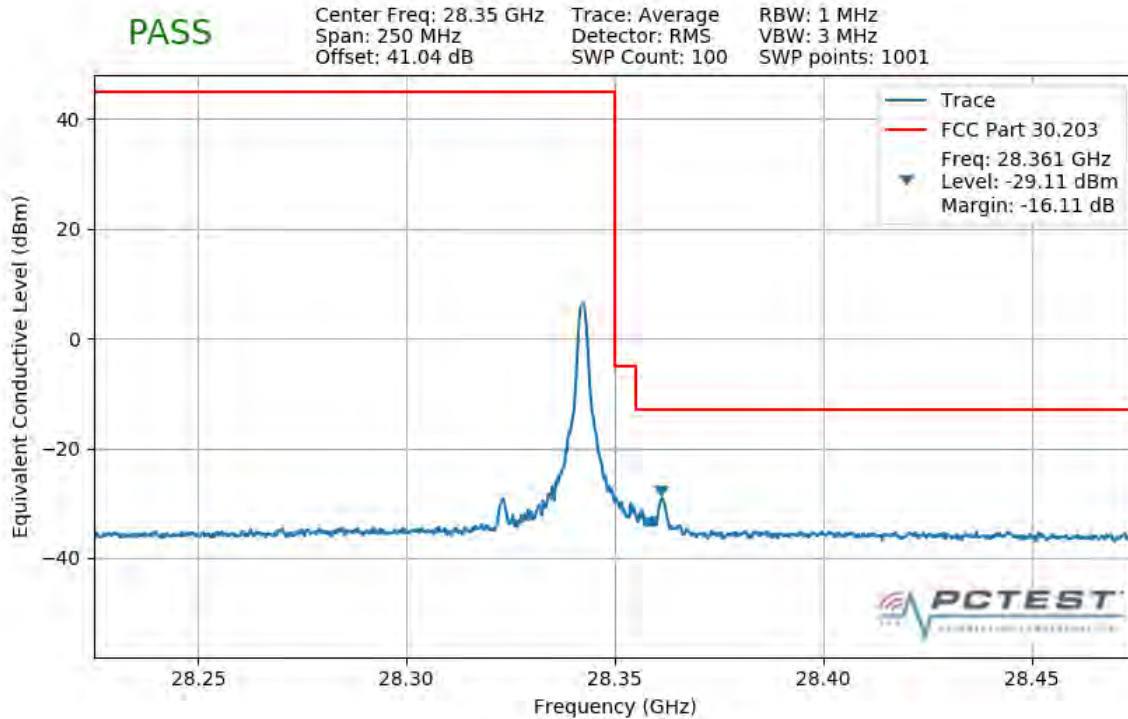
Plot 7-300. Upper Band Edge Plot (1CC 50MHz 64QAM 1 RB)
