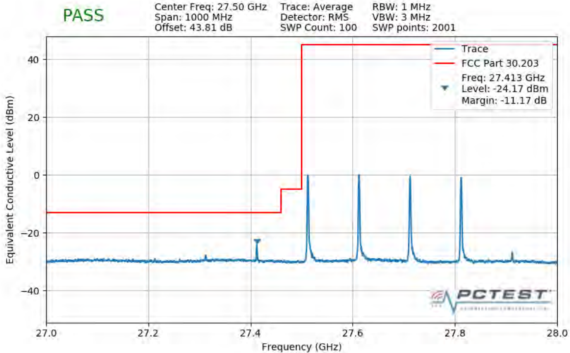
Plot 7-263. Lower Band Edge Plot (4CC 400MHz 16QAM 1 RB)
