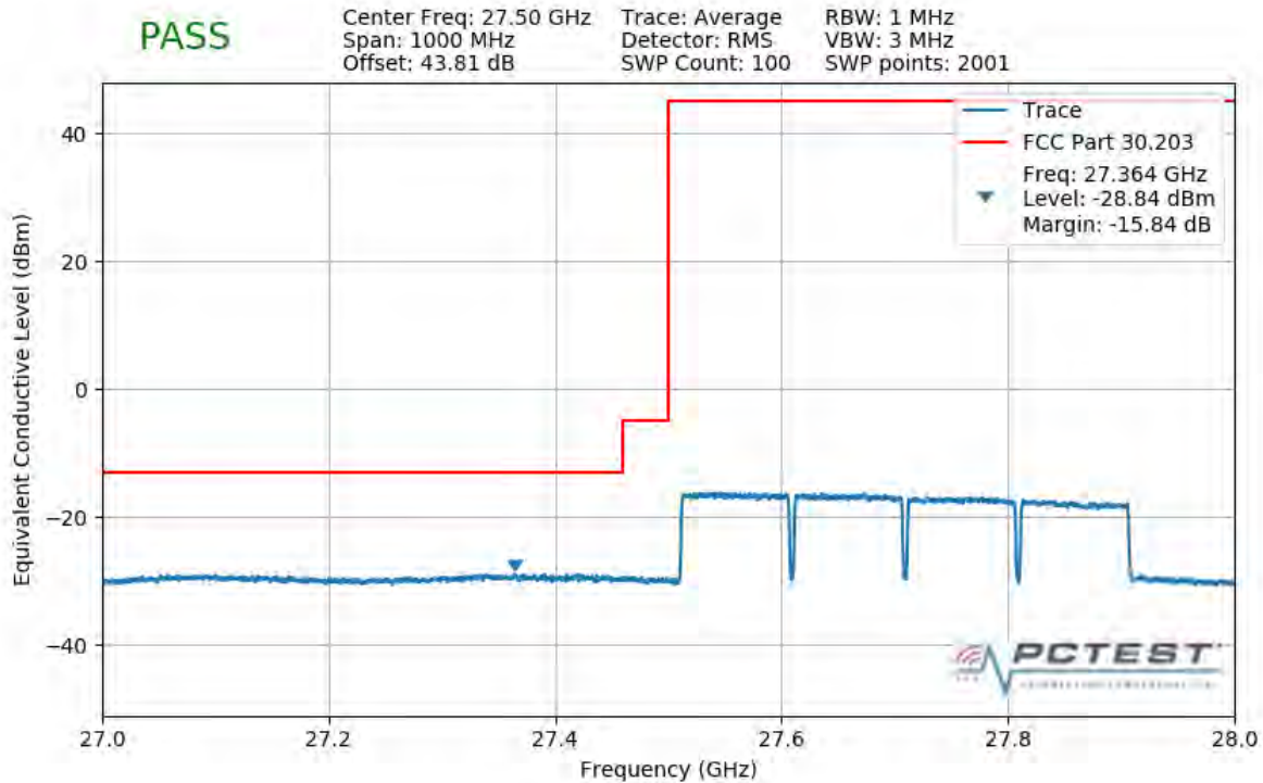
Plot 7-261. Lower Band Edge Plot (4CC 400MHz QPSK Full RB)
