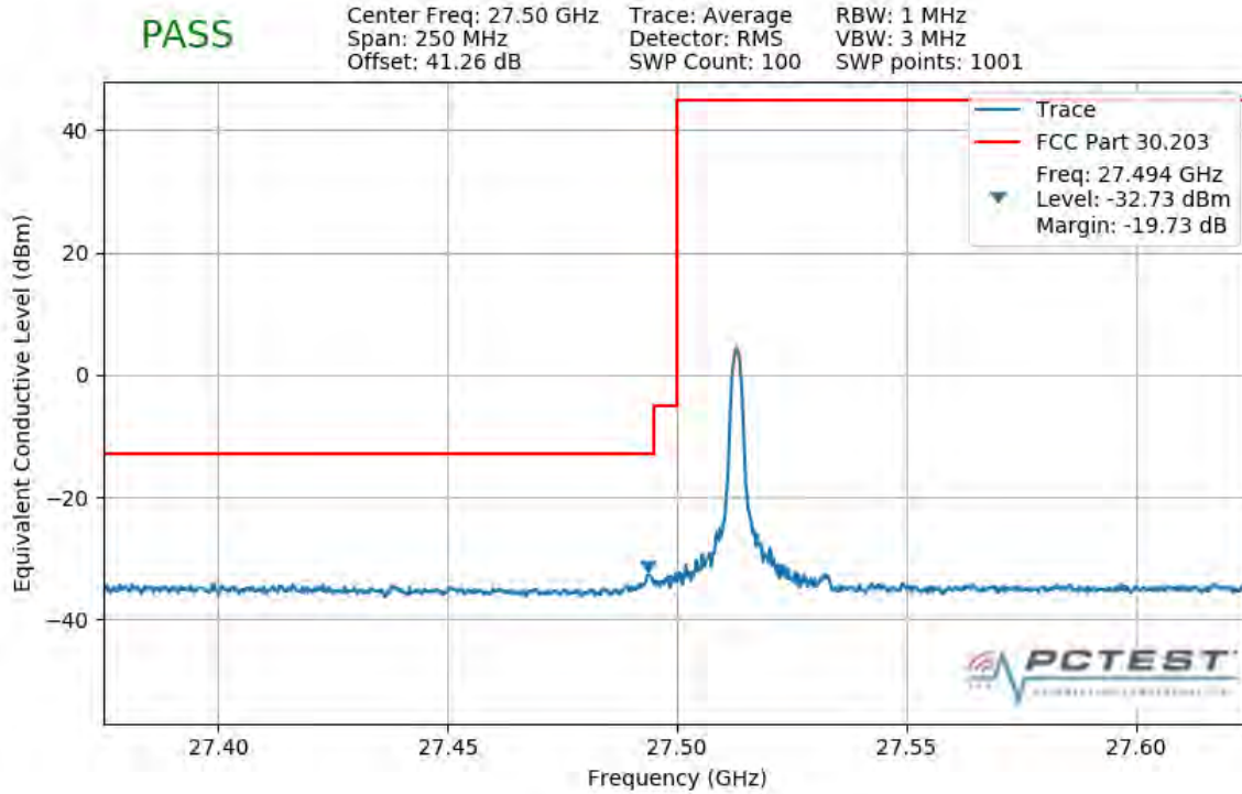
Plot 7-316. Lower Band Edge Plot (1CC 50MHz 64QAM 1 RB)
