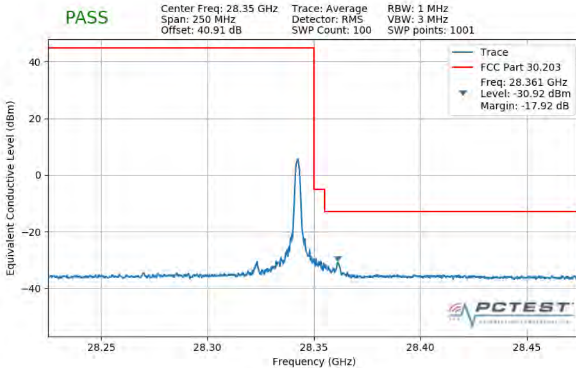
Plot 7-332. Upper Band Edge Plot (1CC 50MHz 64QAM 1 RB)
