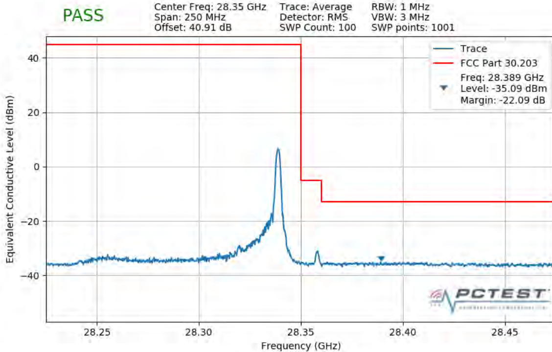
Plot 7-335. Upper Band Edge Plot (1CC 100MHz 16QAM 1 RB)
