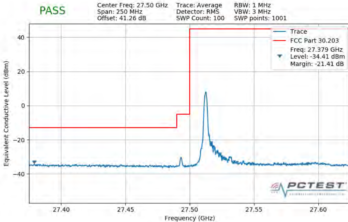
Plot 7-318. Lower Band Edge Plot (1CC 100MHz QPSK 1 RB)
