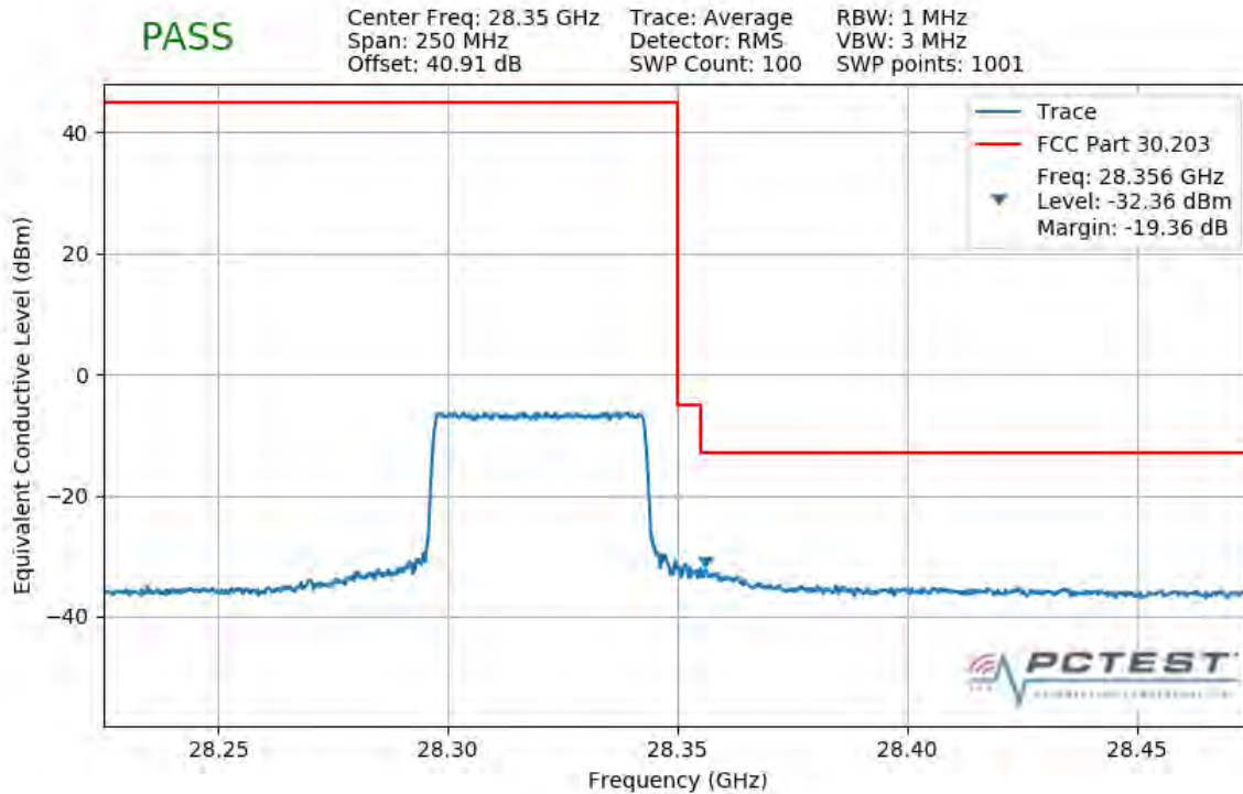
Plot 7-329. Upper Band Edge Plot (1CC 50MHz QPSK Full RB)
