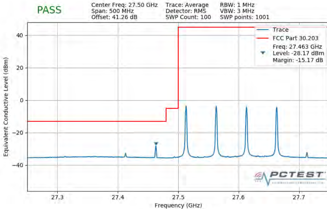
Plot 7-324. Lower Band Edge Plot (4CC 200MHz 64QAM 1 RB)
