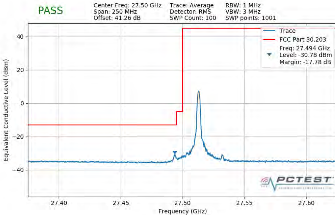
Plot 7-314. Lower Band Edge Plot (1CC 50MHz QPSK 1 RB)
