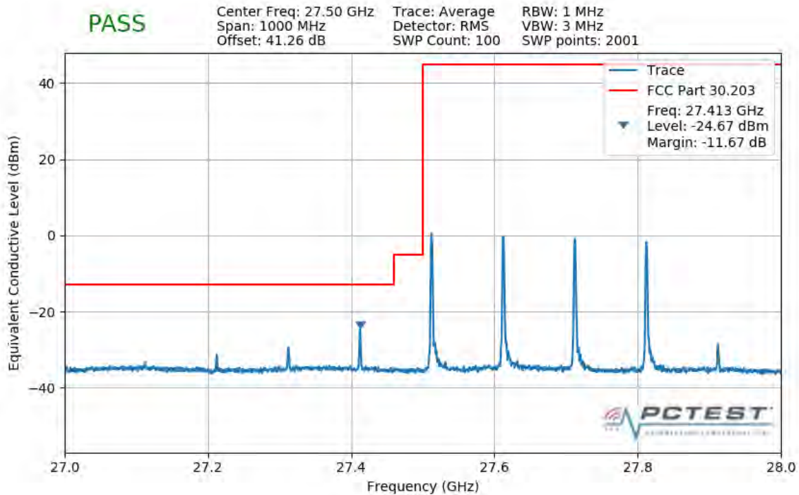
Plot 7-326. Lower Band Edge Plot (4CC 400MHz QPSK 1 RB)
