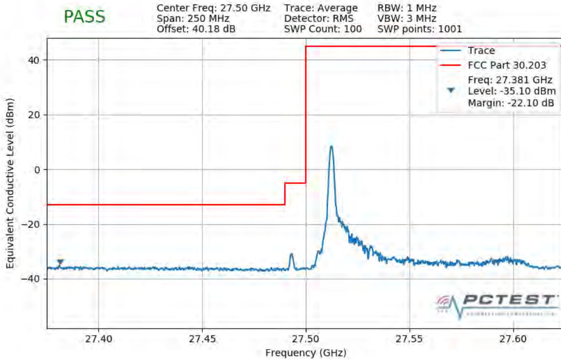
Plot 7-287. Lower Band Edge Plot (1CC 100MHz 16QAM 1 RB)
