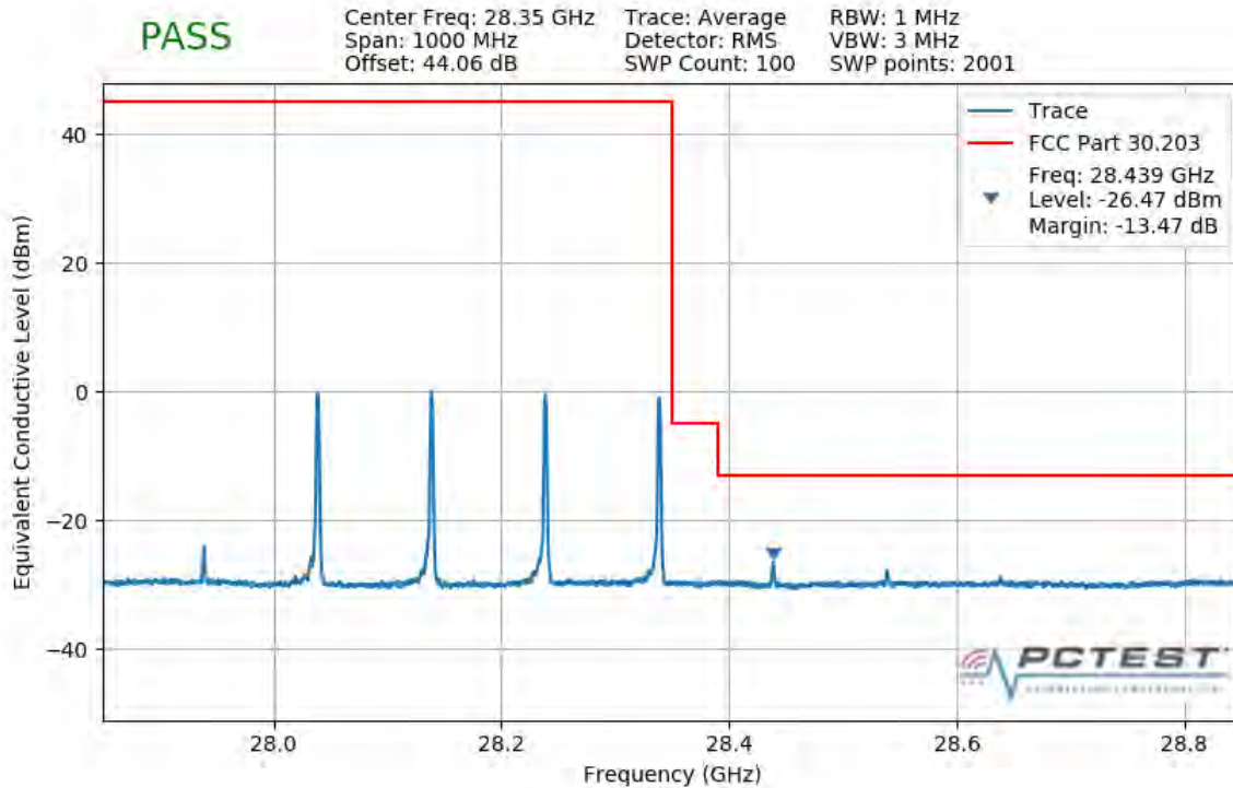
Plot 7-279. Upper Band Edge Plot (4CC 400MHz 16QAM 1 RB)
