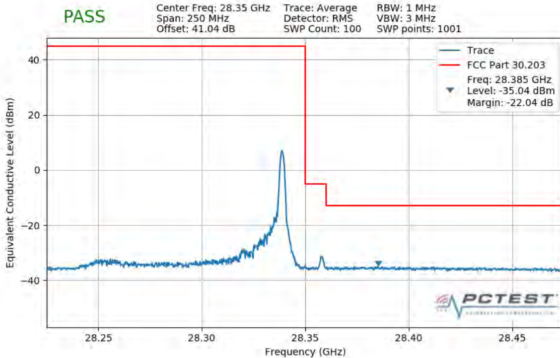
Plot 7-303. Upper Band Edge Plot (1CC 100MHz 16QAM 1 RB)
