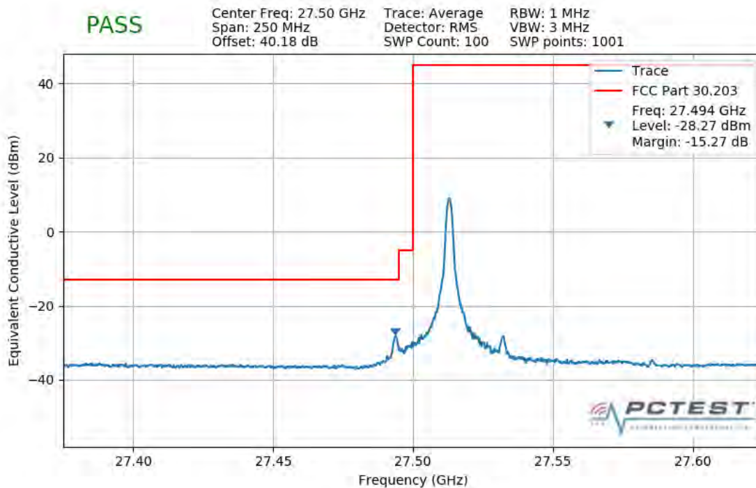
Plot 7-282. Lower Band Edge Plot (1CC 50MHz QPSK 1 RB)
