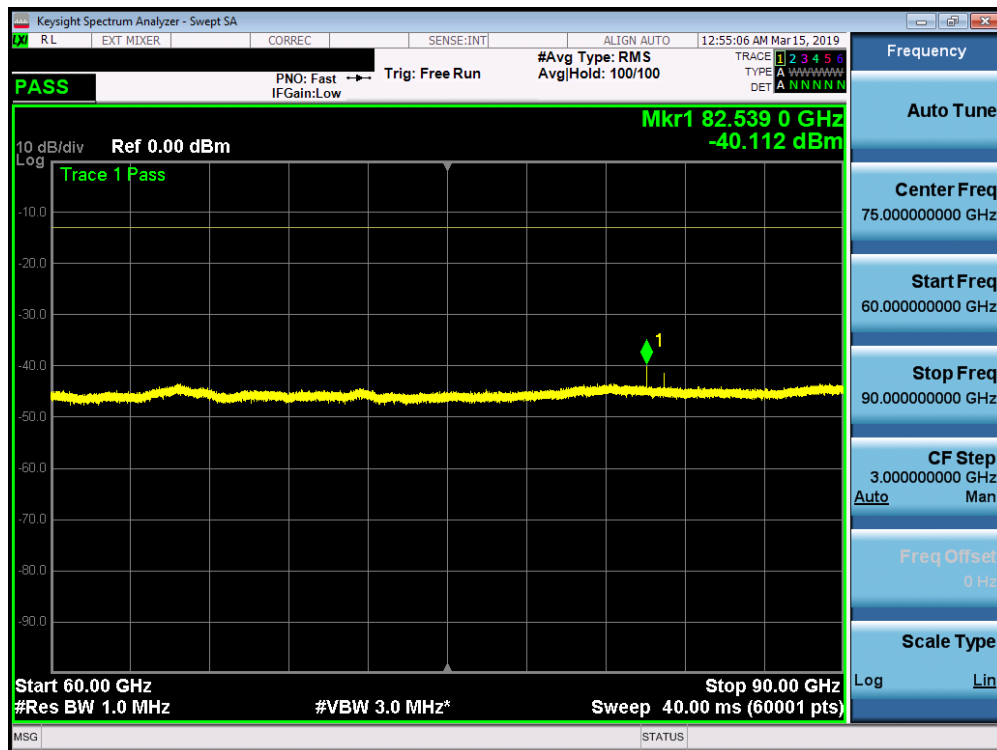
Plot 7-142. K Patch Radiated Spurious Plot 60-90 GHz (1CC QPSK Low Channel V Beam)
