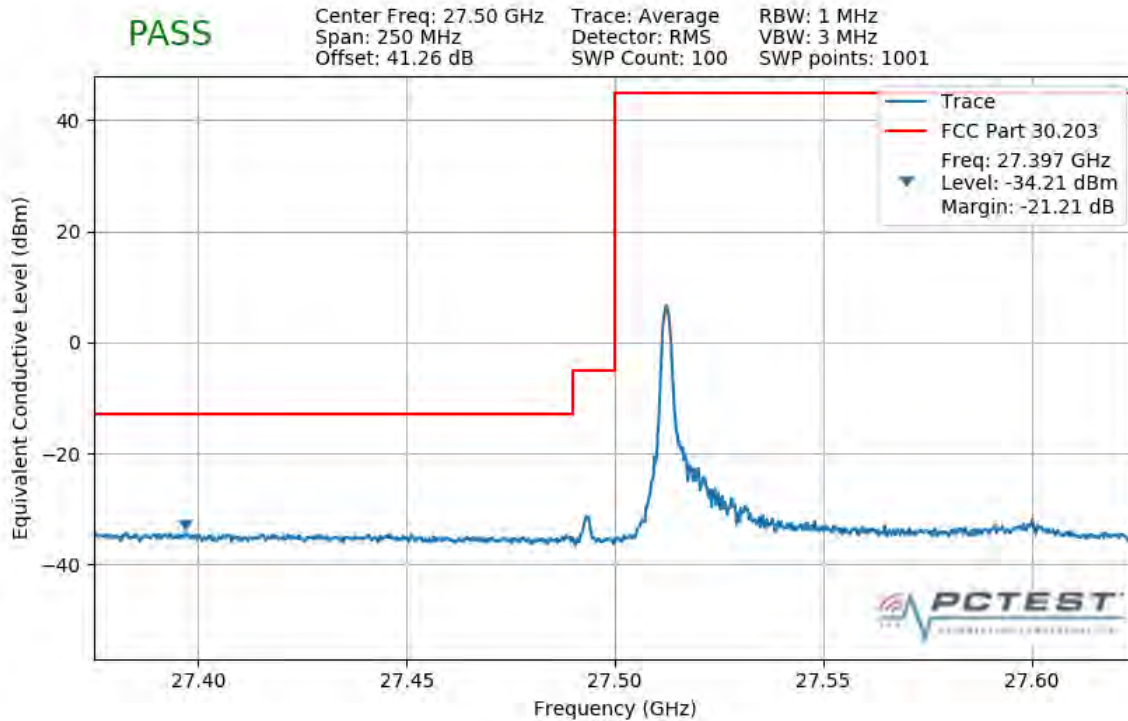
Plot 7-319. Lower Band Edge Plot (1CC 100MHz 16QAM 1 RB)
