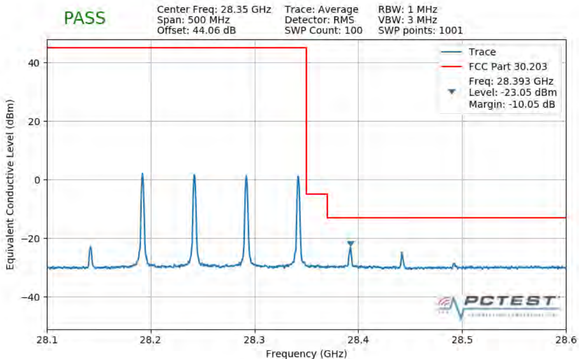
Plot 7-274. Upper Band Edge Plot (4CC 200MHz QPSK 1 RB)
