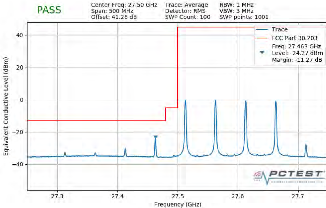
Plot 7-322. Lower Band Edge Plot (4CC 200MHz QPSK 1 RB)
