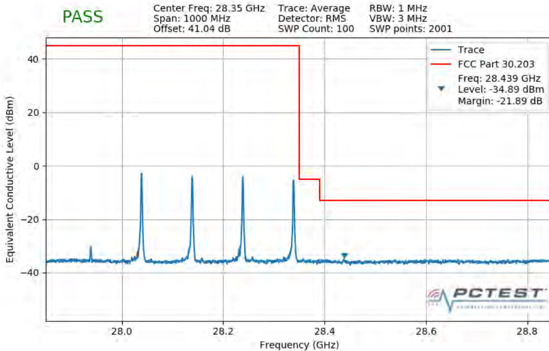
Plot 7-312. Upper Band Edge Plot (4CC 400MHz 64QAM 1 RB)
