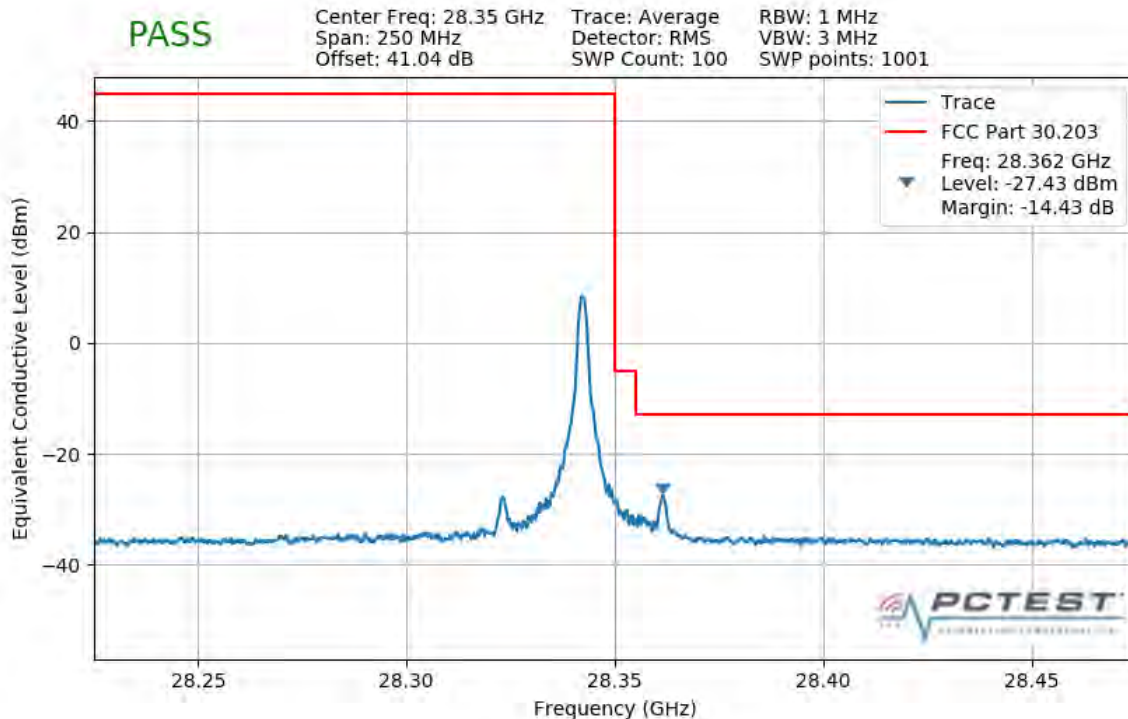
Plot 7-298. Upper Band Edge Plot (1CC 50MHz QPSK 1 RB)
