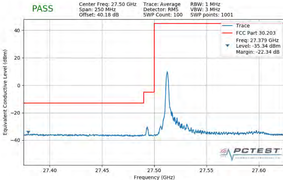
Plot 7-286. Lower Band Edge Plot (1CC 100MHz QPSK 1 RB)
