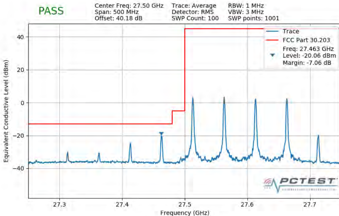
Plot 7-290. Lower Band Edge Plot (4CC 200MHz QPSK 1 RB)
