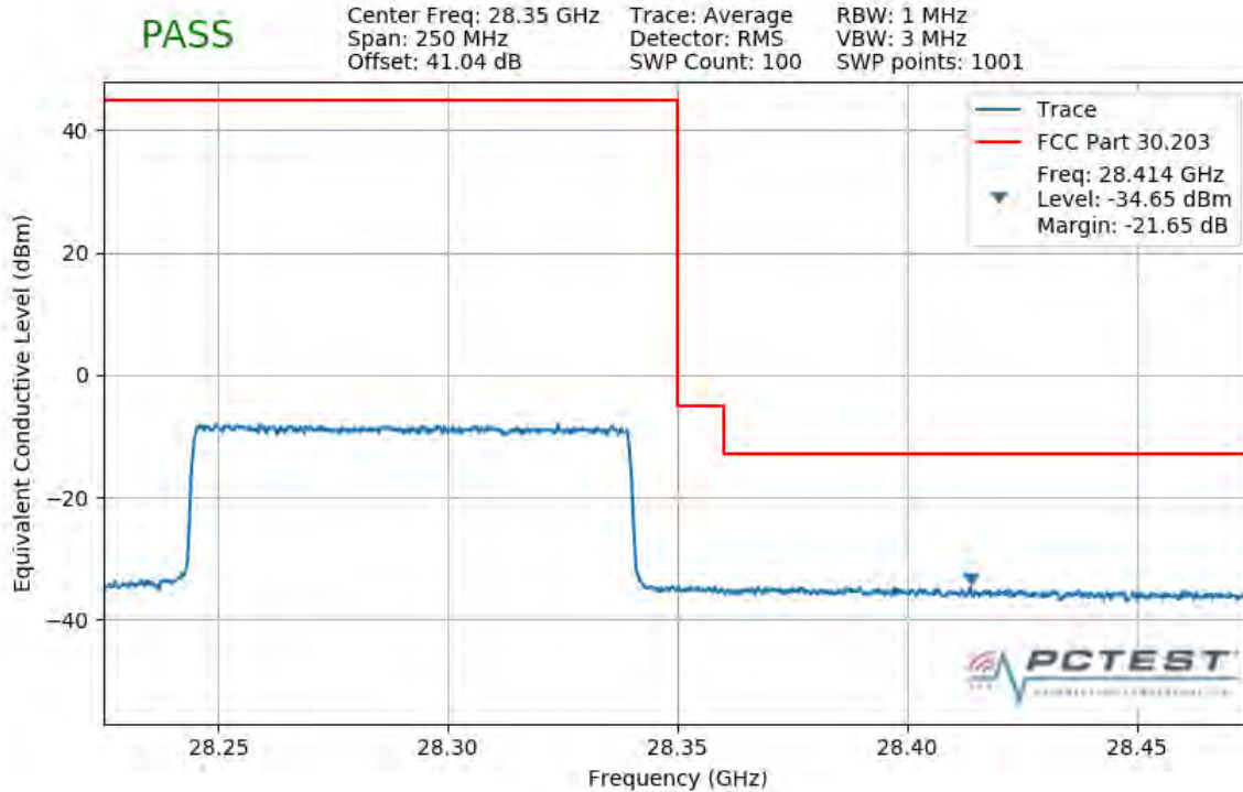
Plot 7-301. Upper Band Edge Plot (1CC 100MHz QPSK Full RB)
