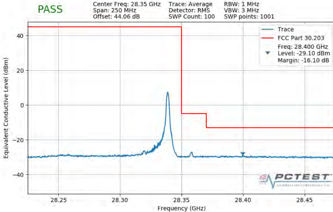
Plot 7-271. Upper Band Edge Plot (1CC 100MHz 16QAM 1 RB)
