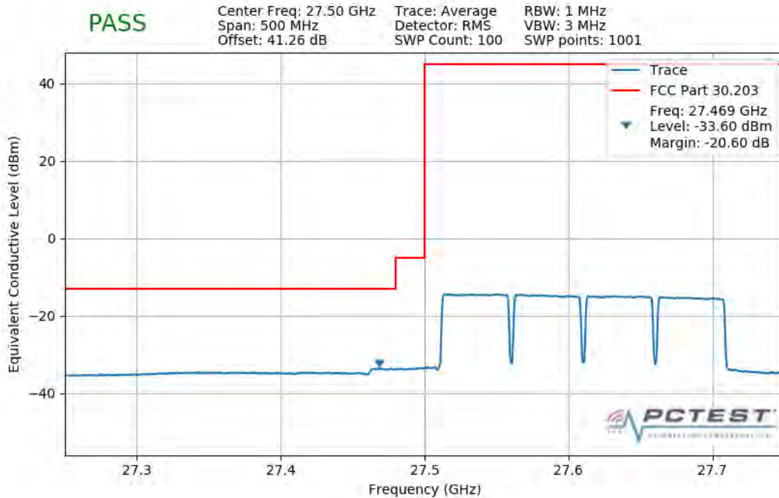
Plot 7-321. Lower Band Edge Plot (4CC 200MHz QPSK Full RB)
