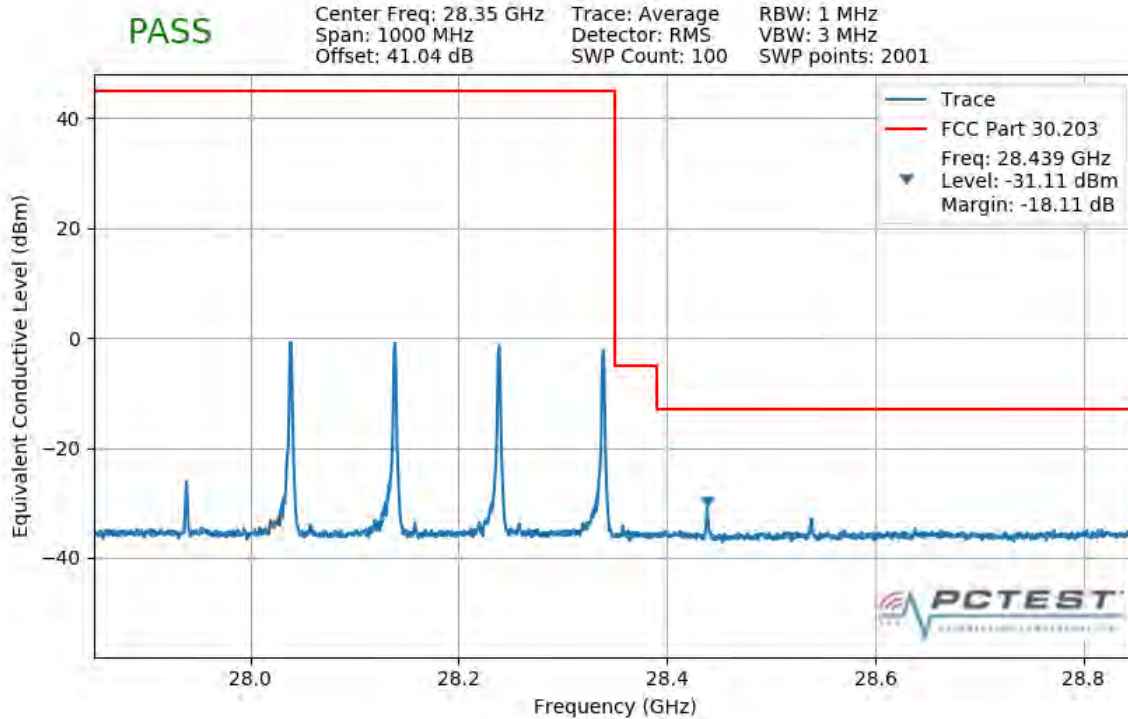
Plot 7-311. Upper Band Edge Plot (4CC 400MHz 16QAM 1 RB)
