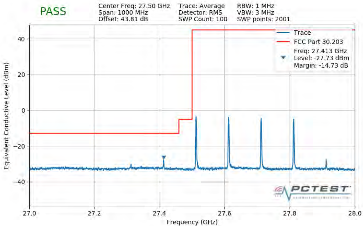
Plot 7-198. Lower Band Edge Plot (4CC 400MHz QPSK 1 RB)
