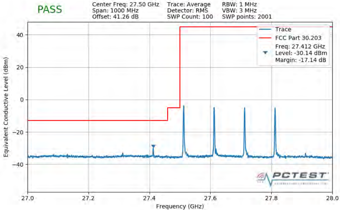
Plot 7-328. Lower Band Edge Plot (4CC 400MHz 64QAM 1 RB)
