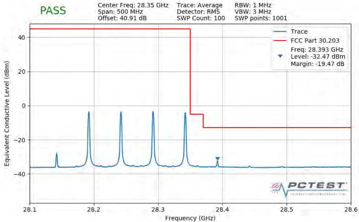
Plot 7-340. Upper Band Edge Plot (4CC 200MHz 64QAM 1 RB)
