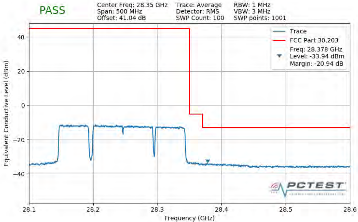
Plot 7-305. Upper Band Edge Plot (4CC 200MHz QPSK Full RB)
