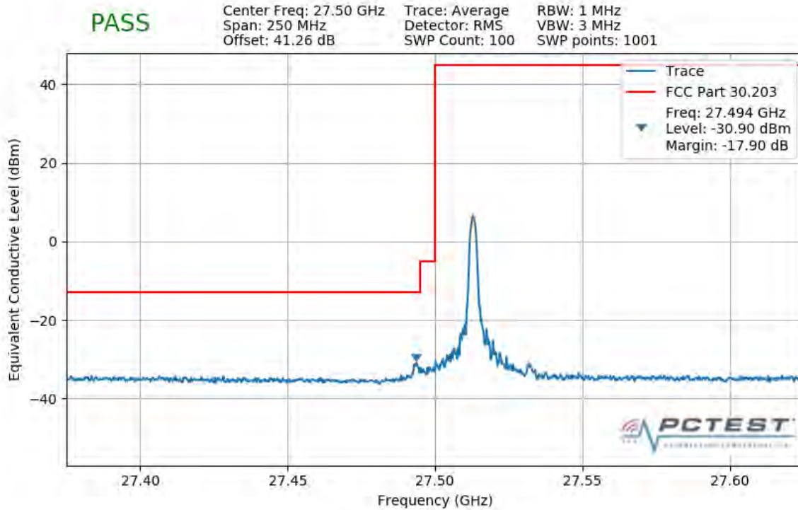
Plot 7-315. Lower Band Edge Plot (1CC 50MHz 16QAM 1 RB)
