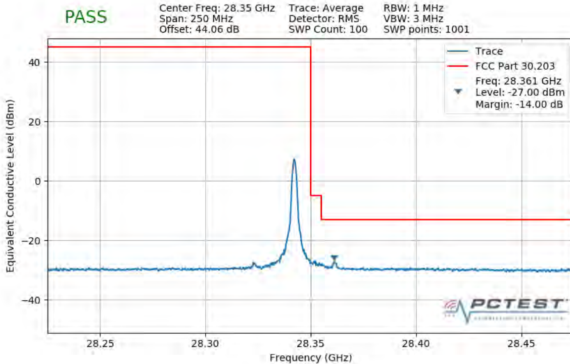
Plot 7-267. Upper Band Edge Plot (1CC 50MHz 16QAM 1 RB)
