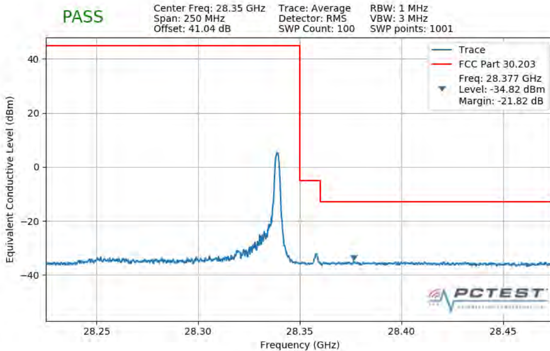
Plot 7-304. Upper Band Edge Plot (1CC 100MHz 64QAM 1 RB)
