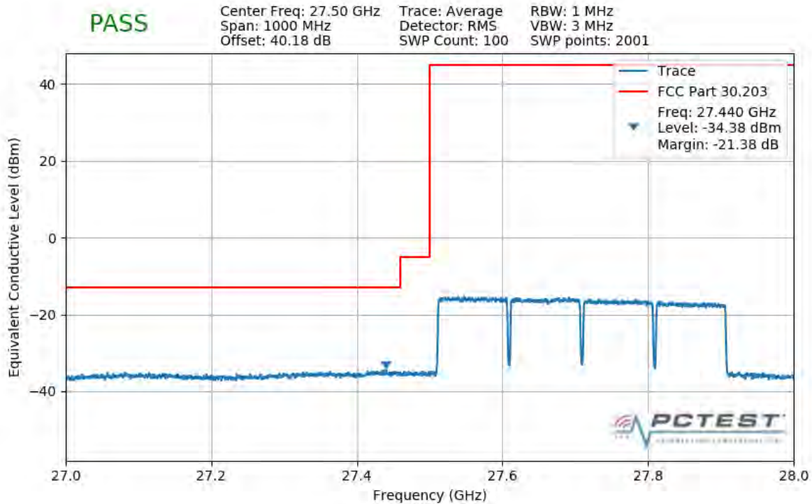
Plot 7-293. Lower Band Edge Plot (4CC 400MHz QPSK Full RB)
