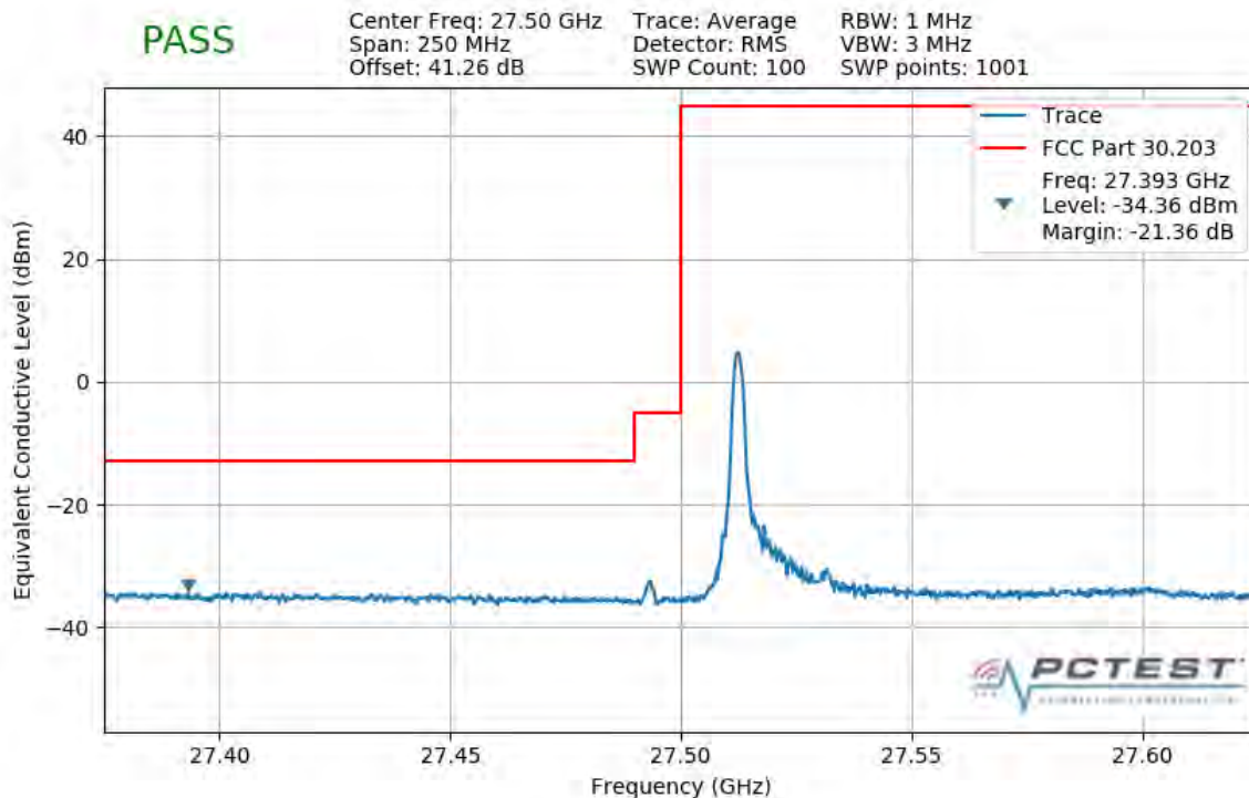
Plot 7-320. Lower Band Edge Plot (1CC 100MHz 64QAM 1 RB)
