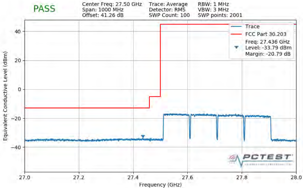
Plot 7-325. Lower Band Edge Plot (4CC 400MHz QPSK Full RB)
