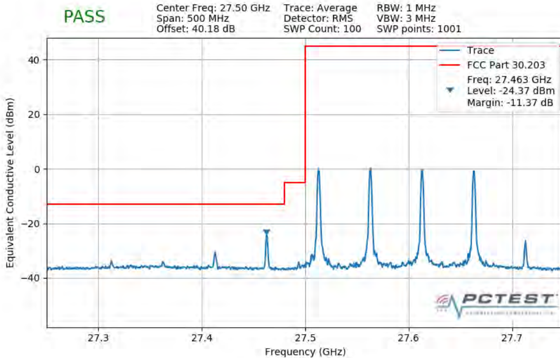
Plot 7-291. Lower Band Edge Plot (4CC 200MHz 16QAM 1 RB)
