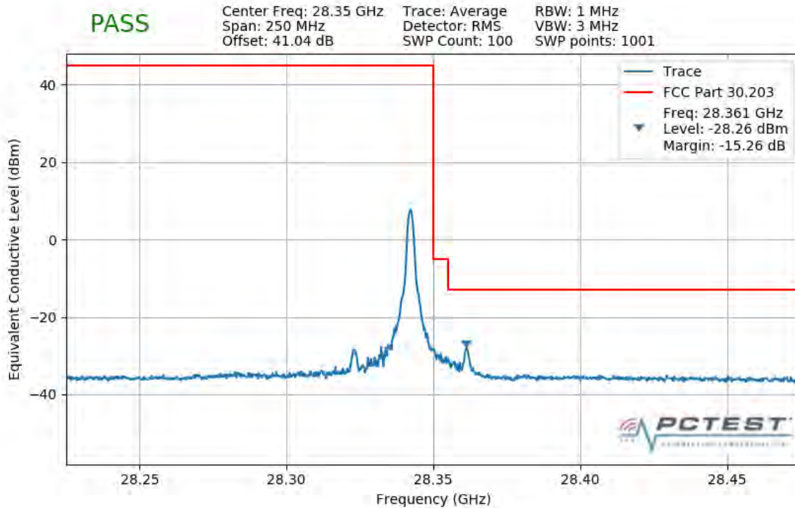
Plot 7-299. Upper Band Edge Plot (1CC 50MHz 16QAM 1 RB)
