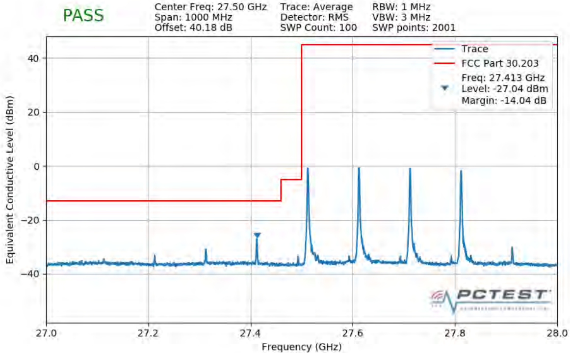
Plot 7-295. Lower Band Edge Plot (4CC 400MHz 16QAM 1 RB)
