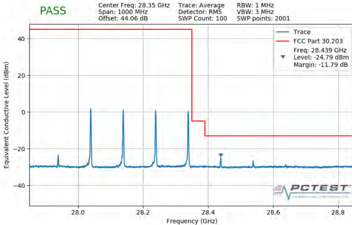
Plot 7-278. Upper Band Edge Plot (4CC 400MHz QPSK 1 RB)
