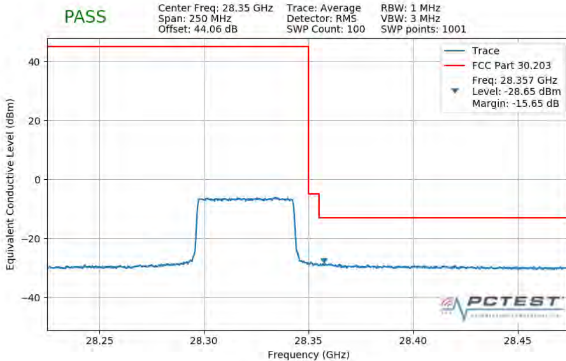
Plot 7-265. Upper Band Edge Plot (1CC 50MHz QPSK Full RB)
