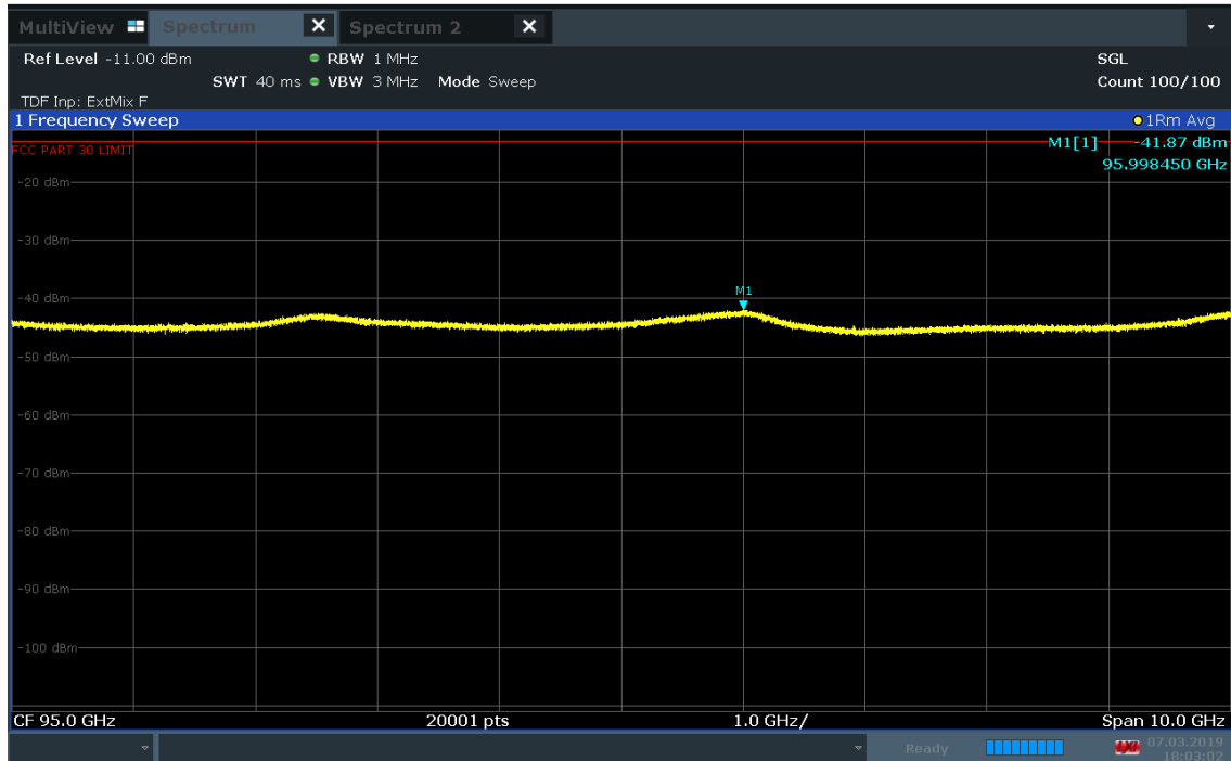
Plot 7-145. K Patch Radiated Spurious Plot 90-100 GHz (1CC QPSK Low Channel H Beam)
