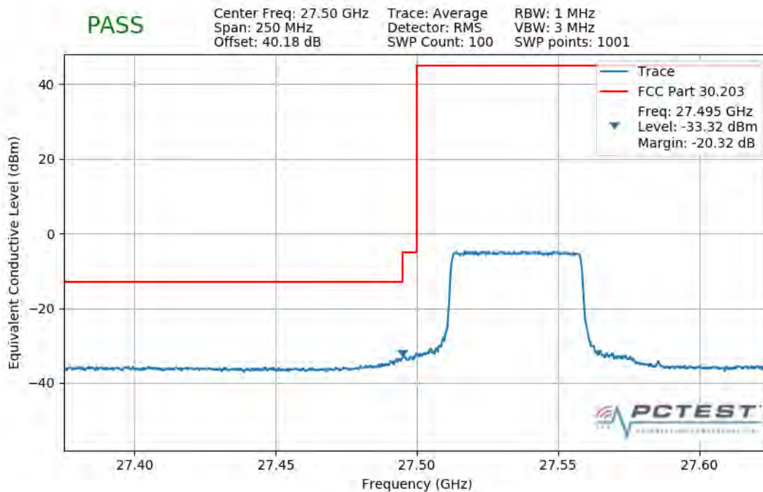
Plot 7-281. Lower Band Edge Plot (1CC 50MHz QPSK Full RB)
