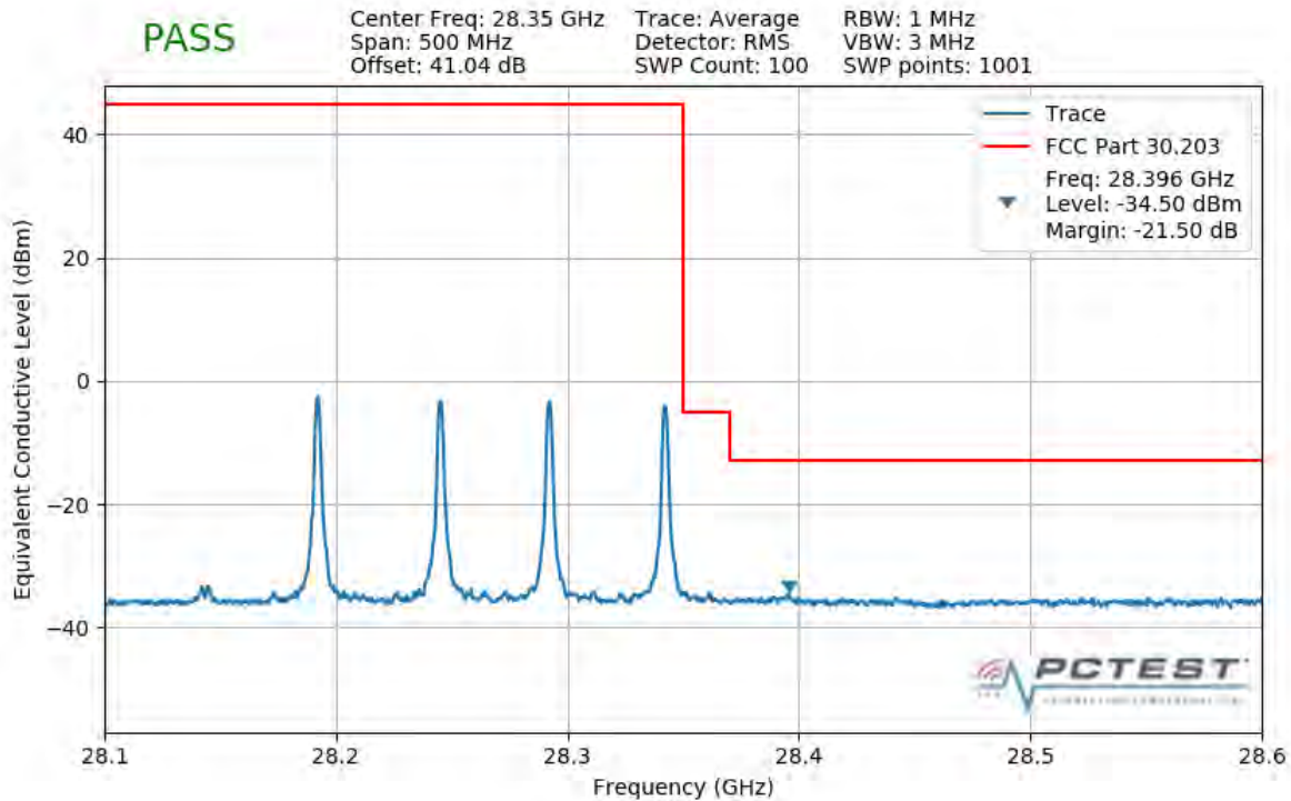
Plot 7-308. Upper Band Edge Plot (4CC 200MHz 64QAM 1 RB)
