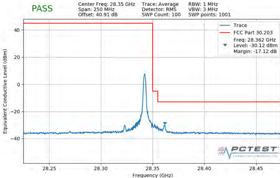
Plot 7-330. Upper Band Edge Plot (1CC 50MHz QPSK 1 RB)
