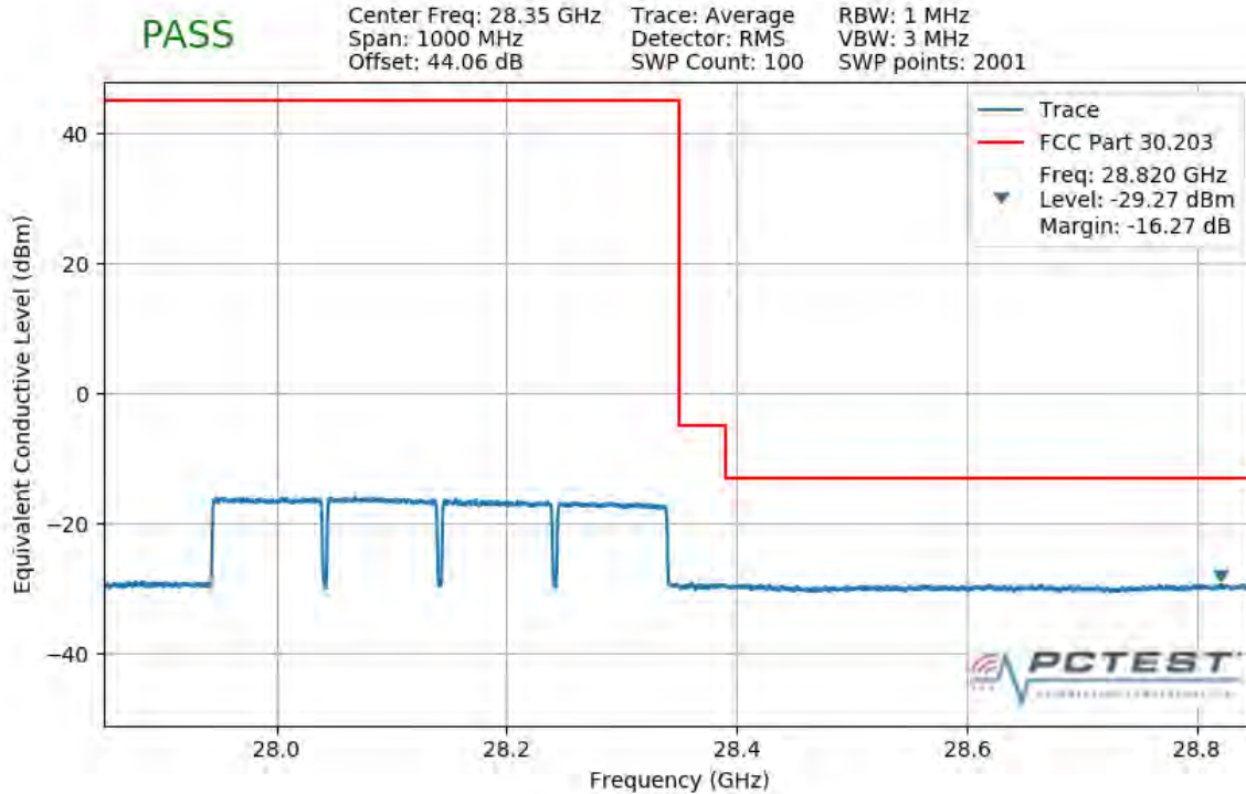
Plot 7-277. Upper Band Edge Plot (4CC 400MHz QPSK Full RB)
