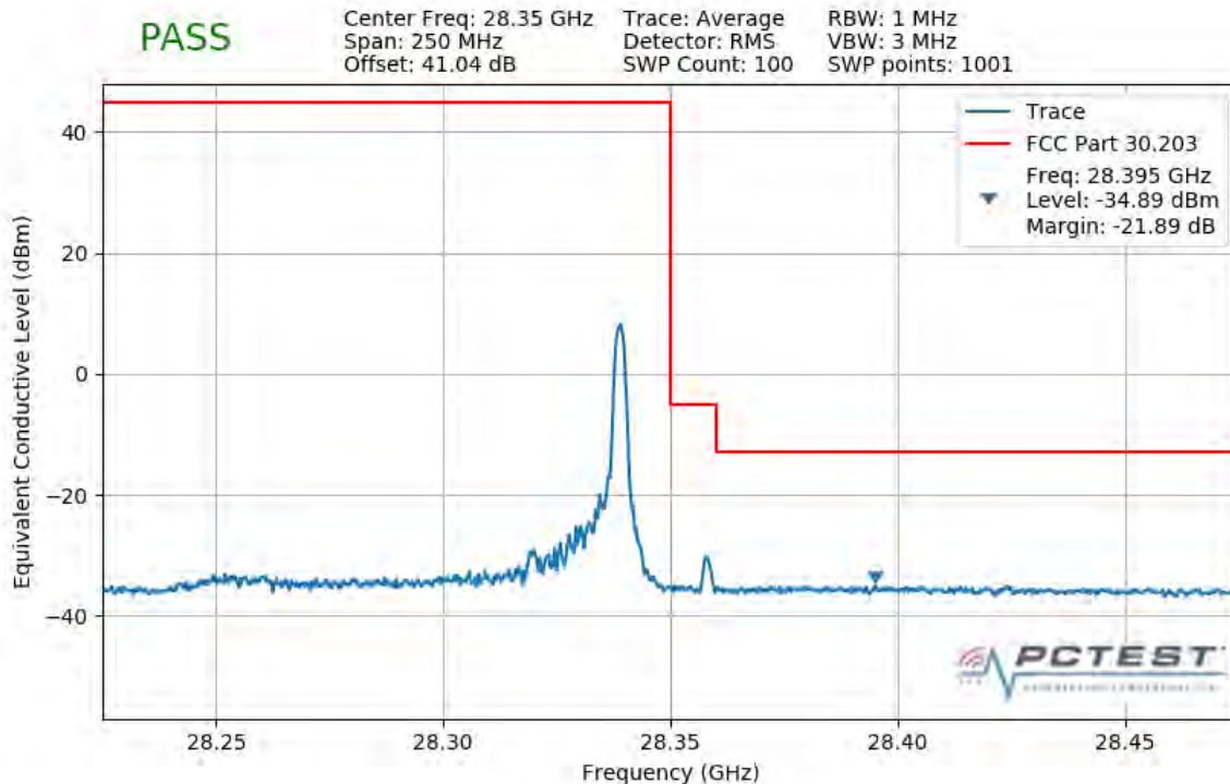
Plot 7-302. Upper Band Edge Plot (1CC 100MHz QPSK 1 RB)
