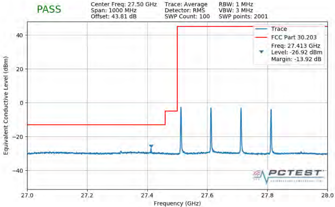
Plot 7-264. Lower Band Edge Plot (4CC 400MHz 64QAM 1 RB)
