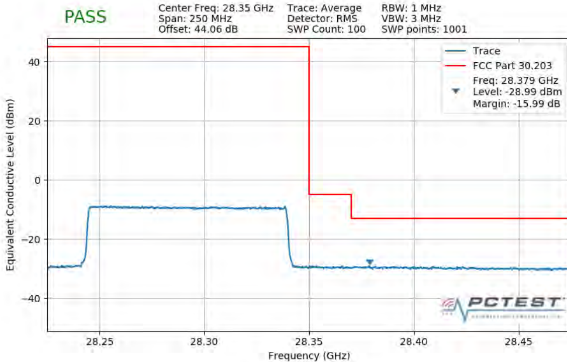
Plot 7-269. Upper Band Edge Plot (1CC 100MHz QPSK Full RB)
