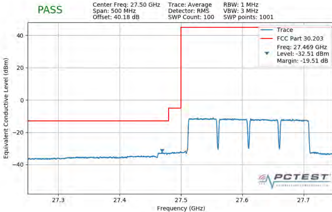
Plot 7-289. Lower Band Edge Plot (4CC 200MHz QPSK Full RB)
