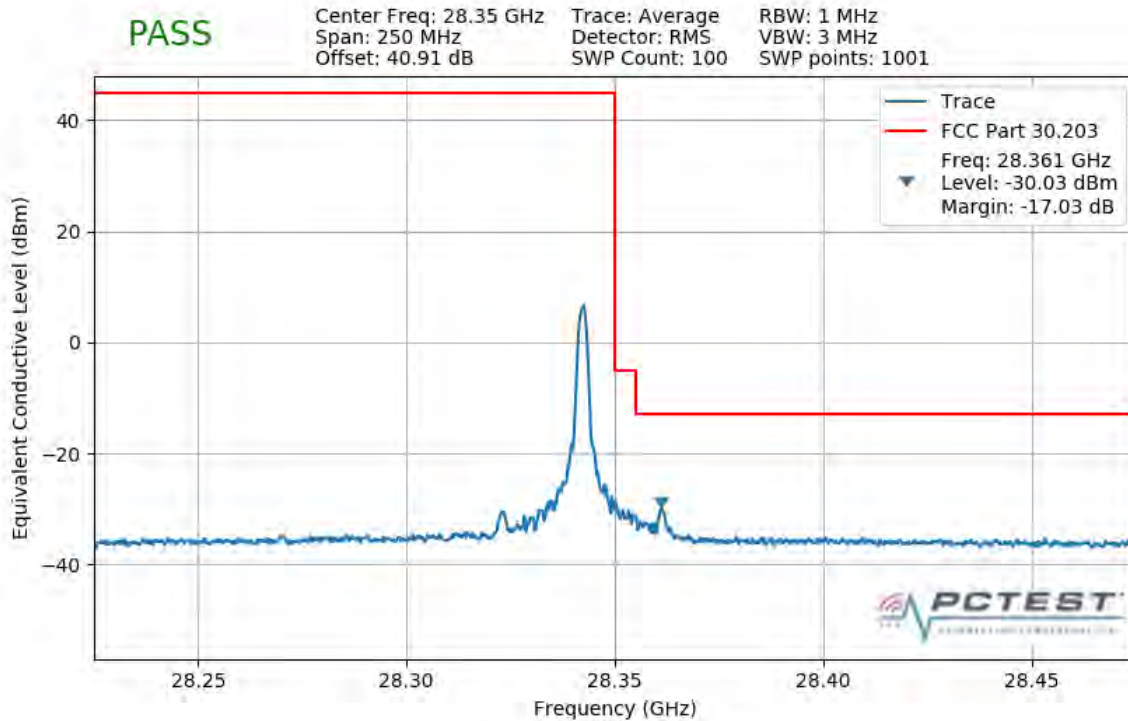
Plot 7-331. Upper Band Edge Plot (1CC 50MHz 16QAM 1 RB)
