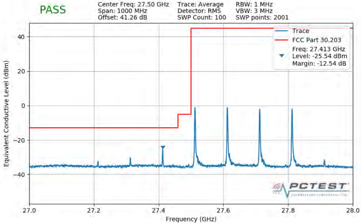
Plot 7-327. Lower Band Edge Plot (4CC 400MHz 16QAM 1 RB)
