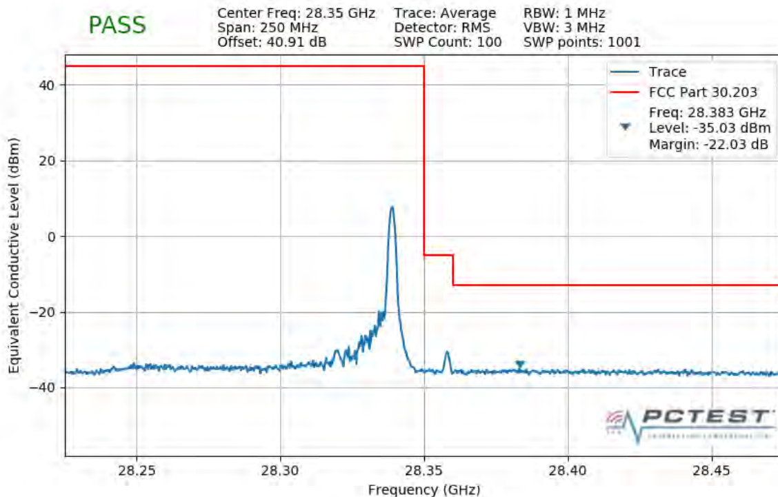
Plot 7-334. Upper Band Edge Plot (1CC 100MHz QPSK 1 RB)
