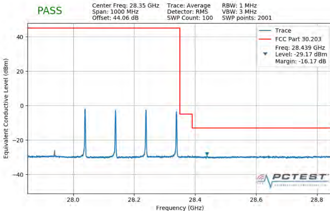
Plot 7-280. Upper Band Edge Plot (4CC 400MHz 64QAM 1 RB)
