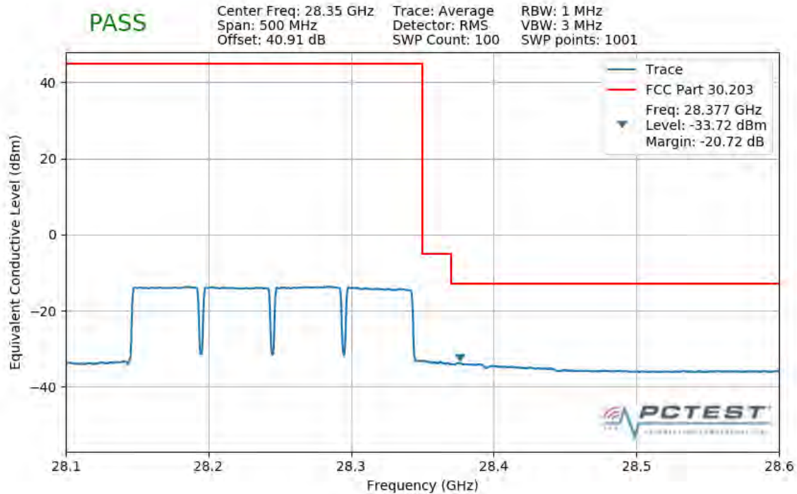
Plot 7-337. Upper Band Edge Plot (4CC 200MHz QPSK Full RB)
