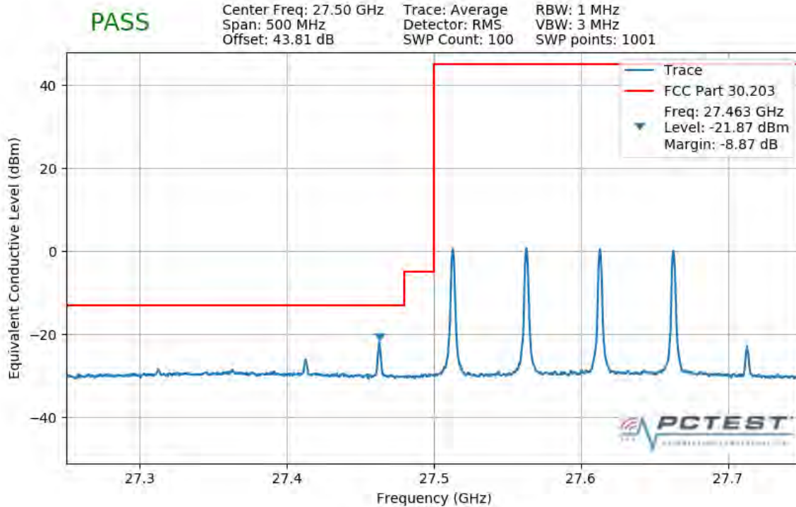
Plot 7-259. Lower Band Edge Plot (4CC 200MHz 16QAM 1 RB)
