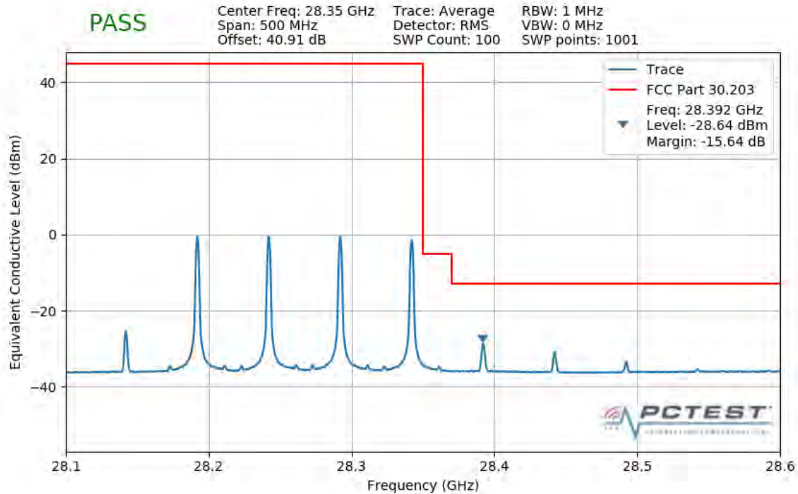
Plot 7-339. Upper Band Edge Plot (4CC 200MHz 16QAM 1 RB)
