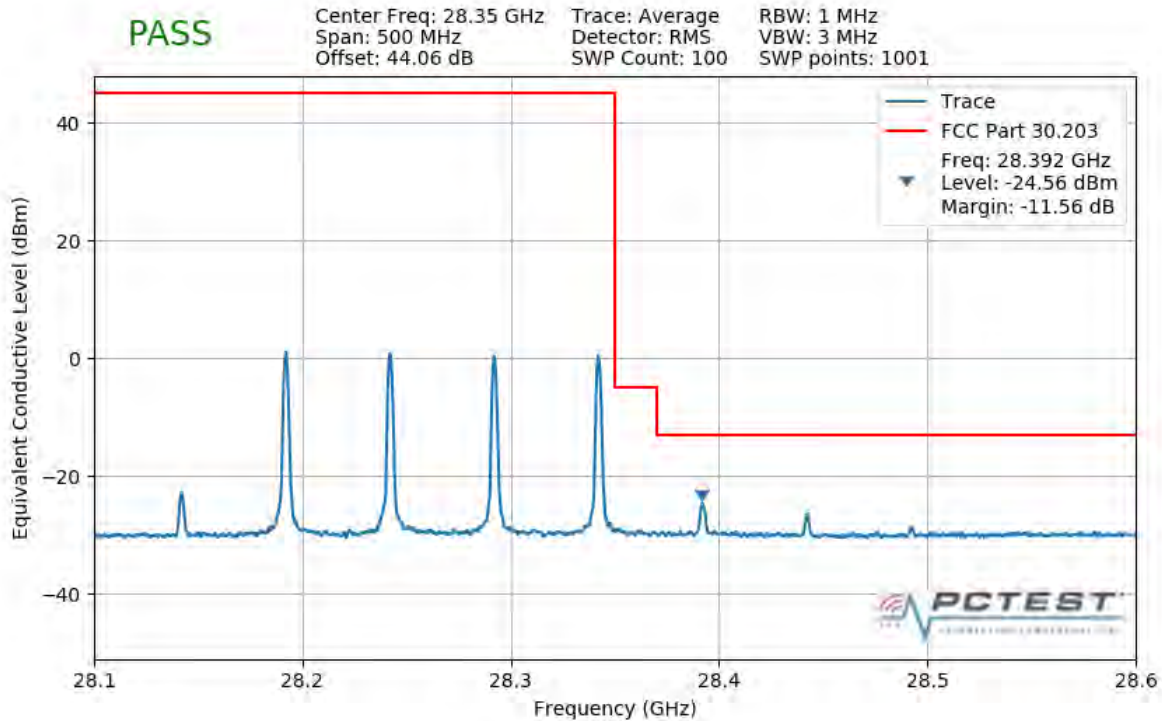
Plot 7-275. Upper Band Edge Plot (4CC 200MHz 16QAM 1 RB)
