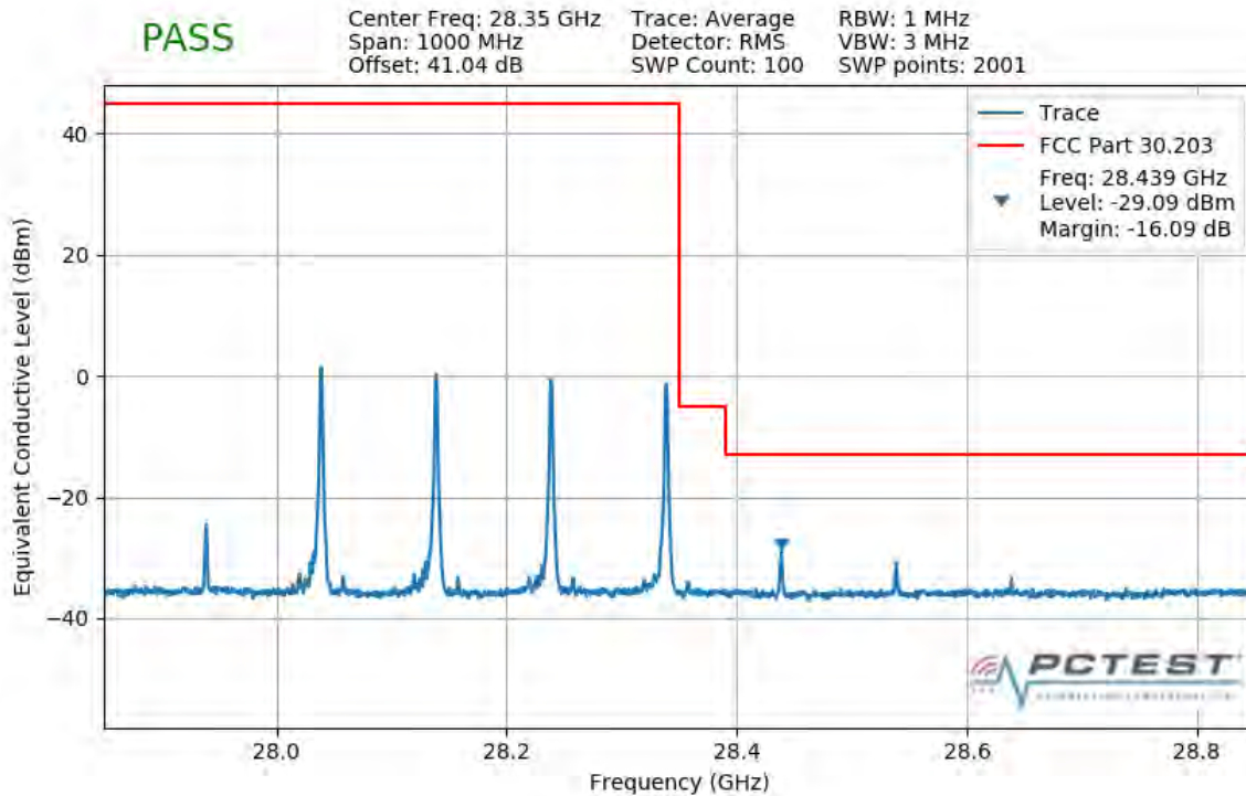
Plot 7-310. Upper Band Edge Plot (4CC 400MHz QPSK 1 RB)
