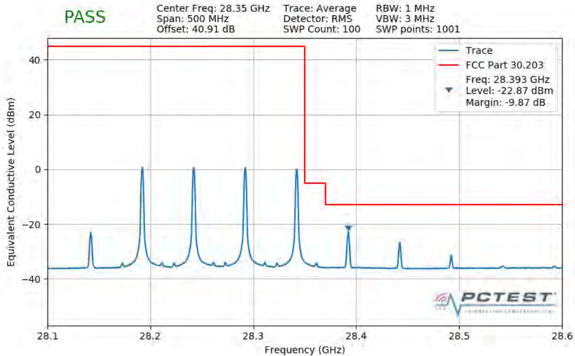
Plot 7-338. Upper Band Edge Plot (4CC 200MHz QPSK 1 RB)
