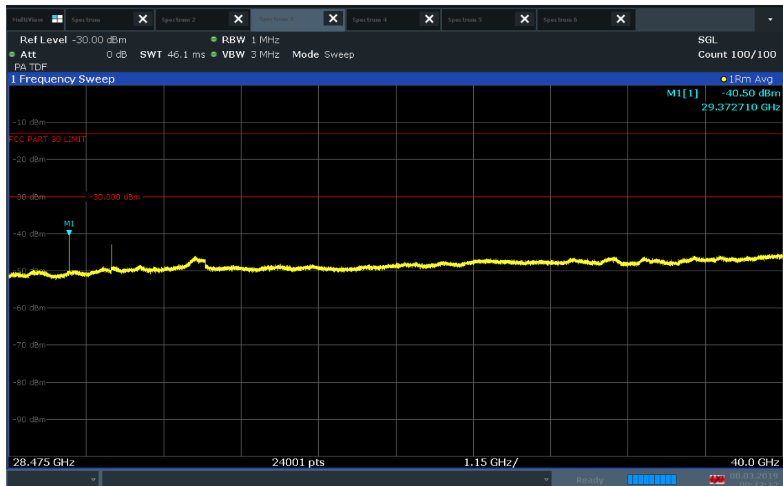
Plot 7-166. L Patch Radiated Spurious Plot 28.475-40 GHz (1CC QPSK High Channel V Beam)
