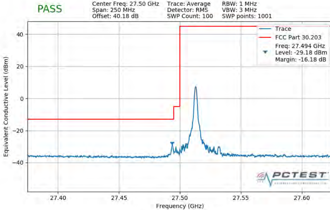
Plot 7-283. Lower Band Edge Plot (1CC 50MHz 16QAM 1 RB)
