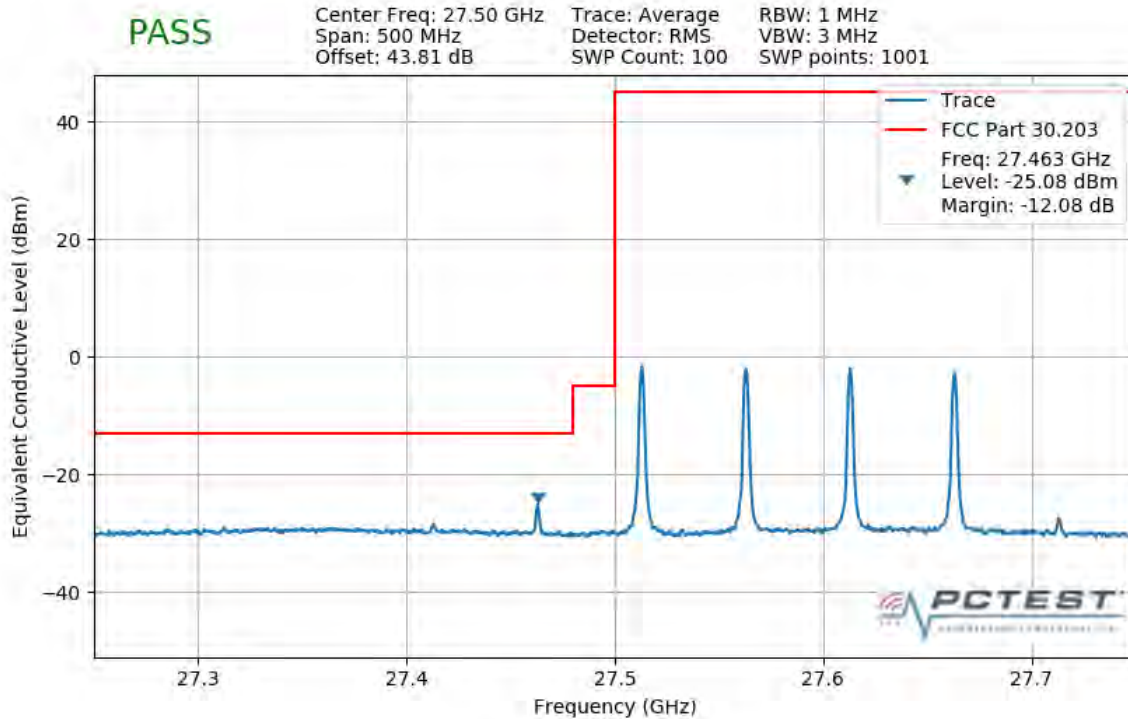
Plot 7-260. Lower Band Edge Plot (4CC 200MHz 64QAM 1 RB)
