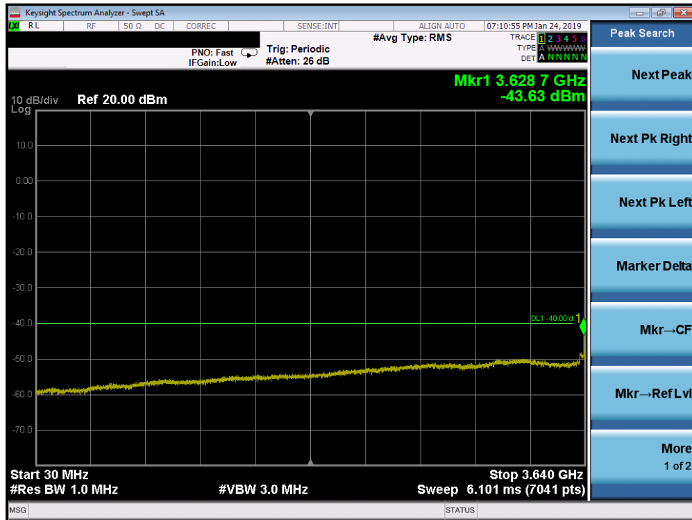
Plot 7-23. Conducted Spurious Plot (Band 48 - 20.0MHz QPSK - RB Size 1, RB Offset 0 - High Channel)
