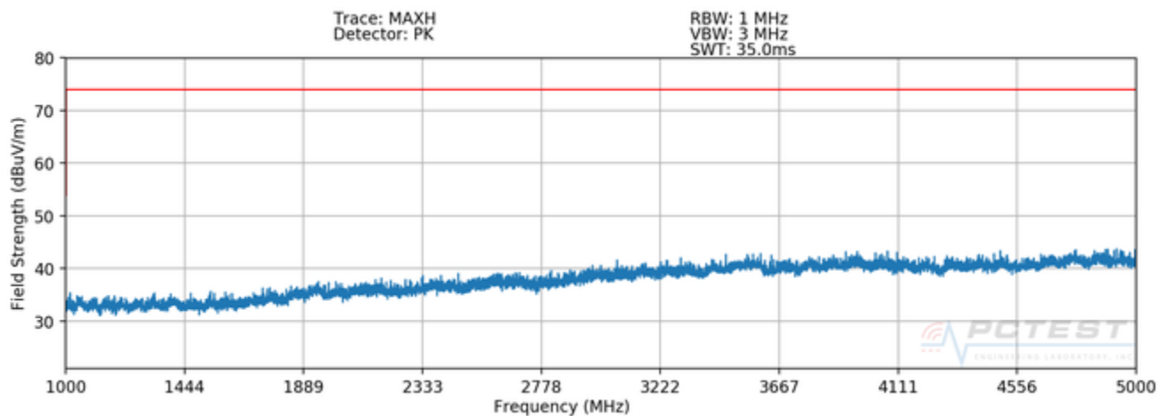
Plot 7-2. Radiated Spurious Plot above 1GHz - Horizontal
