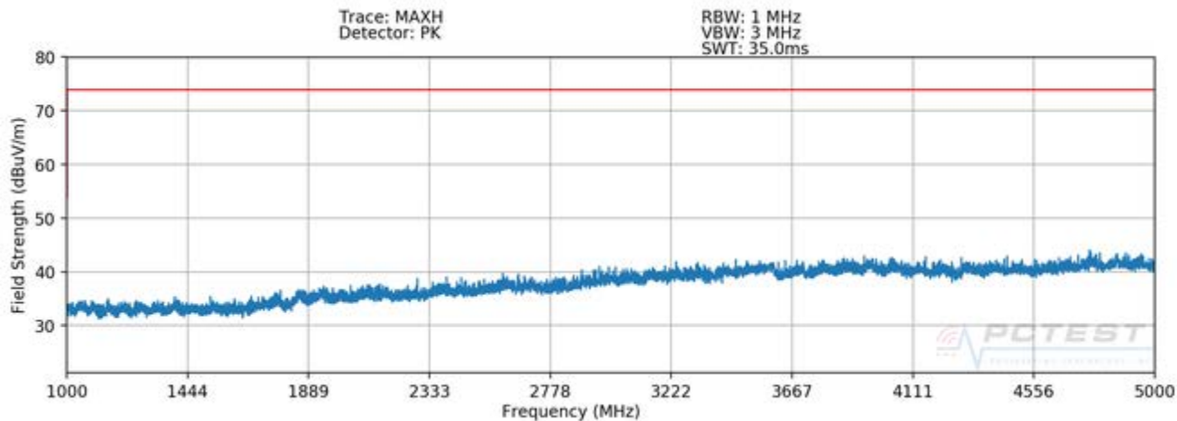
Plot 7-3. Radiated Spurious Plot above 1GHz - Vertical
