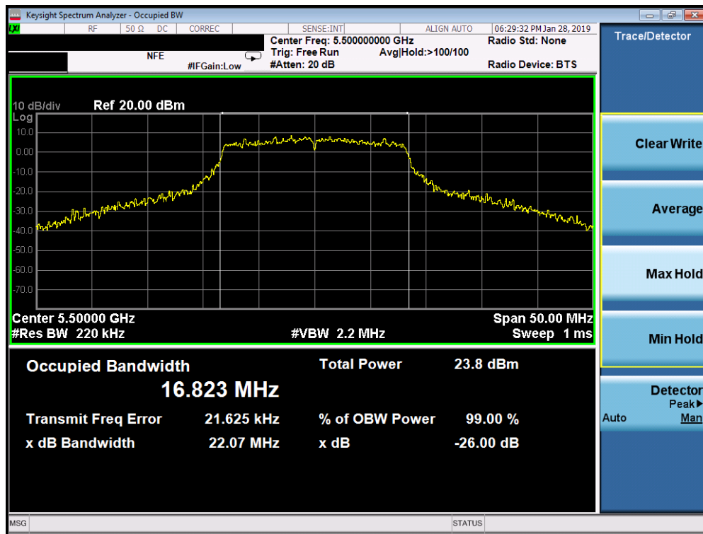
Plot 7-82. 26dB Bandwidth Plot SISO ANT2 (802.11a (UNII Band 2C) – Ch. 100)
