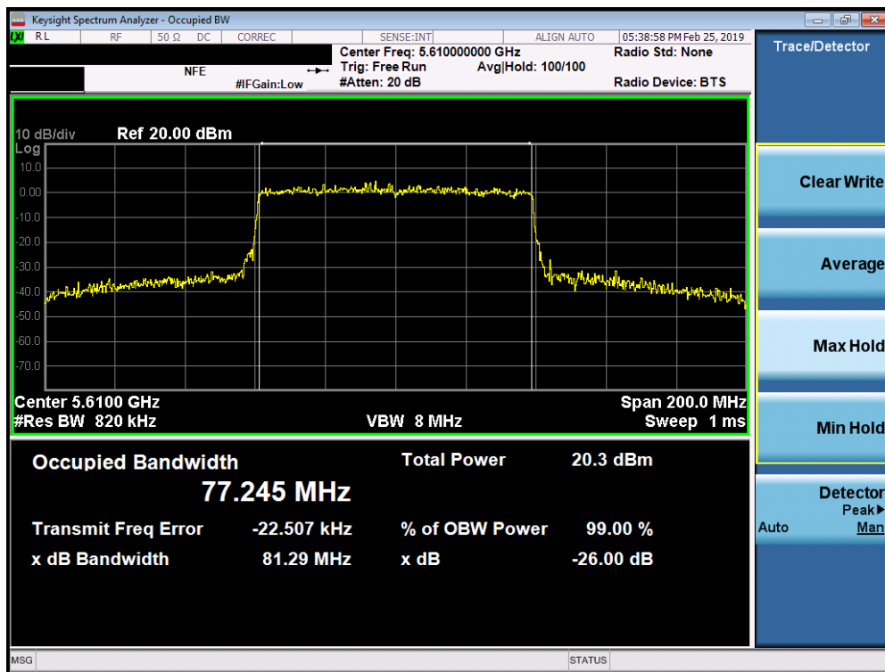
Plot 7-50. 26dB Bandwidth Plot SISO ANT1 (80MHz BW 802.11ax (UNII Band 2C) – Ch. 122)
