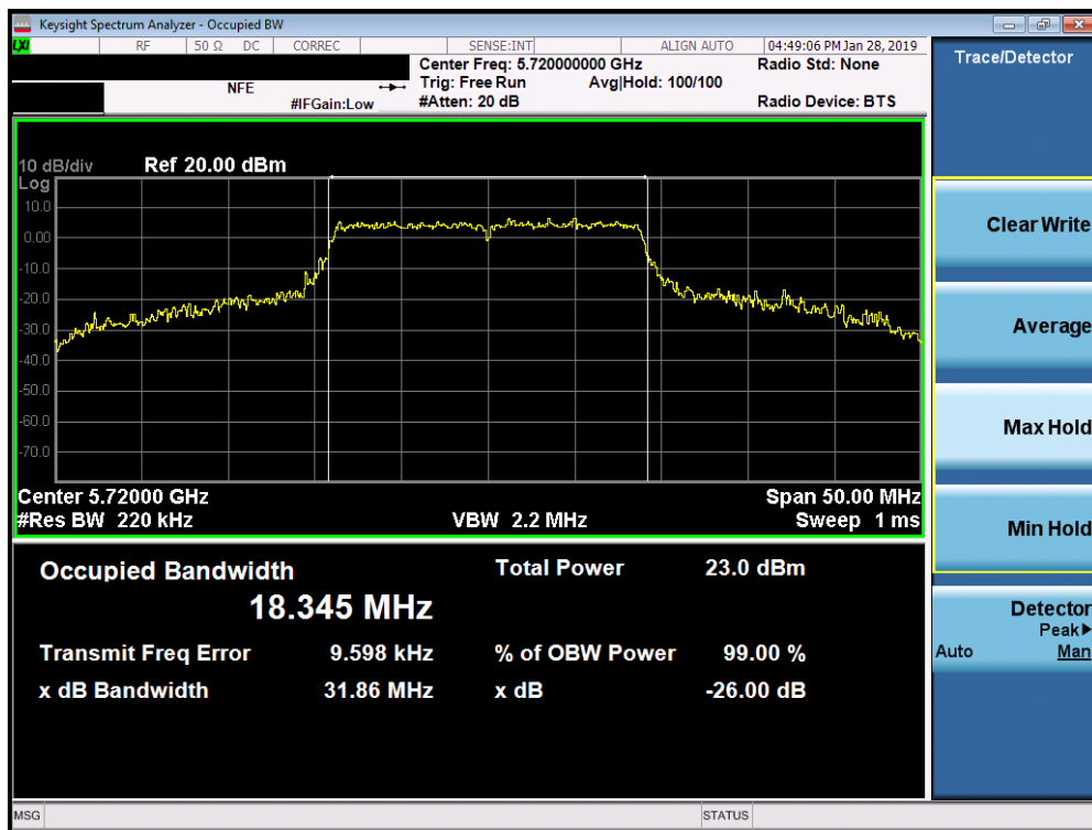
Plot 7-36. 26dB Bandwidth Plot SISO ANT1 (20MHz BW 802.11n (UNII Band 2C) – Ch. 144)
