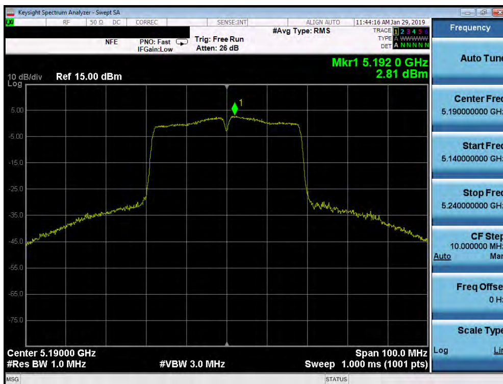
Plot 7-208. Power Spectral Density Plot SISO ANT2 (40MHz BW 802.11n (UNII Band 1) – Ch. 38)
