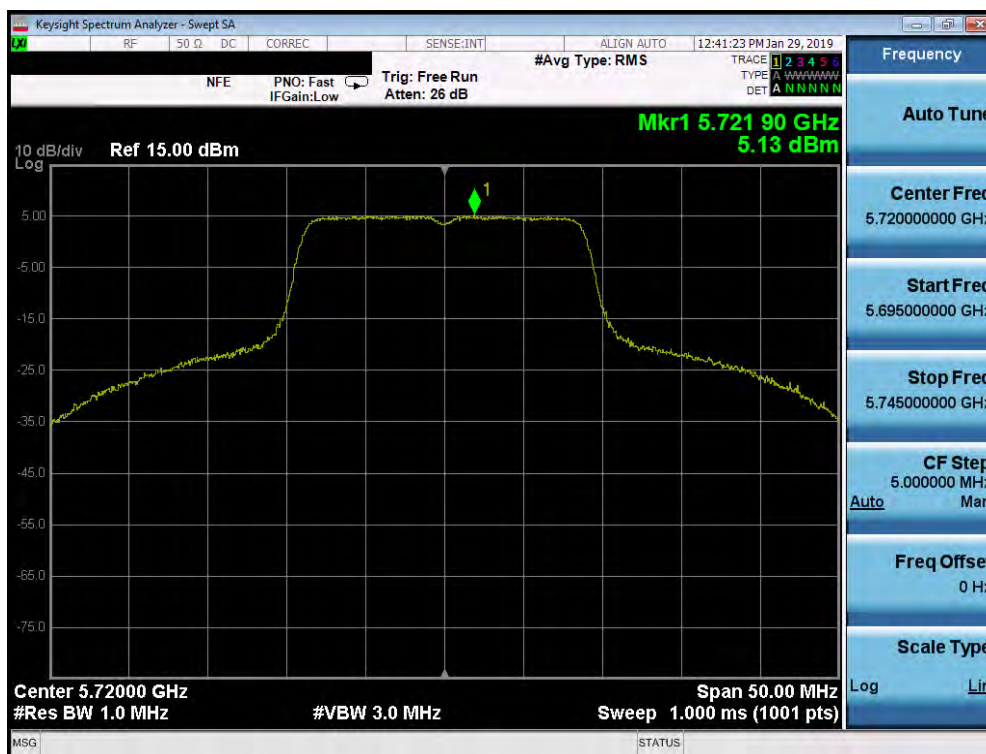
Plot 7-234. Power Spectral Density Plot SISO ANT2 (20MHz BW 802.11n (UNII Band 2C) – Ch. 144)
