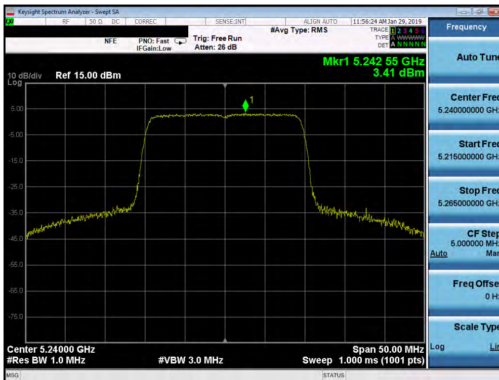
Plot 7-207. Power Spectral Density Plot SISO ANT2 (20MHz BW 802.11ax (UNII Band 1) – Ch. 48)
