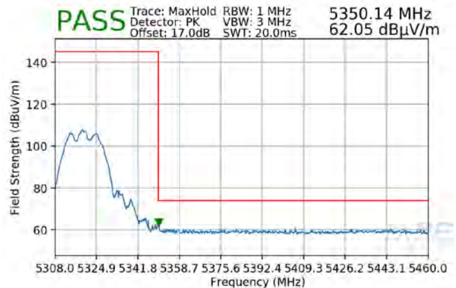
Plot 7-349. Radiated Upper Band Edge Plot CDD (Peak - UNII Band 2A)
