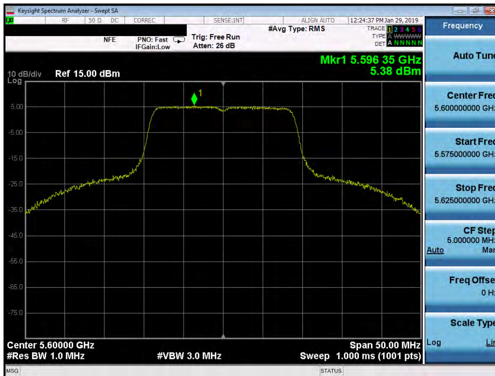
Plot 7-233. Power Spectral Density Plot SISO ANT2 (20MHz BW 802.11n (UNII Band 2C) – Ch. 120)
