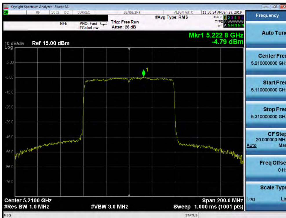
Plot 7-213. Power Spectral Density Plot SISO ANT2 (80MHz BW 802.11ax (UNII Band 1) – Ch. 42)
