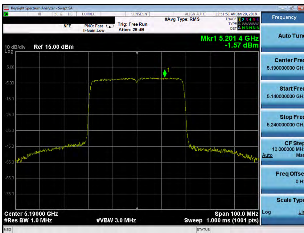
Plot 7-210. Power Spectral Density Plot SISO ANT2 (40MHz BW 802.11ax (UNII Band 1) – Ch. 38)
