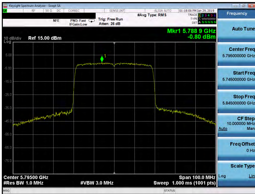
Plot 7-262. Power Spectral Density Plot SISO ANT2 (40MHz BW 802.11ax (UNII Band 3) – Ch. 159)
