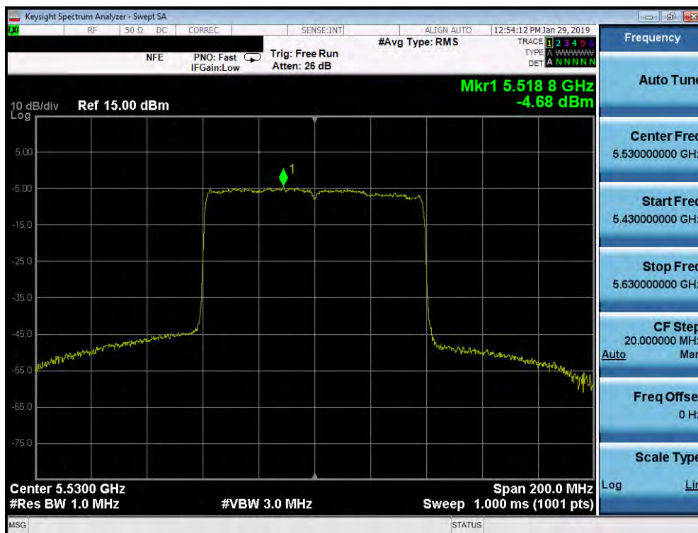
Plot 7-247. Power Spectral Density Plot SISO ANT2 (80MHz BW 802.11ax (UNII Band 2C) – Ch. 106)
