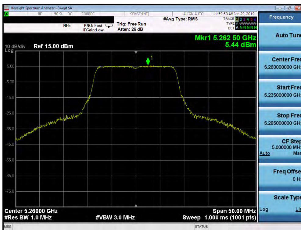
Plot 7-214. Power Spectral Density Plot SISO ANT2 (802.11a (UNII Band 2A) – Ch. 52)
