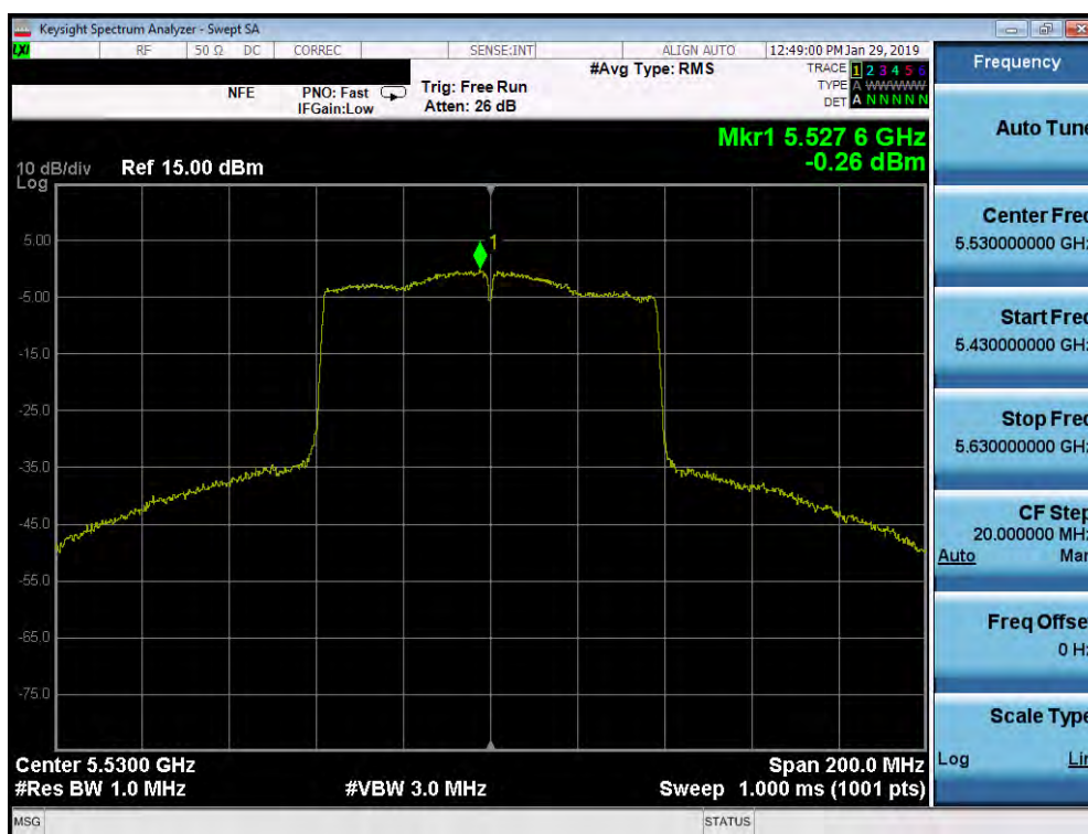
Plot 7-244. Power Spectral Density Plot SISO ANT2 (80MHz BW 802.11ac (UNII Band 2C) – Ch. 106)
