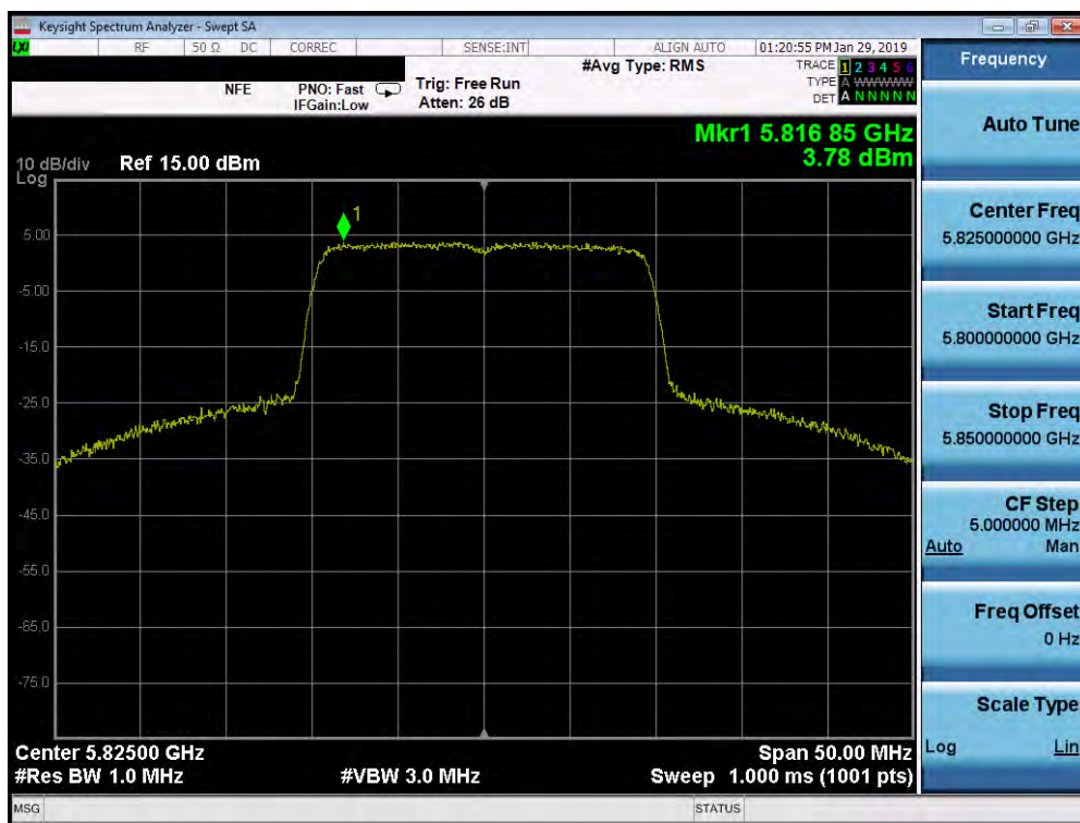
Plot 7-258. Power Spectral Density Plot SISO ANT2 (20MHz BW 802.11ax (UNII Band 3) – Ch. 165)
