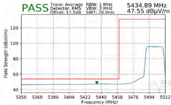
Plot 7-359. Radiated Lower Band Edge Plot MIMO (Average – UNII Band 2C)
