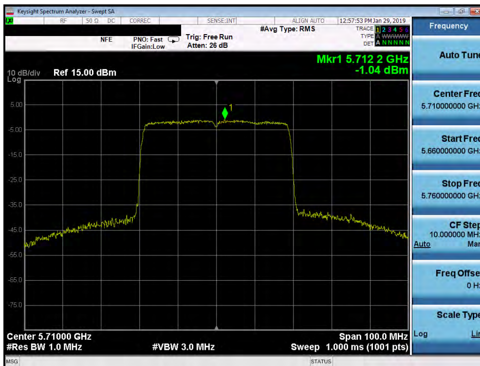
Plot 7-243. Power Spectral Density Plot SISO ANT2 (40MHz BW 802.11ax (UNII Band 2C) – Ch. 142)
