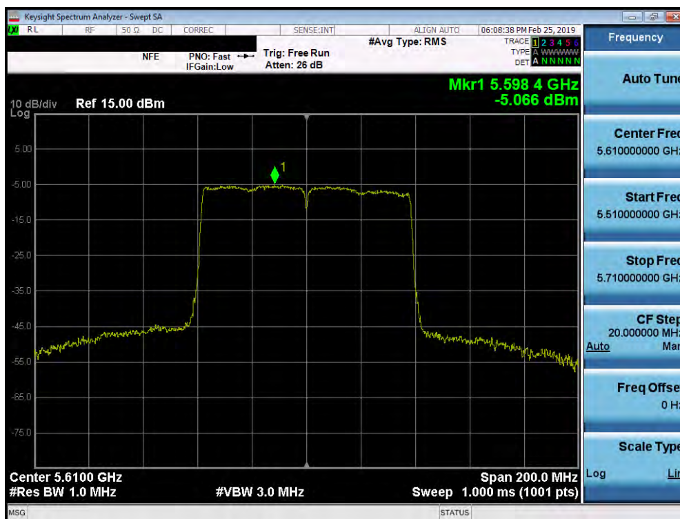
Plot 7-248. Power Spectral Density Plot SISO ANT2 (80MHz BW 802.11ax (UNII Band 2C) – Ch. 122)
