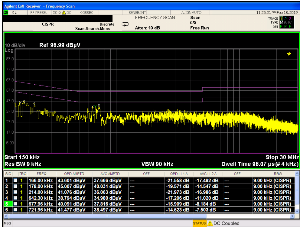
Plot 7-392. Line Conducted Plot with 802.11a UNII Band 3 (L1) with Travel Adapter
