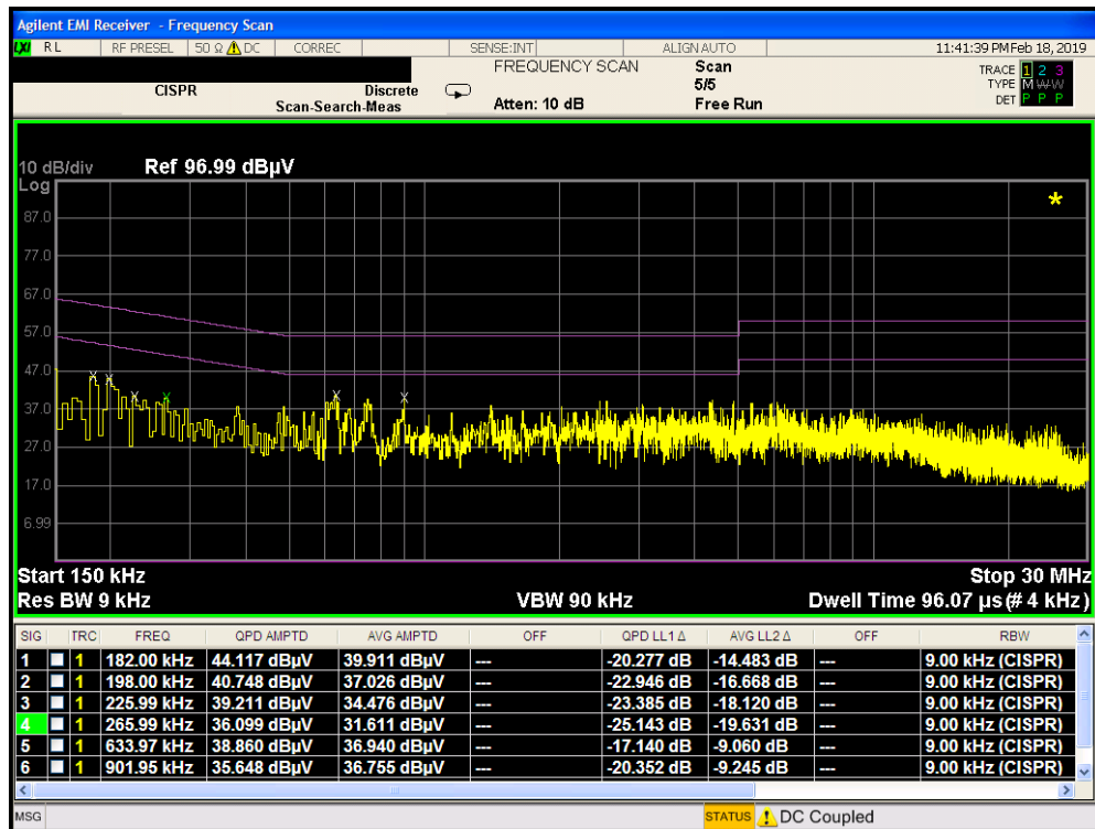
Plot 7-401. Line Conducted Plot with 802.11a UNII Band 3 (N) with Wireless Charging Pad
