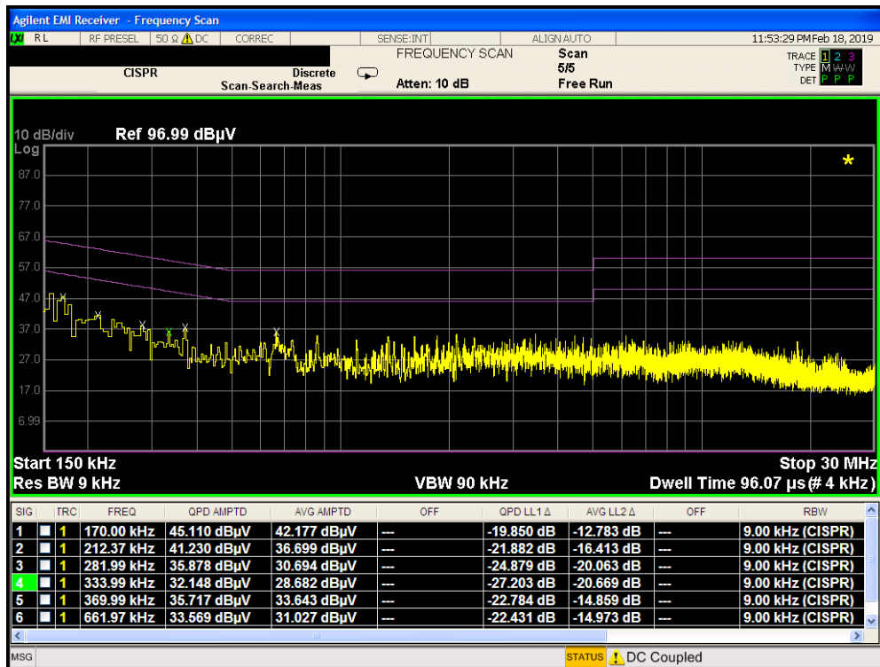
Plot 7-397. Line Conducted Plot with 802.11a UNII Band 2A (N) with Wireless Charging Pad
