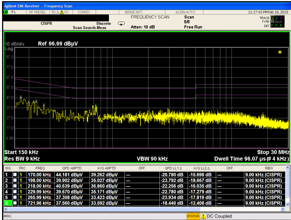
Plot 7-391. Line Conducted Plot with 802.11a UNII Band 2C (N) with Travel Adapter
