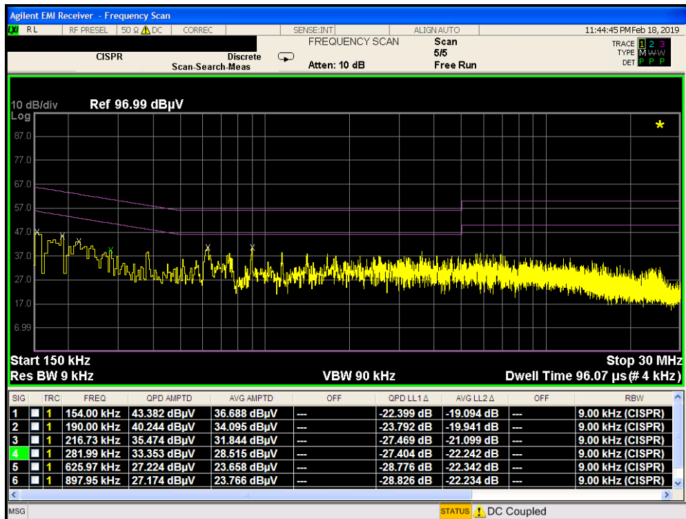
Plot 7-399. Line Conducted Plot with 802.11a UNII Band 2C (N) with Wireless Charging Pad
