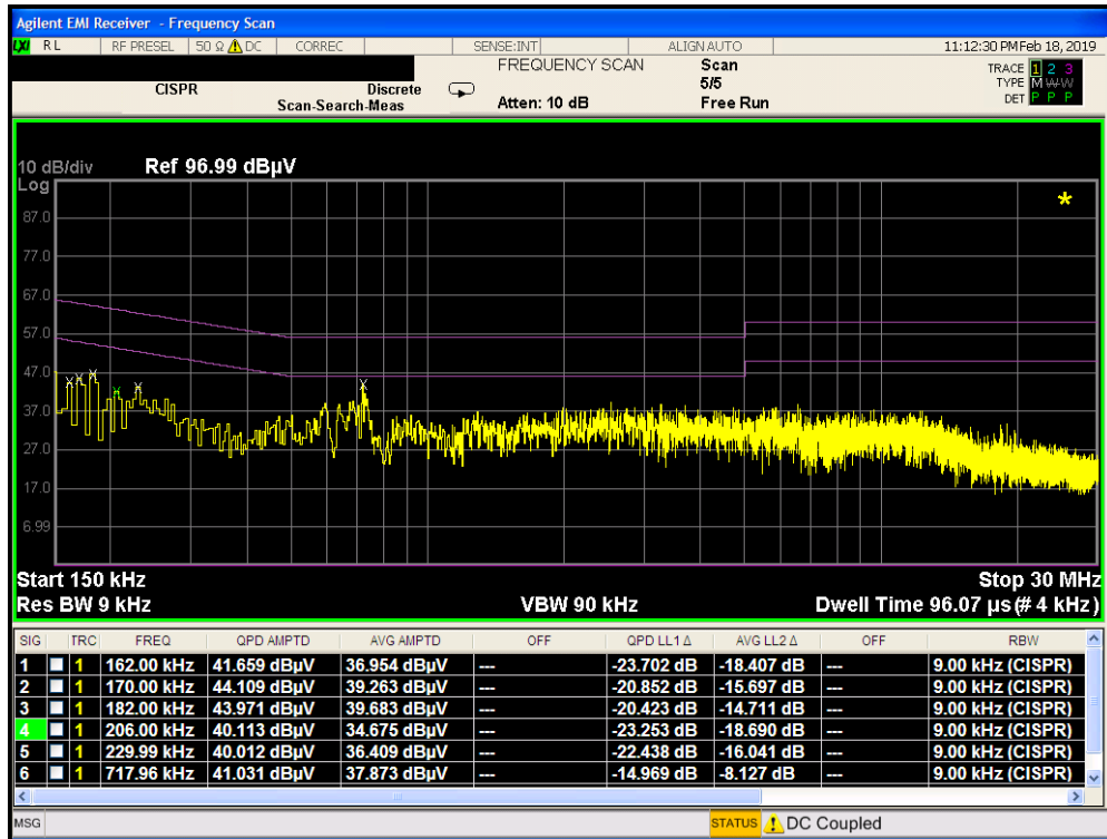
Plot 7-390. Line Conducted Plot with 802.11a UNII Band 2C (L1) with Travel Adapter
