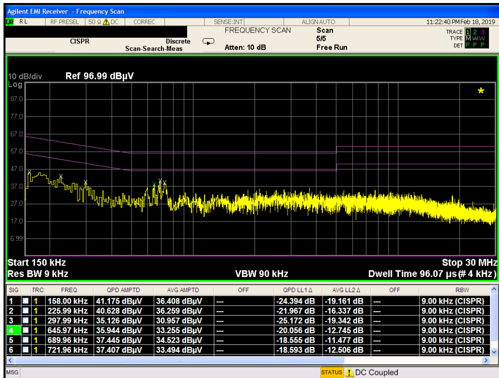
Plot 7-393. Line Conducted Plot with 802.11a UNII Band 3 (N) with Travel Adapter
