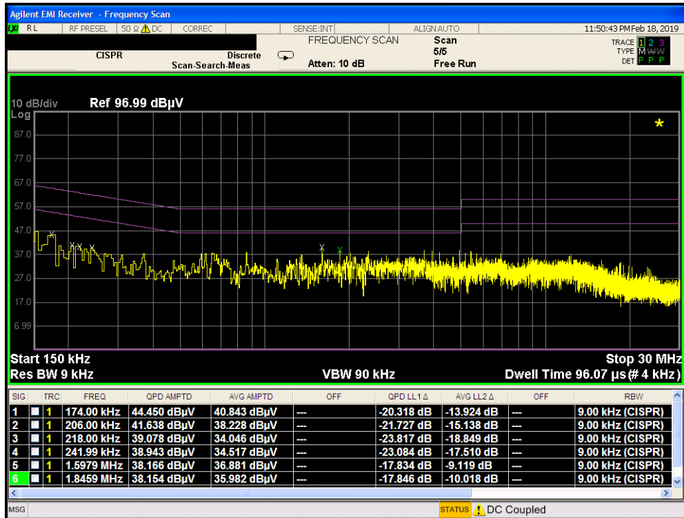
Plot 7-396. Line Conducted Plot with 802.11a UNII Band 2A (L1) with Wireless Charging Pad
