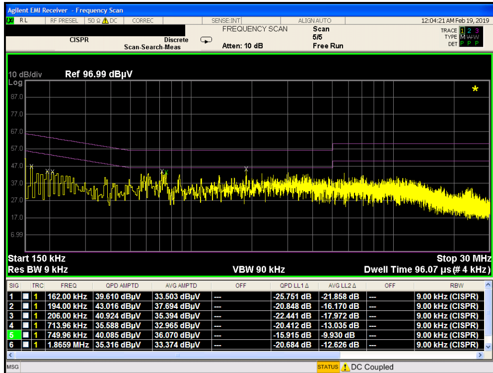
Plot 7-394. Line Conducted Plot with 802.11a UNII Band 1 (L1) with Wireless Charging Pad
