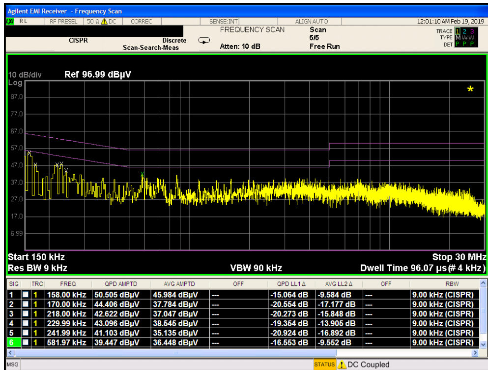
Plot 7-395. Line Conducted Plot with 802.11a UNII Band 1 (N) with Wireless Charging Pad
