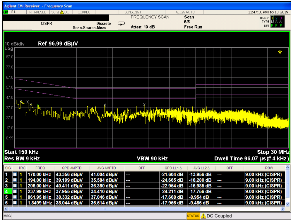
Plot 7-398. Line Conducted Plot with 802.11a UNII Band 2C (L1) with Wireless Charging Pad
