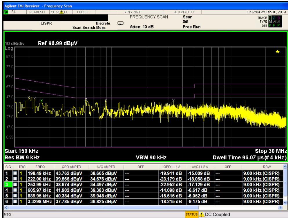
Plot 7-400. Line Conducted Plot with 802.11a UNII Band 3 (L1) with Wireless Charging Pad
