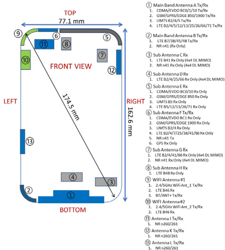
Figure F-1 DUT Antenna Locations
