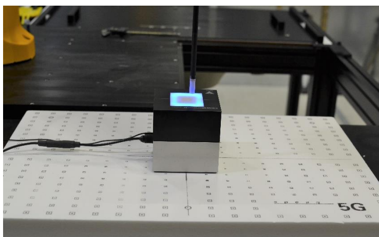
Figure 4-1 System Verification Setup Photo
