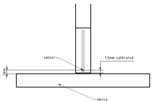
Figure 2-1 EUmWV3 Probe
