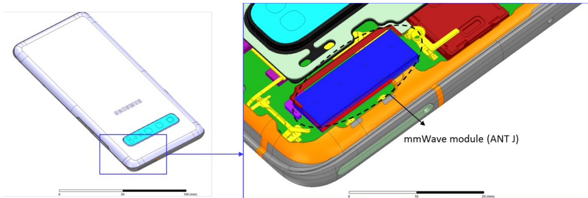
Figure 4. mmWave module (ANT J)
