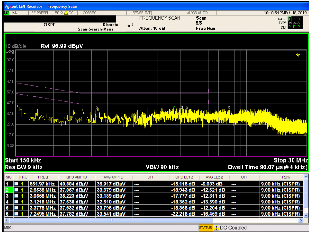
Plot 7-8. Line-Conducted Test Plot (L1) with Travel Adapter
