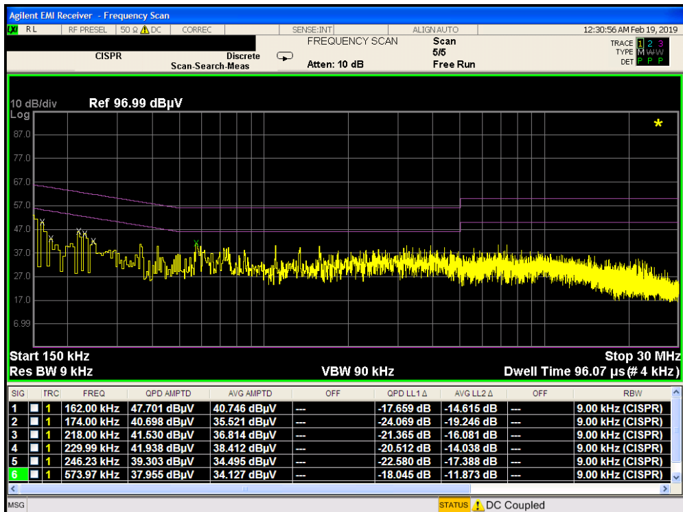
Plot 7-11. Line-Conducted Test Plot (N) with Wireless Charging Pad
