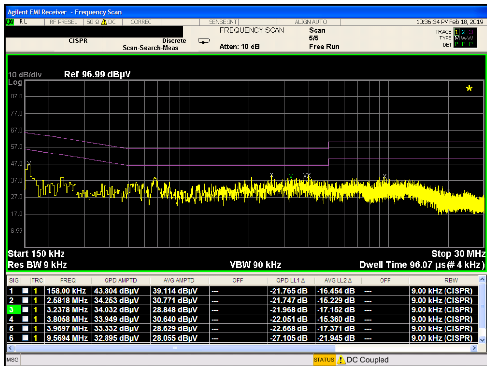
Plot 7-9. Line-Conducted Test Plot (N) with Travel Adapter
