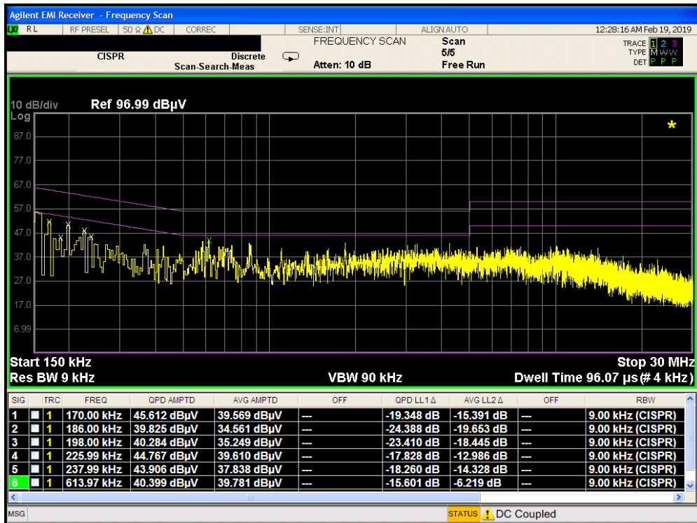
Plot 7-10. Line-Conducted Test Plot (L1) with Wireless Charging Pad
