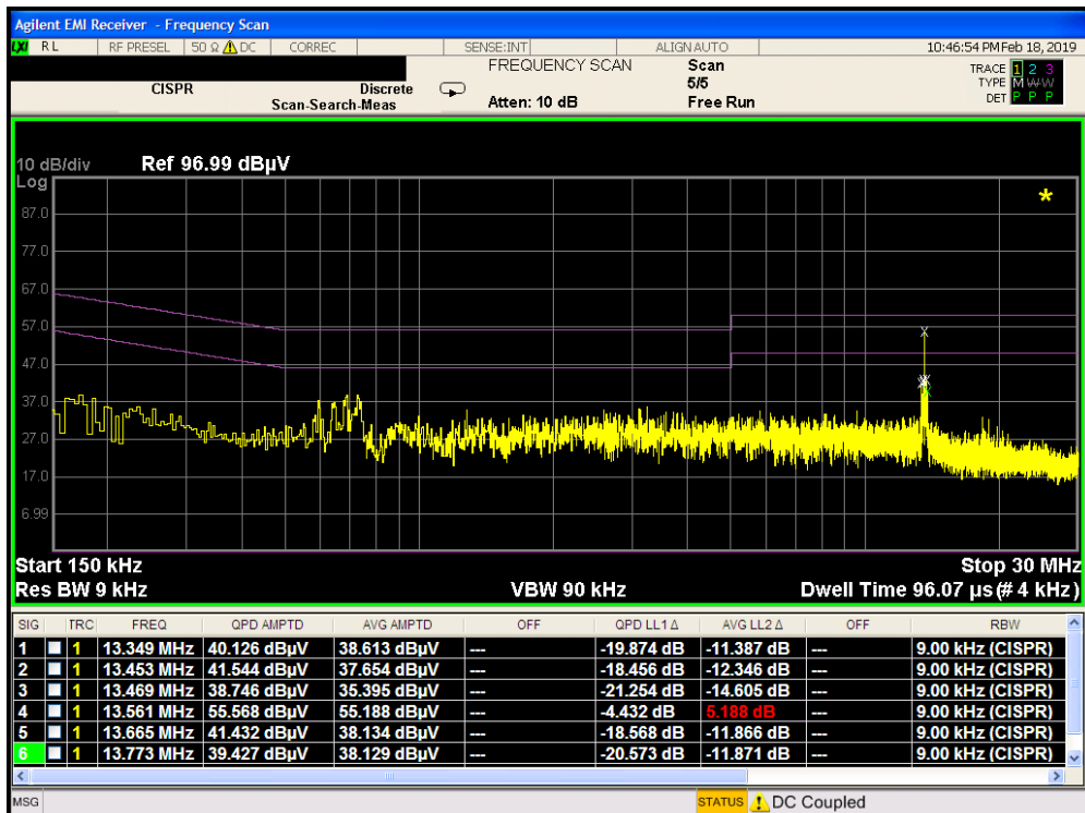
Plot 7-6. Line-Conducted Test Plot (N) with RFID Antenna
