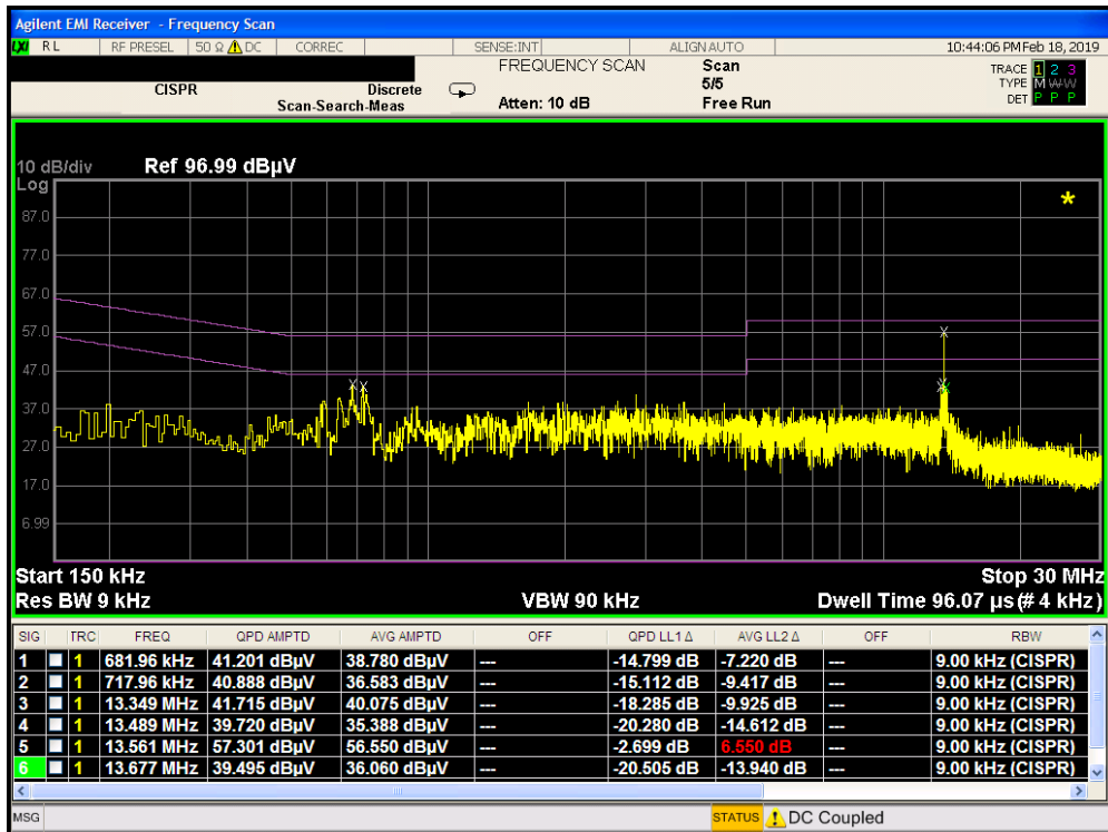
Plot 7-5. Line-Conducted Test Plot (L1) with RFID Antenna
