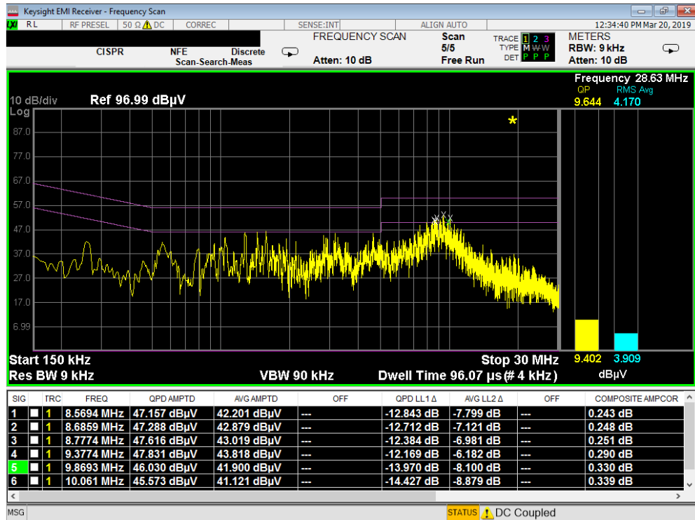
Plot 7-7. Line-Conducted Test Plot (L1) with Antenna Terminated in 50ohms
