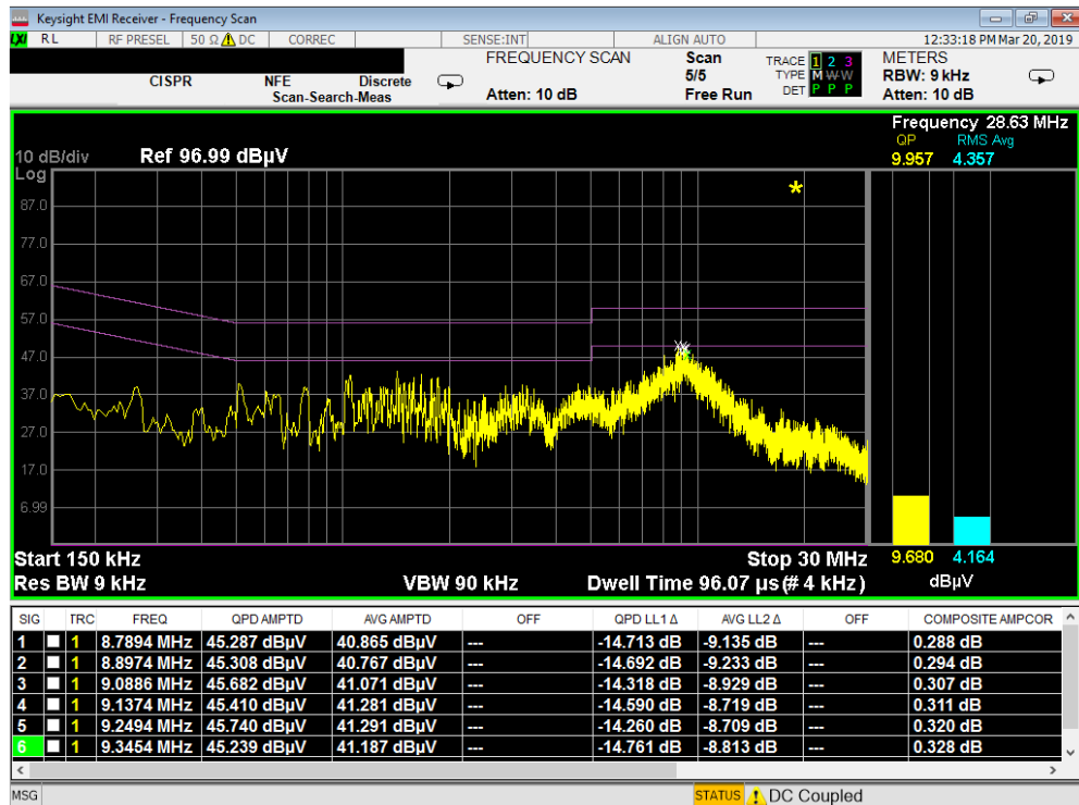
Plot 7-8. Line-Conducted Test Plot (N) with Antenna Terminated in 50ohms
