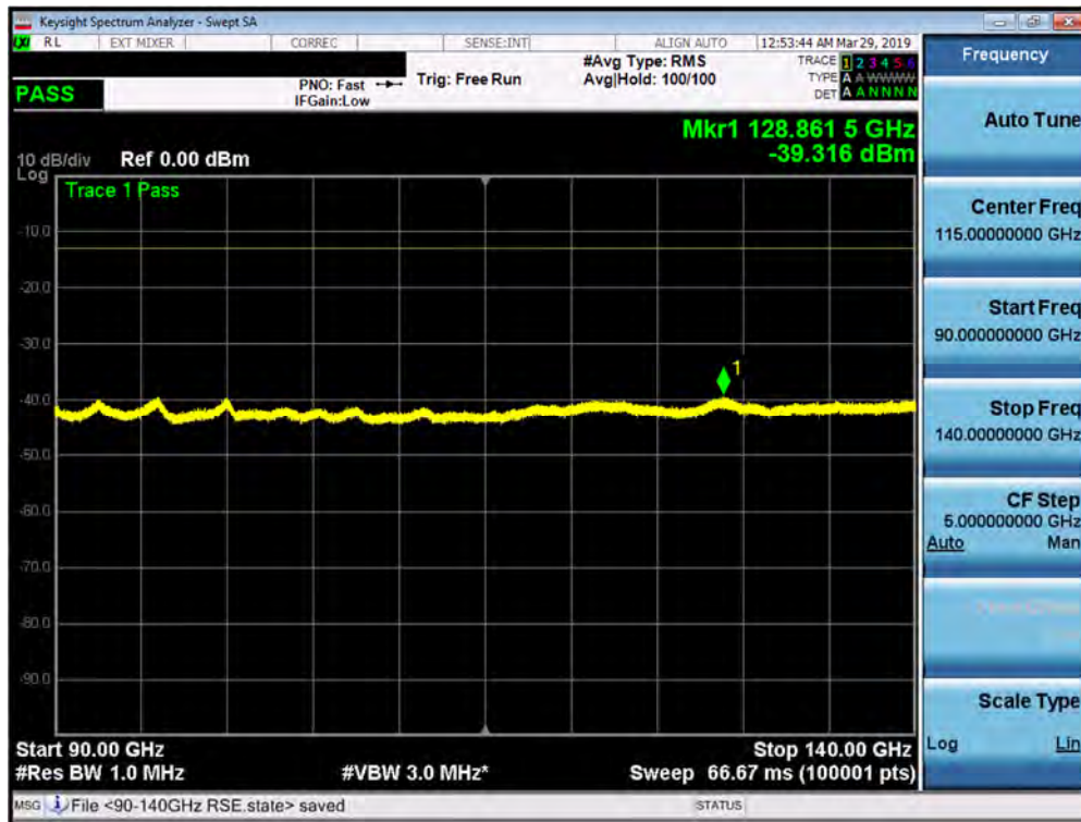
Plot 7-71. J Dipole Radiated Spurious Plot 90-140 GHz (1CC QPSK Low Channel H Beam)
