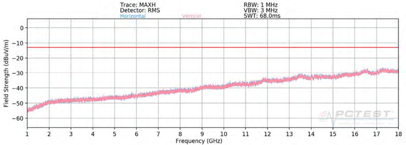
Plot 7-51. J Dipole Radiated Spurious Plot 1-18 GHz (1CC QPSK Mid Channel H Beam)
