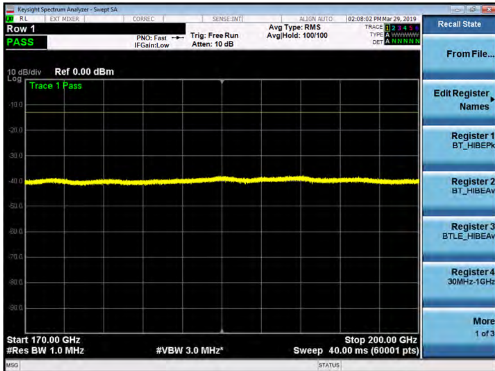
Plot 7-84. J Dipole Radiated Spurious Plot 170-200 GHz (1CC QPSK Mid Channel H Beam)
