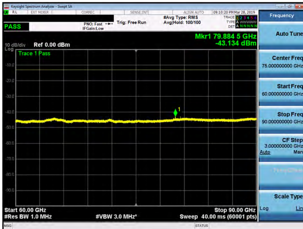
Plot 7-70. J Dipole Radiated Spurious Plot 60-90 GHz (1CC QPSK High Channel V Beam)
