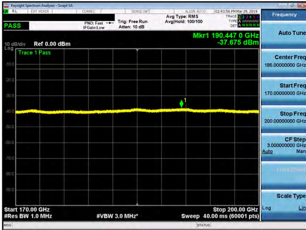
Plot 7-83. J Dipole Radiated Spurious Plot 170-200 GHz (1CC QPSK Low Channel H Beam)
