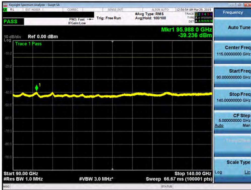
Plot 7-76. J Dipole Radiated Spurious Plot 90-140 GHz (1CC QPSK High Channel V Beam)
