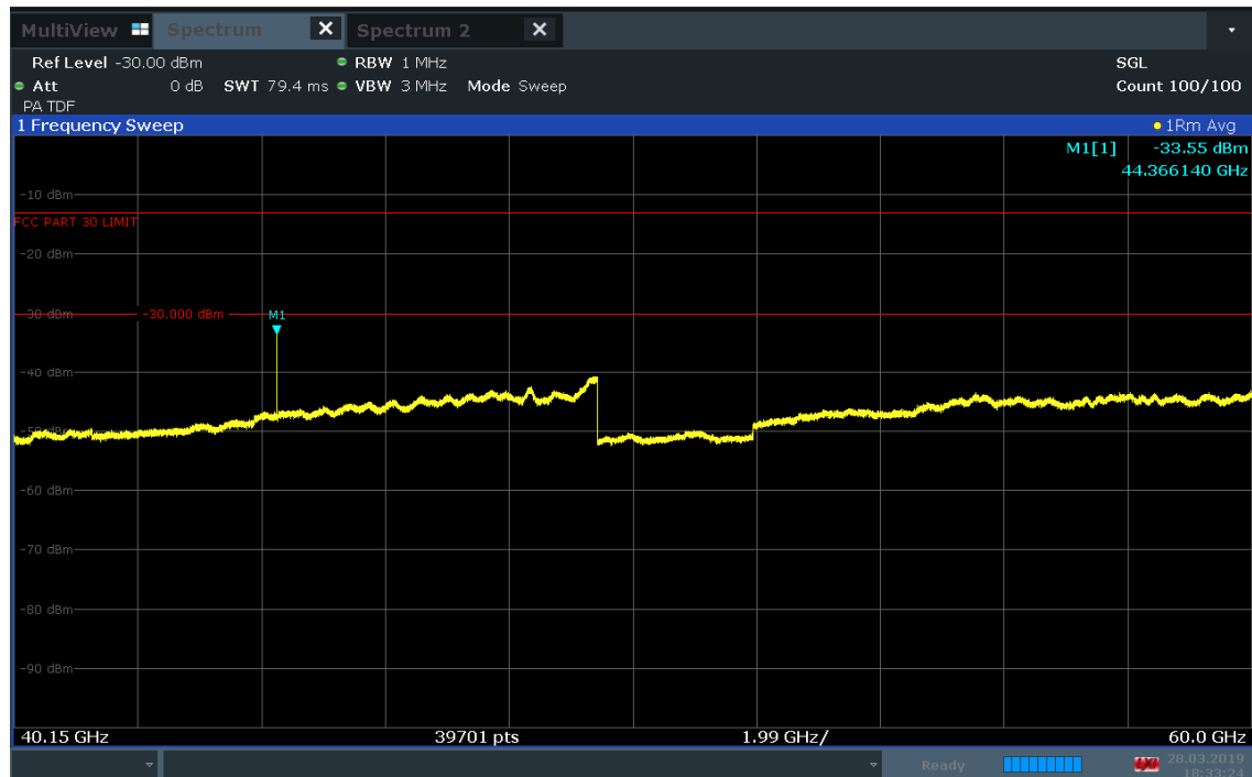
Plot 7-180. L Patch Radiated Spurious Plot 40.15-60 GHz (1CC QPSK Mid Channel H Beam)
