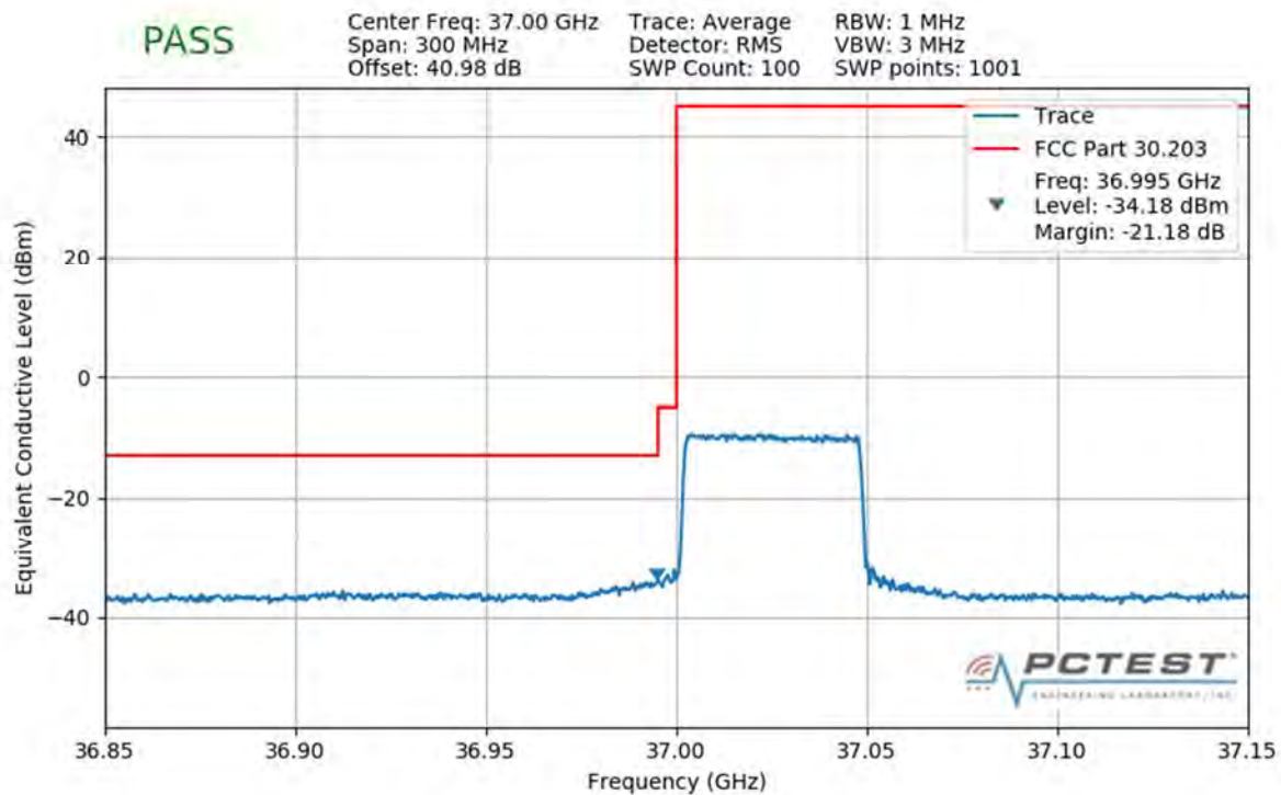
Plot 7-305. Lower Band Edge Plot (1CC 50MHz QPSK Full RB)
