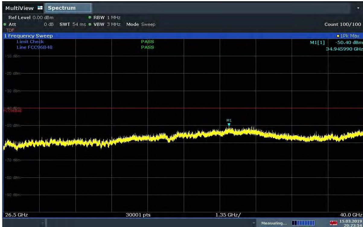
Plot 7-42. Radiated Spurious Plot 26.5 - 40GHz (Band 48 Ant Pol V)
