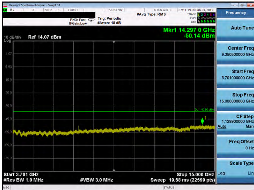
Plot 7-24. Conducted Spurious Plot (Band 48 - 20.0MHz QPSK - RB Size 1, RB Offset 0 - High Channel)
