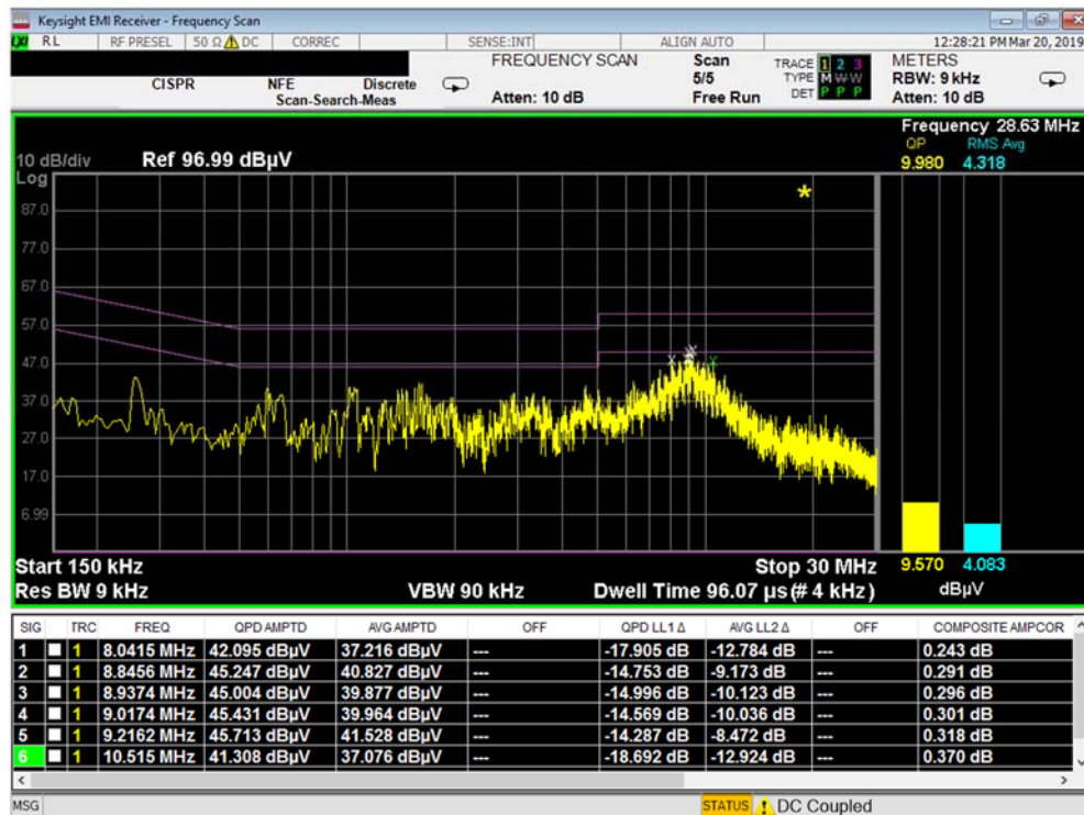
Plot 7-24. Line Conducted Plot (N)
