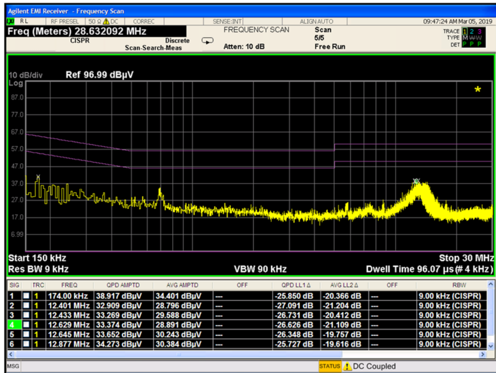
Plot 7-22. Line Conducted Plot (N)
