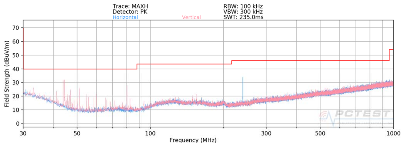
Plot 7-9. Radiated Spurious Plot below 1GHz [Radiated Test Config. 5]
