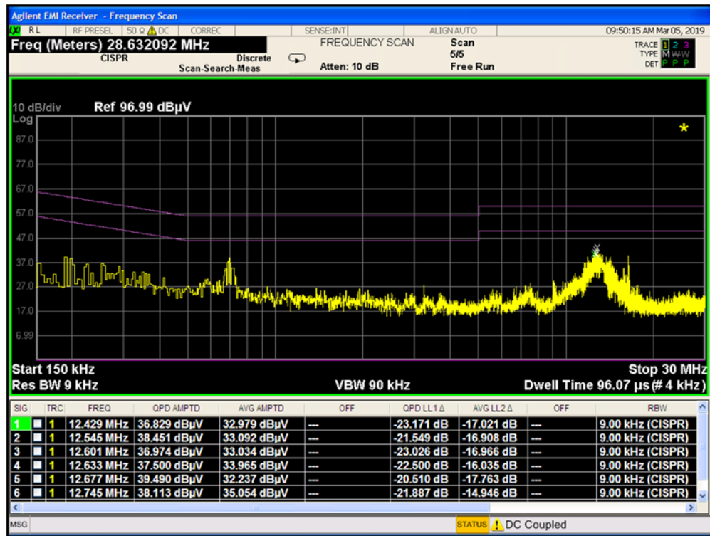
Plot 7-21. Line Conducted Plot (L1)
