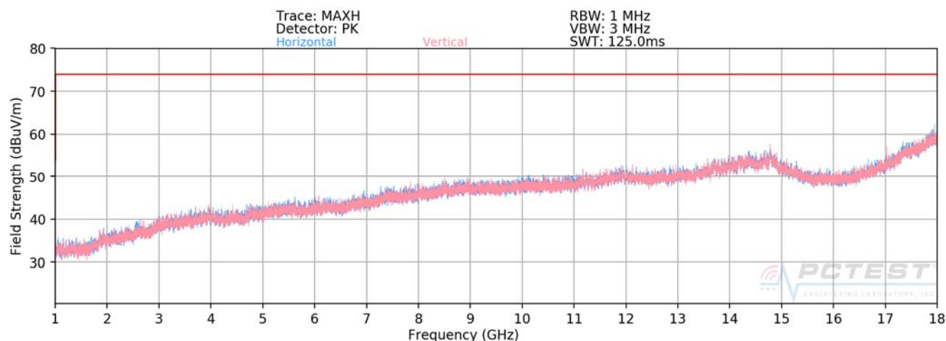
Plot 7-12. Radiated Spurious Plot above 1GHz [Radiated Test Config. 6]
