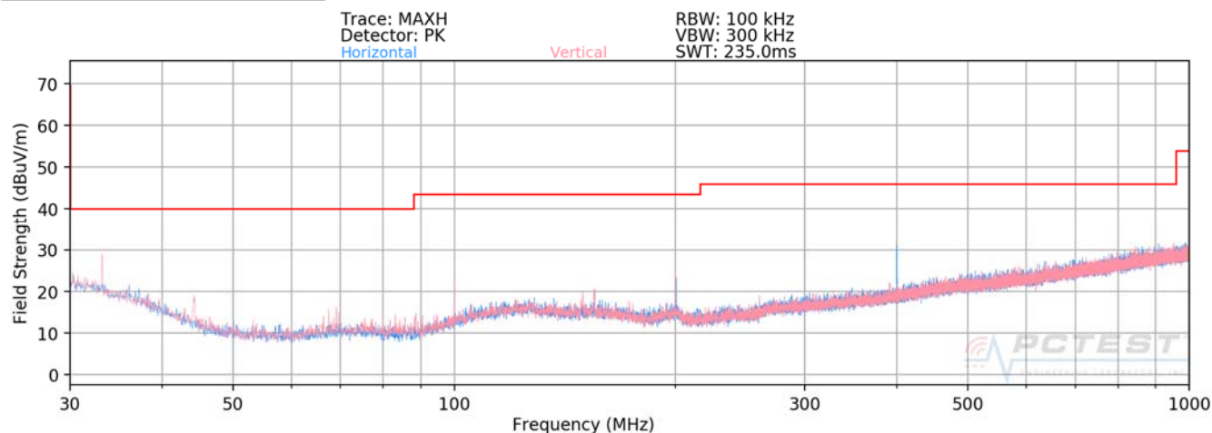
Plot 7-11. Radiated Spurious Plot below 1GHz [Radiated Test Config. 6]
