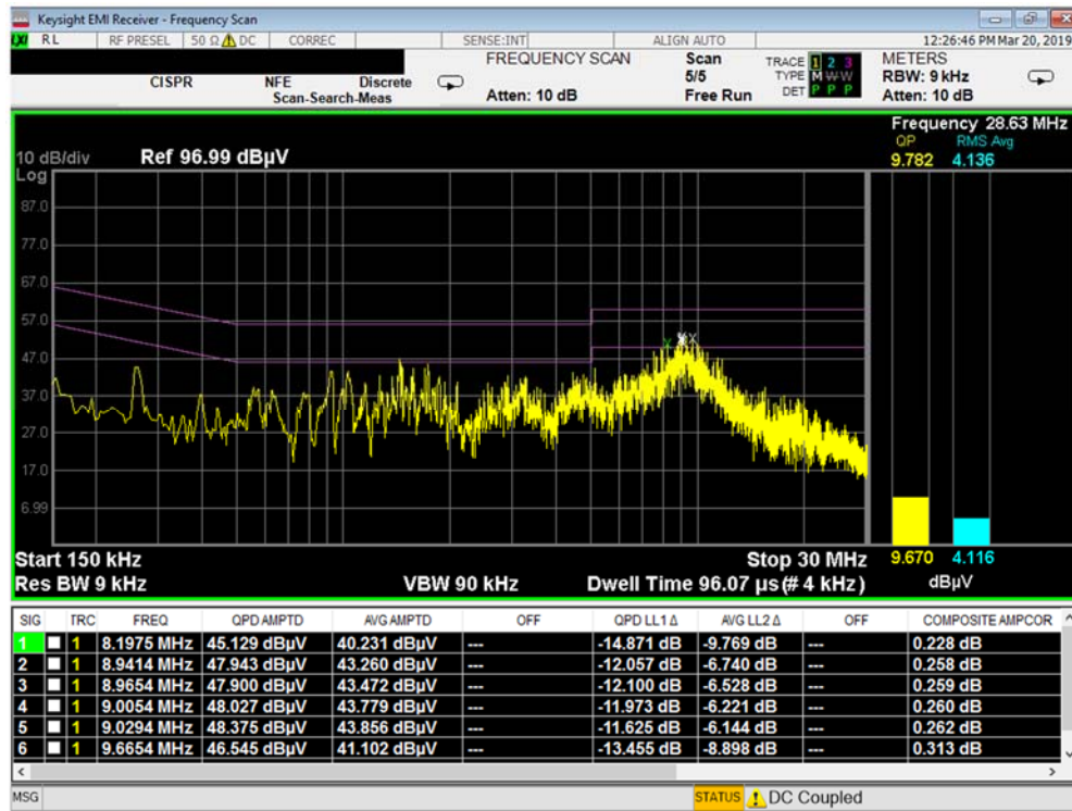
Plot 7-23. Line Conducted Plot (L1)
