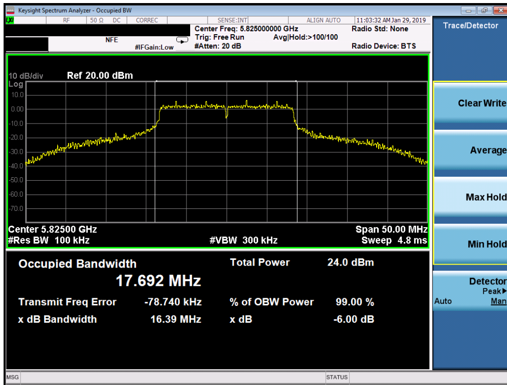
Plot 7-120. 6dB Bandwidth Plot SISO ANT2 (802.11a (UNII Band 3) – Ch. 165)
