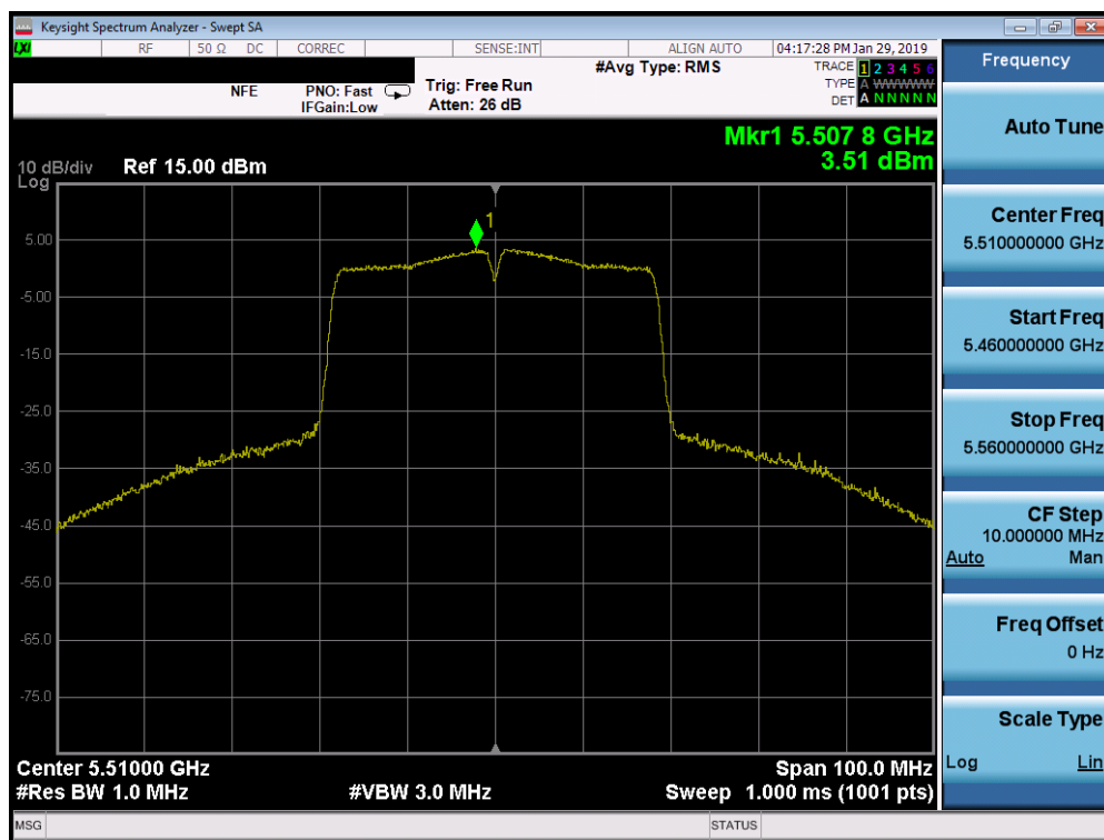
Plot 7-172. Power Spectral Density Plot SISO ANT1 (40MHz BW 802.11n (UNII Band 2C) – Ch. 102)
