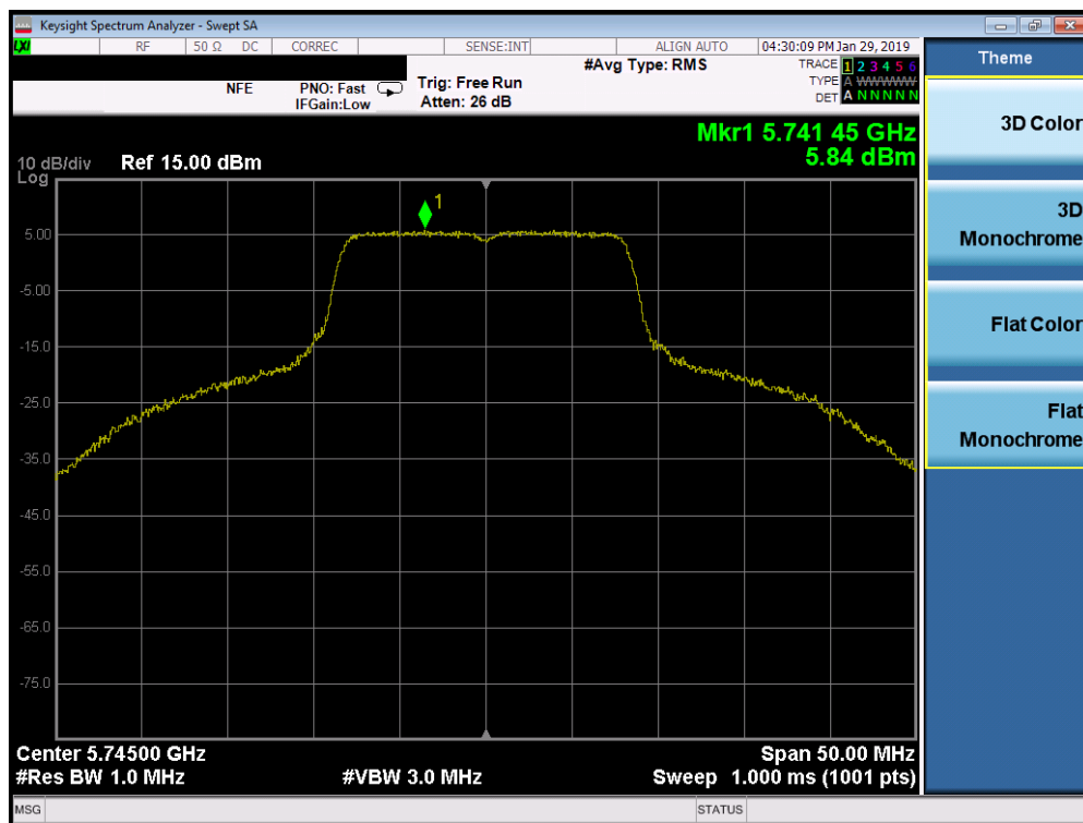
Plot 7-184. Power Spectral Density Plot SISO ANT1 (802.11a (UNII Band 3) – Ch. 149)
