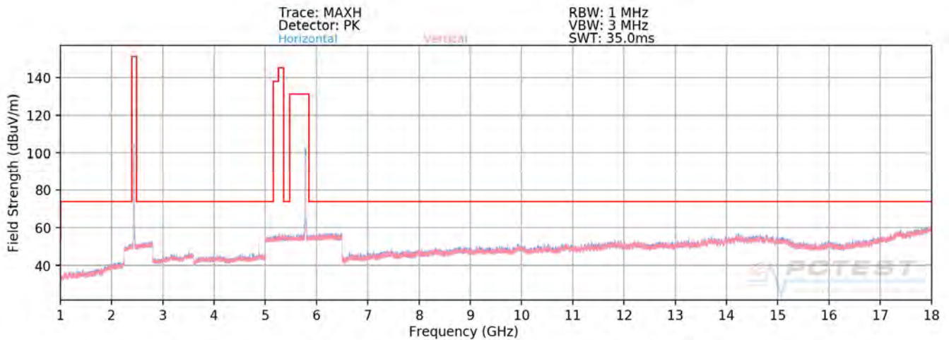
Plot 7-283. Radiated Spurious Plot above 1GHz (2.4GHz – 5GHz)
