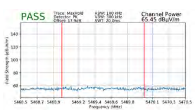
Plot 7-306. Radiated Lower Band Edge Plot SISO ANT1 (Peak – UNII Band 2C)
