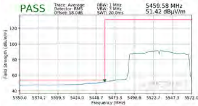
Plot 7-341. Radiated Lower Band Edge Plot SISO ANT2 (Average – UNII Band 2C)
