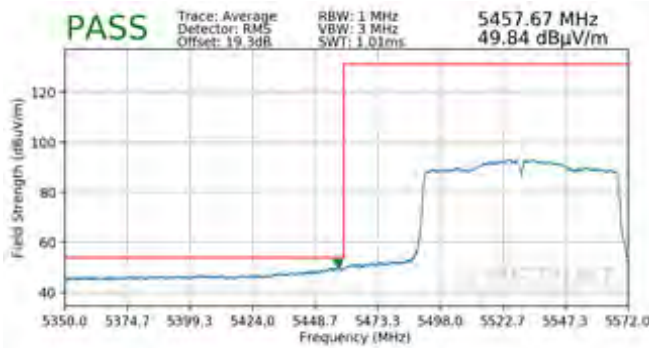
Plot 7-380. Radiated Band Edge Plot ANT (Average – WCP)
