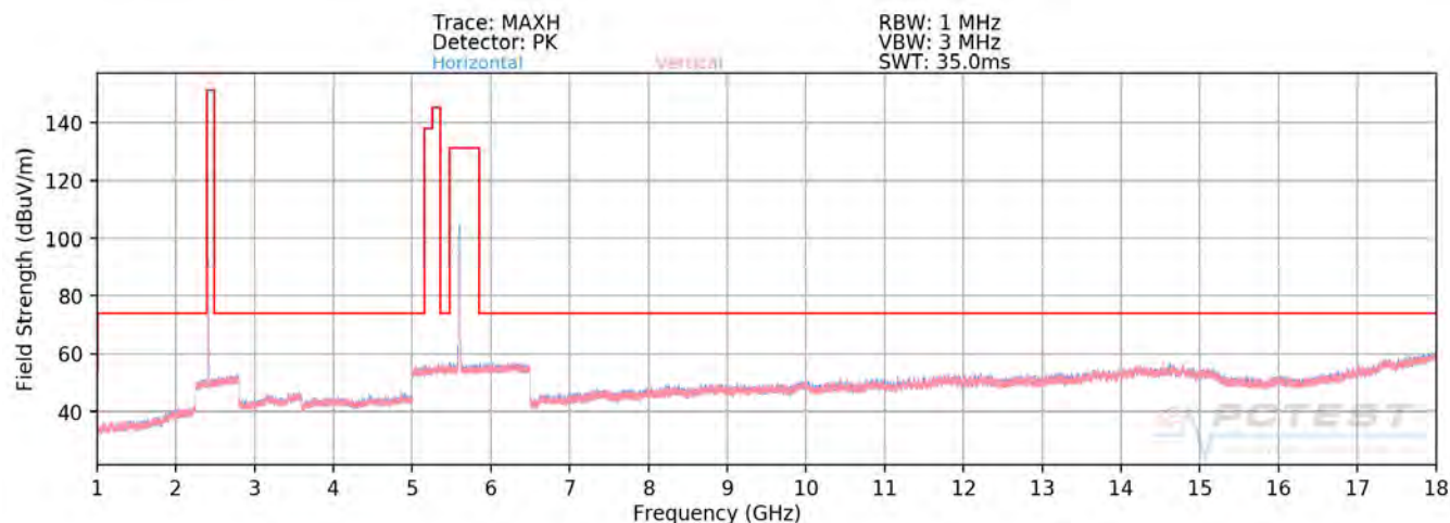
Plot 7-286. Radiated Spurious Plot above 1GHz (5GHz – 2.4 GHz)
