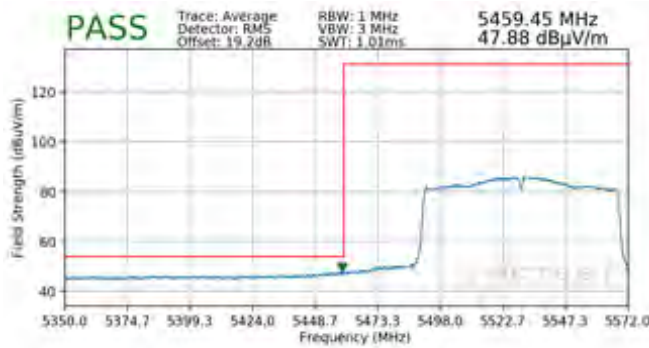
Plot 7-344. Radiated Band Edge Plot SISO ANT2 (Average – WCP)
