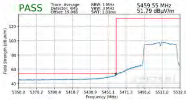
Plot 7-308. Radiated Band Edge Plot SISO ANT1 (Average – WCP)
