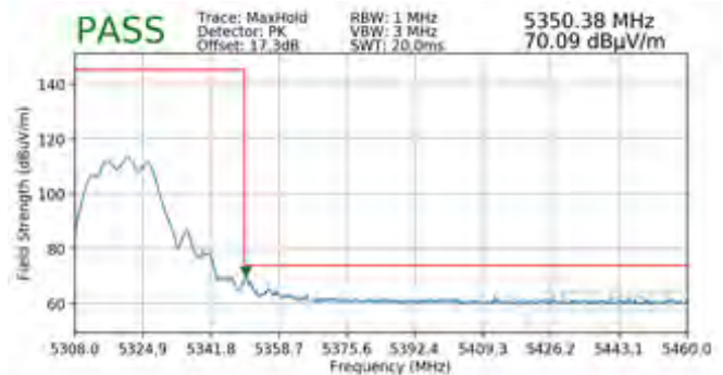
Plot 7-349. Radiated Upper Band Edge Plot CDD (Peak – UNII Band 2A)
