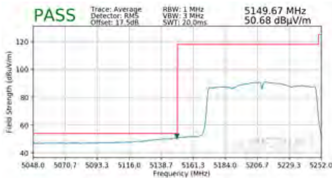
Plot 7-337. Radiated Lower Band Edge Plot SISO ANT2 (Average – UNII Band 1)
