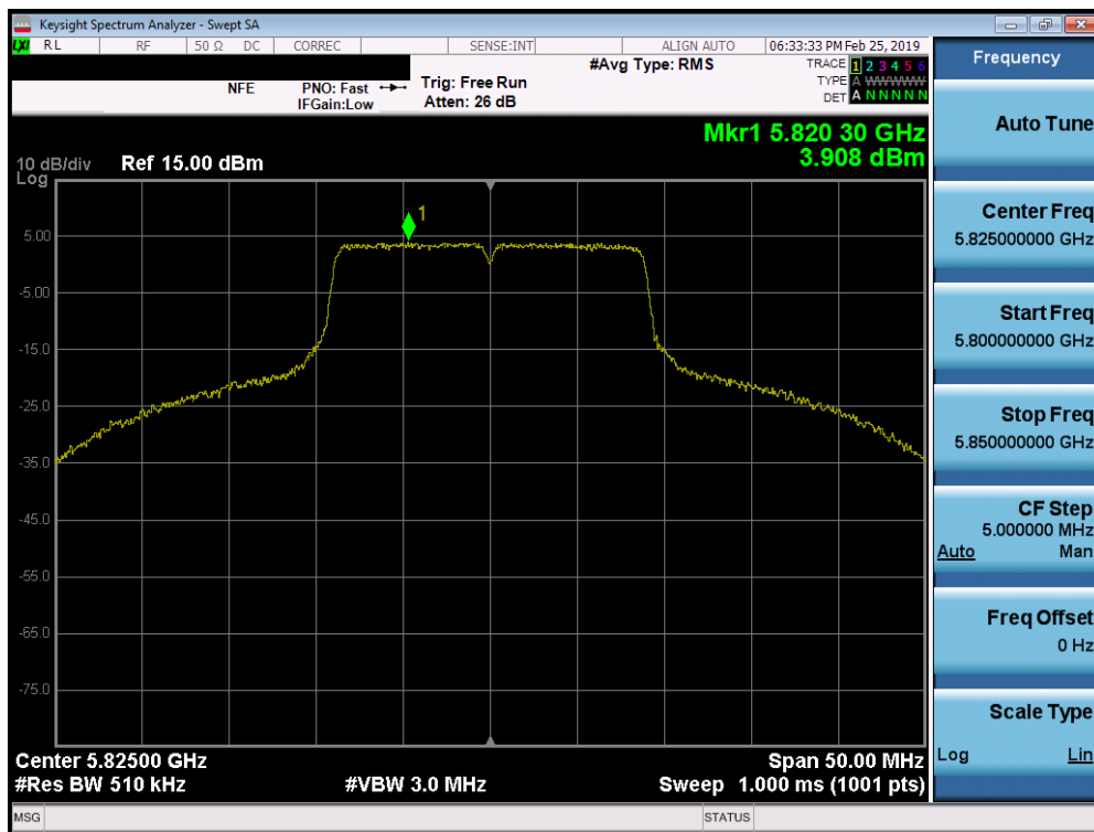
Plot 7-252. Power Spectral Density Plot SISO ANT2 (802.11a (UNII Band 3) – Ch. 165)
