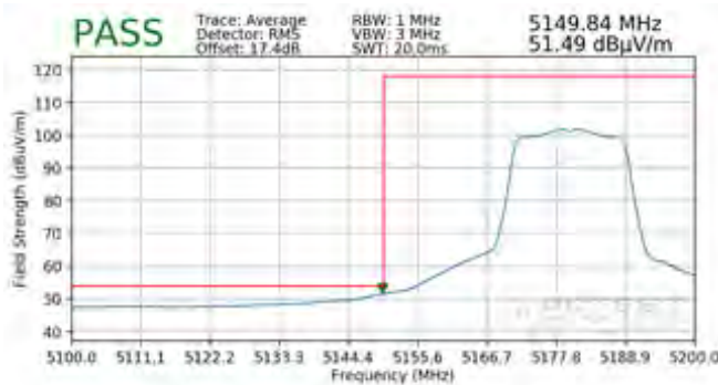
Plot 7-292. Radiated Lower Band Edge Plot SISO ANT1 (Average – UNII Band 1)
