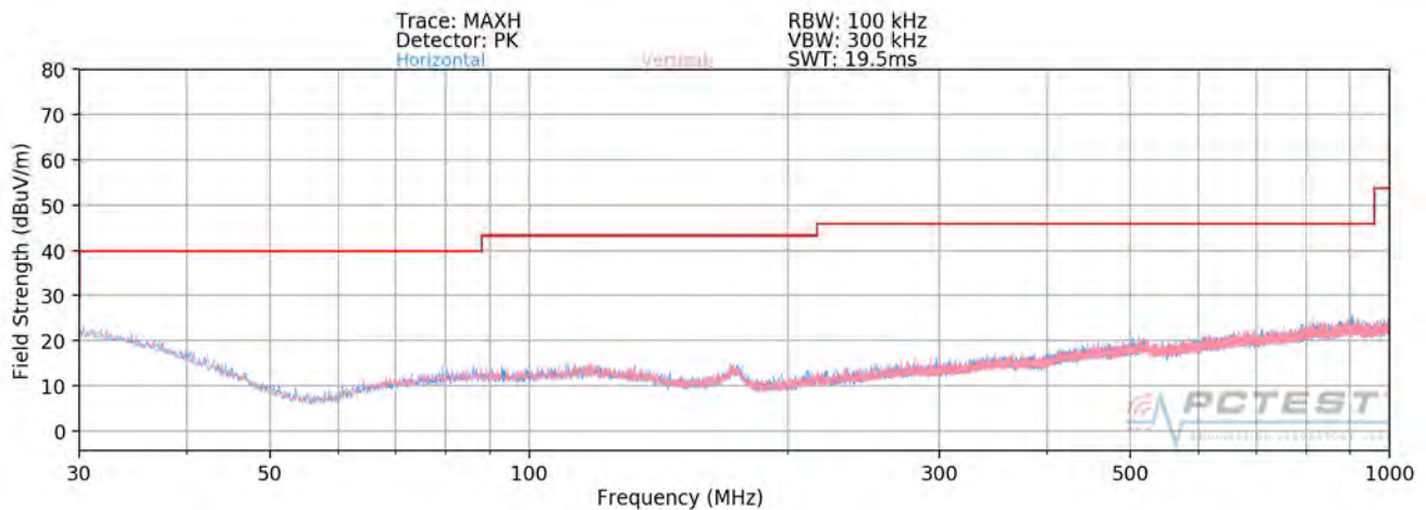
Plot 7-385. Radiated Spurious Plot below 1GHz (5GHz – 2.4 GHz)
