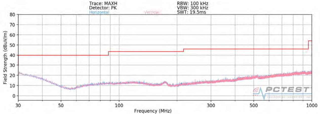
Plot 7-384. Radiated Spurious Plot below 1GHz (2.4GHz – 5GHz)
