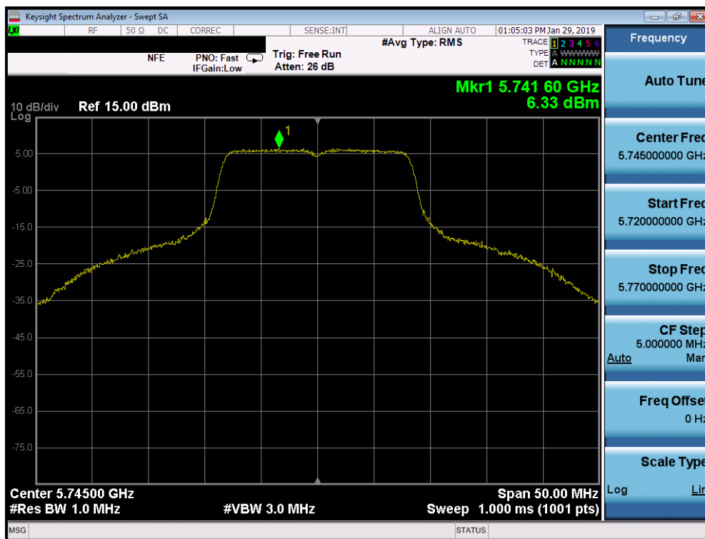
Plot 7-250. Power Spectral Density Plot SISO ANT2 (802.11a (UNII Band 3) – Ch. 149)
