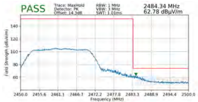
Plot 7-112. Radiated Restricted Band Edge Measurement MIMO with WCP (Peak)
