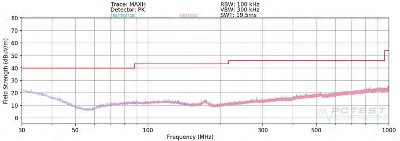
Plot 7-115. Radiated Spurious Plot below 1GHz CDD/MIMO
