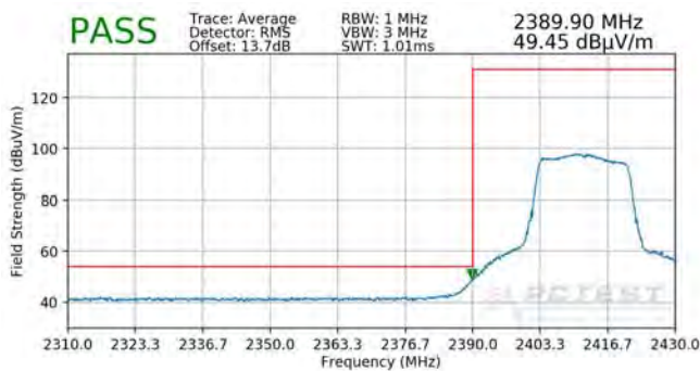
Plot 7-89. Radiated Restricted Lower Band Edge Measurement SISO ANT1 (Average)
