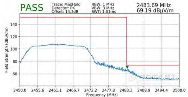
Plot 7-92. Radiated Restricted Upper Band Edge Measurement SISO ANT1 (Peak)
