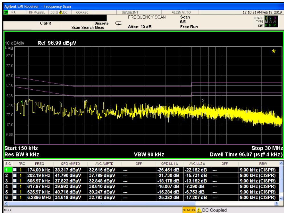
Plot 7-119. Line Conducted Plot with 802.11b (N) with Wireless Charging Pad
