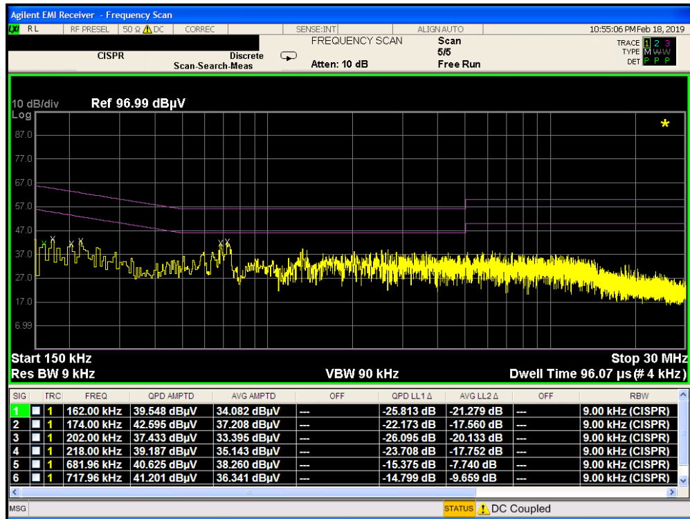
Plot 7-116. Line Conducted Plot with 802.11b (L1) with Travel Adapter
