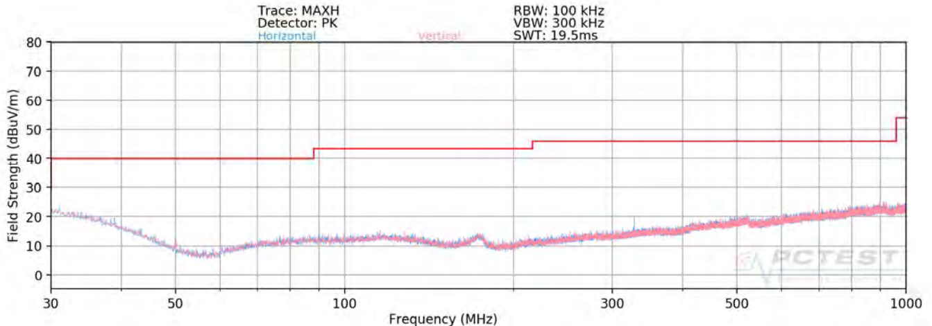
Plot 7-114. Radiated Spurious Plot below 1GHz SISO ANT2
