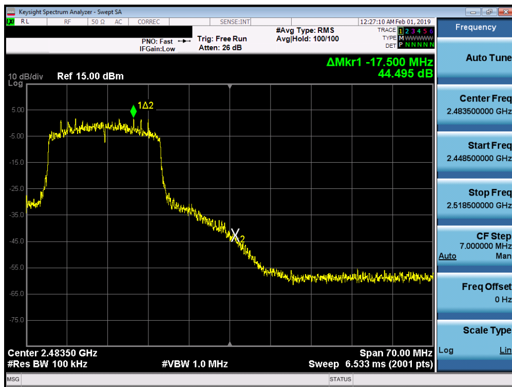
Plot 7-64. Band Edge Plot SISO ANT2 (802.11ax (2.4GHz) – Ch. 11)
