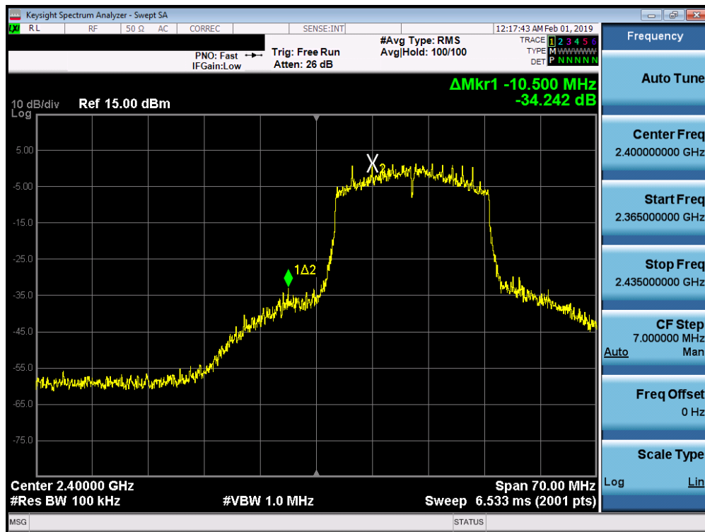
Plot 7-63. Band Edge Plot SISO ANT2 (802.11ax (2.4GHz) – Ch. 1)
