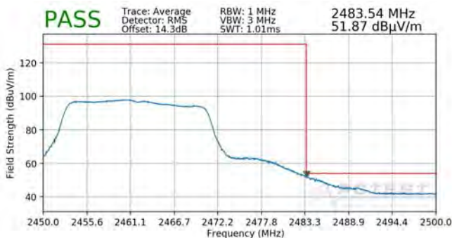
Plot 7-109. Radiated Restricted Upper Band Edge Measurement MIMO (Average)
