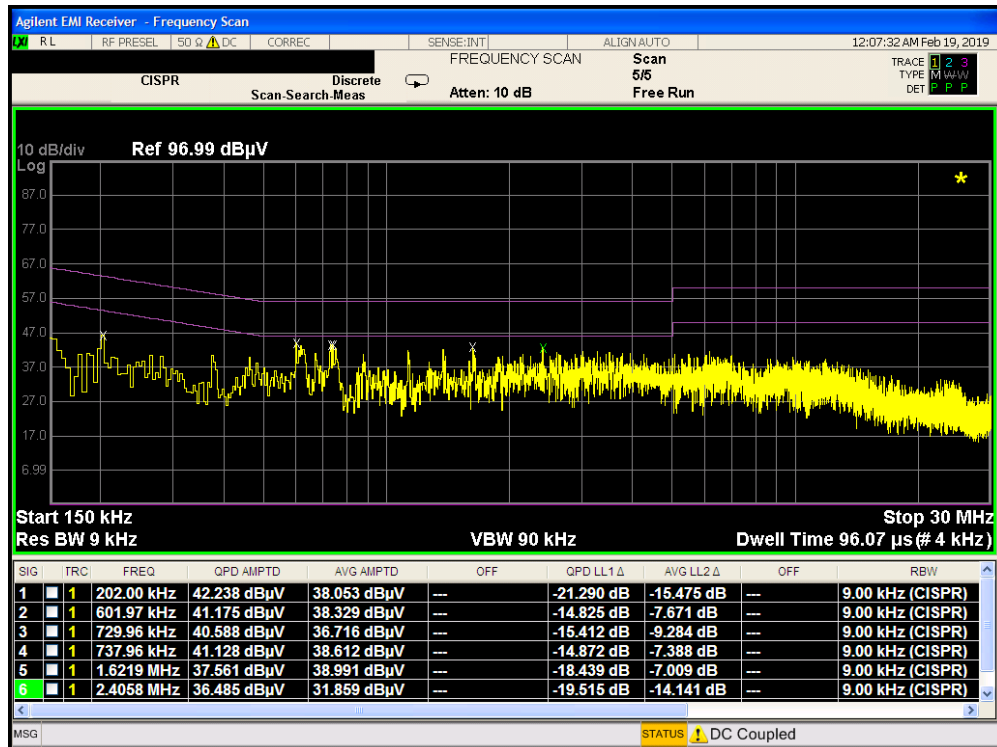
Plot 7-118. Line Conducted Plot with 802.11b (L1) with Wireless Charging Pad
