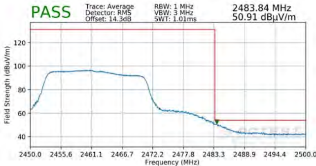
Plot 7-97. Radiated Restricted Upper Band Edge Measurement SISO ANT2 (Average)
