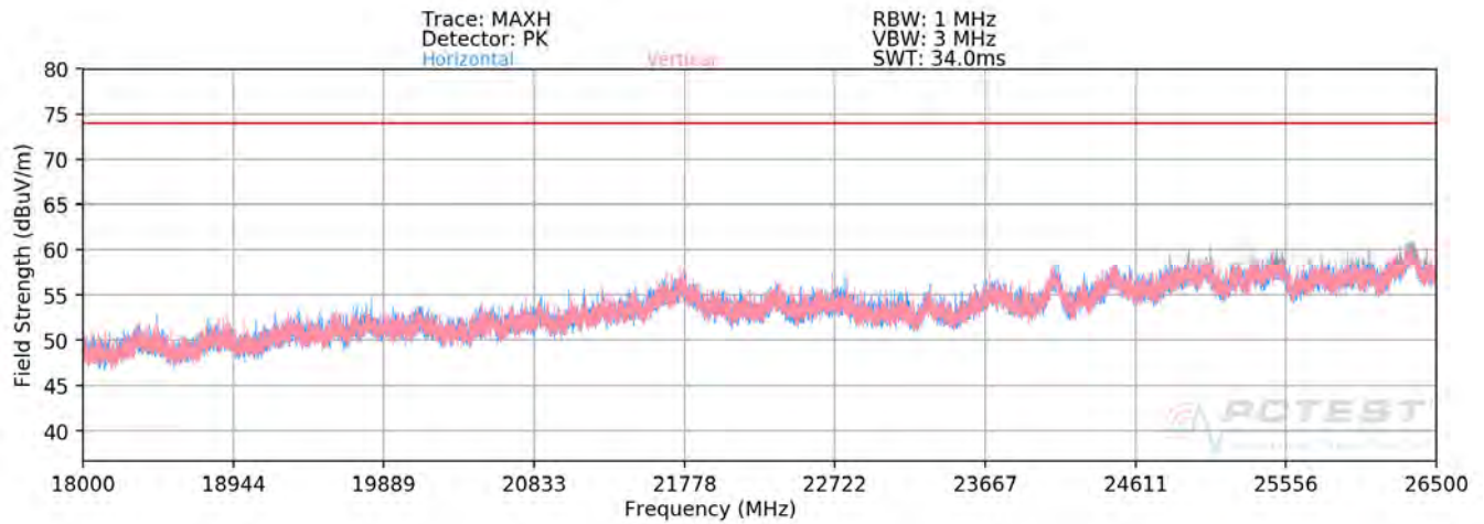
Plot 7-88. Radiated Spurious Plot above 18GHz MIMO/CDD
