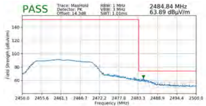
Plot 7-94. Radiated Restricted Band Edge Measurement SISO ANT1 with WCP (Peak)
