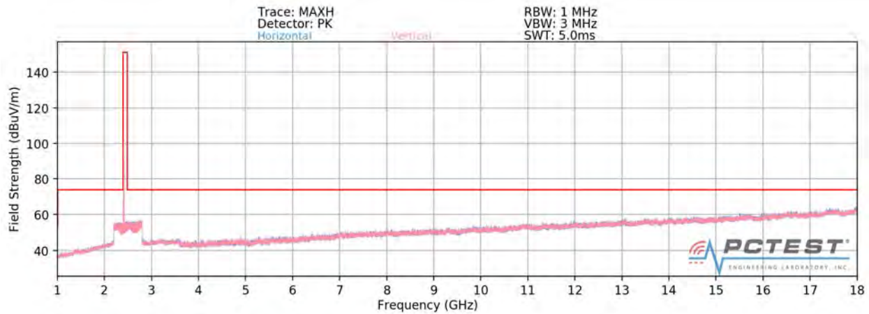
Plot 7-81. Radiated Spurious Plot above 1GHz SISO ANT2 (802.11b – Ch. 1)
