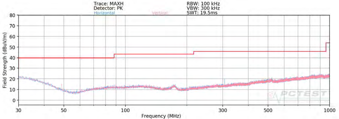
Plot 7-113. Radiated Spurious Plot below 1GHz SISO ANT1
