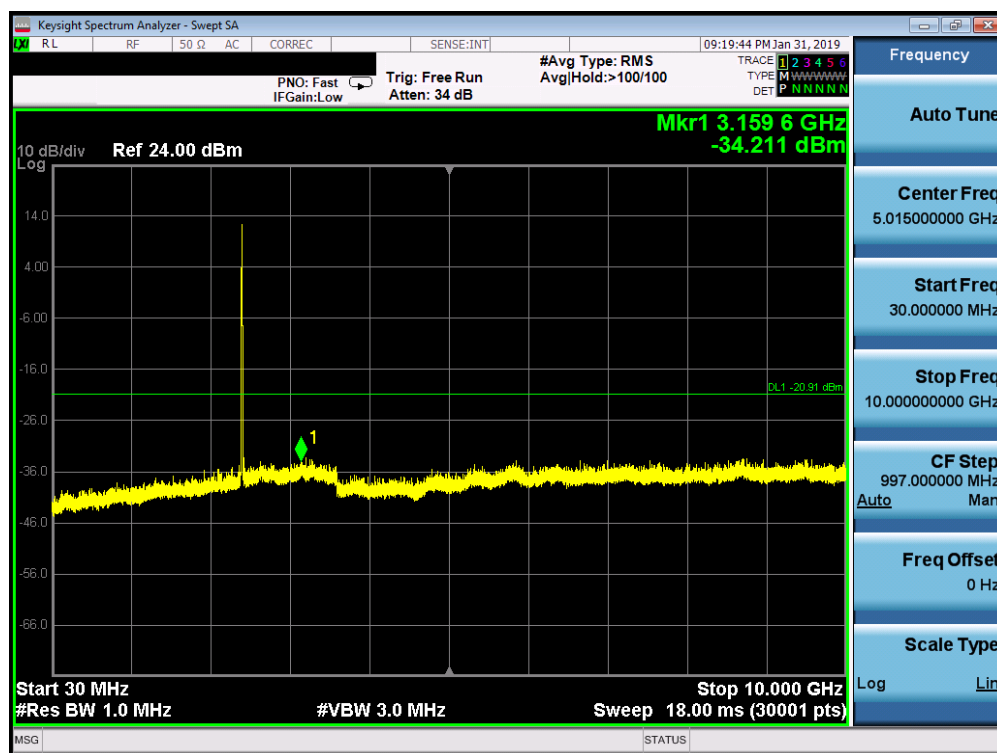
Plot 7-65. Conducted Spurious Plot SISO ANT1 (802.11b – Ch. 1)
