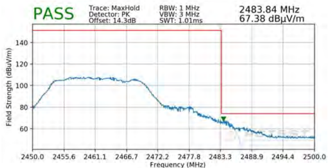
Plot 7-104. Radiated Restricted Upper Band Edge Measurement CDD (Peak)
