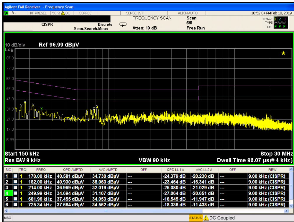
Plot 7-117. Line Conducted Plot with 802.11b (N) with Travel Adapter
