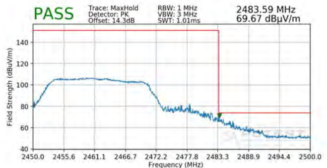
Plot 7-110. Radiated Restricted Upper Band Edge Measurement MIMO (Peak)
