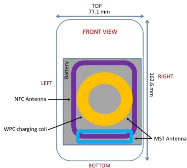
Figure F-2 NFC Antenna Locations
