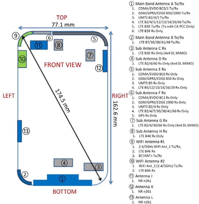
Figure F-1 DUT Antenna Locations
