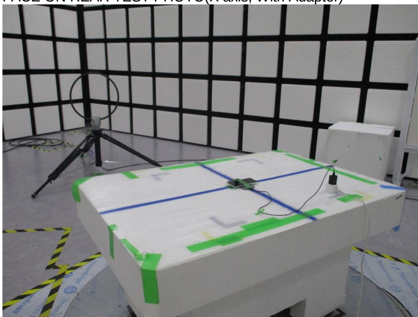
FACE ON REAR TEST PHOTO(X axis, With Adapter)
