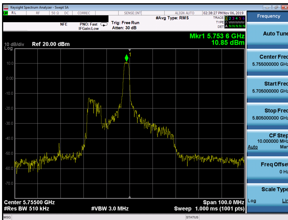
Plot 7-79. Power Spectral Density Plot SISO ANT1 (40MHz BW 802.11ax – 26 Tones (UNII Band 3) – Ch. 151)
