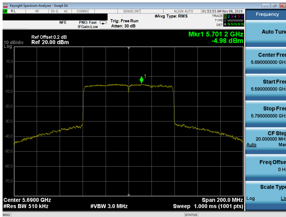
Plot 7-102. Power Spectral Density Plot SISO ANT1 (80MHz BW 802.11ax – Full Tones (UNII Band 2C) – Ch. 138)
