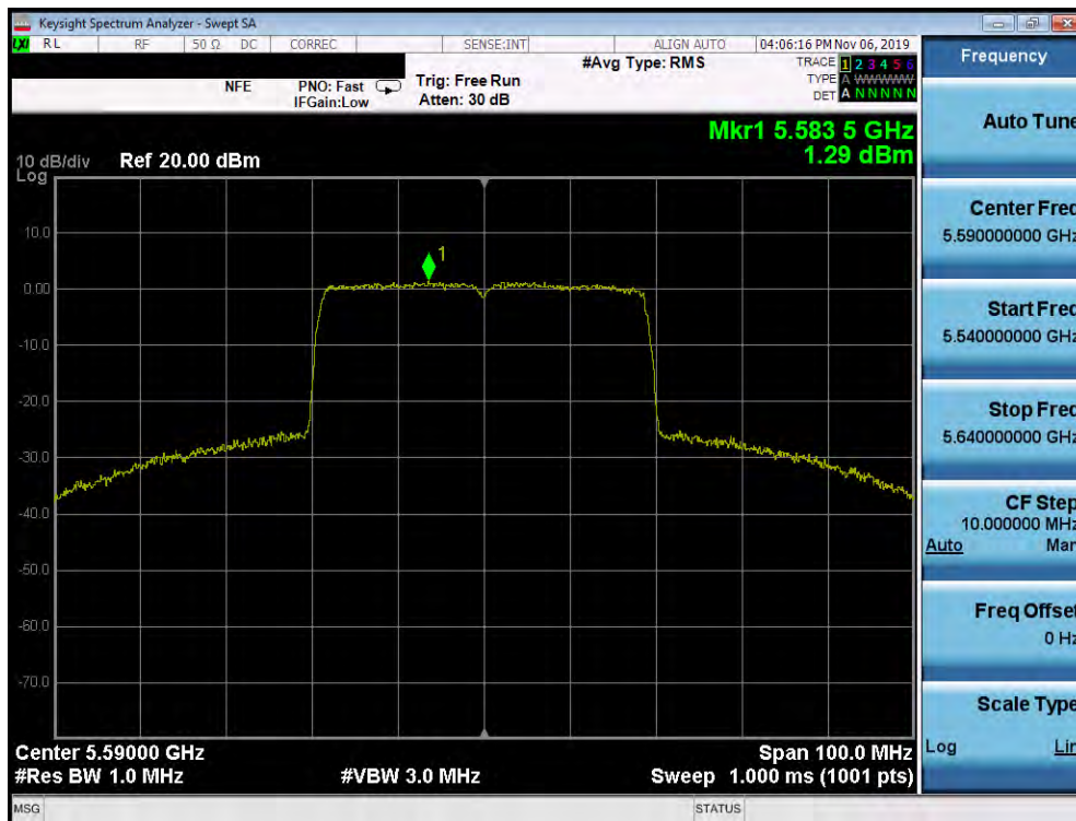
Plot 7-98. Power Spectral Density Plot SISO ANT1 (40MHz BW 802.11ax – Full Tones (UNII Band 2C) – Ch. 118)
