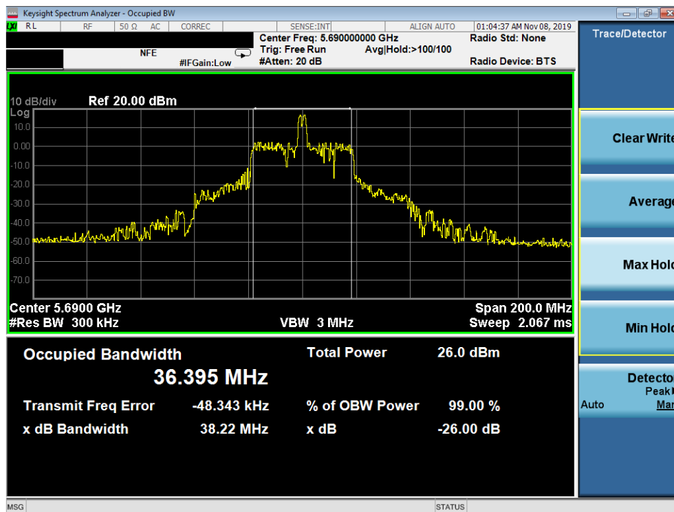
Plot 7-42. 26dB Bandwidth Plot SISO ANT2 (80MHz BW 802.11ax – 26 Tones (UNII Band 2C) – Ch. 138)
