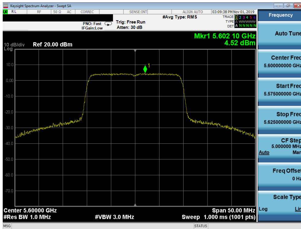
Plot 7-95. Power Spectral Density Plot SISO ANT1 (20MHz BW 802.11ax – Full Tones (UNII Band 2C) – Ch. 120)
