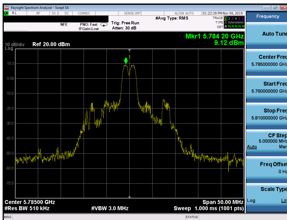
Plot 7-77. Power Spectral Density Plot SISO ANT1 (20MHz BW 802.11ax – 26 Tones (UNII Band 3) – Ch. 157)
