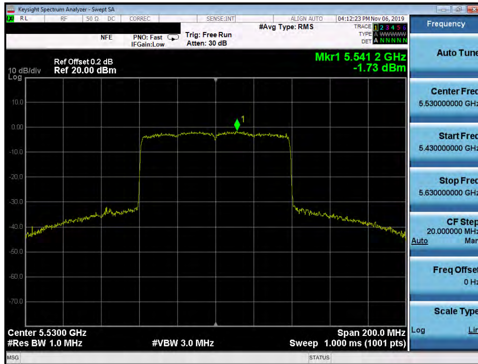
Plot 7-100. Power Spectral Density Plot SISO ANT1 (80MHz BW 802.11ax – Full Tones (UNII Band 2C) – Ch. 106)
