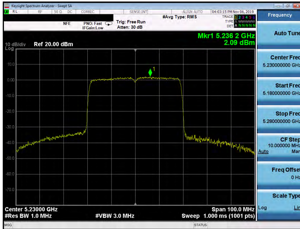
Plot 7-86. Power Spectral Density Plot SISO ANT1 (40MHz BW 802.11ax - Full Tones (UNII Band 1) - Ch. 46)
