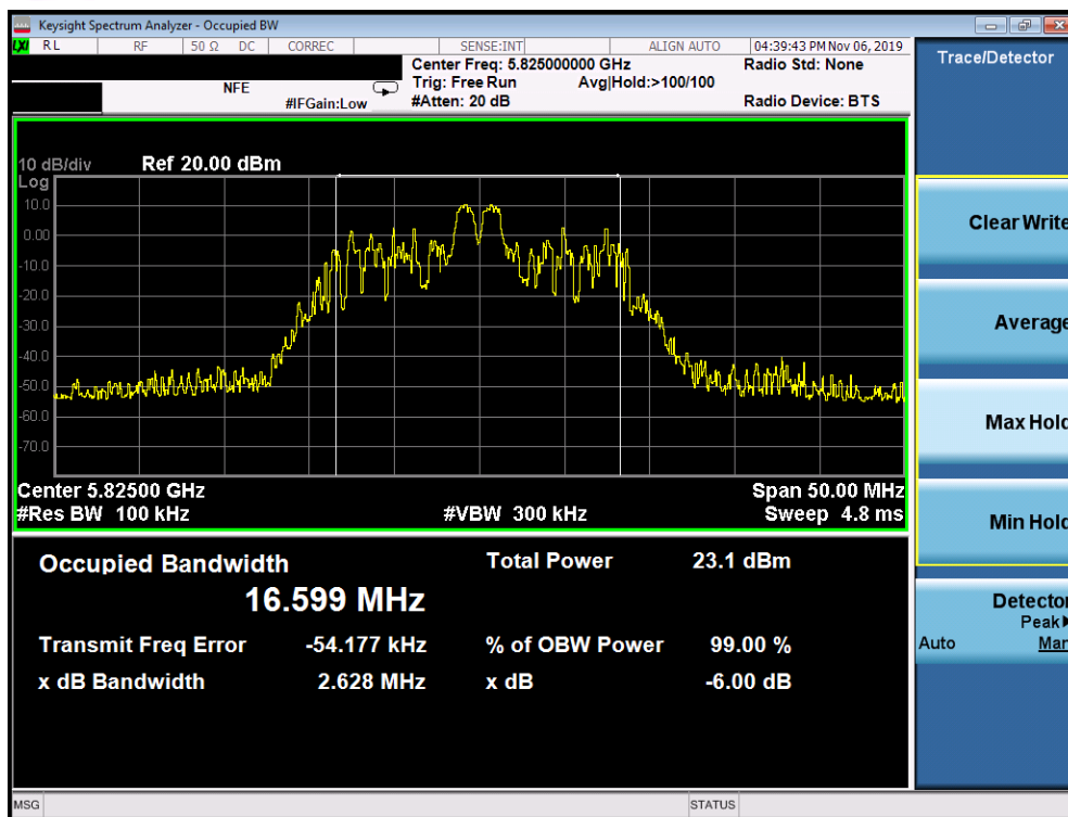
Plot 7-51. 6dB Bandwidth Plot SISO ANT2 (20MHz BW 802.11ax – 26 Tones (UNII Band 3) – Ch. 165)
