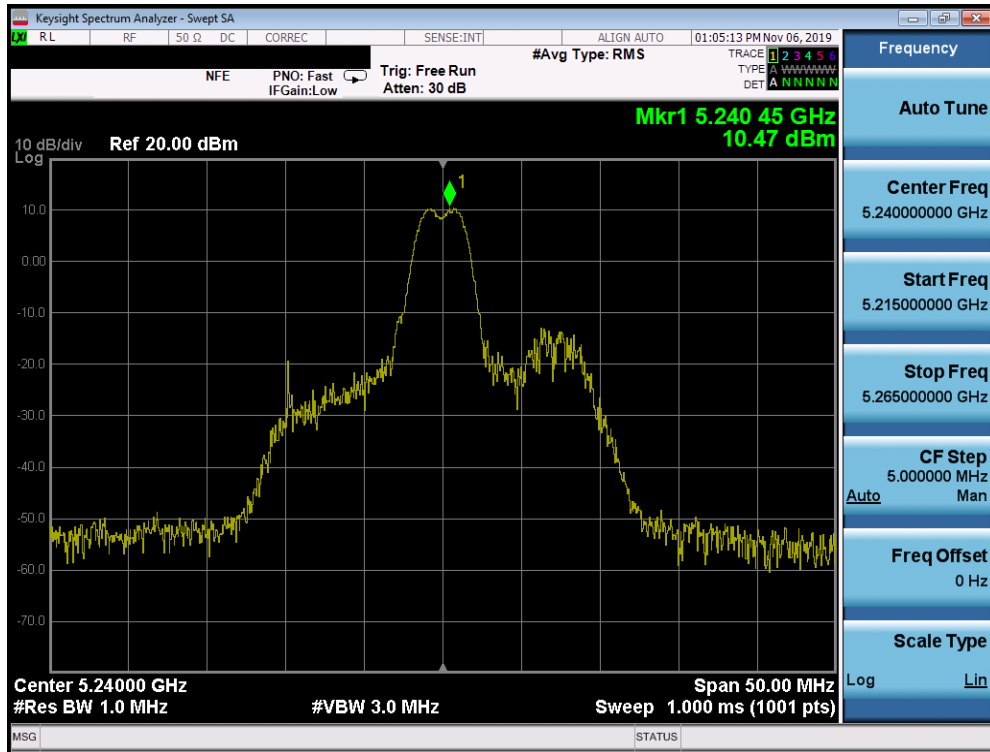
Plot 7-57. Power Spectral Density Plot SISO ANT1 (20MHz BW 802.11ax – 26 Tones (UNII Band 1) – Ch. 48)
