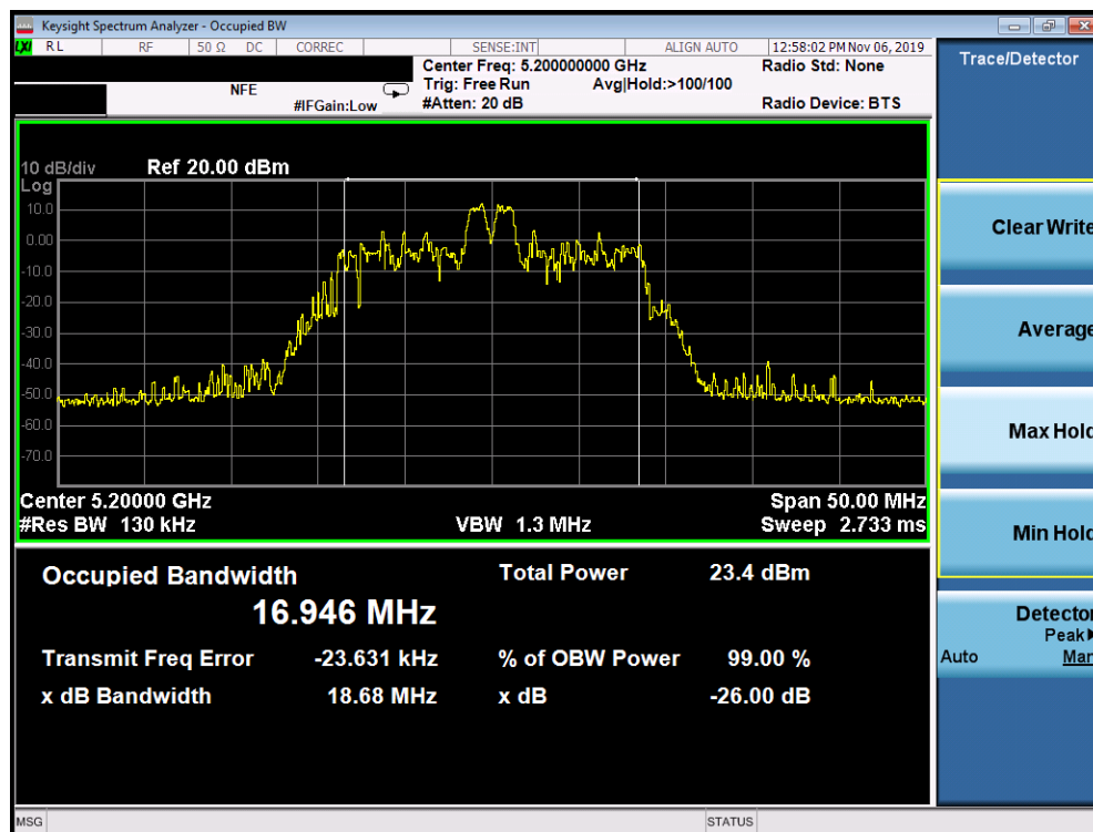
Plot 7-2. 26dB Bandwidth Plot SISO ANT1 (20MHz BW 802.11ax – 26 Tones (UNII Band 1) – Ch. 40)
