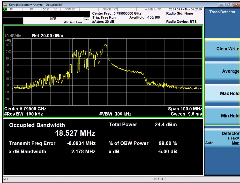
Plot 7-47. 6dB Bandwidth Plot SISO ANT1 (40MHz BW 802.11ax – 26 Tones (UNII Band 3) – Ch. 159)
