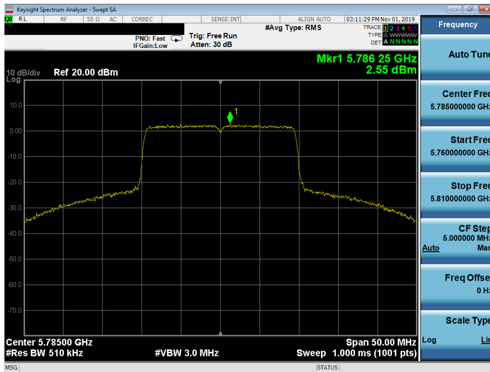
Plot 7-104. Power Spectral Density Plot SISO ANT1 (20MHz BW 802.11ax – Full Tones (UNII Band 3) – Ch. 157)
