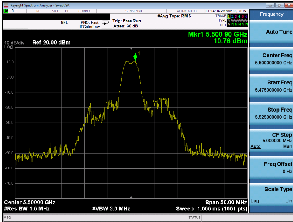
Plot 7-67. Power Spectral Density Plot SISO ANT1 (20MHz BW 802.11ax – 26 Tones (UNII Band 2C) – Ch. 100)
