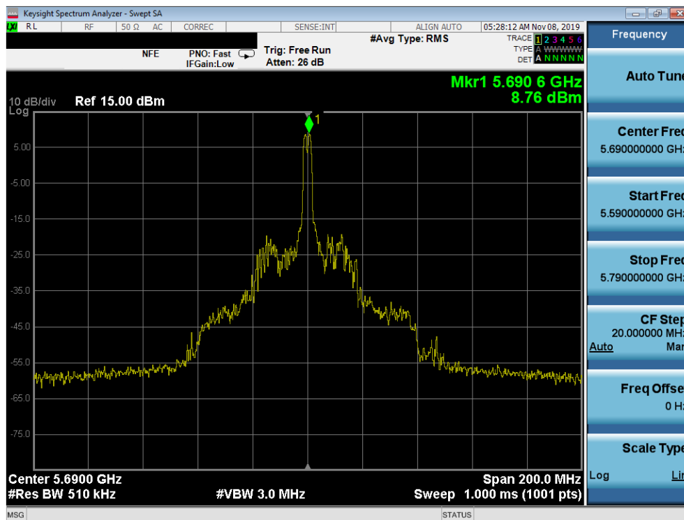
Plot 7-75. Power Spectral Density Plot SISO ANT1 (80MHz BW 802.11ax – 26 Tones (UNII Band 2C) – Ch. 138)
