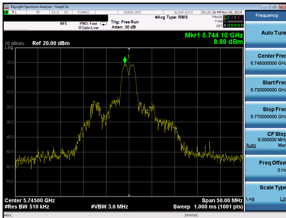
Plot 7-76. Power Spectral Density Plot SISO ANT1 (20MHz BW 802.11ax – 26 Tones (UNII Band 3) – Ch. 149)
