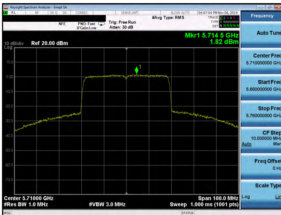
Plot 7-99. Power Spectral Density Plot SISO ANT1 (40MHz BW 802.11ax – Full Tones (UNII Band 2C) – Ch. 142)
