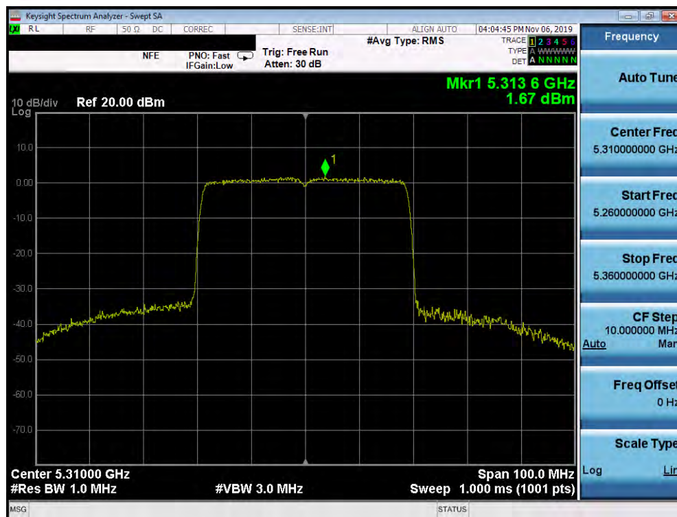
Plot 7-92. Power Spectral Density Plot SISO ANT1 (40MHz BW 802.11ax – Full Tones (UNII Band 2A) – Ch. 62)
