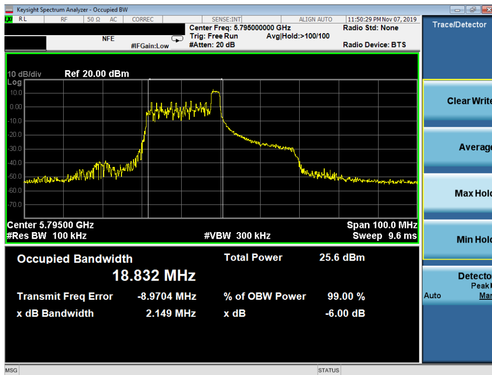
Plot 7-53. 6dB Bandwidth Plot SISO ANT2 (40MHz BW 802.11ax – 26 Tones (UNII Band 3) – Ch. 159)
