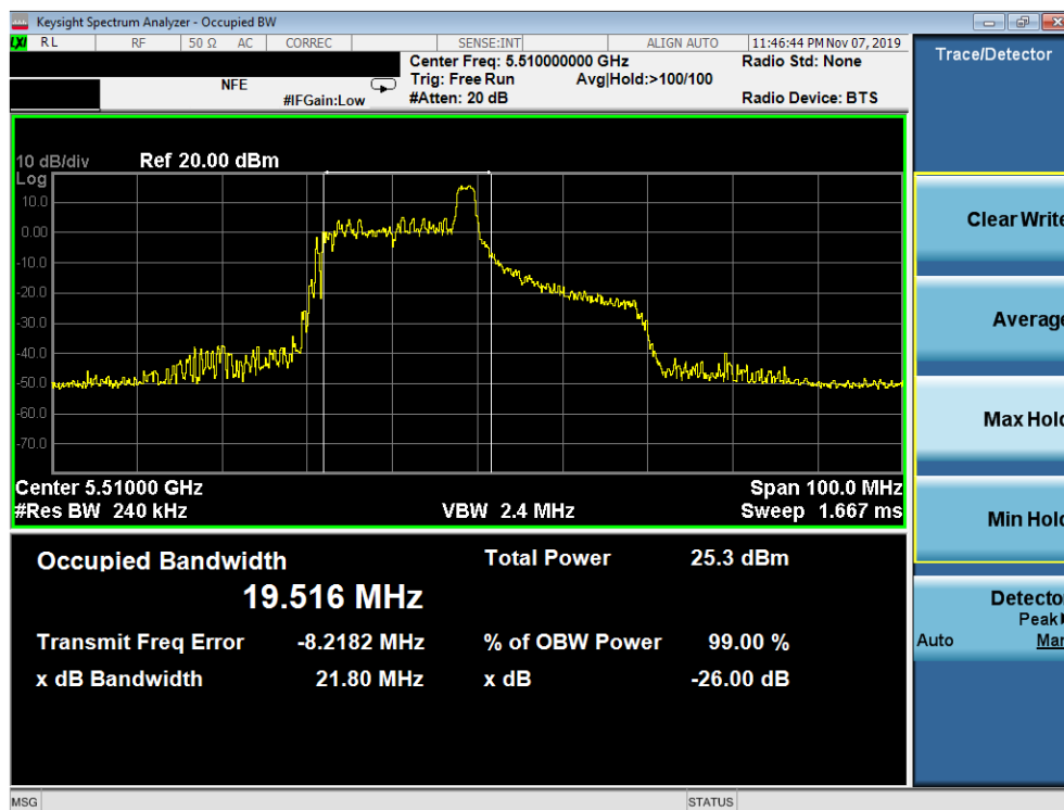
Plot 7-37. 26dB Bandwidth Plot SISO ANT2 (40MHz BW 802.11ax - 26 Tones (UNII Band 2C) - Ch. 102)
