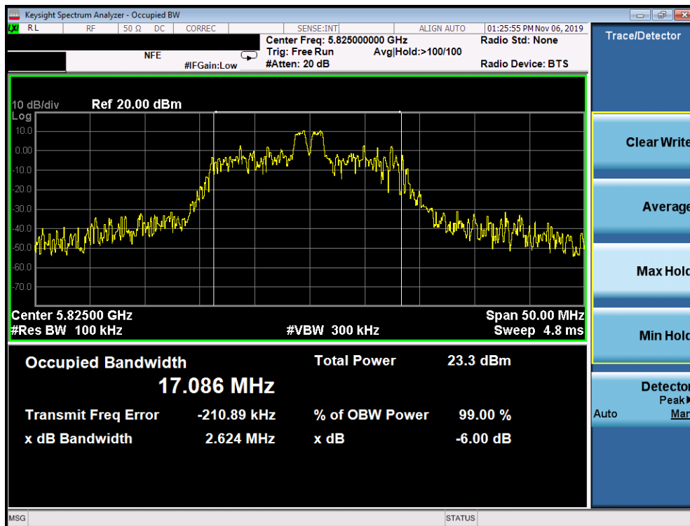
Plot 7-45. 6dB Bandwidth Plot SISO ANT1 (20MHz BW 802.11ax – 26 Tones (UNII Band 3) – Ch. 165)
