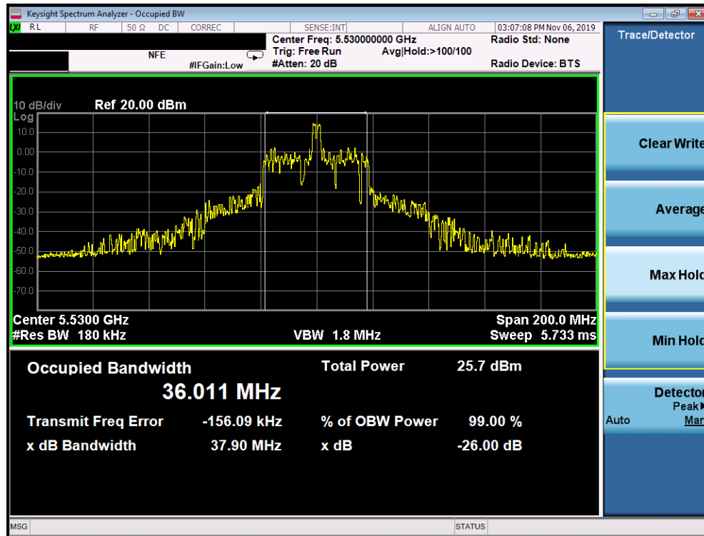
Plot 7-19. 26dB Bandwidth Plot SISO ANT1 (80MHz BW 802.11ax – 26 Tones (UNII Band 2C) – Ch. 106)
