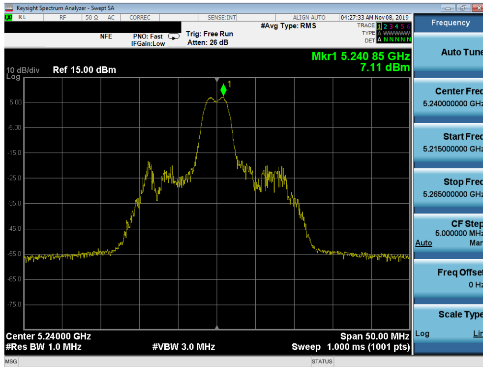
Plot 7-165. Power Spectral Density Plot MIMO ANT1 (20MHz BW 802.11ax – 26 Tones (UNII Band 1) – Ch. 48)
