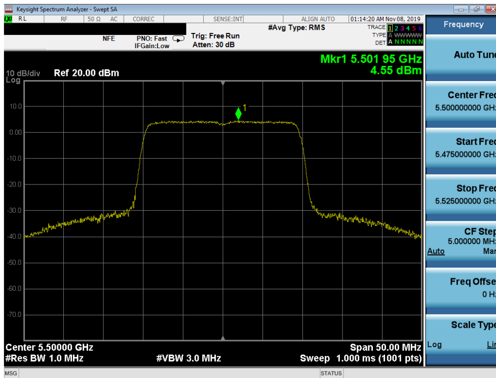
Plot 7-148. Power Spectral Density Plot SISO ANT2 (20MHz BW 802.11ax – Full Tones (UNII Band 2C) – Ch. 100)
