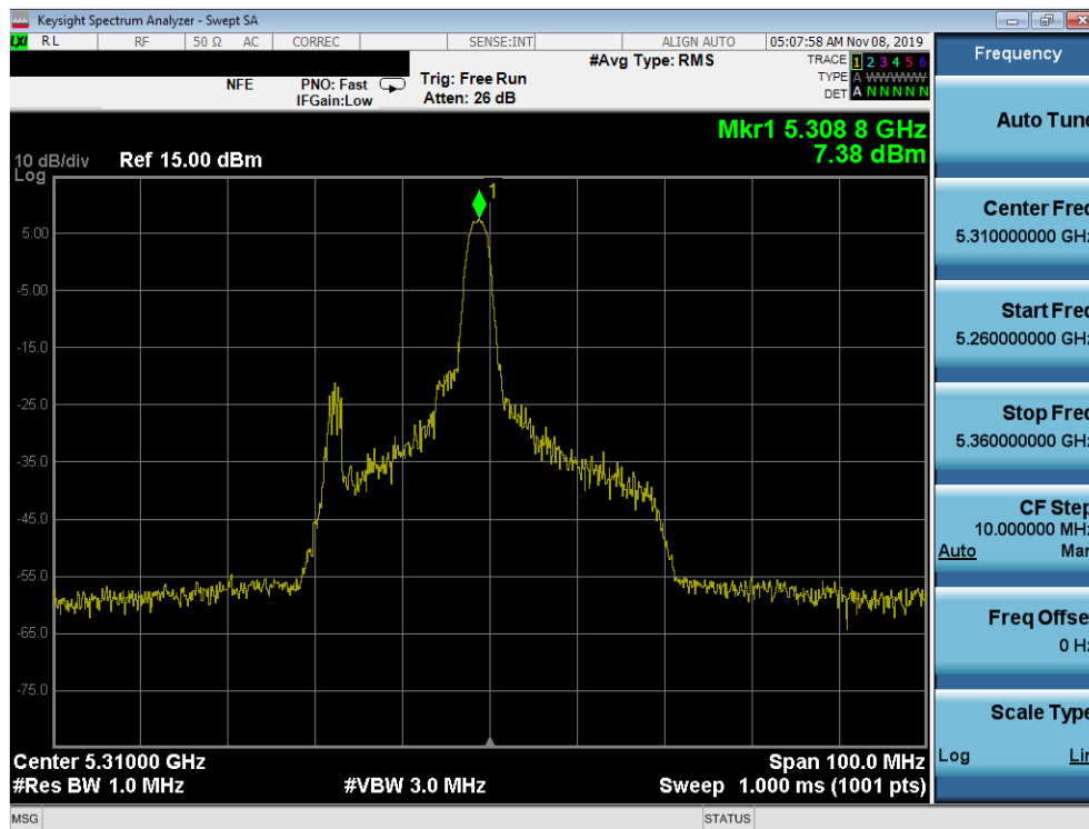
Plot 7-227. Power Spectral Density Plot MIMO ANT2 (40MHz BW 802.11ax – 26 Tones (UNII Band 2A) – Ch. 62)
