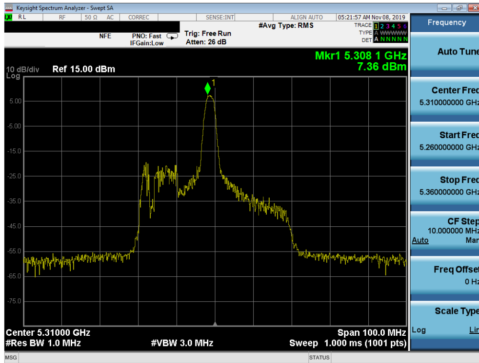
Plot 7-173. Power Spectral Density Plot MIMO ANT1 (40MHz BW 802.11ax – 26 Tones (UNII Band 2A) – Ch. 62)
