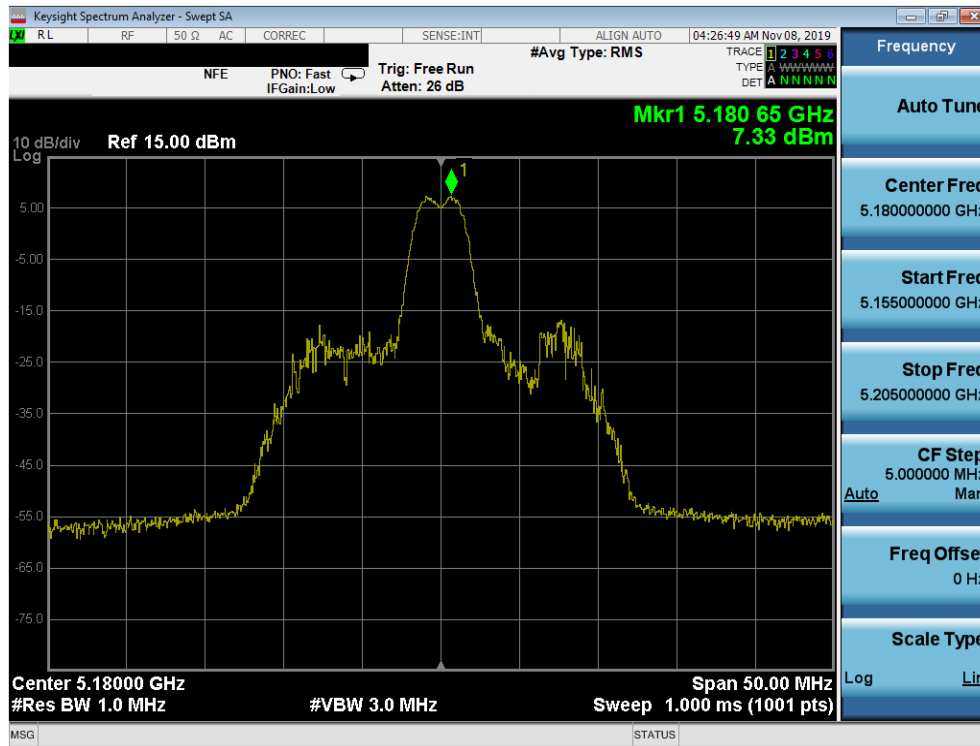
Plot 7-163. Power Spectral Density Plot MIMO ANT1 (20MHz BW 802.11ax – 26 Tones (UNII Band 1) – Ch. 36)
