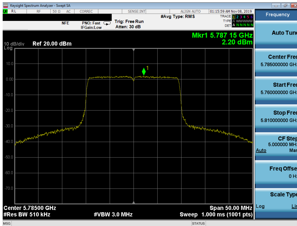
Plot 7-158. Power Spectral Density Plot SISO ANT2 (20MHz BW 802.11ax – Full Tones (UNII Band 3) – Ch. 157)
