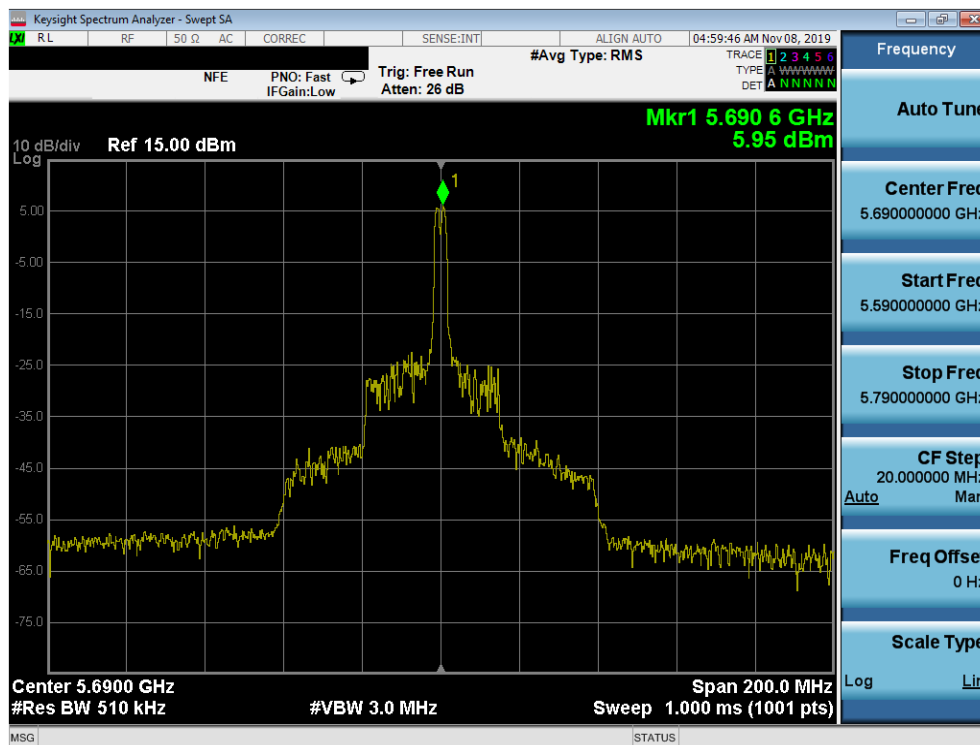
Plot 7-237. Power Spectral Density Plot MIMO ANT2 (80MHz BW 802.11ax – 26 Tones (UNII Band 2C) – Ch. 138)
