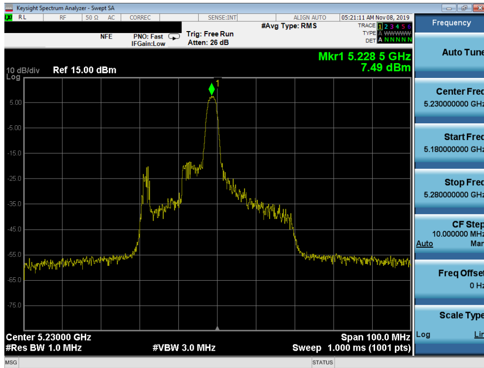
Plot 7-167. Power Spectral Density Plot MIMO ANT1 (40MHz BW 802.11ax – 26 Tones (UNII Band 1) – Ch. 46)
