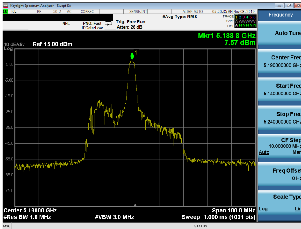
Plot 7-166. Power Spectral Density Plot MIMO ANT1 (40MHz BW 802.11ax – 26 Tones (UNII Band 1) – Ch. 38)
