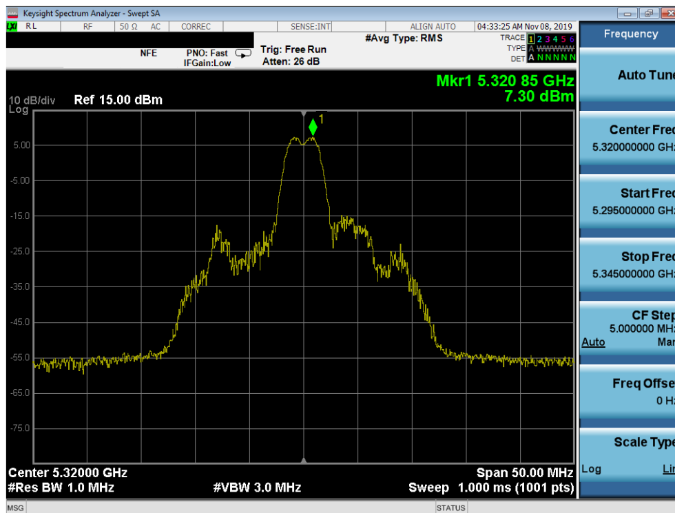
Plot 7-225. Power Spectral Density Plot MIMO ANT2 (20MHz BW 802.11ax – 26 Tones (UNII Band 2A) – Ch. 64)
