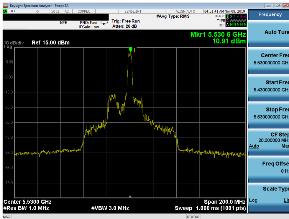
Plot 7-127. Power Spectral Density Plot SISO ANT2 (80MHz BW 802.11ax - 26 Tones (UNII Band 2C) - Ch. 106)
