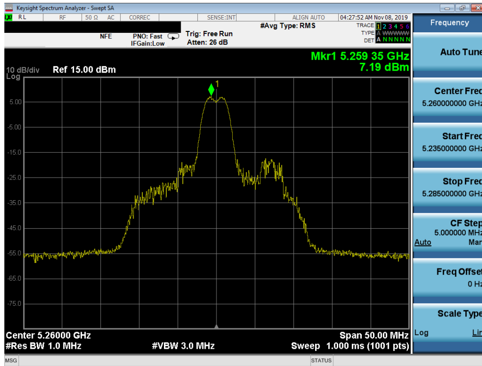
Plot 7-169. Power Spectral Density Plot MIMO ANT1 (20MHz BW 802.11ax – 26 Tones (UNII Band 2A) – Ch. 52)
