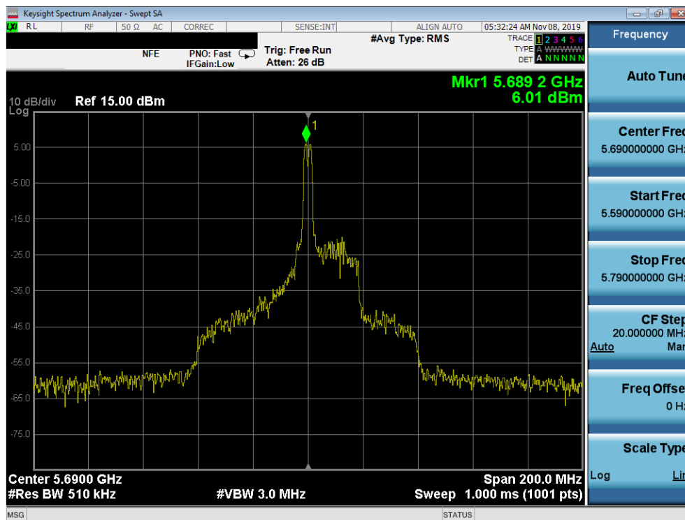
Plot 7-183. Power Spectral Density Plot MIMO ANT1 (80MHz BW 802.11ax – 26 Tones (UNII Band 2C) – Ch. 138)
