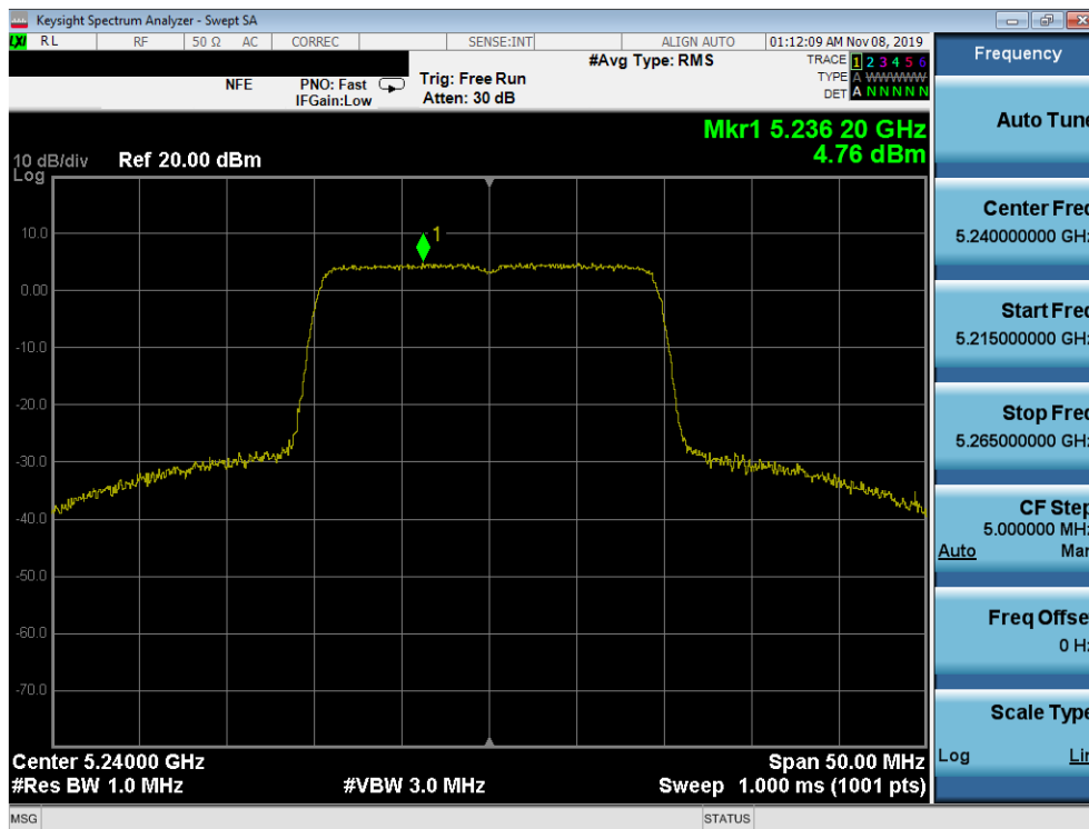
Plot 7-138. Power Spectral Density Plot SISO ANT2 (20MHz BW 802.11ax – Full Tones (UNII Band 1) – Ch. 48)
