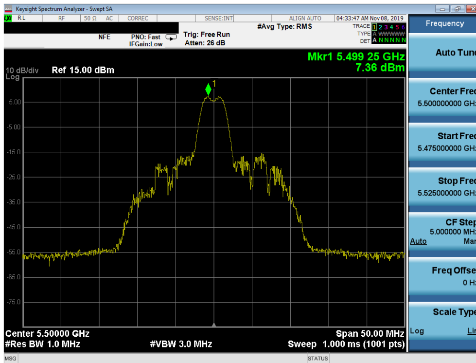
Plot 7-229. Power Spectral Density Plot MIMO ANT2 (20MHz BW 802.11ax – 26 Tones (UNII Band 2C) – Ch. 100)
