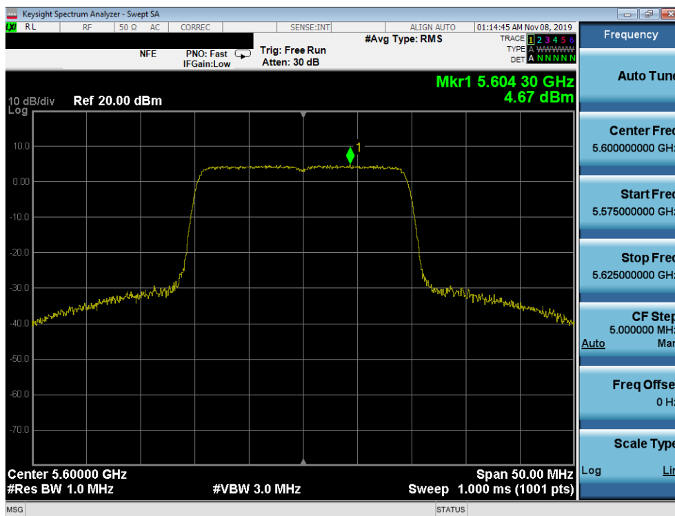
Plot 7-149. Power Spectral Density Plot SISO ANT2 (20MHz BW 802.11ax – Full Tones (UNII Band 2C) – Ch. 120)
