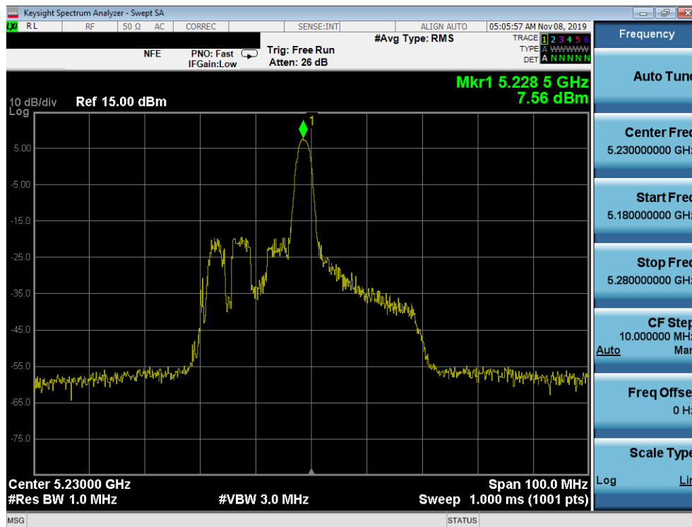
Plot 7-221. Power Spectral Density Plot MIMO ANT2 (40MHz BW 802.11ax – 26 Tones (UNII Band 1) – Ch. 46)
