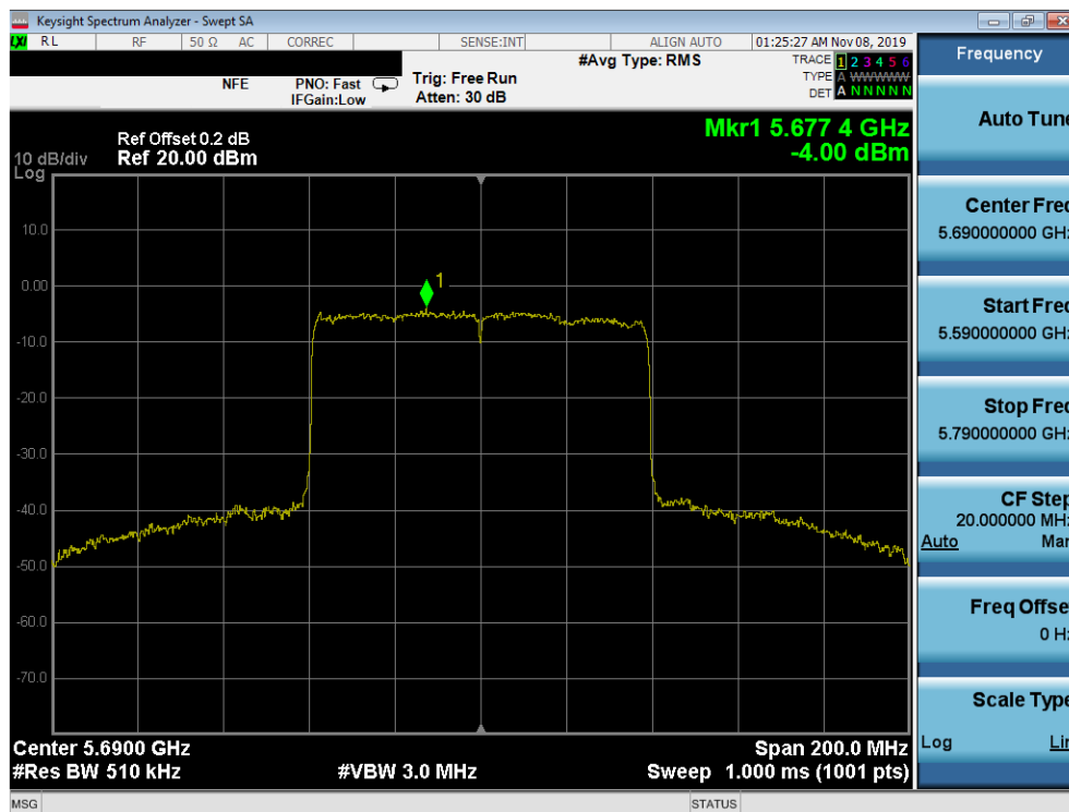
Plot 7-156. Power Spectral Density Plot SISO ANT2 (80MHz BW 802.11ax – Full Tones (UNII Band 2C) – Ch. 138)
