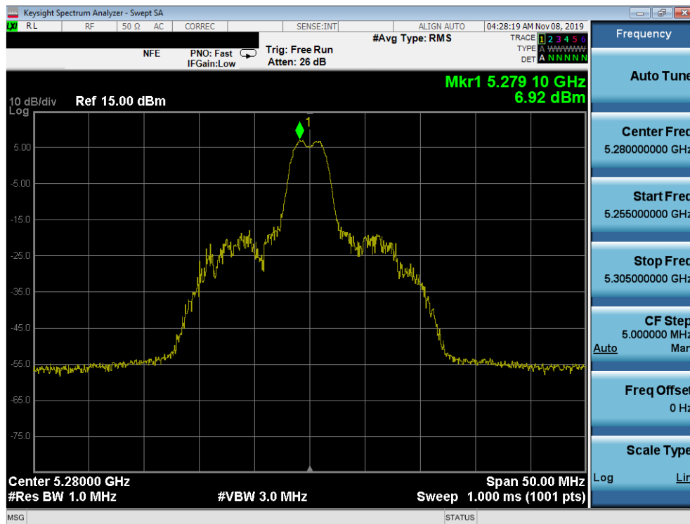
Plot 7-170. Power Spectral Density Plot MIMO ANT1 (20MHz BW 802.11ax – 26 Tones (UNII Band 2A) – Ch. 56)
