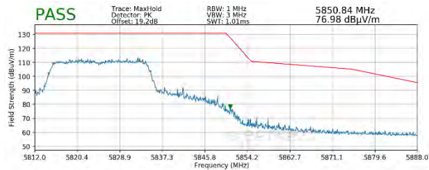
Plot 7-313. Radiated Upper Band Edge Plot SISO ANT1 (Peak – UNII Band 3 – 242 Tones)
