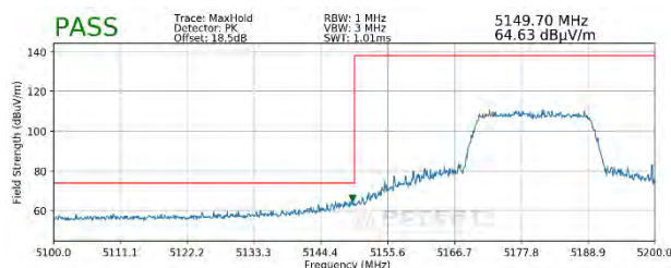
Plot 7-308. Radiated Lower Band Edge Plot SISO ANT1 (Peak - UNII Band 1 - 242 Tones)
