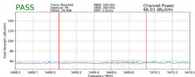
Plot 7-319. Radiated Lower Band Edge Plot SISO ANT1 (Peak - UNII Band 2C - 484 Tones)
