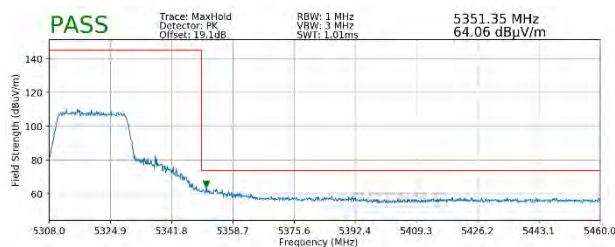
Plot 7-310. Radiated Upper Band Edge Plot SISO ANT1 (Peak - UNII Band 2A - 242 Tones)
