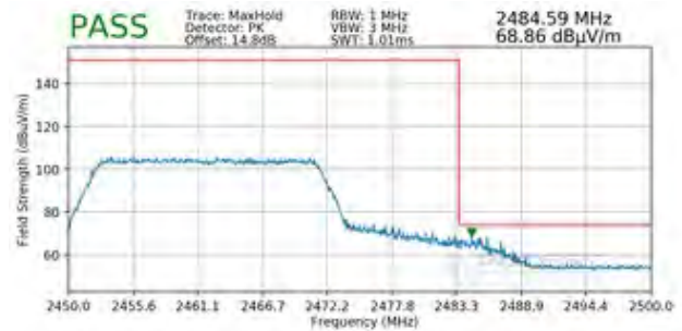
Plot 7-92. Radiated Restricted Upper Band Edge Measurement SISO ANT1 (Peak – 242 Tones)
