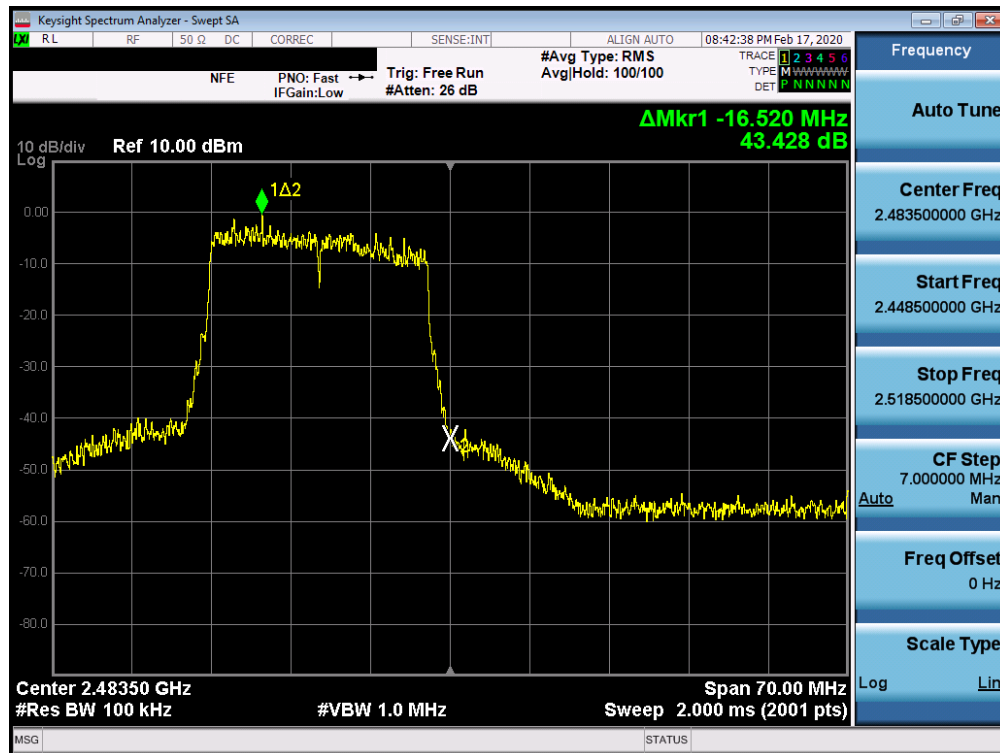
Plot 7-28. Band Edge Plot SISO ANT1 (802.11ax OFDMA - 242 Tones - Ch. 13)
