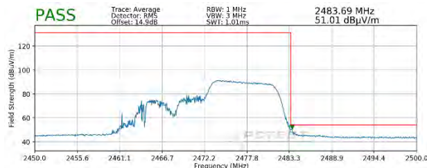
Plot 7-119. Radiated Restricted Upper Band Edge Measurement MIMO (Average – 106 Tones)
