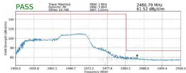
Plot 7-100. Radiated Restricted Upper Band Edge Measurement SISO ANT2 (Peak – 106 Tones)
