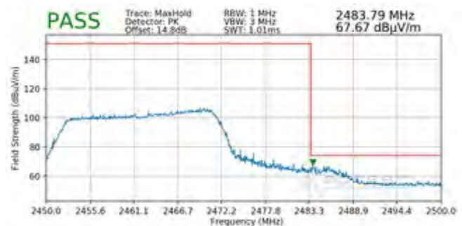
Plot 7-108. Radiated Restricted Upper Band Edge Measurement SISO ANT2 (Peak – 242 Tones)
