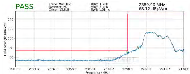
Plot 7-114. Radiated Restricted Lower Band Edge Measurement MIMO (Peak – 106 Tones)
