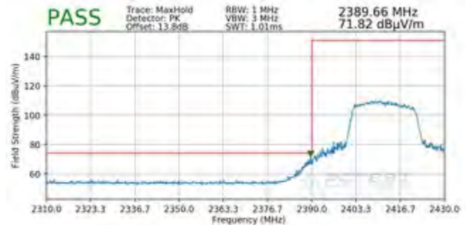
Plot 7-90. Radiated Restricted Lower Band Edge Measurement SISO ANT1 (Peak – 242 Tones)
