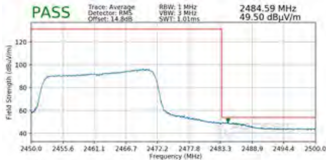
Plot 7-109. Radiated Restricted Upper Band Edge Measurement SISO ANT2 (Average – 242 Tones)
