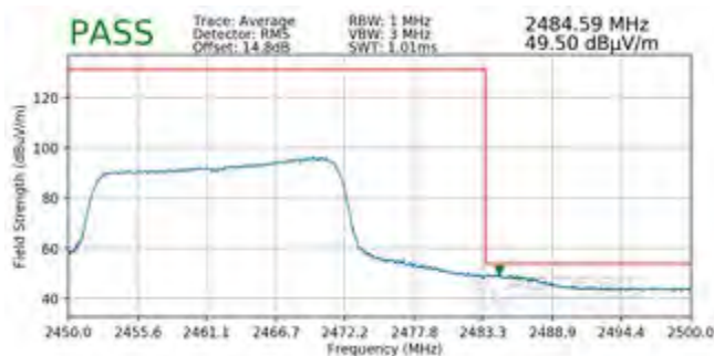
Plot 7-107. Radiated Restricted Upper Band Edge Measurement SISO ANT2 (Average – 242 Tones)
