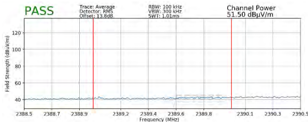
Plot 7-113. Radiated Restricted Lower Band Edge Measurement MIMO (Average – 106 Tones)
