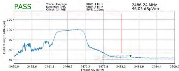
Plot 7-99. Radiated Restricted Upper Band Edge Measurement SISO ANT2 (Average – 106 Tones)
