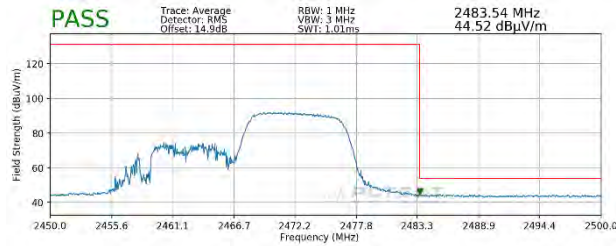
Plot 7-85. Radiated Restricted Upper Band Edge Measurement SISO ANT1 (Average – 106 Tones)
