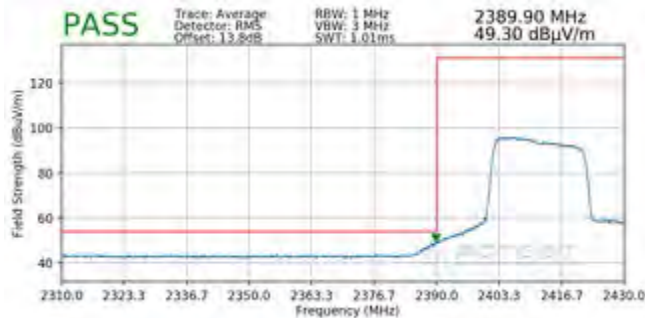
Plot 7-105. Radiated Restricted Lower Band Edge Measurement SISO ANT2 (Average – 242 Tones)
