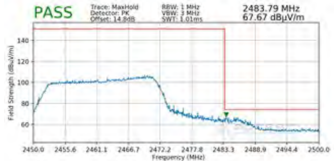
Plot 7-110. Radiated Restricted Upper Band Edge Measurement SISO ANT2 (Peak – 242 Tones)
