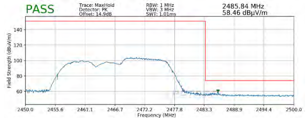
Plot 7-118. Radiated Restricted Upper Band Edge Measurement MIMO (Peak – 106 Tones)
