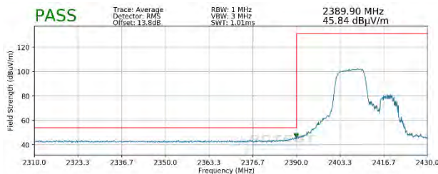
Plot 7-81. Radiated Restricted Lower Band Edge Measurement SISO ANT1 (Average – 106 Tones)
