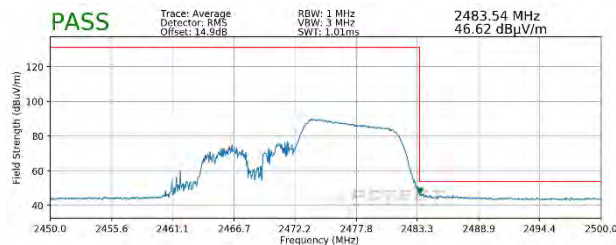
Plot 7-103. Radiated Restricted Upper Band Edge Measurement SISO ANT2 (Average – 106 Tones)
