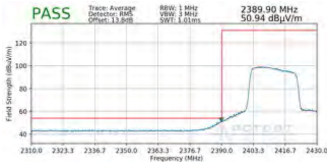
Plot 7-121. Radiated Restricted Lower Band Edge Measurement MIMO (Average – 242 Tones)
