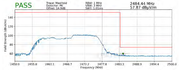
Plot 7-86. Radiated Restricted Upper Band Edge Measurement SISO ANT1 (Peak – 106 Tones)
