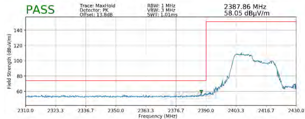
Plot 7-98. Radiated Restricted Lower Band Edge Measurement SISO ANT2 (Peak – 106 Tones)
