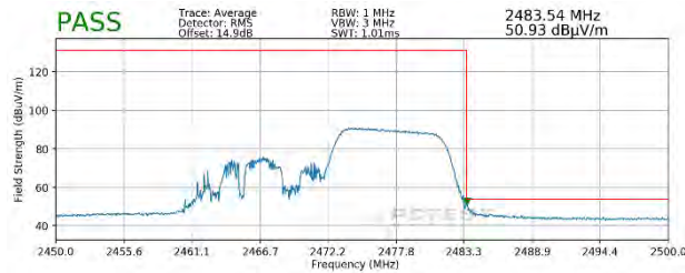
Plot 7-87. Radiated Restricted Upper Band Edge Measurement SISO ANT1 (Average – 106 Tones)
