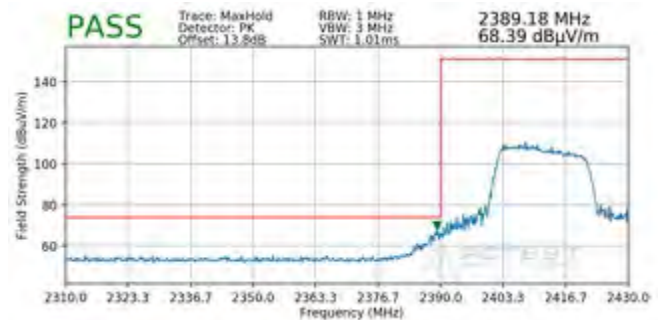
Plot 7-122. Radiated Restricted Lower Band Edge Measurement MIMO (Peak – 242 Tones)
