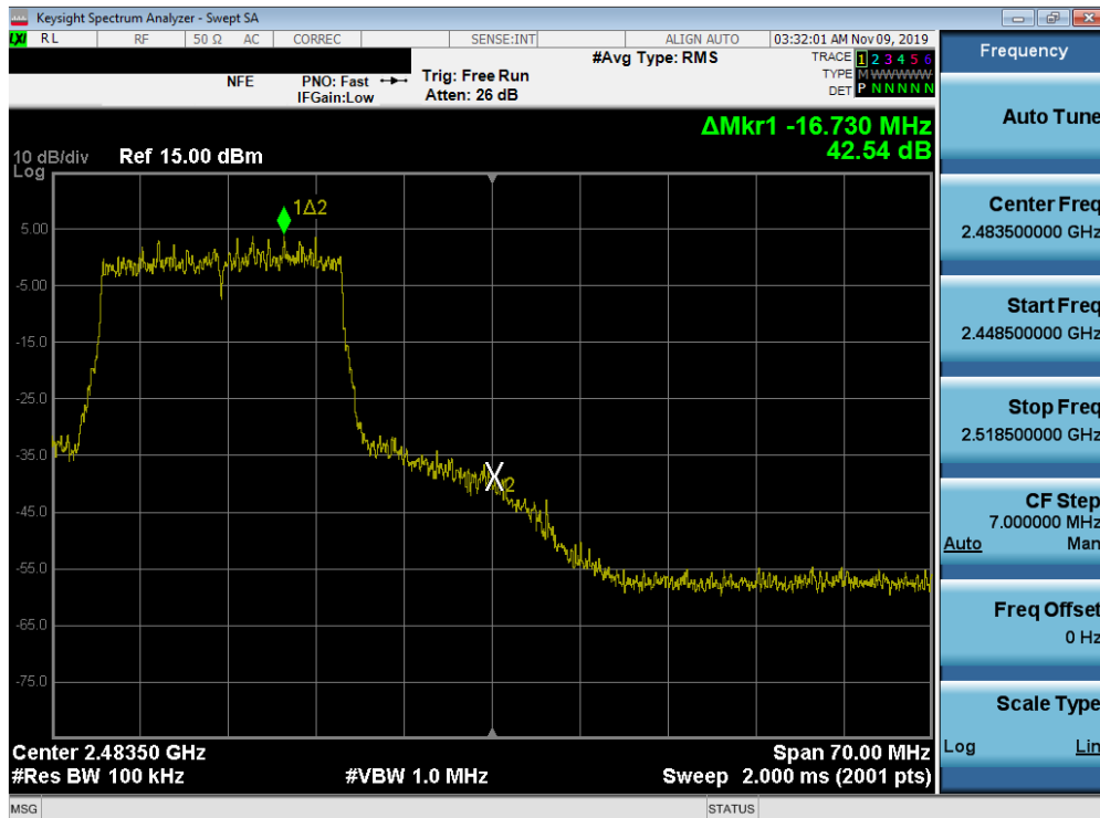
Plot 7-30. Band Edge Plot SISO ANT2 (802.11ax OFDMA – 242 Tones – Ch. 11)
