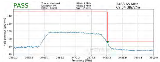
Plot 7-96. Radiated Restricted Upper Band Edge Measurement SISO ANT1 (Peak – 242 Tones)
