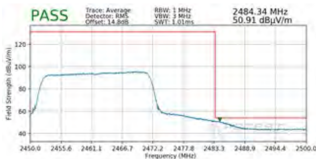
Plot 7-123. Radiated Restricted Upper Band Edge Measurement MIMO (Average – 242 Tones)
