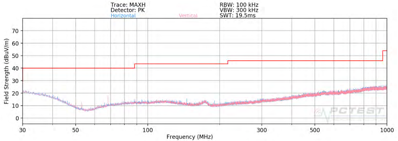
Plot 7-129. Radiated Spurious Plot below 1GHz MIMO (106 Tones)
