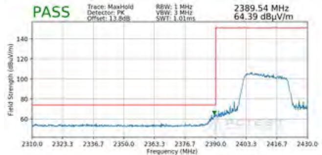
Plot 7-106. Radiated Restricted Lower Band Edge Measurement SISO ANT2 (Peak – 242 Tones)
