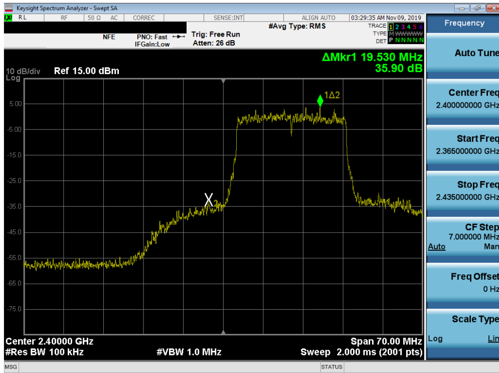
Plot 7-29. Band Edge Plot SISO ANT2 (802.11ax OFDMA – 242 Tones – Ch. 1)
