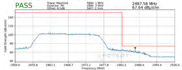
Plot 7-94. Radiated Restricted Upper Band Edge Measurement SISO ANT1 (Peak – 242 Tones)
