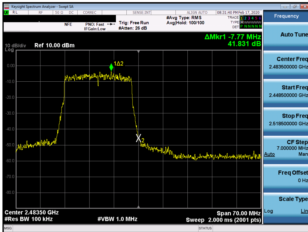
Plot 7-32. Band Edge Plot SISO ANT2 (802.11ax OFDMA – 242 Tones – Ch. 13)
