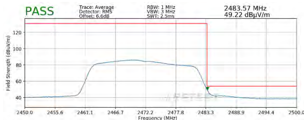
Plot 7-127. Radiated Restricted Upper Band Edge Measurement MIMO (Average – 242 Tones)
