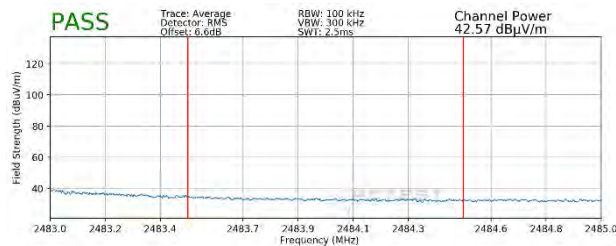
Plot 7-95. Radiated Restricted Upper Band Edge Measurement SISO ANT1 (Average – 242 Tones)
