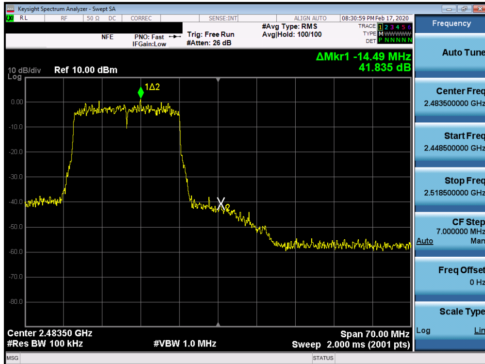
Plot 7-31. Band Edge Plot SISO ANT2 (802.11ax OFDMA – 242 Tones – Ch. 12)
