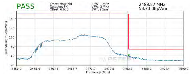
Plot 7-102. Radiated Restricted Upper Band Edge Measurement SISO ANT2 (Peak – 106 Tones)
