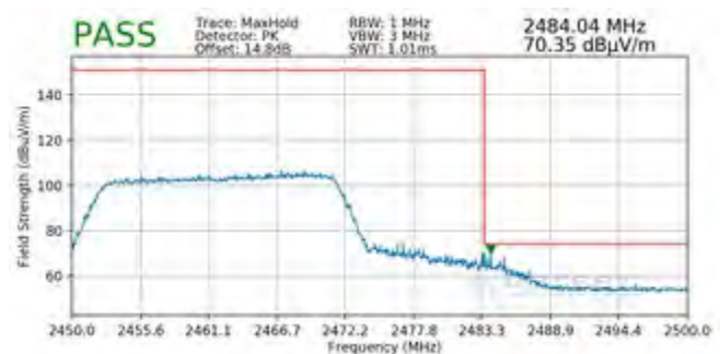
Plot 7-124. Radiated Restricted Upper Band Edge Measurement MIMO (Peak – 242 Tones)
