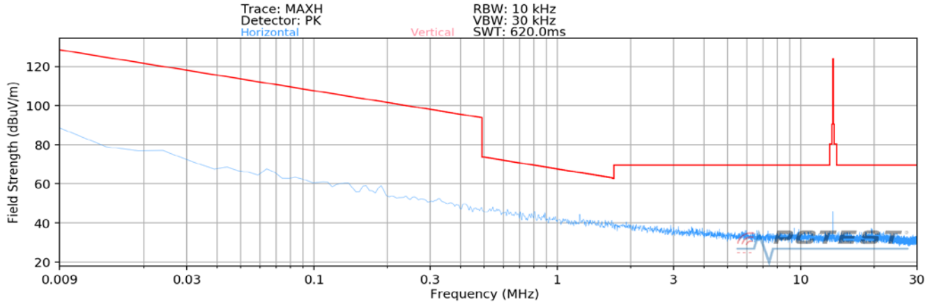
Plot 7-1. Radiated Spurious Plot 9kHz – 30MHz (Pol. X)
