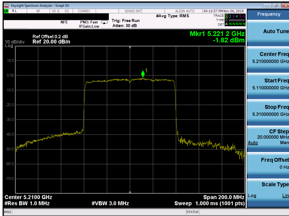
Plot 7-147. Power Spectral Density Plot SISO ANT1 (80MHz BW 802.11aax (UNII Band 1) – Ch. 42)
