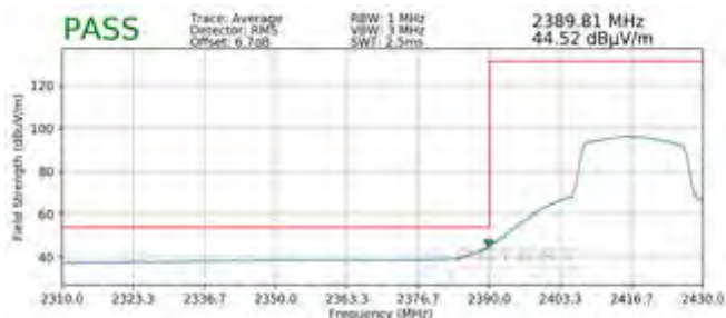
Plot 7-113. Radiated Restricted Lower Band Edge Measurement SISO ANT2 (Average)
