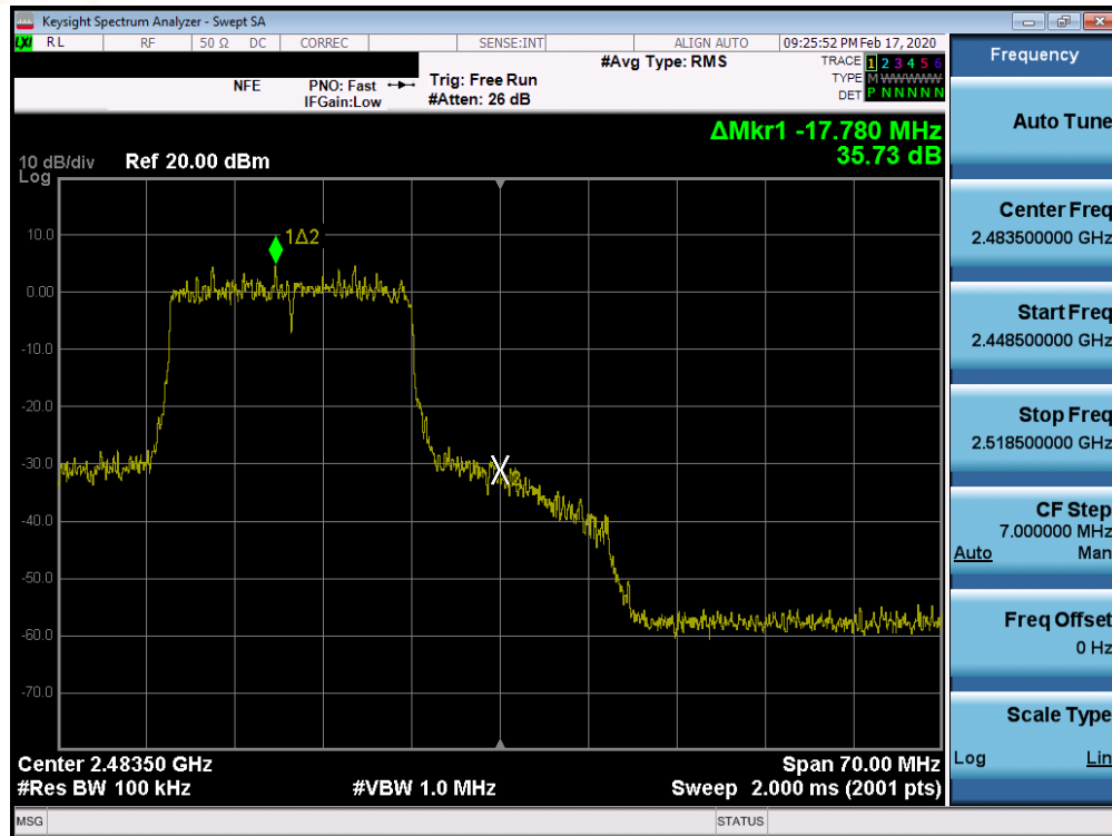
Plot 7-73. Band Edge Plot SISO ANT2 (802.11ax - Ch. 12)
