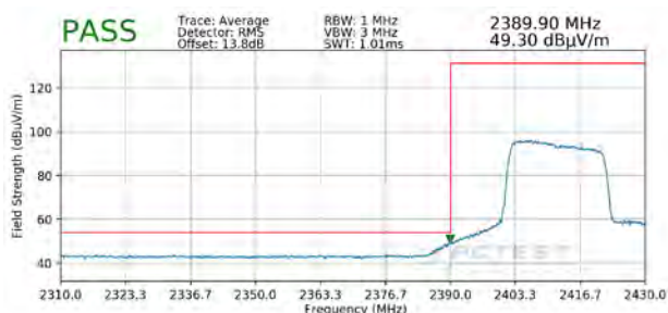
Plot 7-111. Radiated Restricted Lower Band Edge Measurement SISO ANT2 (Average)
