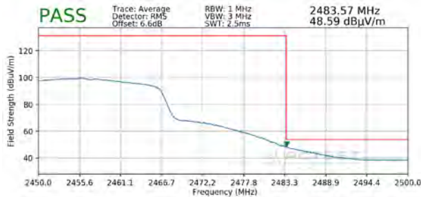
Plot 7-103. Radiated Restricted Upper Band Edge Measurement SISO ANT1 (Average)
