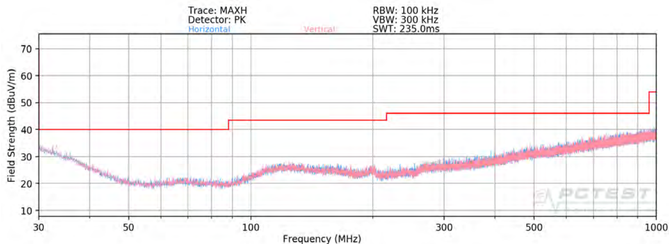
Plot 7-136. Radiated Spurious Plot below 1GHz SISO ANT2
