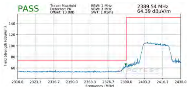
Plot 7-112. Radiated Restricted Lower Band Edge Measurement SISO ANT2 (Peak)
