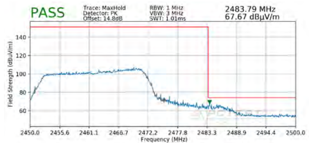
Plot 7-118. Radiated Restricted Upper Band Edge Measurement SISO ANT2 (Peak)
