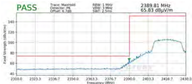
Plot 7-114. Radiated Restricted Lower Band Edge Measurement SISO ANT2 (Peak)
