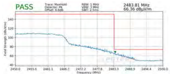
Plot 7-128. Radiated Restricted Upper Band Edge Measurement MIMO (Peak)
