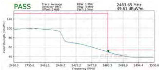
Plot 7-127. Radiated Restricted Upper Band Edge Measurement MIMO (Average)
