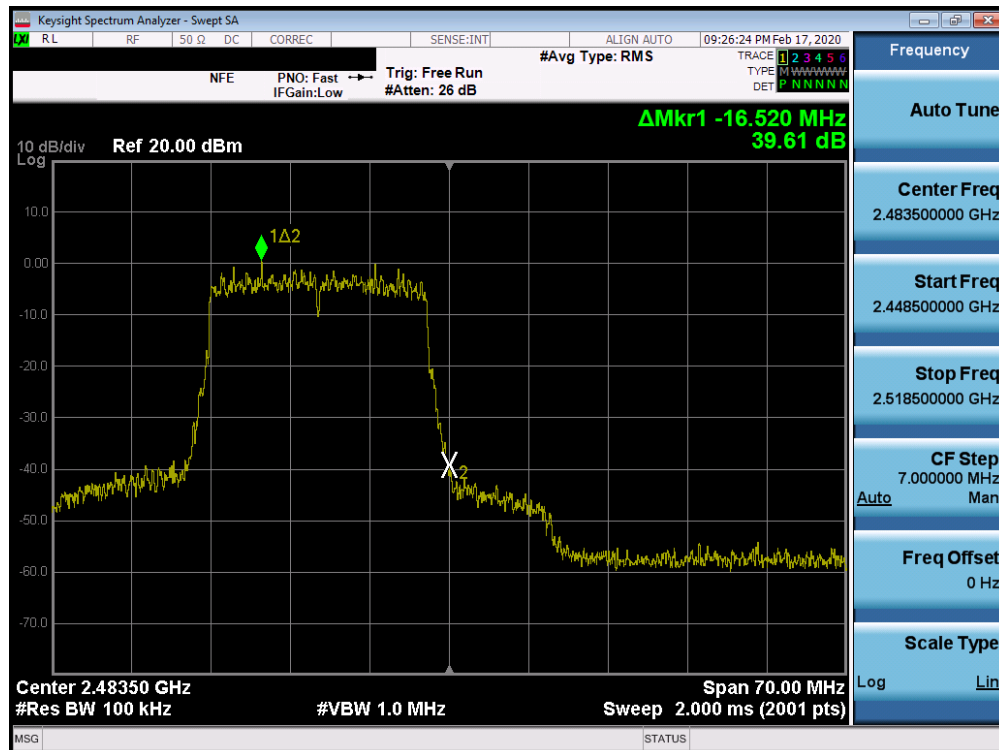
Plot 7-74. Band Edge Plot SISO ANT2 (802.11ax - Ch. 13)
