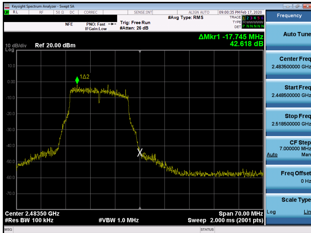
Plot 7-50. Band Edge Plot SISO ANT1 (802.11g - Ch. 13)
