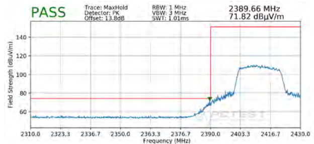
Plot 7-100. Radiated Restricted Lower Band Edge Measurement SISO ANT1 (Peak)
