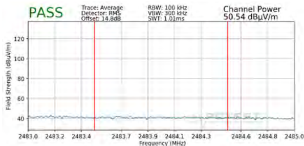
Plot 7-105. Radiated Restricted Upper Band Edge Measurement SISO ANT1 (Average)
