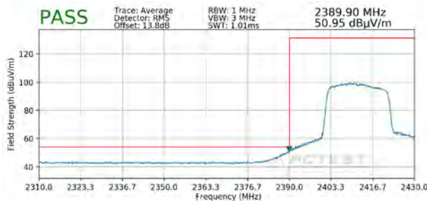
Plot 7-99. Radiated Restricted Lower Band Edge Measurement SISO ANT1 (Average)
