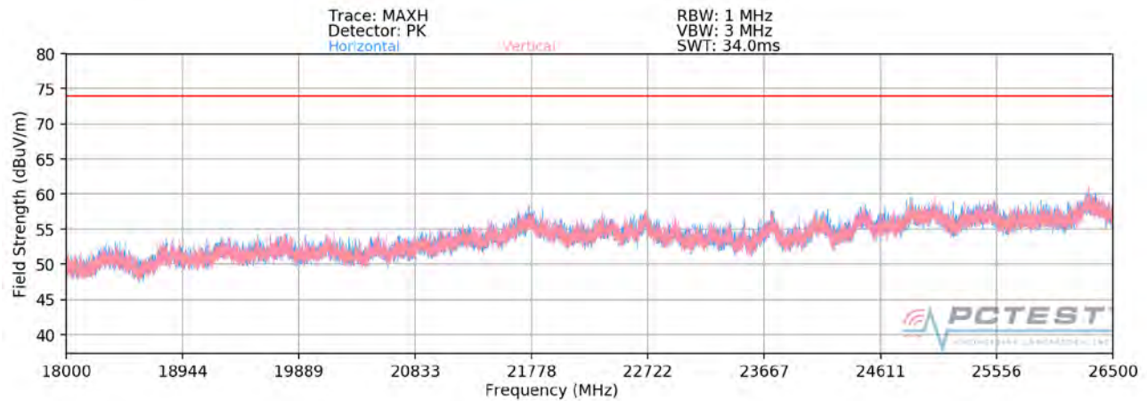
Plot 7-98. Radiated Spurious Plot above 18GHz MIMO/CDD
