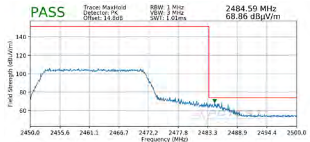
Plot 7-106. Radiated Restricted Upper Band Edge Measurement SISO ANT1 (Peak)
