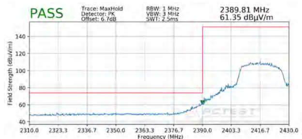
Plot 7-102. Radiated Restricted Lower Band Edge Measurement SISO ANT1 (Peak)
