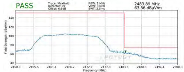
Plot 7-132. Radiated Restricted Upper Band Edge Measurement MIMO (Peak)
