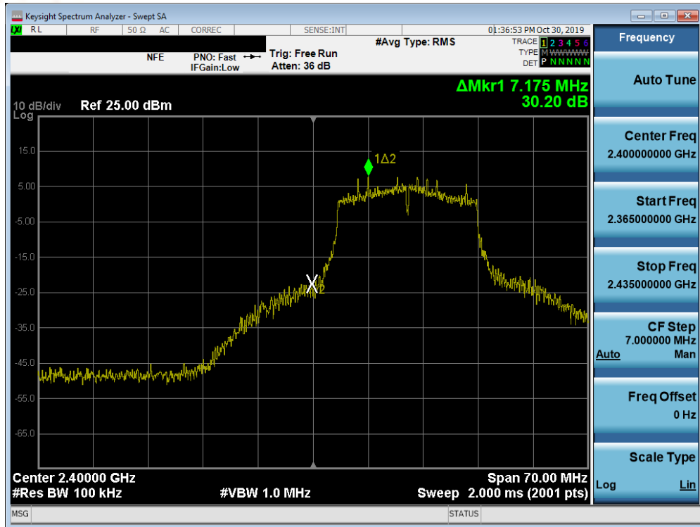
Plot 7-67. Band Edge Plot SISO ANT2 (802.11n (2.4GHz) – Ch. 1)
