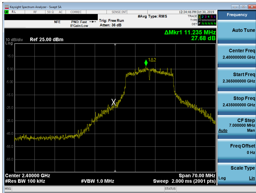
Plot 7-47. Band Edge Plot SISO ANT1 (802.11g- Ch. 1)
