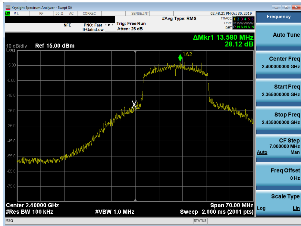
Plot 7-55. Band Edge Plot SISO ANT1 (802.11ax (2.4GHz) – Ch. 1)
