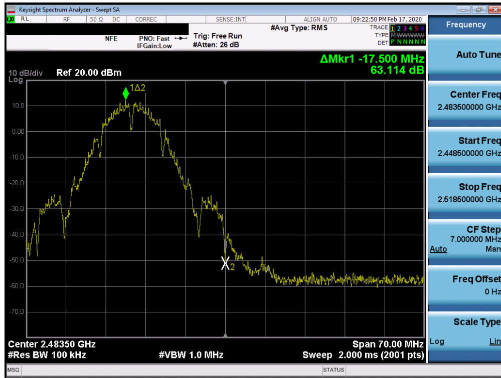
Plot 7-61. Band Edge Plot SISO ANT2 (802.11b - Ch. 12)
