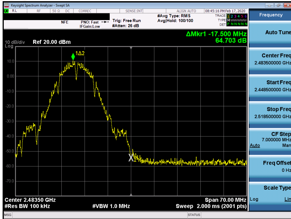
Plot 7-45. Band Edge Plot SISO ANT1 (802.11b - Ch. 12)
