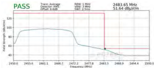
Plot 7-129. Radiated Restricted Upper Band Edge Measurement MIMO (Average)
