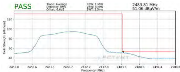
Plot 7-119. Radiated Restricted Upper Band Edge Measurement SISO ANT2 (Average)
