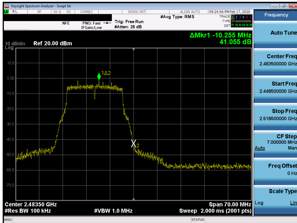
Plot 7-66. Band Edge Plot SISO ANT2 (802.11g - Ch. 13)
