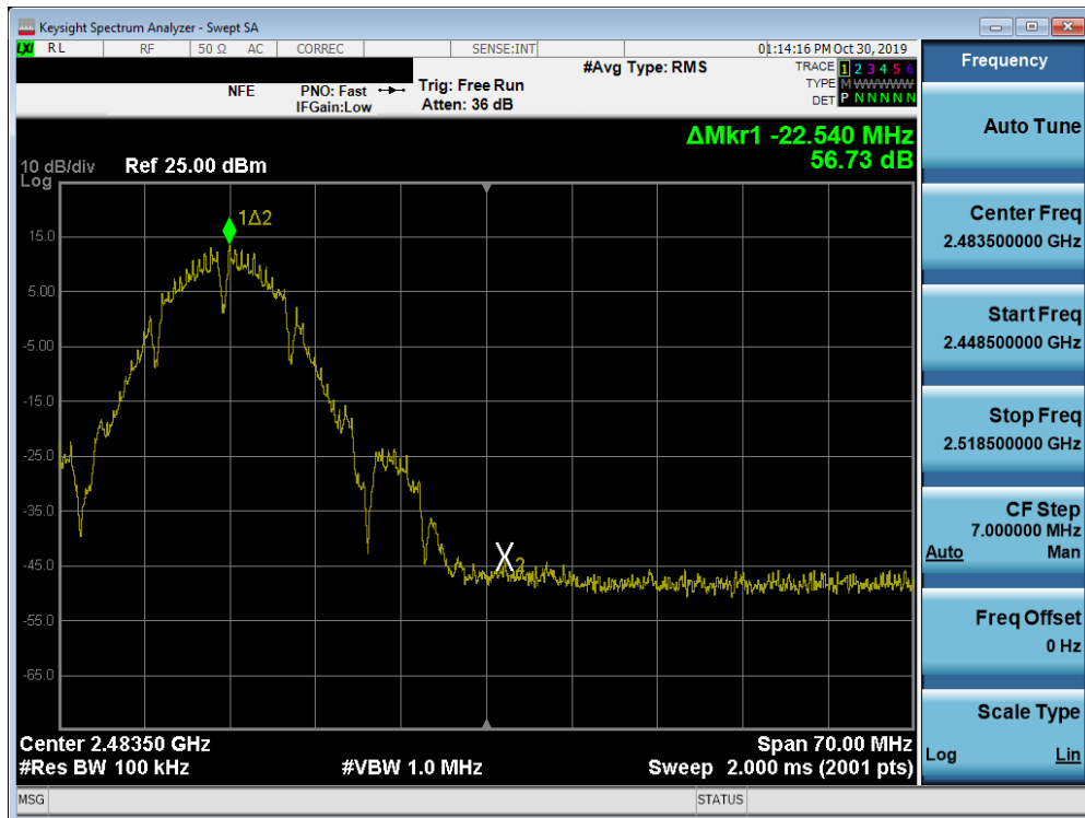
Plot 7-60. Band Edge Plot SISO ANT2 (802.11b - Ch. 11)
