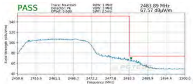
Plot 7-130. Radiated Restricted Upper Band Edge Measurement MIMO (Peak)
