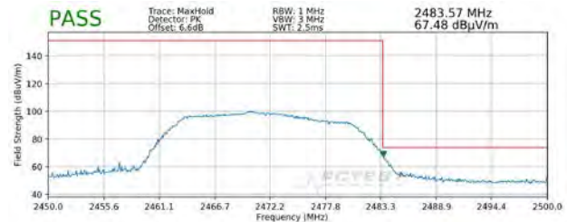
Plot 7-134. Radiated Restricted Upper Band Edge Measurement MIMO (Peak)
