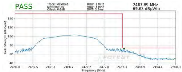
Plot 7-120. Radiated Restricted Upper Band Edge Measurement SISO ANT2 (Peak)
