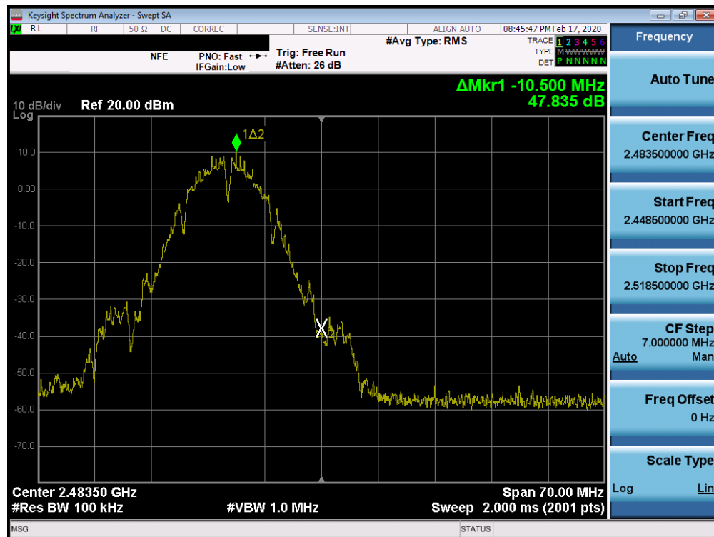
Plot 7-46. Band Edge Plot SISO ANT1 (802.11b - Ch. 13)
