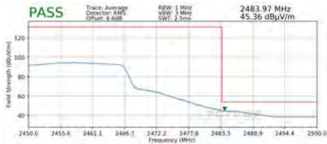
Plot 7-115. Radiated Restricted Upper Band Edge Measurement SISO ANT2 (Average)
