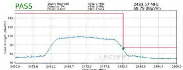
Plot 7-122. Radiated Restricted Upper Band Edge Measurement SISO ANT2 (Peak)
