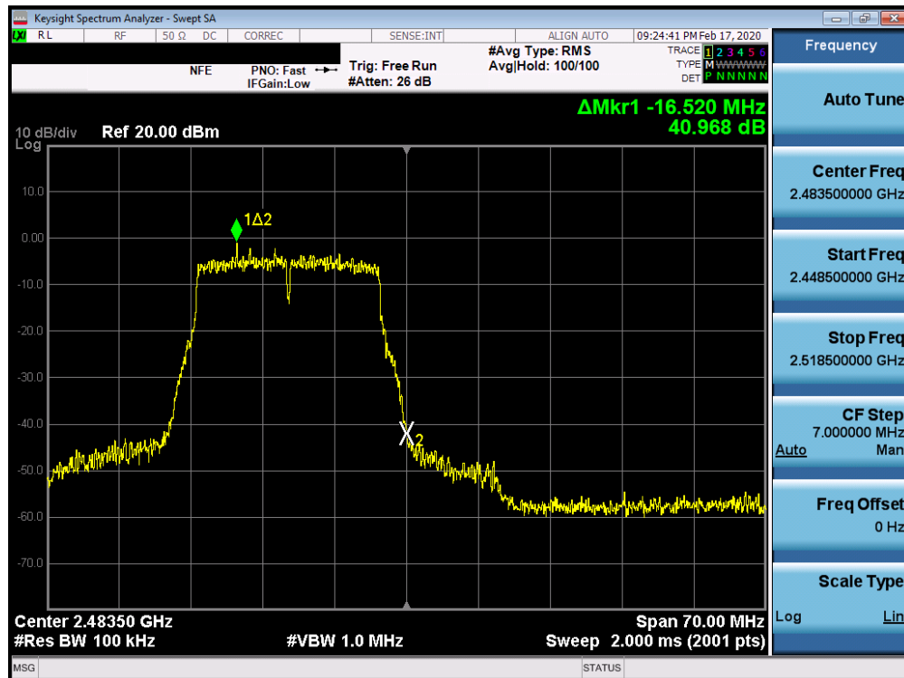
Plot 7-70. Band Edge Plot SISO ANT2 (802.11n – Ch. 13)
