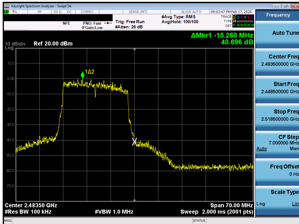
Plot 7-58. Band Edge Plot SISO ANT1 (802.11ax - Ch. 13)
