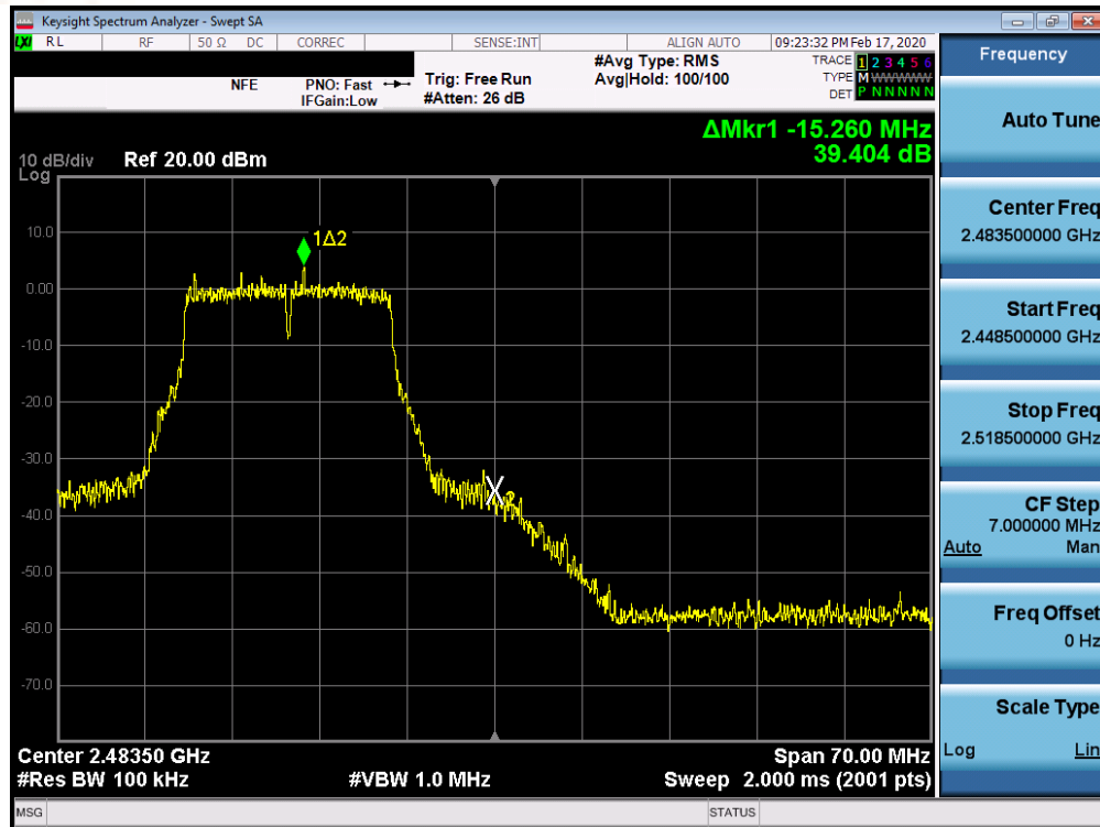
Plot 7-65. Band Edge Plot SISO ANT2 (802.11g - Ch. 12)
