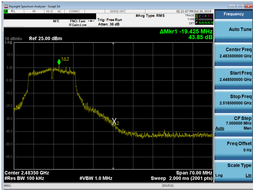
Plot 7-64. Band Edge Plot SISO ANT2 (802.11g - Ch. 11)
