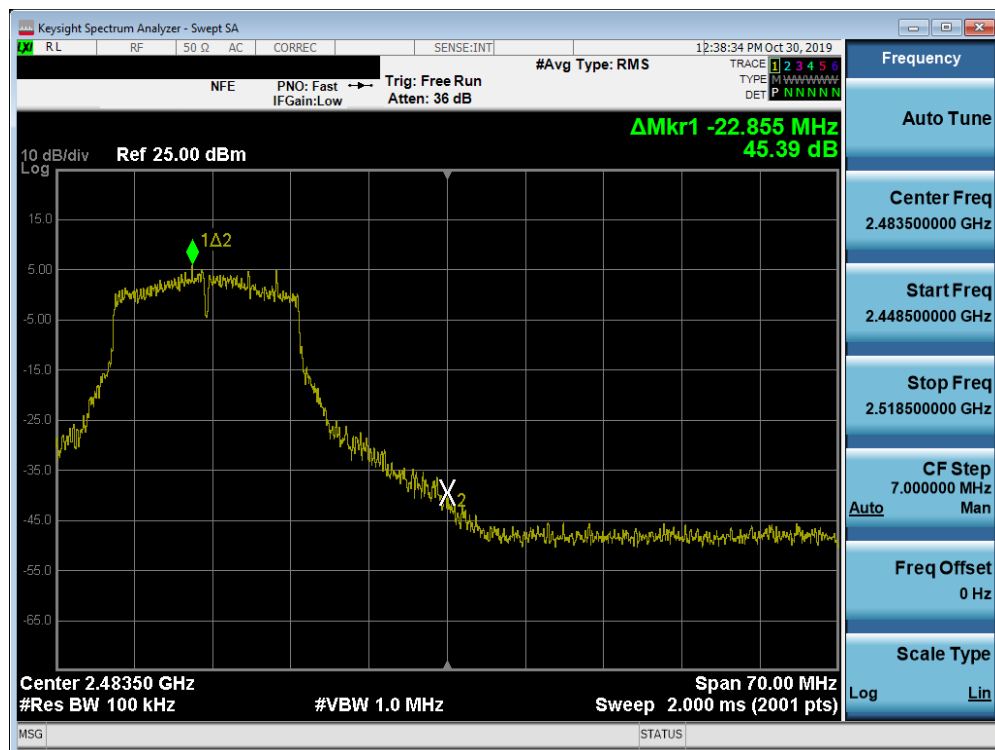
Plot 7-48. Band Edge Plot SISO ANT1 (802.11g – Ch. 11)
