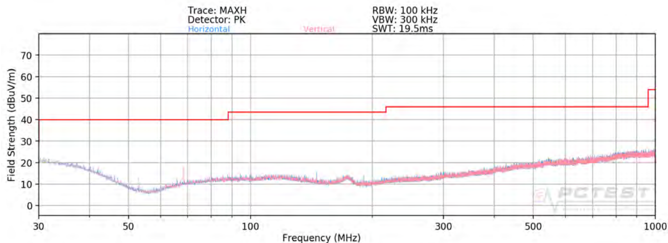
Plot 7-135. Radiated Spurious Plot below 1GHz SISO ANT1
