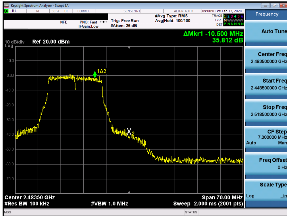
Plot 7-49. Band Edge Plot SISO ANT1 (802.11g - Ch. 12)
