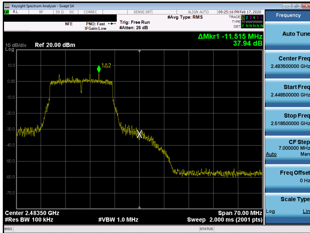
Plot 7-69. Band Edge Plot SISO ANT2 (802.11n – Ch. 12)
