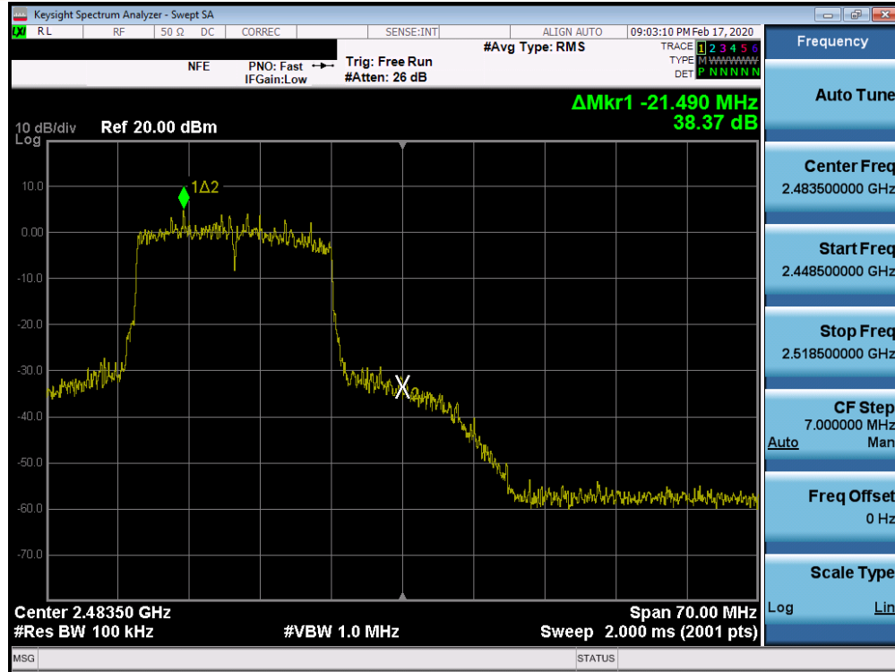
Plot 7-57. Band Edge Plot SISO ANT1 (802.11ax - Ch. 12)
