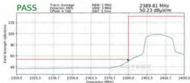
Plot 7-123. Radiated Restricted Lower Band Edge Measurement MIMO (Average)
