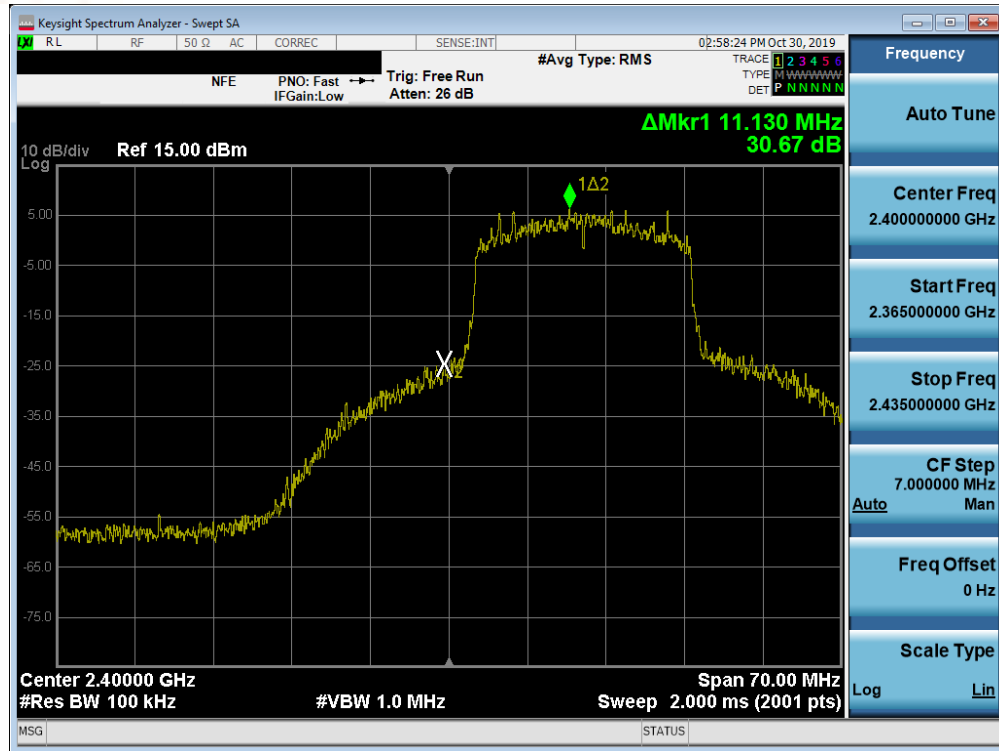
Plot 7-71. Band Edge Plot SISO ANT2 (802.11ax (2.4GHz) – Ch. 1)
