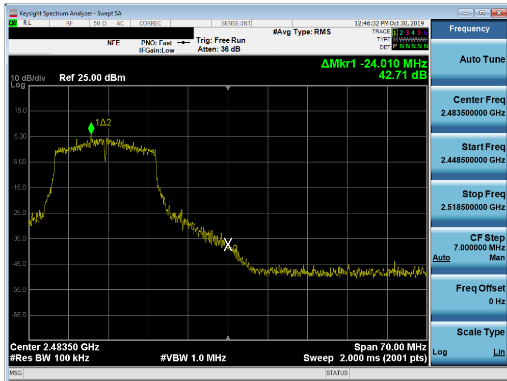
Plot 7-52. Band Edge Plot SISO ANT1 (802.11n (2.4GHz) – Ch. 11)
