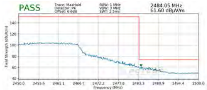
Plot 7-116. Radiated Restricted Upper Band Edge Measurement SISO ANT2 (Peak)
