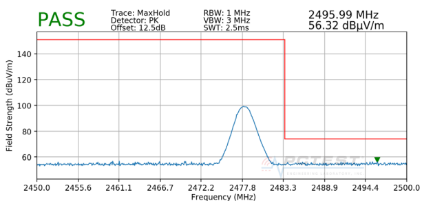
Plot 7-5. Radiated Restricted Upper Band Edge Measurement (Peak)
