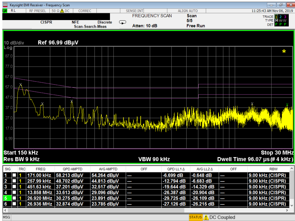
Plot 7-54. Line Conducted Plot with Bluetooth LE (L1)
