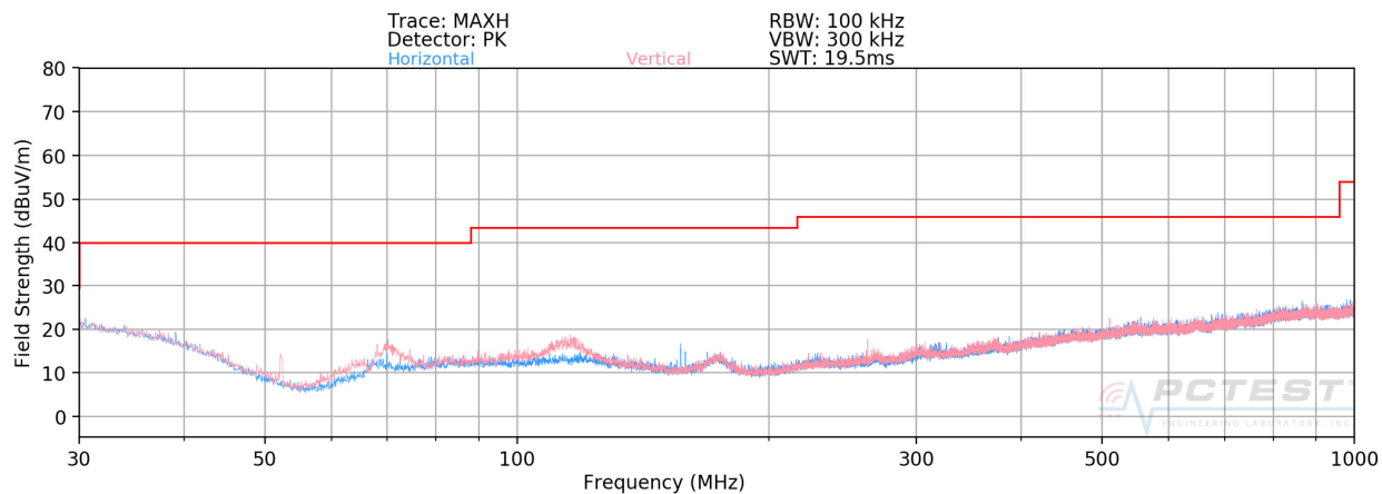
Plot 7-53. Radiated Spurious Plot below 1GHz
