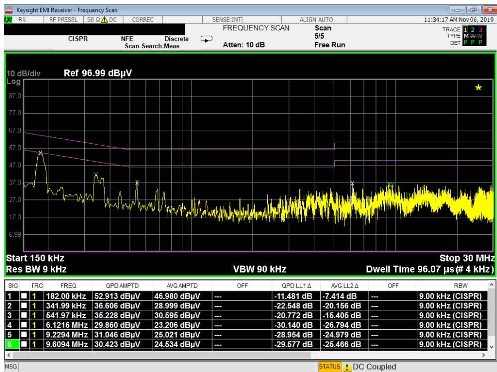
Plot 7-55. Line Conducted Plot with Bluetooth LE (N)
