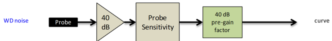
Figure 5-2 Audio Band Magnetic Curve Measurement Block Diagram
