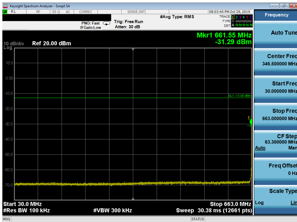
Plot 7-168. Conducted Spurious Plot (Band 71 - 20.0MHz QPSK - RB Size 1, RB Offset 0 - Mid Channel)
