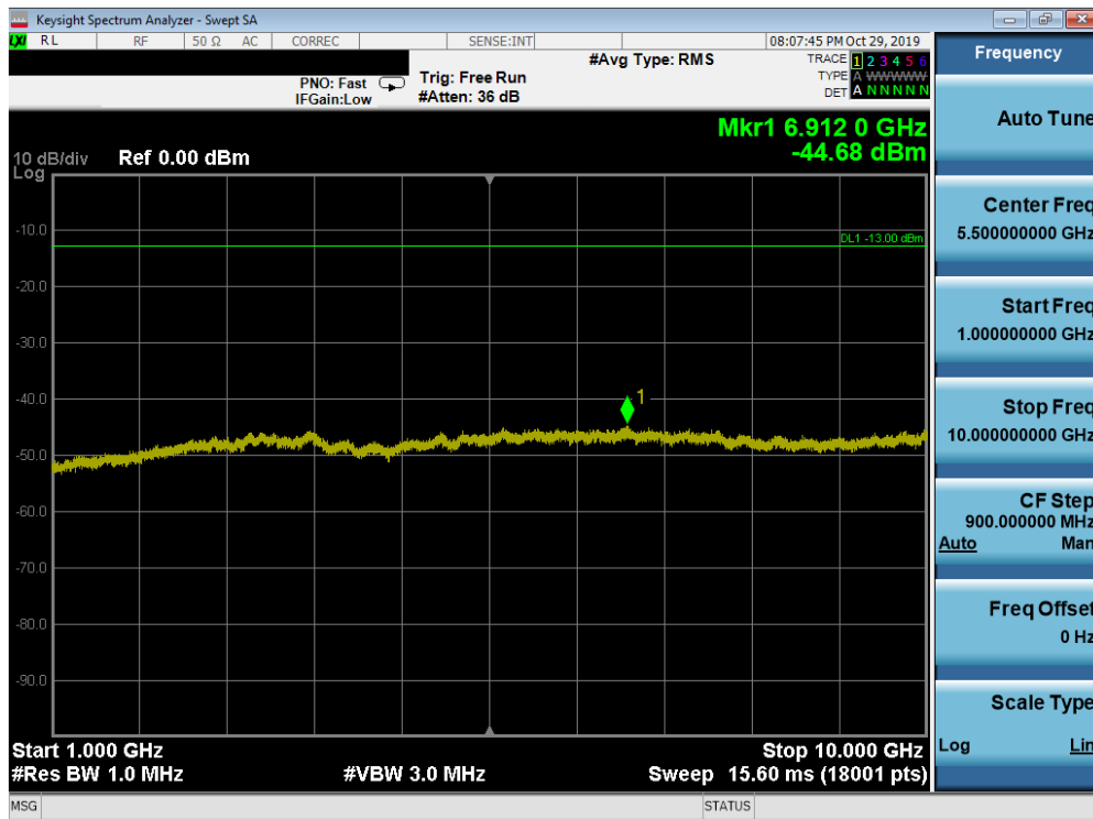
Plot 7-167. Conducted Spurious Plot (Band 71 - 20.0MHz QPSK - RB Size 1, RB Offset 0 - Low Channel)
