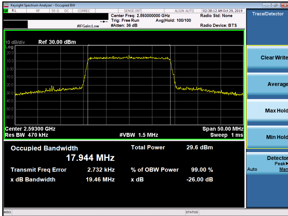
Plot 7-163. Occupied Bandwidth Plot (Band 41 (PC3) - 20.0MHz 64-QAM - Full RB Configuration)
