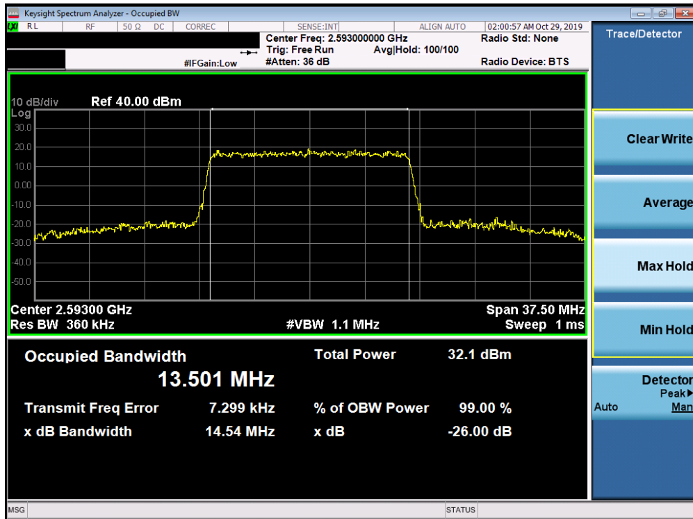
Plot 7-143. Occupied Bandwidth Plot (Band 41 (PC2) - 15.0MHz 64-QAM - Full RB Configuration)
