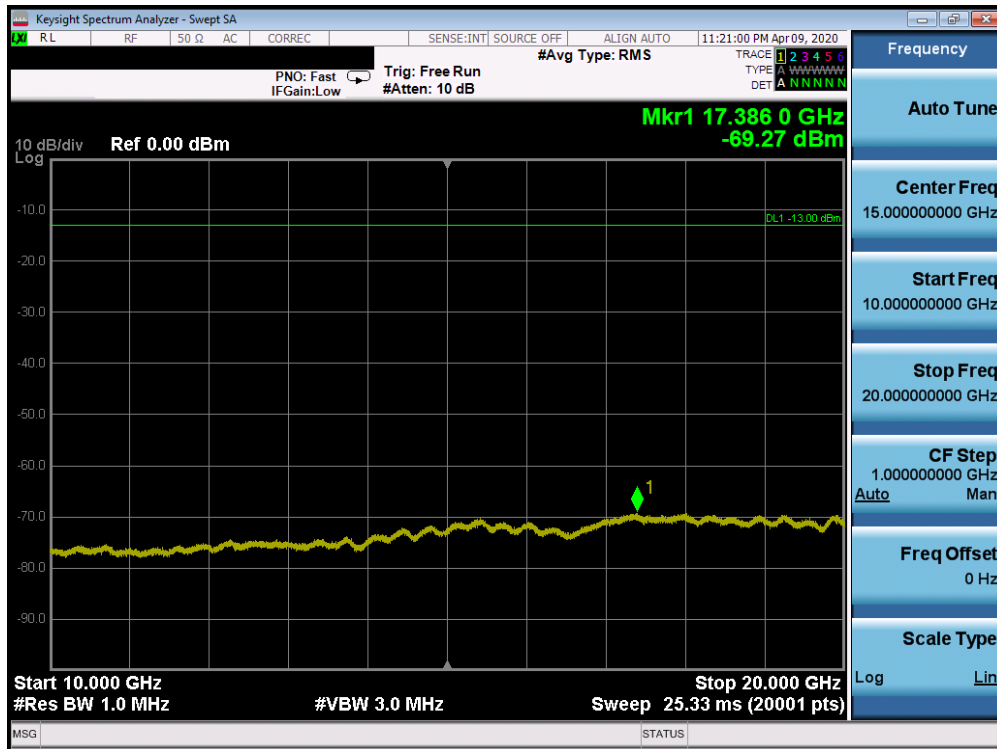
Plot 7-53. Conducted Spurious Plot (n2 - 20.0MHz DFT-s OFDM \pi/2 BPSK - RB Size 1, RB Offset 1 - Low Channel)
