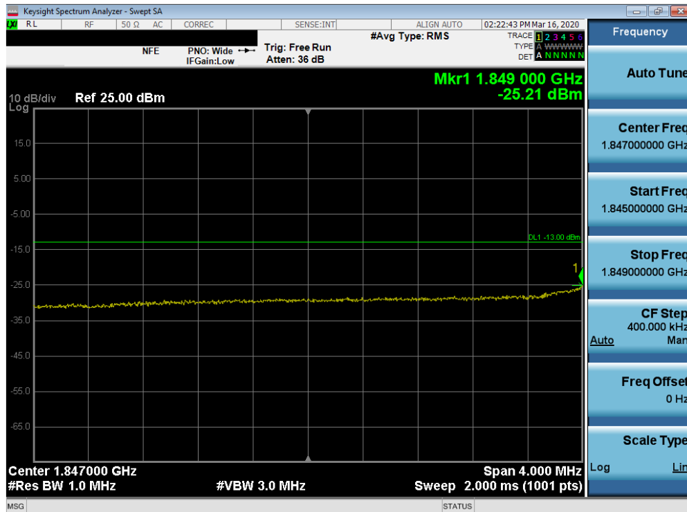
Plot 7-78. Lower Extended Band Edge Plot (n2 - 20.0MHz DFT-s OFDM \pi/2 BPSK - Full RB Configuration)
