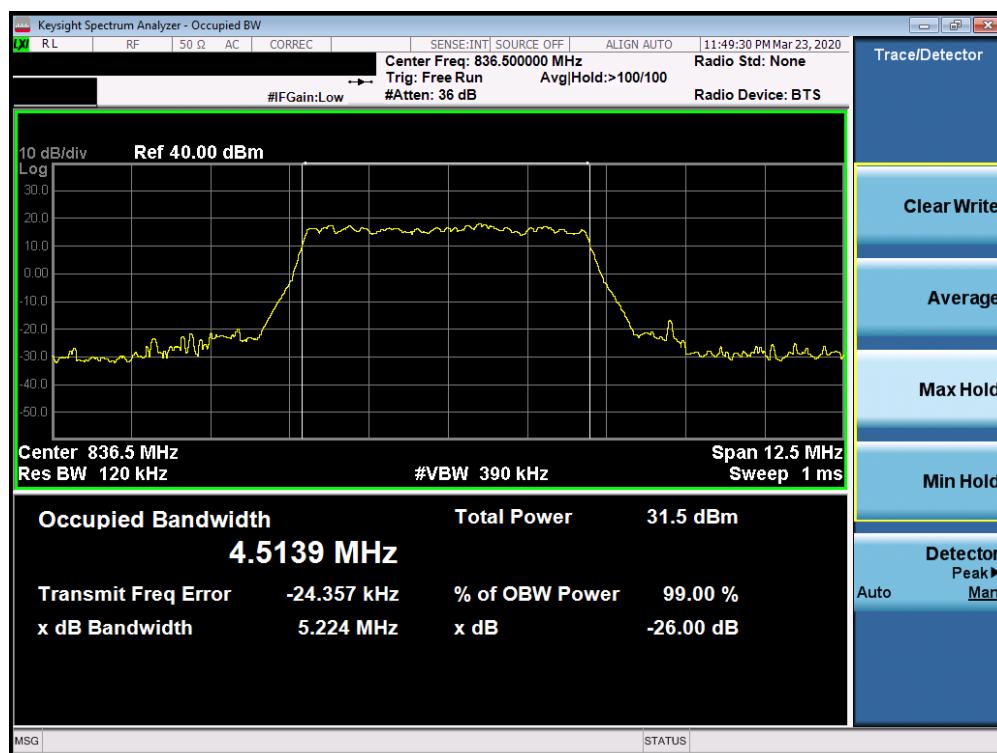
Plot 7-5. Occupied Bandwidth Plot (n5 - 5.0MHz DFT-s OFDM \pi/2 BPSK - Full RB Configuration)
