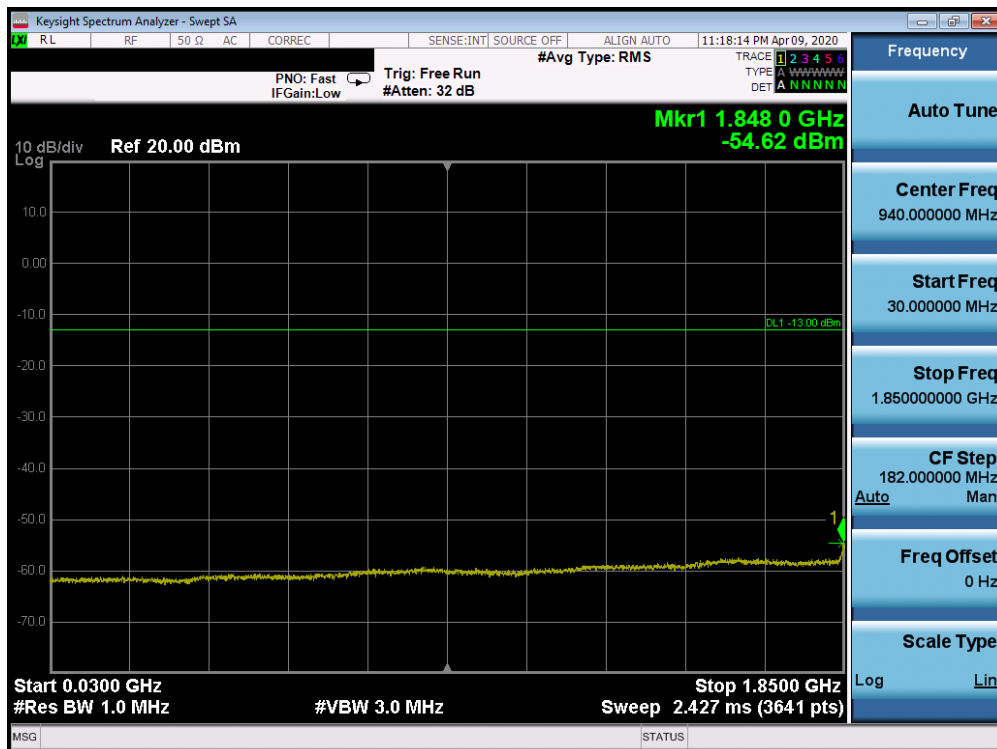
Plot 7-54. Conducted Spurious Plot (n2 - 20.0MHz DFT-s OFDM \pi/2 BPSK - RB Size 1, RB Offset 1 - Mid Channel)
