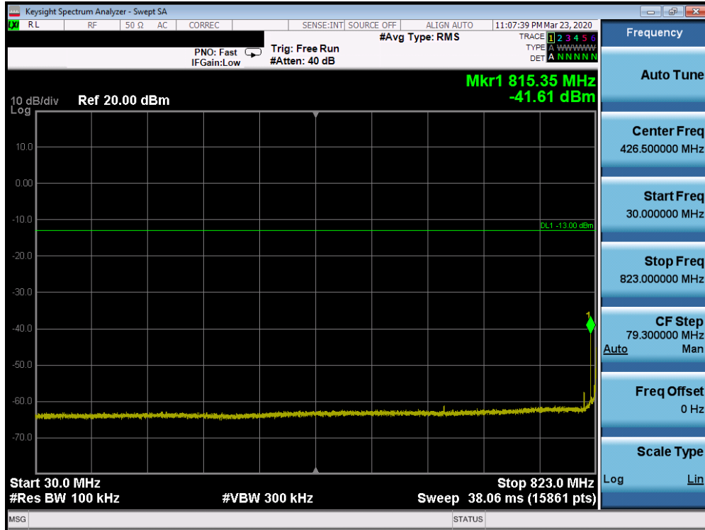
Plot 7-33. Conducted Spurious Plot (n5 - 20.0MHz DFT-s OFDM \pi/2 BPSK - RB Size 1, RB Offset 1 - Low Channel)
