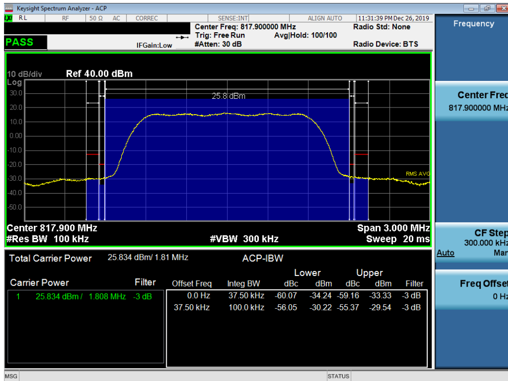
Plot 7-49. Channel Edge Plot (CDMA BC10 - Ch. 476)
