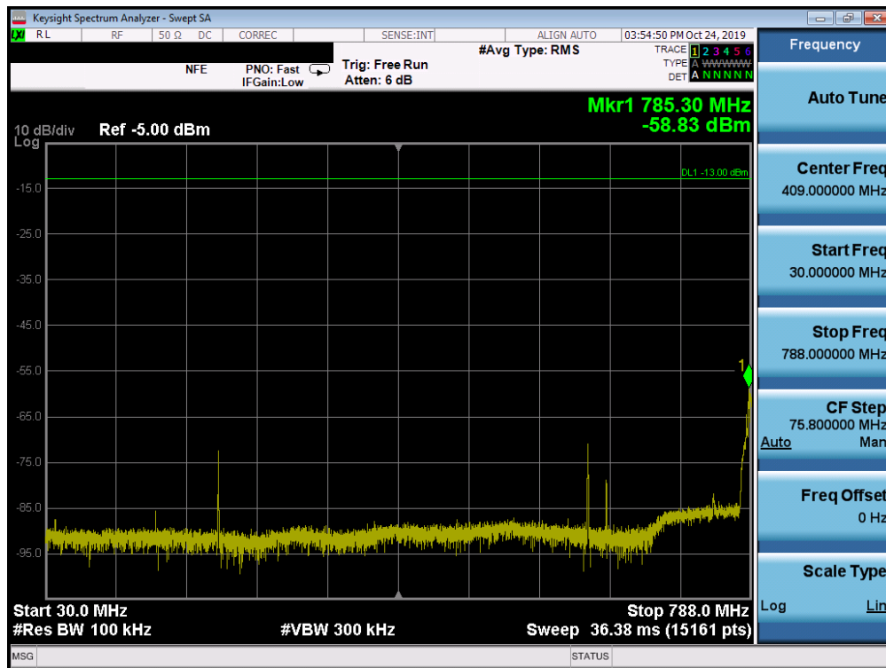
Plot 7-46. Conducted Spurious Plot (LTE Band 14, 5.0 MHz QPSK – RB Size 1, RB Offset 0 – High Channel)
