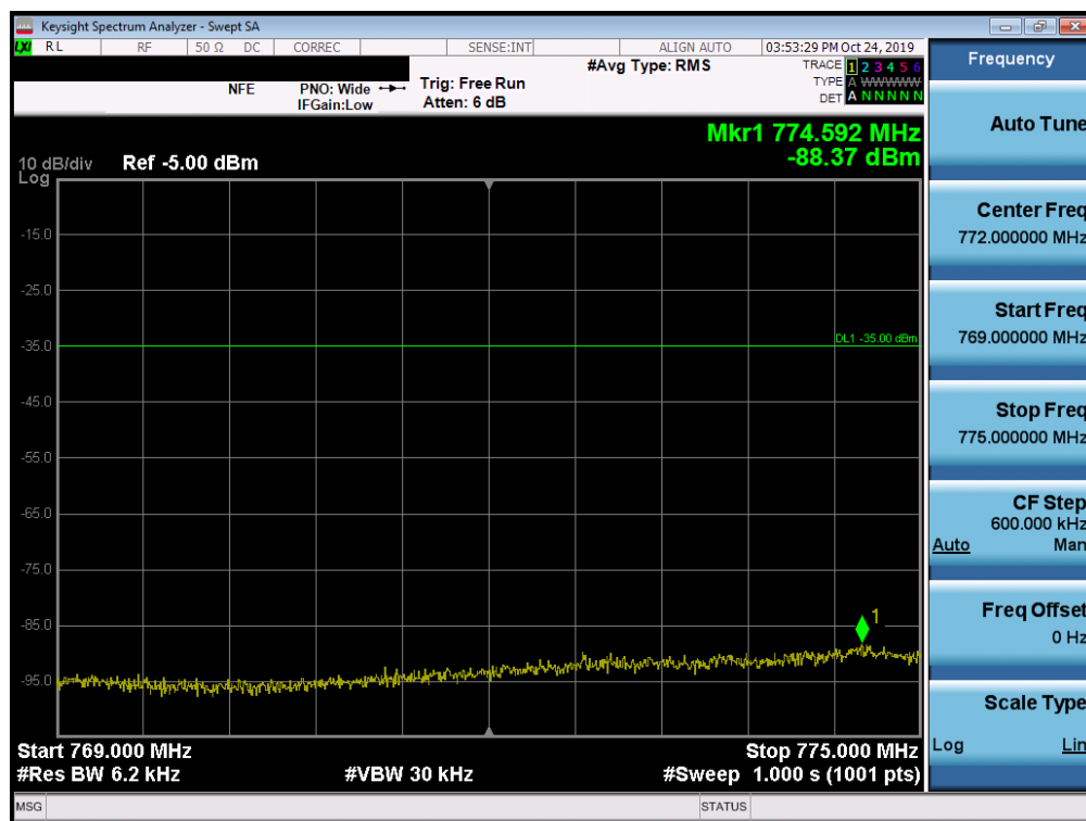
Plot 7-60. Lower Emission Mask Plot (LTE Band 14, 5MHz QPSK - RB Size 25)
