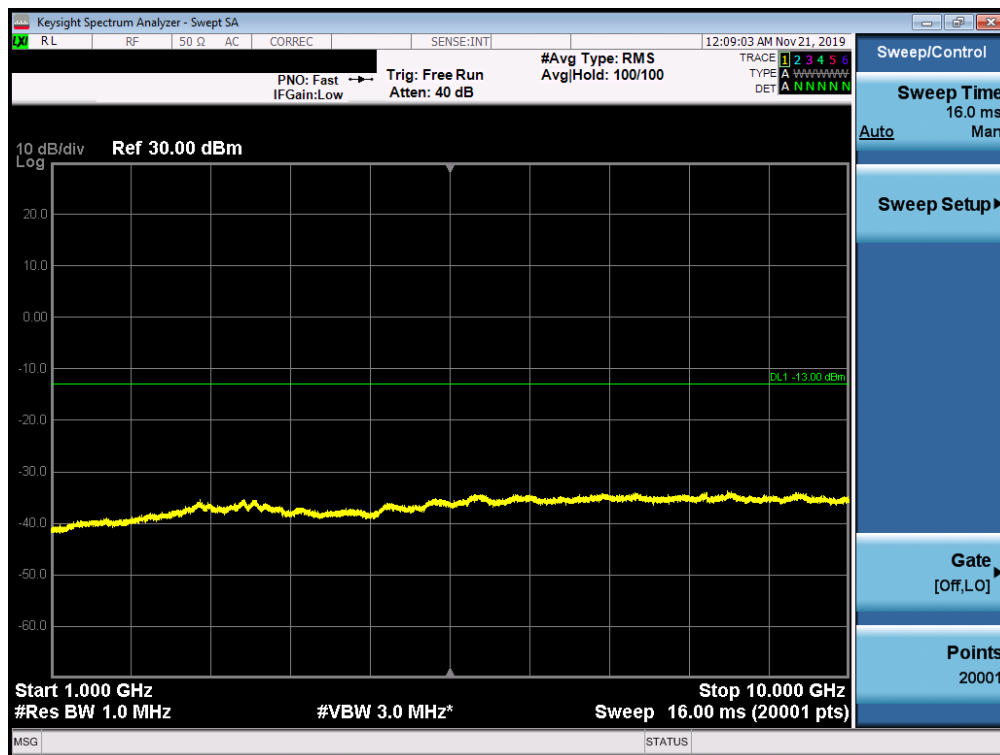
Plot 7-33. Conducted Spurious Plot (CDMA/EvDO, Ch. 476)
