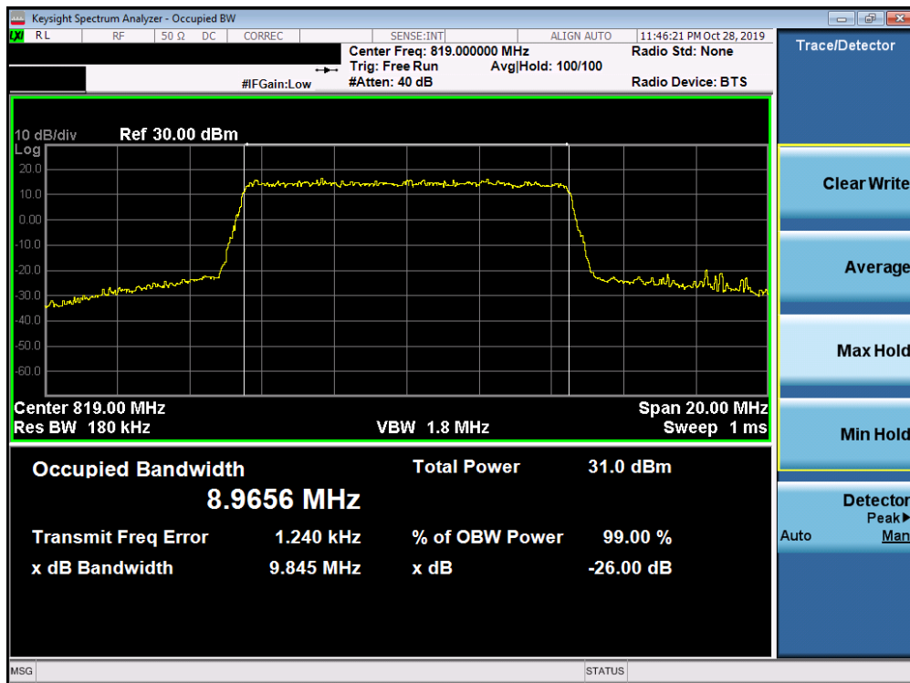
Plot 7-9. Occupied Bandwidth Plot (LTE Band 26 - 10MHz 64-QAM - Full RB Configuration)
