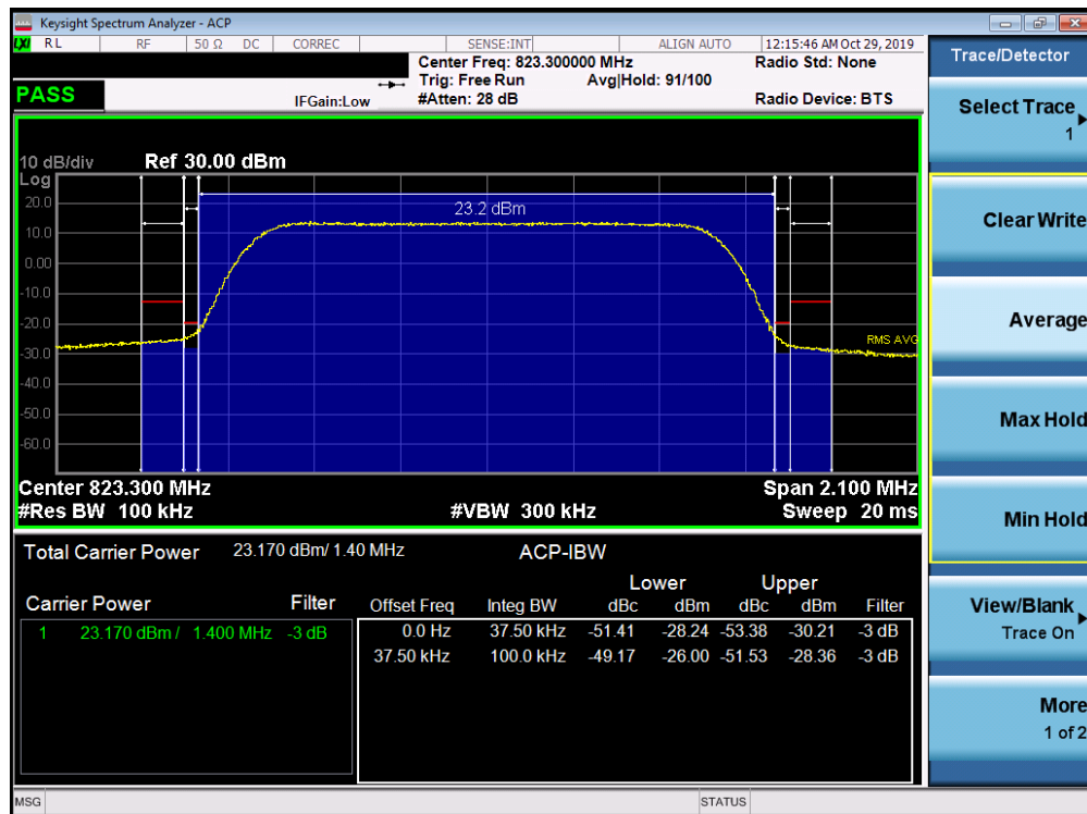
Plot 7-58. Channel Edge Plot (LTE Band 26 - 1.4MHz QPSK - High Channel)
