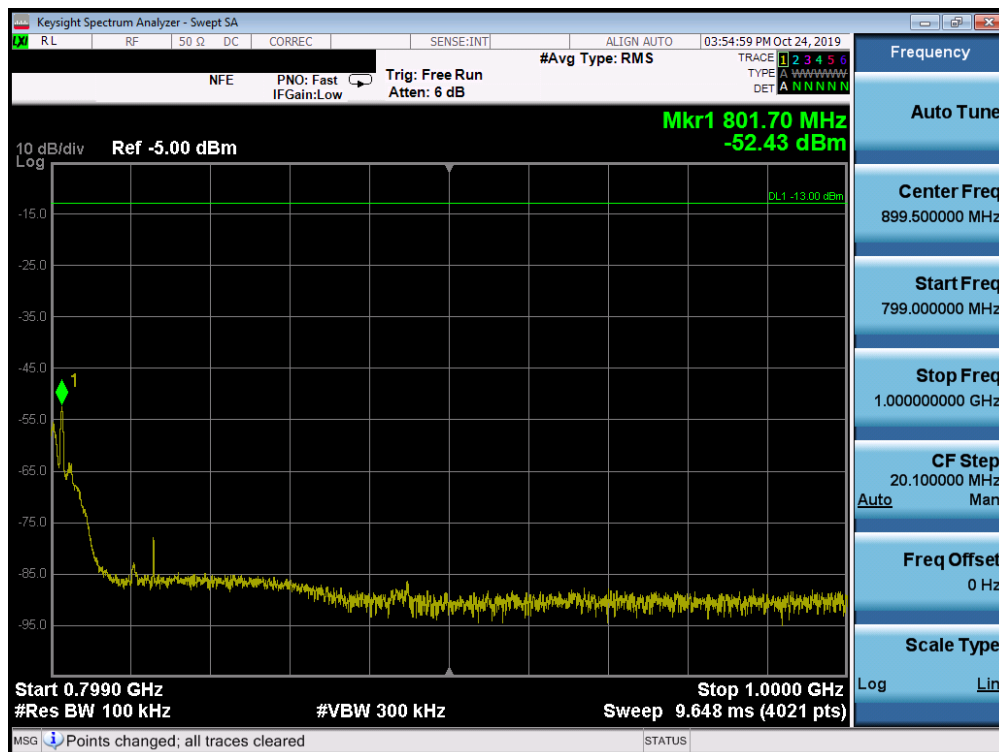
Plot 7-47. Conducted Spurious Plot (LTE Band 14, 5.0 MHz QPSK – RB Size 1, RB Offset 0 – High Channel)
