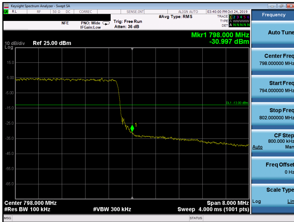
Plot 7-65. Upper Band Edge Plot (LTE Band 14, 10MHz QPSK - RB Size 50)
