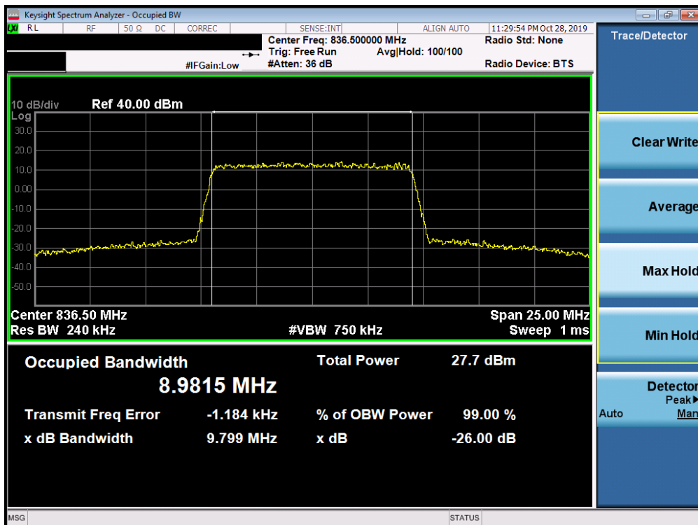
Plot 7-10. Occupied Bandwidth Plot (LTE Band 26 - 10MHz 256-QAM - Full RB Configuration)
