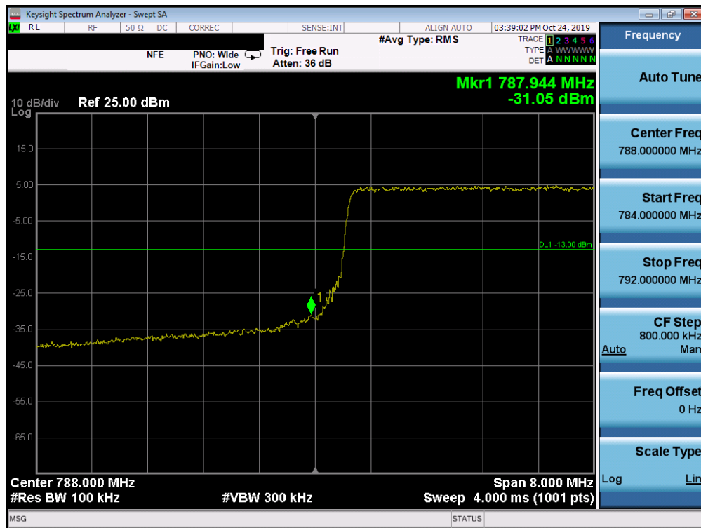
Plot 7-63. Lower Band Edge Plot (LTE Band 14, 10MHz QPSK - RB Size 50)
