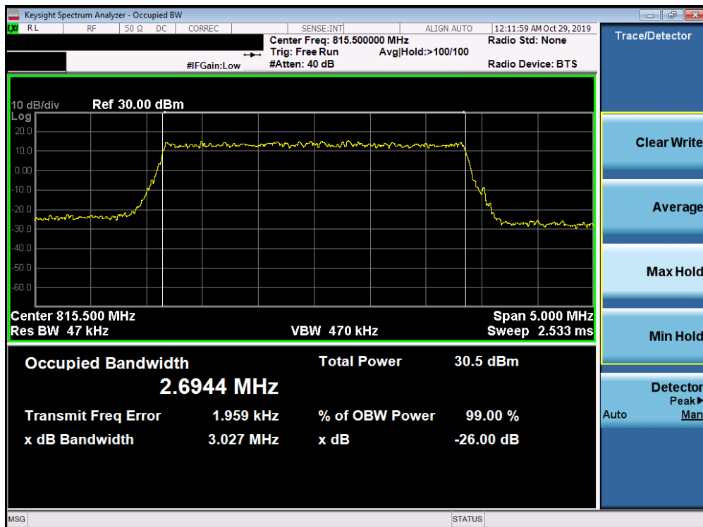
Plot 7-16. Occupied Bandwidth Plot (LTE Band 26 - 3MHz 16-QAM - Full RB Configuration)
