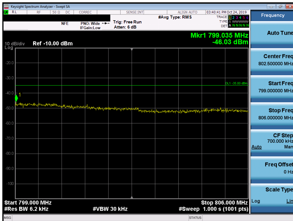
Plot 7-66. Upper Emission Mask Plot (LTE Band 14, 10MHz QPSK - RB Size 50)
