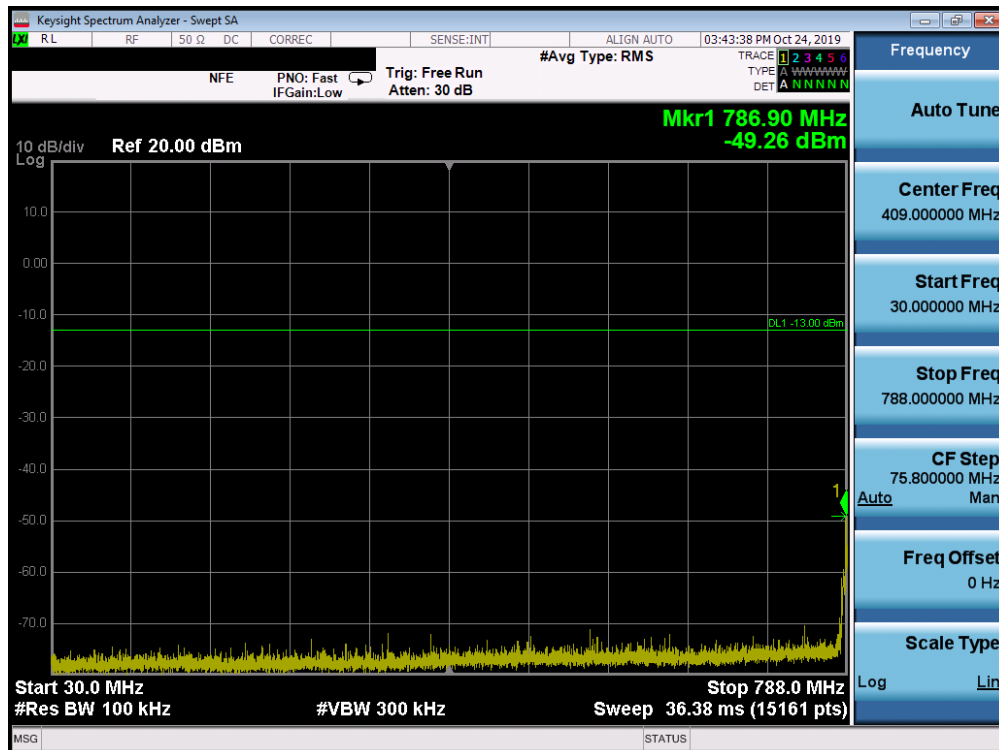
Plot 7-43. Conducted Spurious Plot (LTE Band 14, 5.0 MHz QPSK – RB Size 1, RB Offset 0 – Mid Channel)
