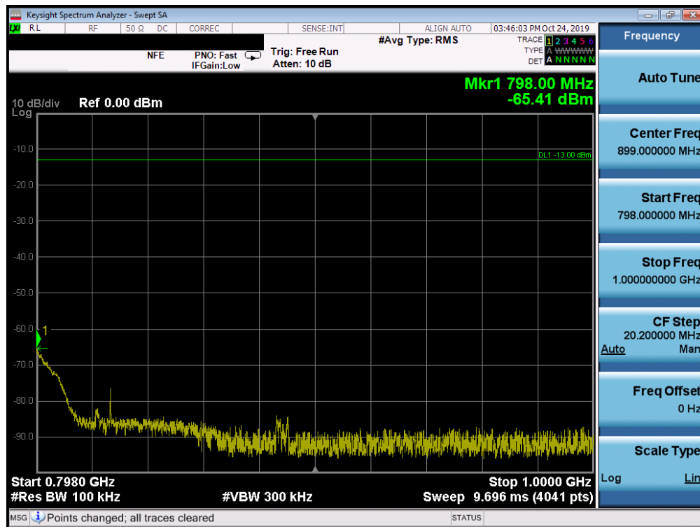
Plot 7-41. Conducted Spurious Plot (LTE Band 14, 5.0 MHz QPSK – RB Size 1, RB Offset 0 – Low Channel)
