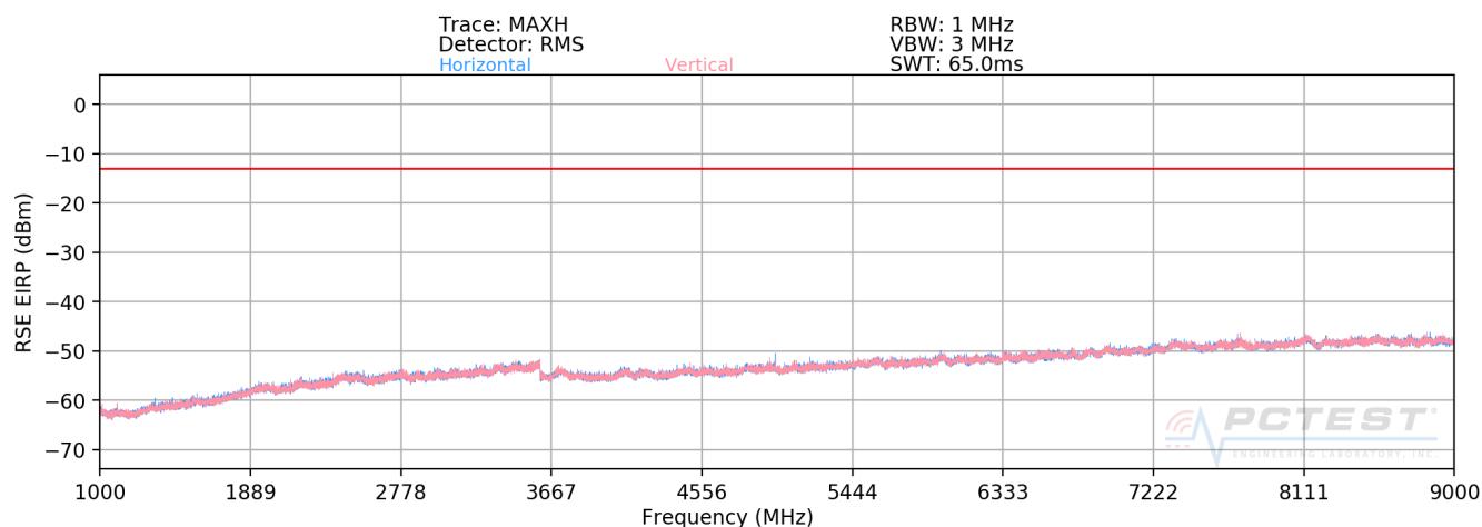
Plot 7-70. Radiated Spurious Plot (Band 26)
