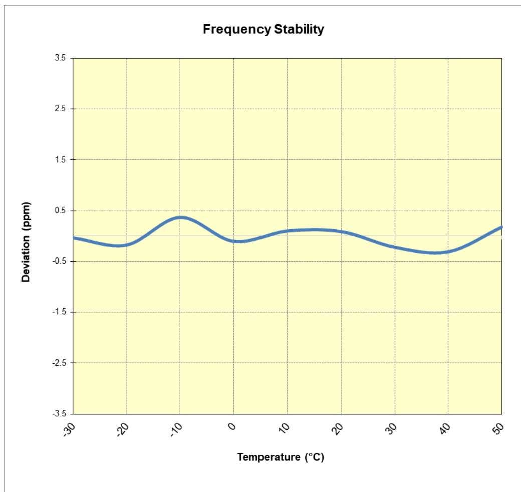
Figure 7-6. CDMA BC10 Frequency Stability Chart
