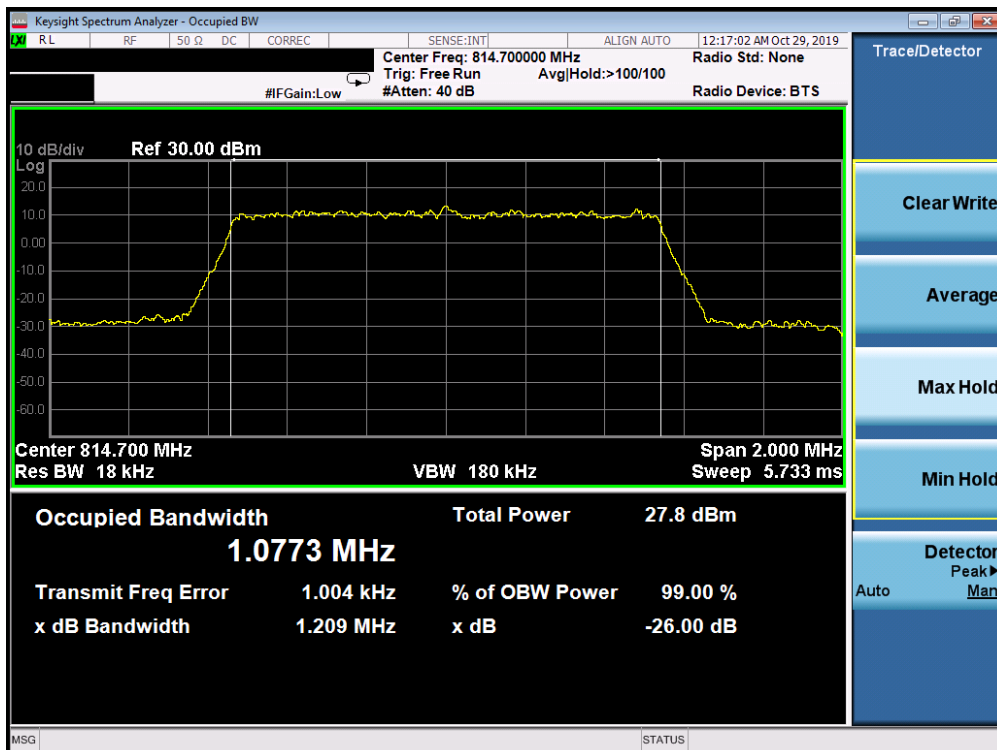
Plot 7-22. Occupied Bandwidth Plot (LTE Band 26 - 1.4MHz 256-QAM - Full RB Configuration)
