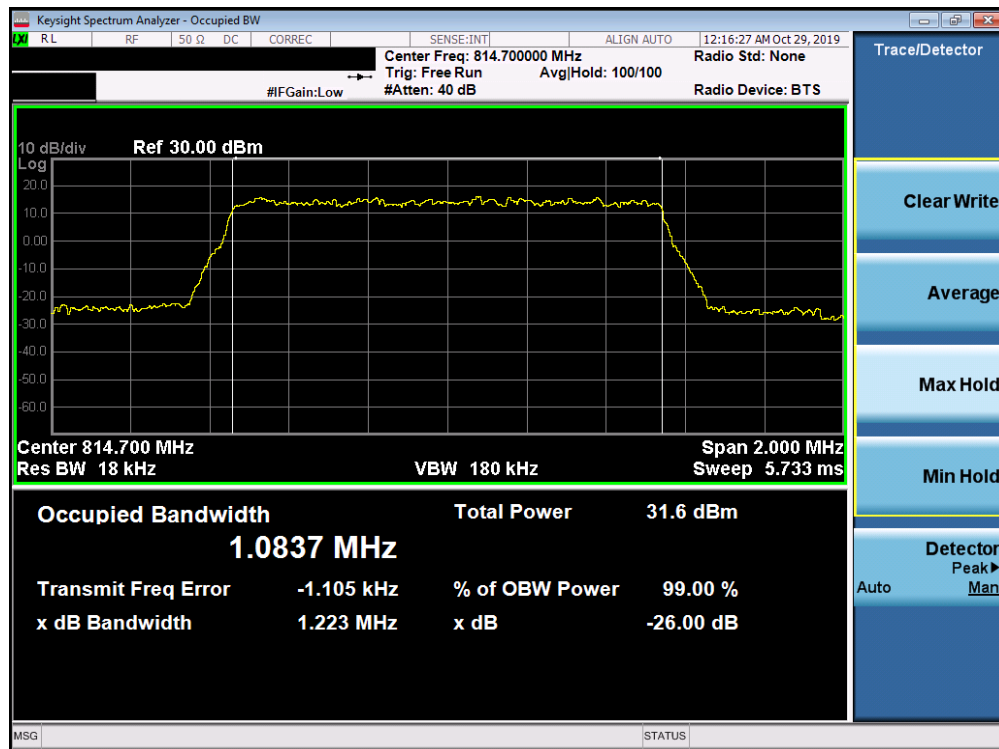
Plot 7-19. Occupied Bandwidth Plot (LTE Band 26 - 1.4MHz QPSK - Full RB Configuration)
