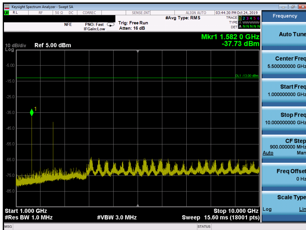
Plot 7-45. Conducted Spurious Plot (LTE Band 14, 5.0 MHz QPSK – RB Size 1, RB Offset 0 – Mid Channel)
