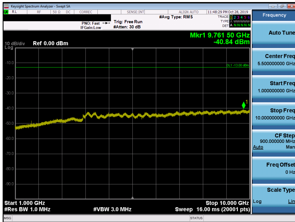
Plot 7-39. Conducted Spurious Plot (LTE Band 26 - 10MHz QPSK - RB Size 1, RB Offset 0 - Mid Channel)
