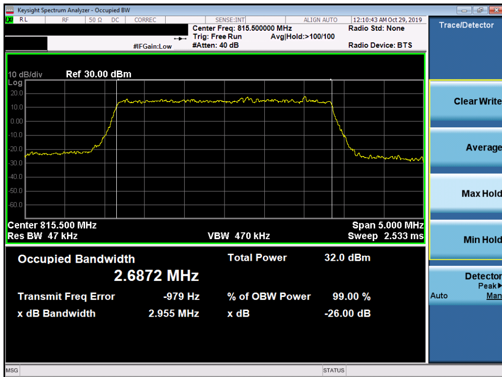
Plot 7-15. Occupied Bandwidth Plot (LTE Band 26 - 3MHz QPSK - Full RB Configuration)
