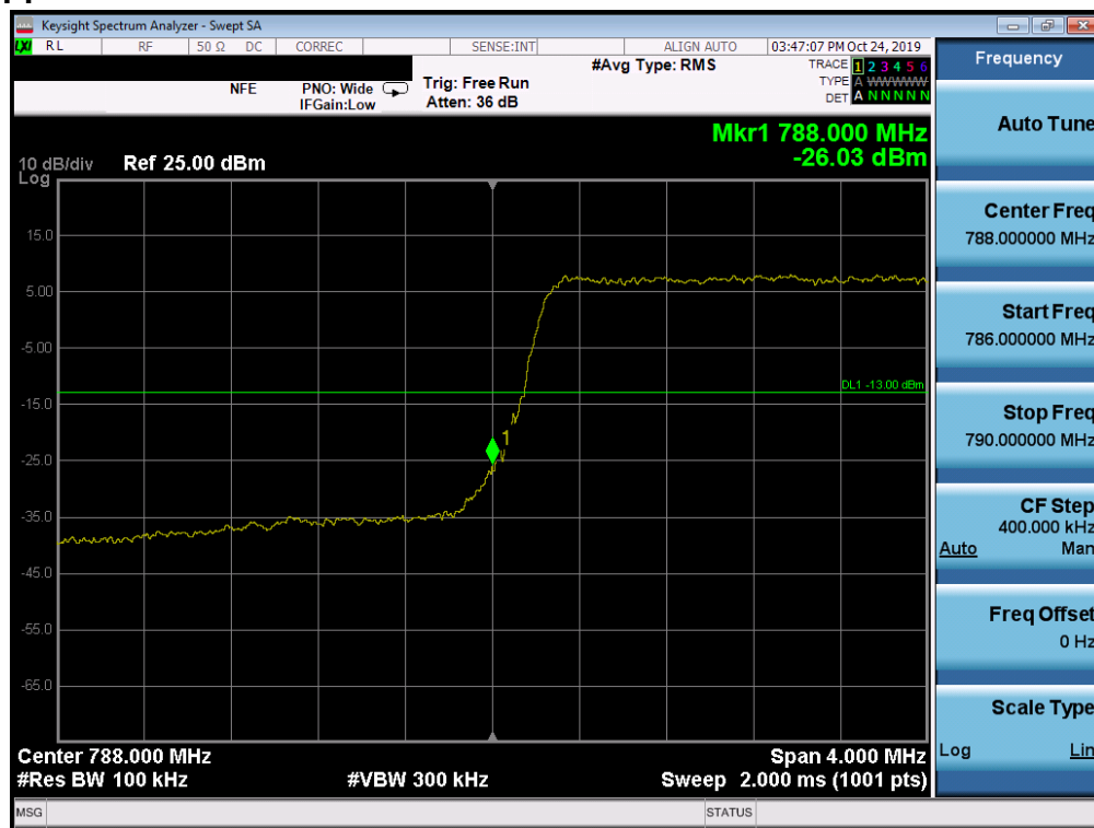
Plot 7-59. Lower Band Edge Plot (LTE Band 14, 5MHz QPSK - RB Size 25)
