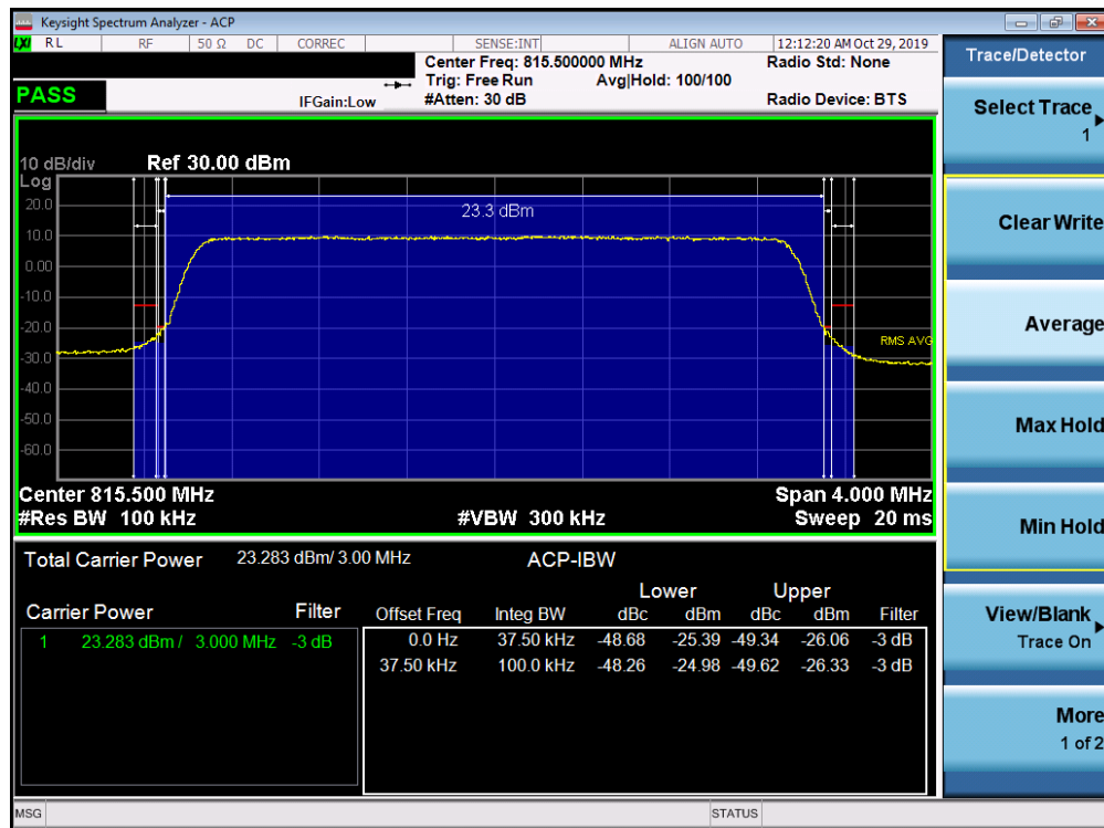
Plot 7-55. Channel Edge Plot (LTE Band 26 - 3MHz QPSK - Low Channel)
