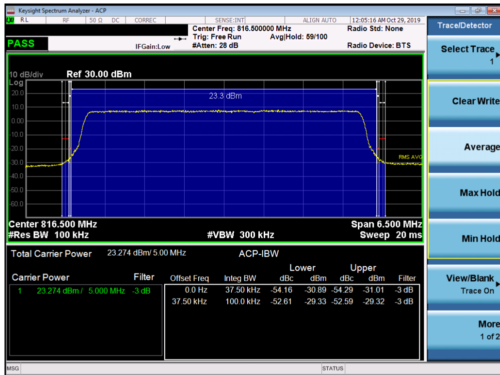
Plot 7-53. Channel Edge Plot (LTE Band 26 - 5MHz QPSK - Low Channel)
