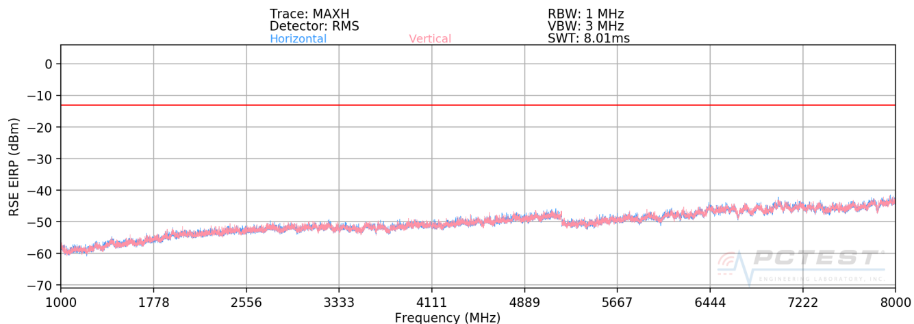
Plot 7-71. Radiated Spurious Plot (Band 14)
