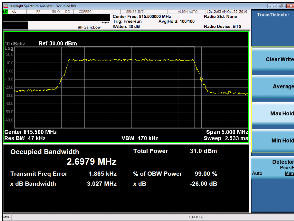
Plot 7-17. Occupied Bandwidth Plot (LTE Band 26 - 3MHz 64-QAM - Full RB Configuration)
