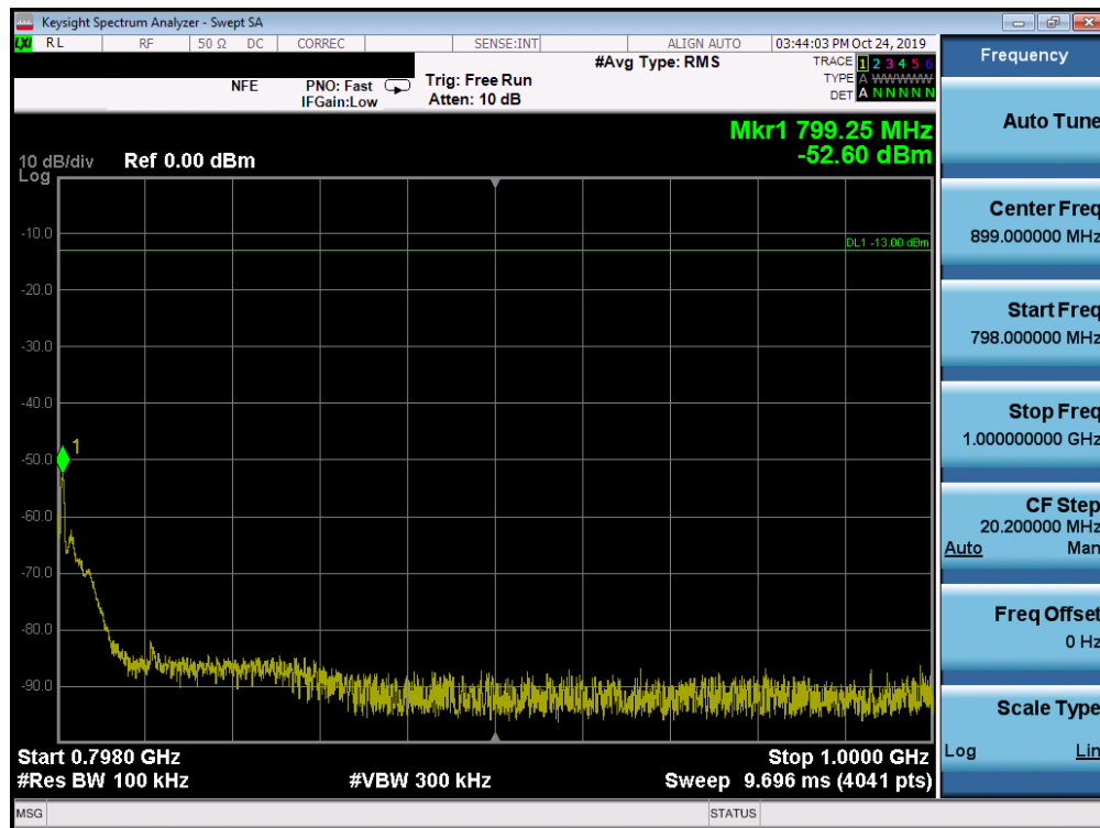
Plot 7-44. Conducted Spurious Plot (LTE Band 14, 5.0 MHz QPSK – RB Size 1, RB Offset 0 – Mid Channel)
