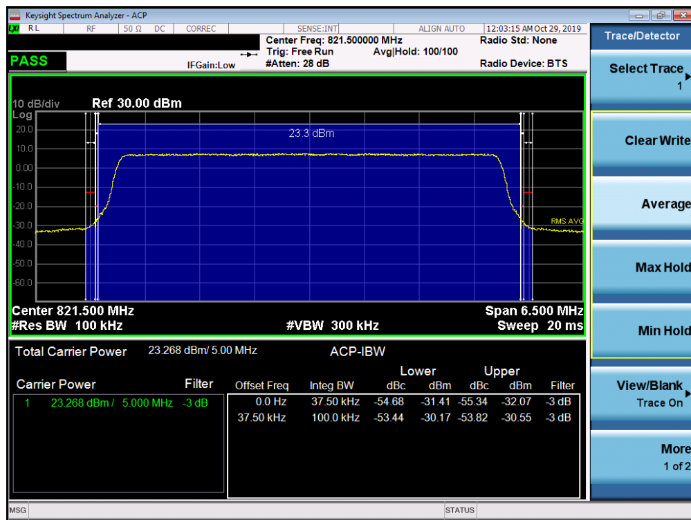
Plot 7-54. Channel Edge Plot (LTE Band 26 - 5MHz QPSK - High Channel)
