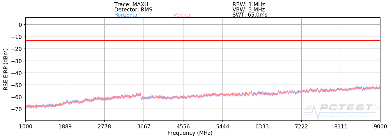
Plot 7-69. Radiated Spurious Plot (CDMA BC10)
