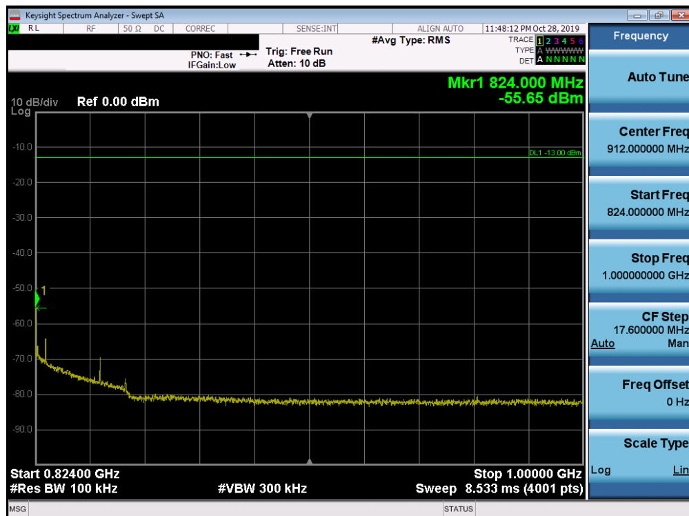
Plot 7-38. Conducted Spurious Plot (LTE Band 26 - 10MHz QPSK - RB Size 1, RB Offset 0 - Mid Channel)
