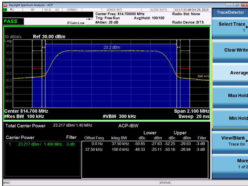
Plot 7-57. Channel Edge Plot (LTE Band 26 - 1.4MHz QPSK - Low Channel)
