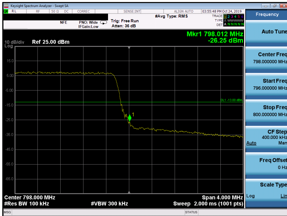
Plot 7-61. Upper Band Edge Plot (LTE Band 14, 5MHz QPSK - RB Size 25)
