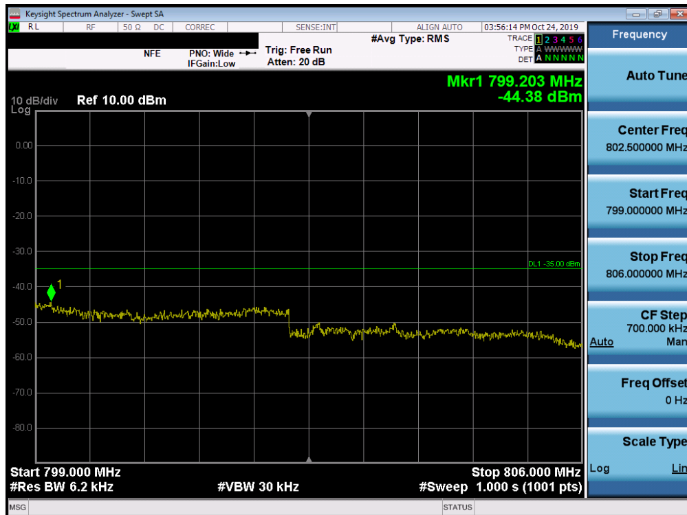
Plot 7-62. Upper Emission Mask Plot (LTE Band 14, 5MHz QPSK - RB Size 25)
