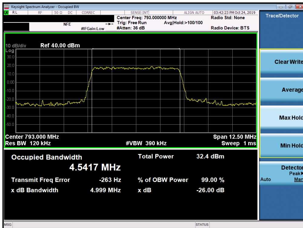
Plot 7-27. Occupied Bandwidth Plot (LTE Band 14 - 5MHz QPSK - Full RB Configuration)
