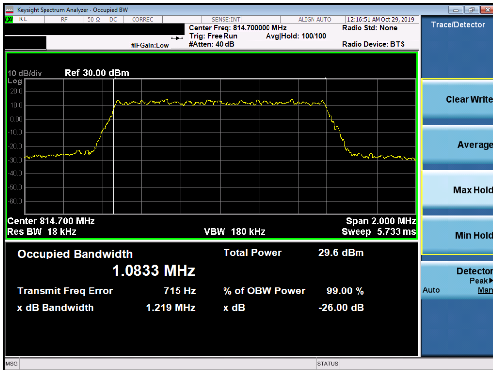
Plot 7-21. Occupied Bandwidth Plot (LTE Band 26 - 1.4MHz 64-QAM - Full RB Configuration)
