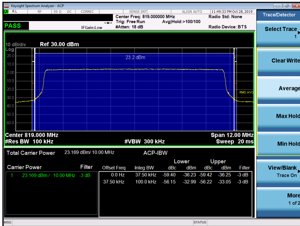
Plot 7-52. Channel Edge Plot (LTE Band 26 - 10MHz QPSK - Low Channel)
