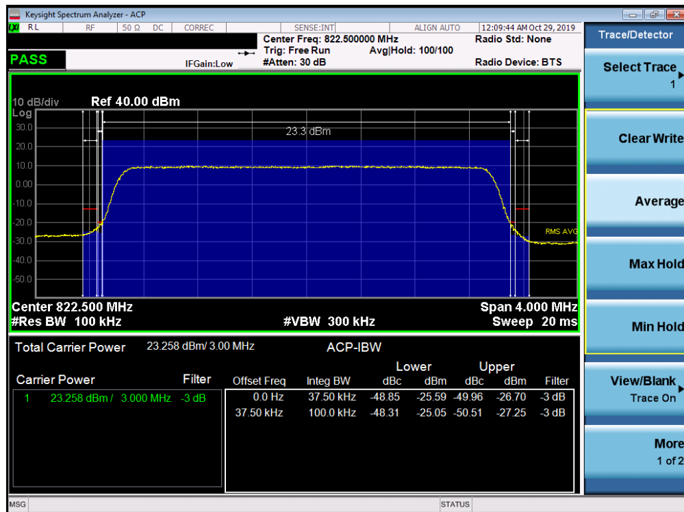
Plot 7-56. Channel Edge Plot (LTE Band 26 - 3MHz QPSK - High Channel)
