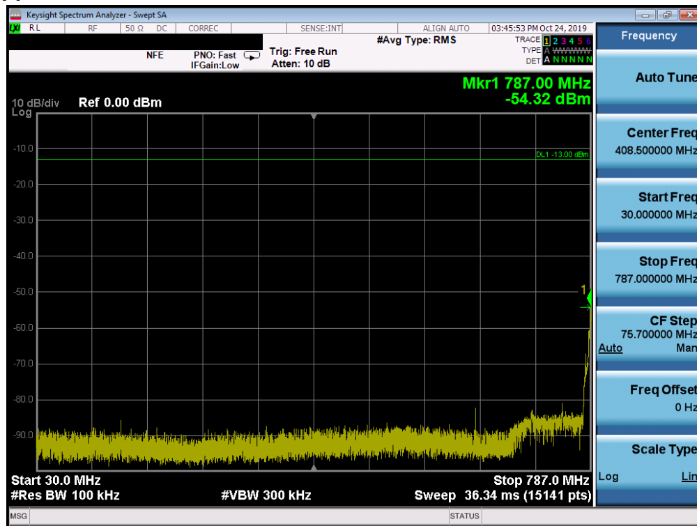
Plot 7-40. Conducted Spurious Plot (LTE Band 14, 5.0 MHz QPSK – RB Size 1, RB Offset 0 – Low Channel)
