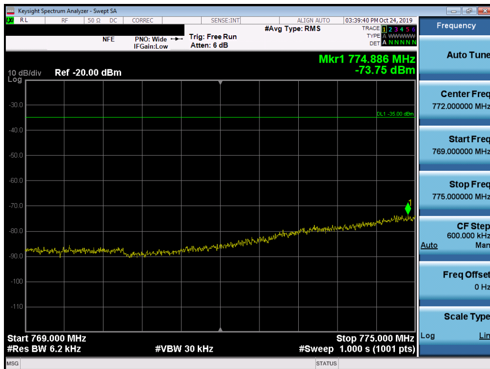
Plot 7-64. Lower Emission Mask Plot (LTE Band 14, 10MHz QPSK - RB Size 50)
