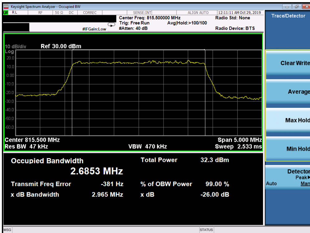
Plot 7-18. Occupied Bandwidth Plot (LTE Band 26 - 3MHz 256-QAM - Full RB Configuration)
