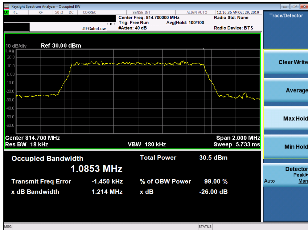
Plot 7-20. Occupied Bandwidth Plot (LTE Band 26 - 1.4MHz 16-QAM - Full RB Configuration)
