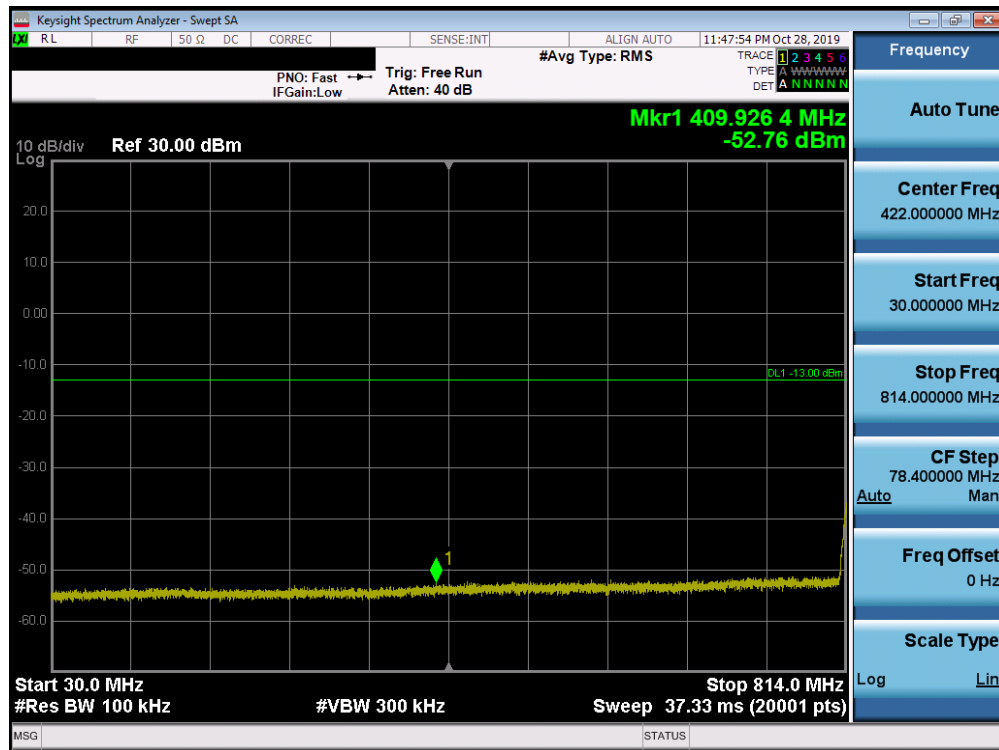
Plot 7-37. Conducted Spurious Plot (LTE Band 26 - 10MHz QPSK - RB Size 1, RB Offset 0 - Mid Channel)
