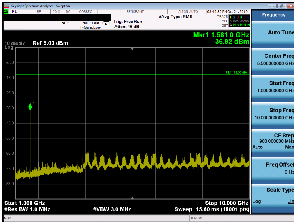
Plot 7-42. Conducted Spurious Plot (LTE Band 14, 5.0 MHz QPSK – RB Size 1, RB Offset 0 – Low Channel)
