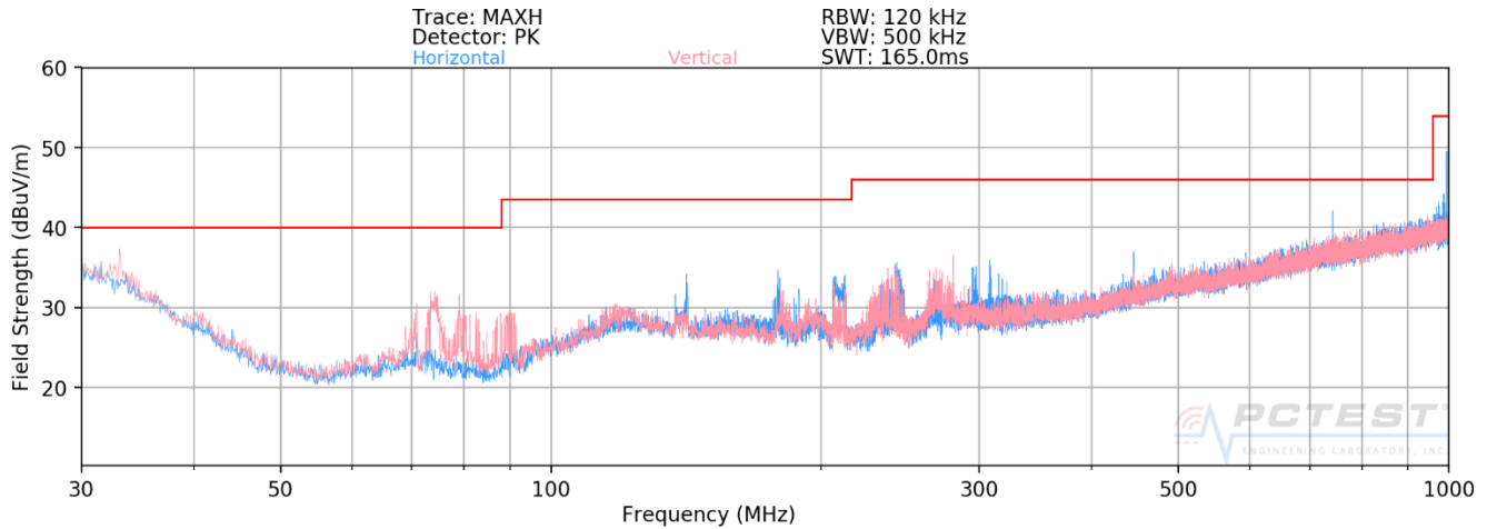
Plot 7-7. Radiated Spurious Plot below 1GHz [Radiated Test Config. 4]
