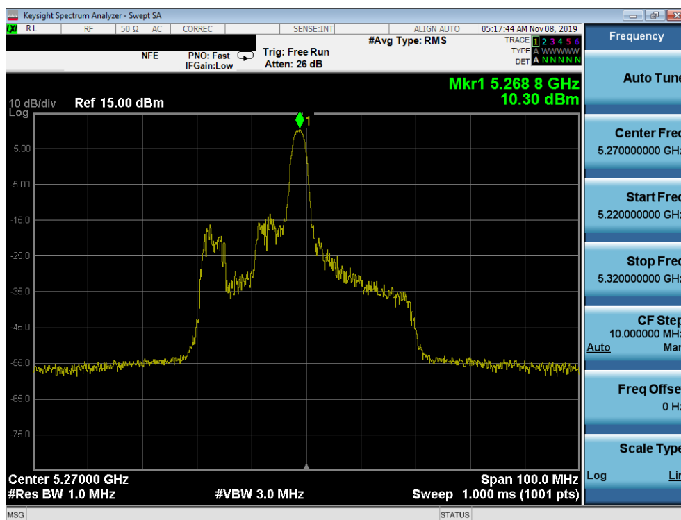
Plot 7-64. Power Spectral Density Plot SISO ANT1 (40MHz BW 802.11ax – 26 Tones (UNII Band 2A) – Ch. 54)
