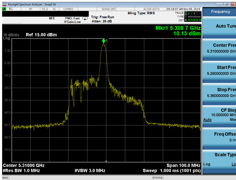
Plot 7-65. Power Spectral Density Plot SISO ANT1 (40MHz BW 802.11ax – 26 Tones (UNII Band 2A) – Ch. 62)
