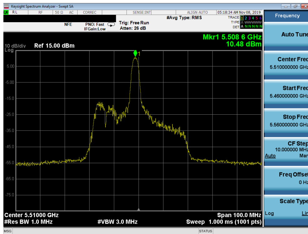
Plot 7-70. Power Spectral Density Plot SISO ANT1 (40MHz BW 802.11ax – 26 Tones (UNII Band 2C) – Ch. 102)
