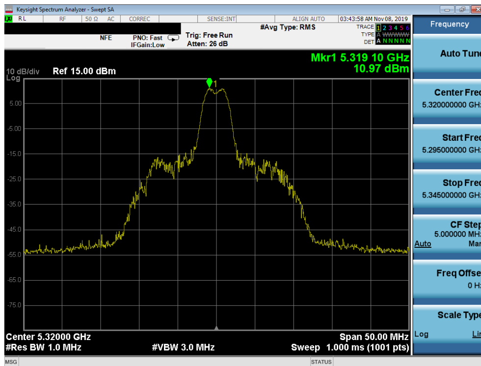
Plot 7-63. Power Spectral Density Plot SISO ANT1 (20MHz BW 802.11ax – 26 Tones (UNII Band 2A) – Ch. 64)
