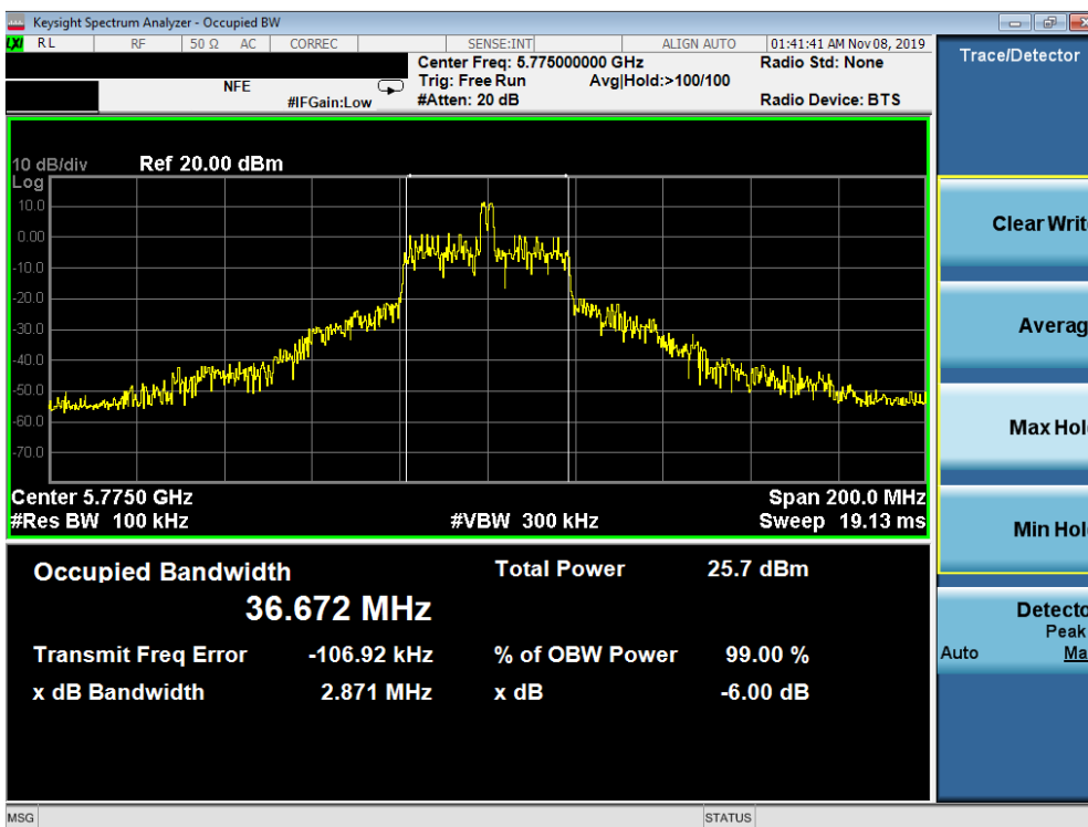
Plot 7-48. 6dB Bandwidth Plot SISO ANT1 (80MHz BW 802.11ax – 26 Tones (UNII Band 3) – Ch. 155)
