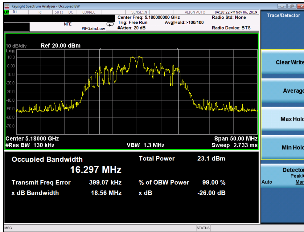
Plot 7-22. 26dB Bandwidth Plot SISO ANT2 (20MHz BW 802.11ax – 26 Tones (UNII Band 1) – Ch. 36)
