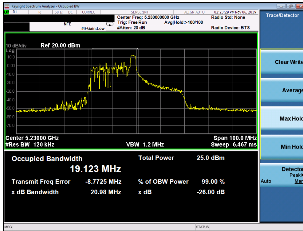
Plot 7-5. 26dB Bandwidth Plot SISO ANT1 (40MHz BW 802.11ax – 26 Tones (UNII Band 1) – Ch. 46)
