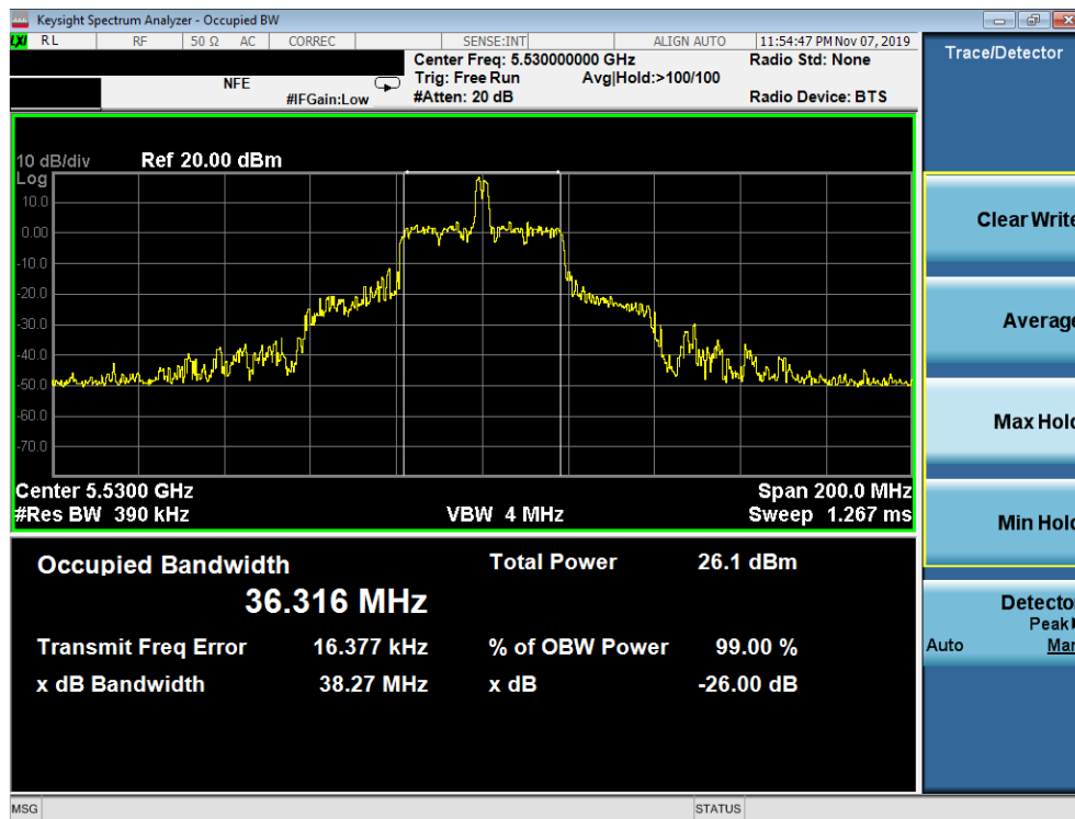
Plot 7-40. 26dB Bandwidth Plot SISO ANT2 (80MHz BW 802.11ax – 26 Tones (UNII Band 2C) – Ch. 106)
