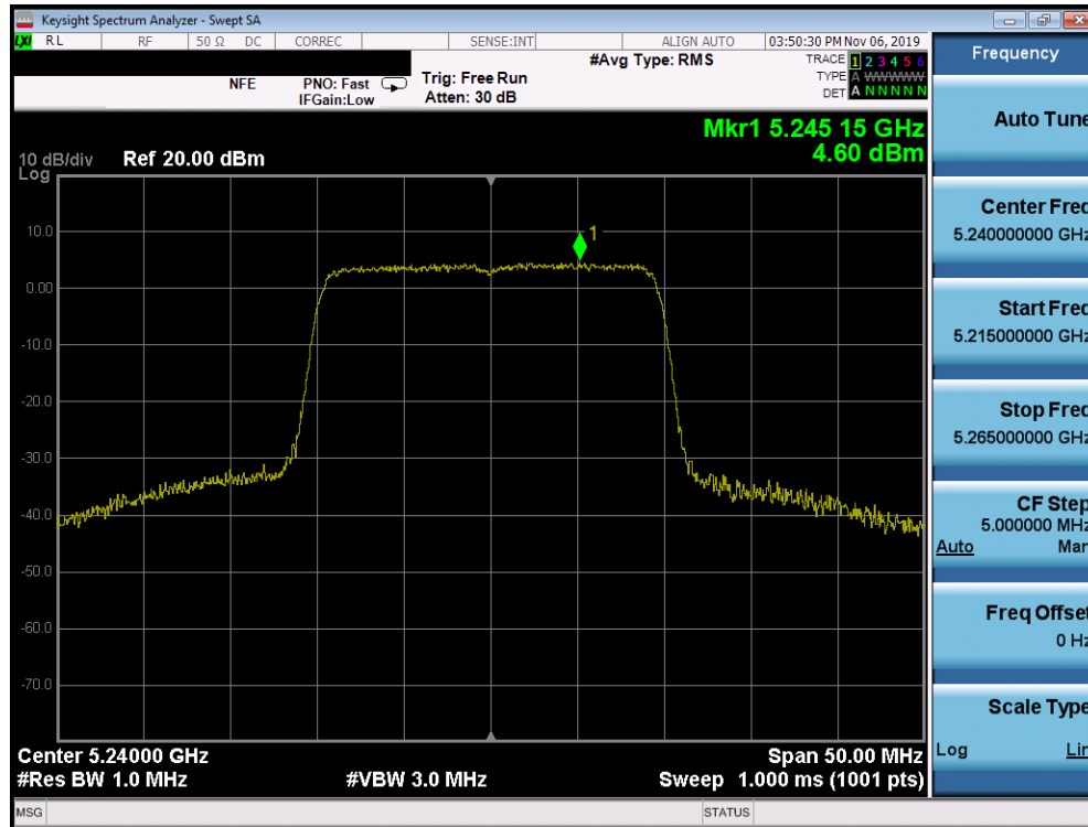
Plot 7-84. Power Spectral Density Plot SISO ANT1 (20MHz BW 802.11ax – Full Tones (UNII Band 1) – Ch. 48)
