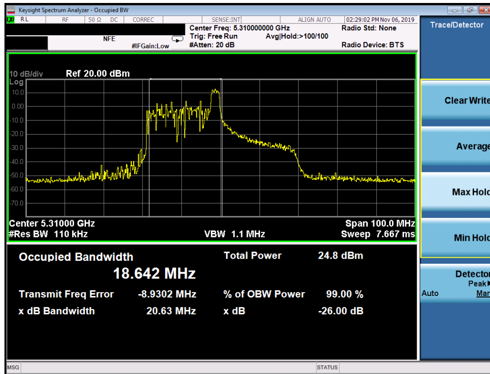
Plot 7-11. 26dB Bandwidth Plot SISO ANT1 (40MHz BW 802.11ax – 26 Tones (UNII Band 2A) – Ch. 62)
