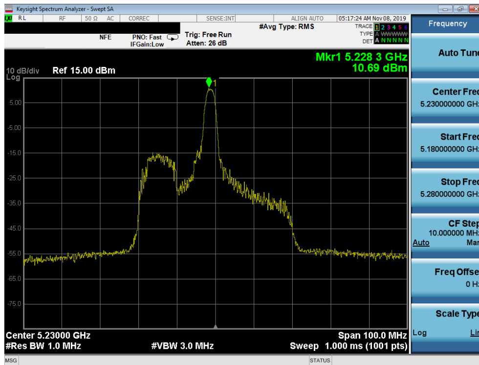
Plot 7-59. Power Spectral Density Plot SISO ANT1 (40MHz BW 802.11ax – 26 Tones (UNII Band 1) – Ch. 46)
