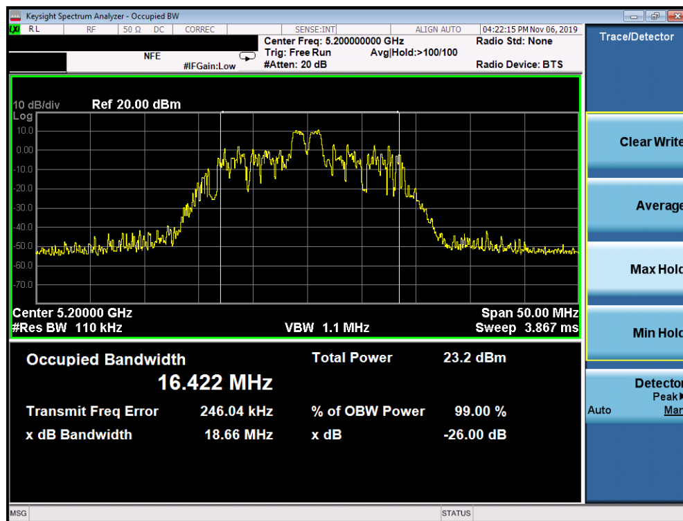
Plot 7-23. 26dB Bandwidth Plot SISO ANT2 (20MHz BW 802.11ax – 26 Tones (UNII Band 1) – Ch. 40)
