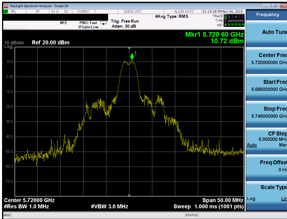
Plot 7-69. Power Spectral Density Plot SISO ANT1 (20MHz BW 802.11ax – 26 Tones (UNII Band 2C) – Ch. 144)
