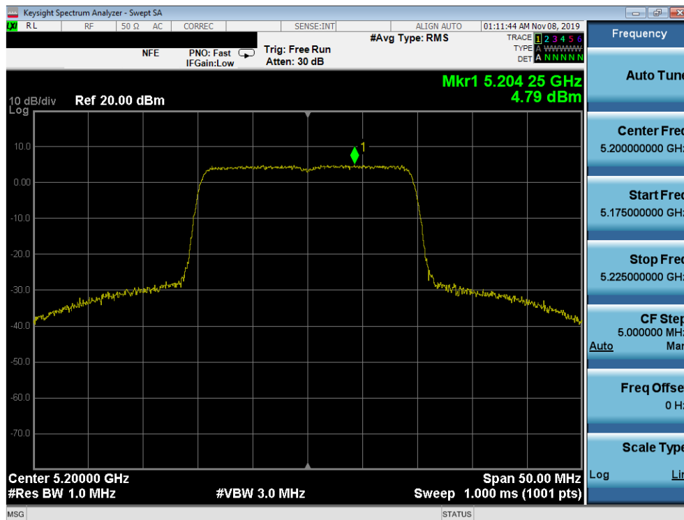
Plot 7-137. Power Spectral Density Plot SISO ANT2 (20MHz BW 802.11ax – Full Tones (UNII Band 1) – Ch. 40)
