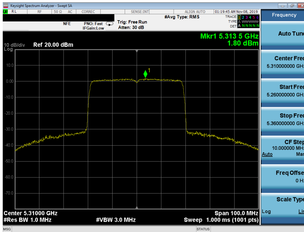
Plot 7-146. Power Spectral Density Plot SISO ANT2 (40MHz BW 802.11ax – Full Tones (UNII Band 2A) – Ch. 62)
