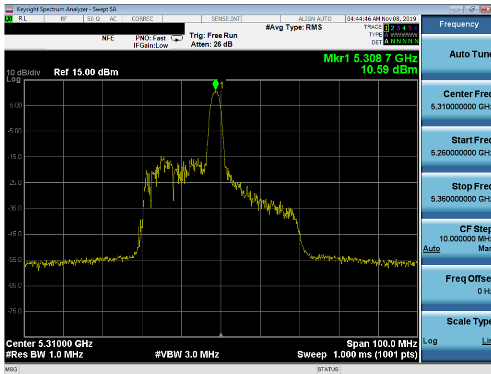
Plot 7-119. Power Spectral Density Plot SISO ANT2 (40MHz BW 802.11ax – 26 Tones (UNII Band 2A) – Ch. 62)
