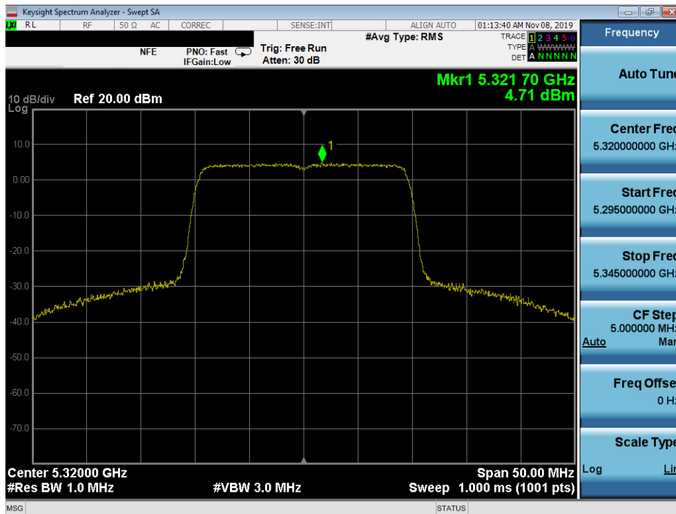
Plot 7-144. Power Spectral Density Plot SISO ANT2 (20MHz BW 802.11ax – Full Tones (UNII Band 2A) – Ch. 64)
