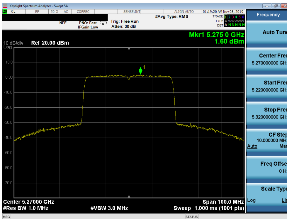
Plot 7-145. Power Spectral Density Plot SISO ANT2 (40MHz BW 802.11ax – Full Tones (UNII Band 2A) – Ch. 54)
