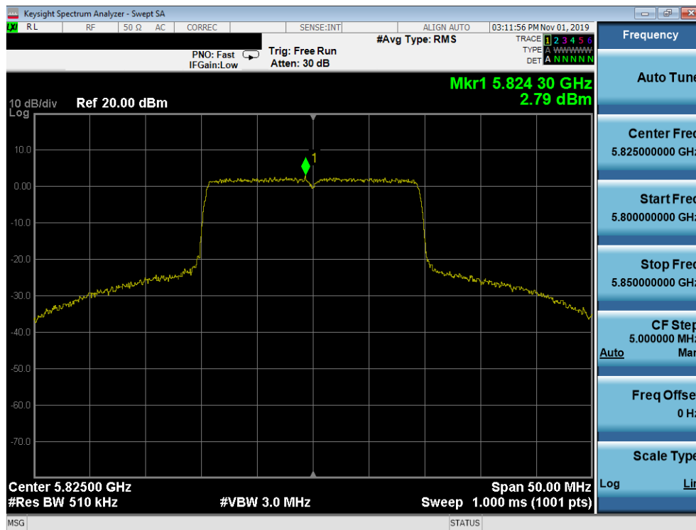
Plot 7-105. Power Spectral Density Plot SISO ANT1 (20 MHz BW 802.11ax – Full Tones (UNII Band 3) – Ch. 165)
