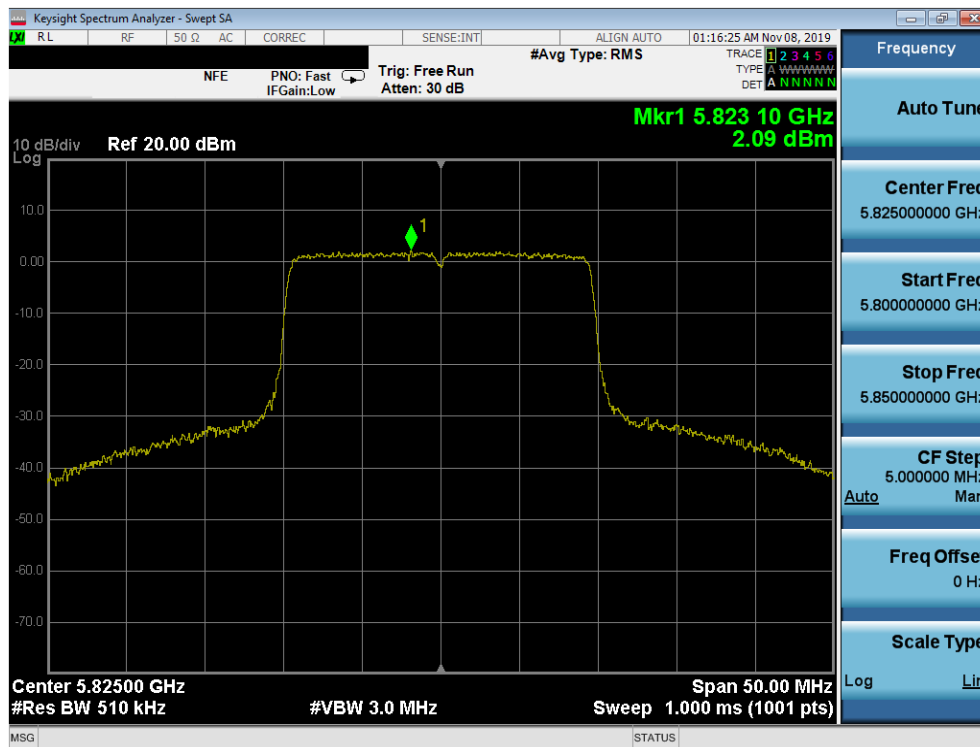
Plot 7-159. Power Spectral Density Plot SISO ANT2 (20 MHz BW 802.11ax – Full Tones (UNII Band 3) – Ch. 165)
