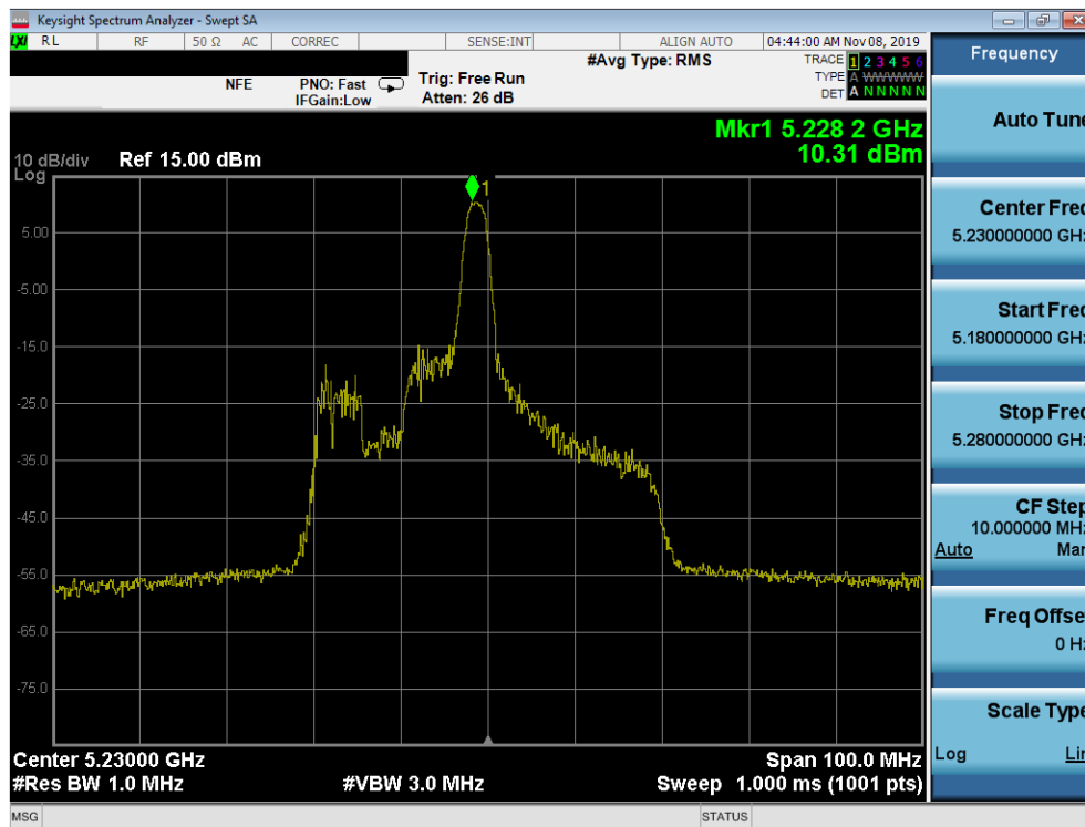
Plot 7-113. Power Spectral Density Plot SISO ANT2 (40MHz BW 802.11ax – 26 Tones (UNII Band 1) – Ch. 46)
