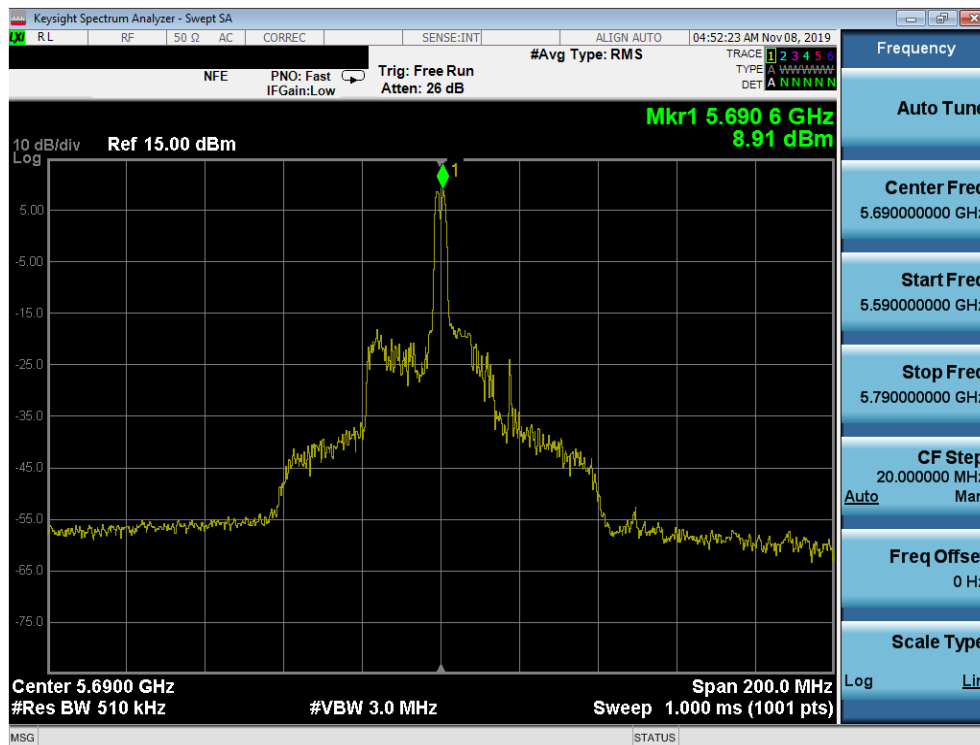
Plot 7-129. Power Spectral Density Plot SISO ANT2 (80MHz BW 802.11ax – 26 Tones (UNII Band 2C) – Ch. 138)
