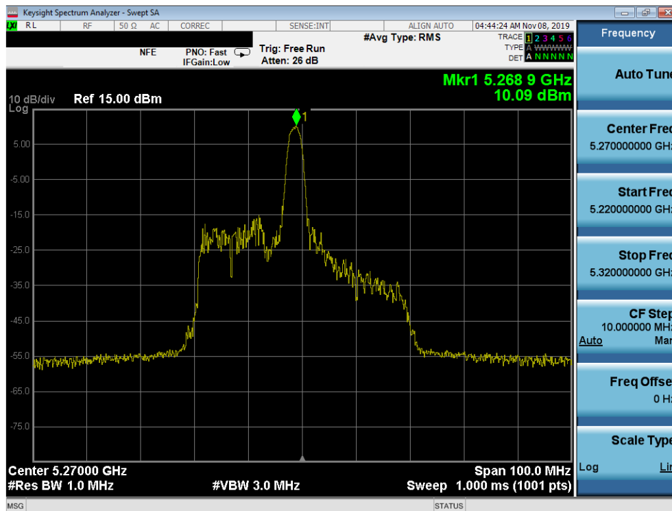
Plot 7-118. Power Spectral Density Plot SISO ANT2 (40MHz BW 802.11ax – 26 Tones (UNII Band 2A) – Ch. 54)
