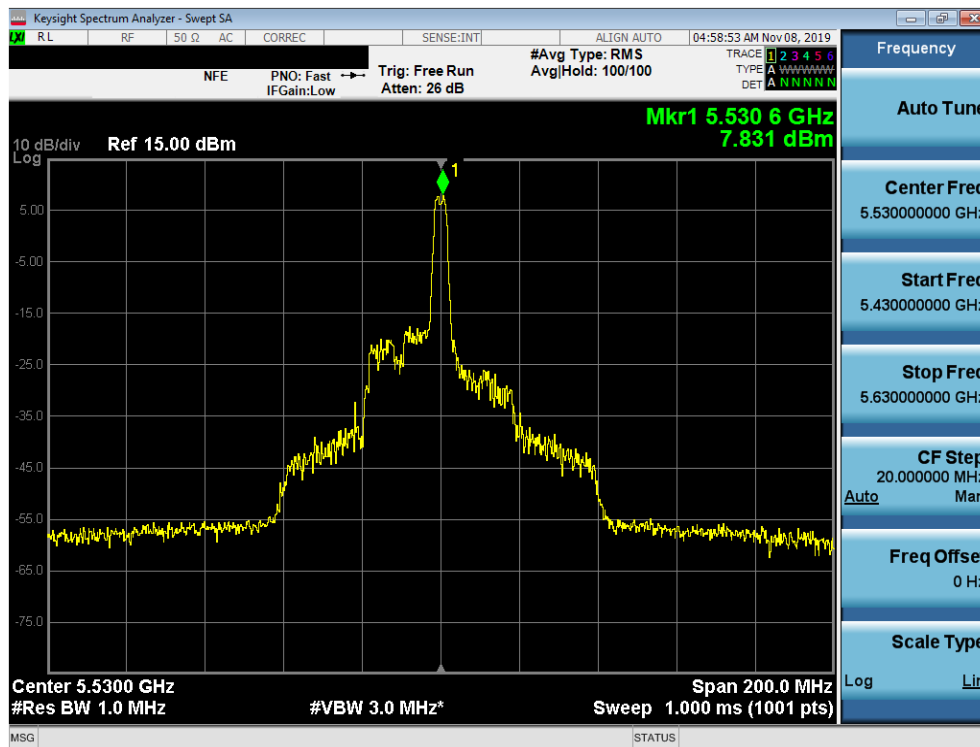
Plot 7-235. Power Spectral Density Plot MIMO ANT2 (80MHz BW 802.11ax – 26 Tones (UNII Band 2C) – Ch. 106)
