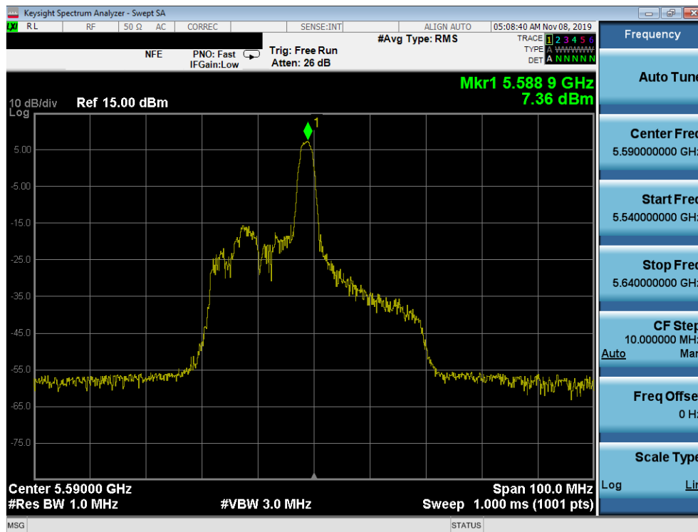
Plot 7-233. Power Spectral Density Plot MIMO ANT2 (40MHz BW 802.11ax – 26 Tones (UNII Band 2C) – Ch. 118)
