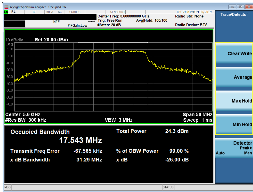
Plot 7-32. 26dB Bandwidth Plot SISO ANT1 (802.11a (UNII Band 2C) – Ch. 120)
