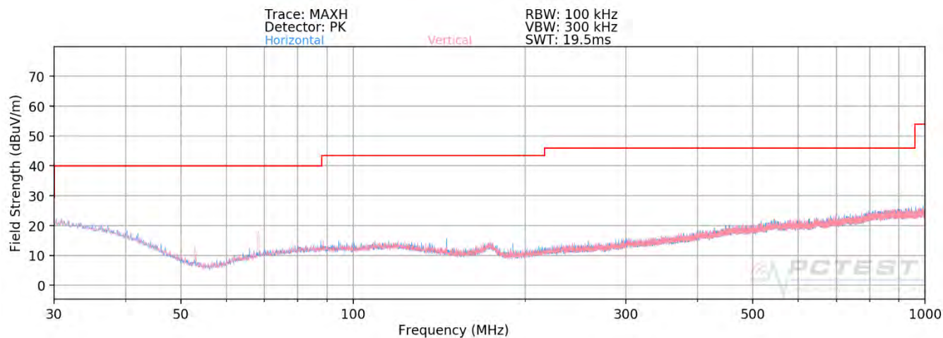
Plot 7-101. Radiated Spurious Plot below 1GHz MIMO (106 Tones)
