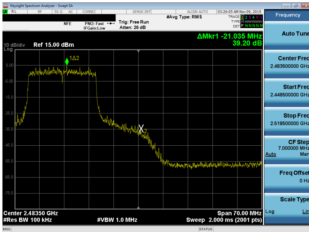
Plot 7-26. Band Edge Plot SISO ANT1 (802.11ax OFDMA – 242 Tones – Ch. 11)
