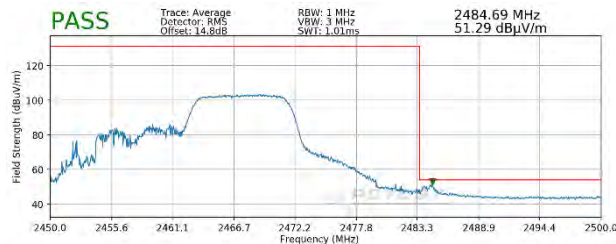
Plot 7-95. Radiated Restricted Upper Band Edge Measurement MIMO (Average – 106 Tones)
