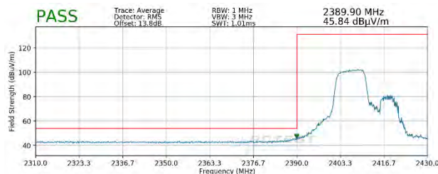
Plot 7-77. Radiated Restricted Lower Band Edge Measurement SISO ANT1 (Average – 106 Tones)
