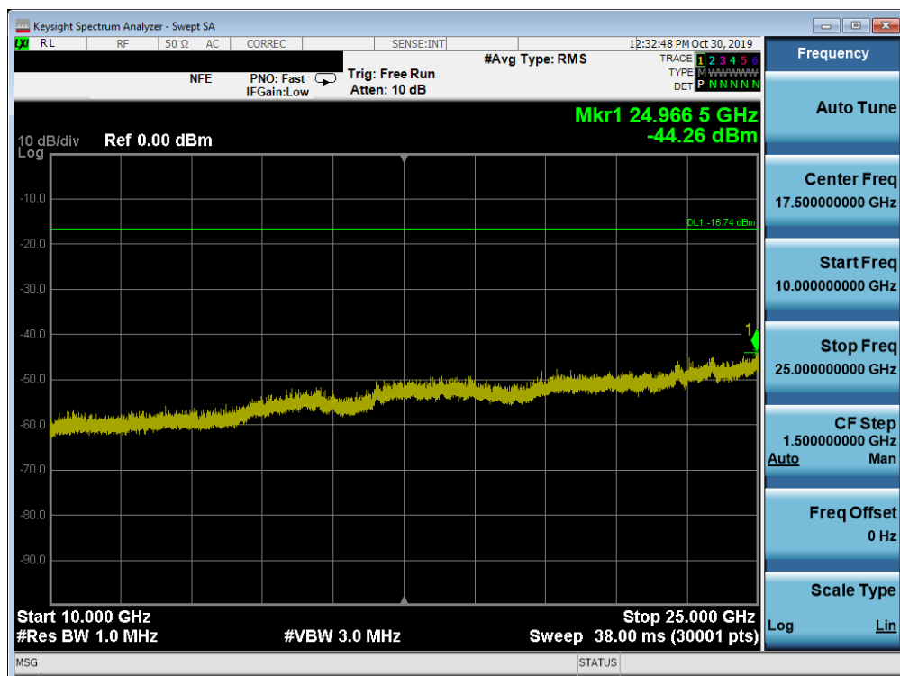
Plot 7-64. Conducted Spurious Plot SISO ANT1 (802.11b – Ch. 11)
