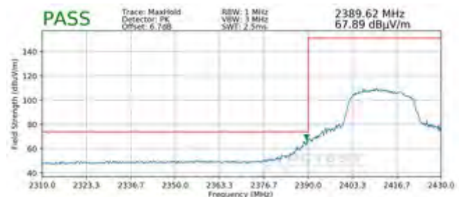
Plot 7-100. Radiated Restricted Lower Band Edge Measurement MIMO (Peak)
