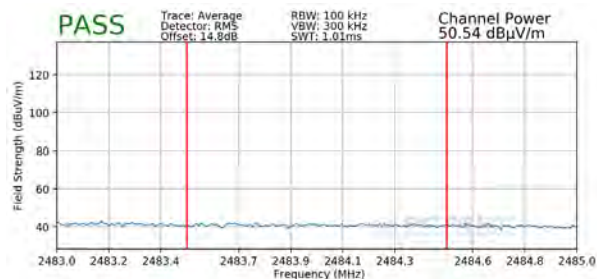
Plot 7-89. Radiated Restricted Upper Band Edge Measurement SISO ANT1 (Average)
