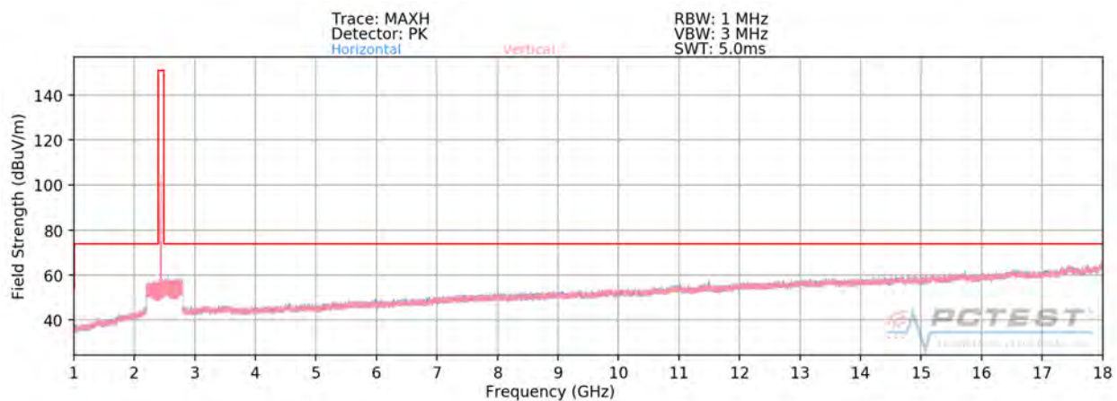
Plot 7-76. Radiated Spurious Plot above 1GHz SISO ANT2 (802.11b – Ch. 6)
