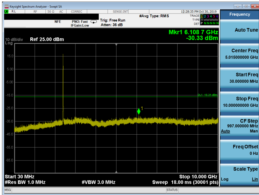
Plot 7-59. Conducted Spurious Plot SISO ANT1 (802.11b – Ch. 1)
