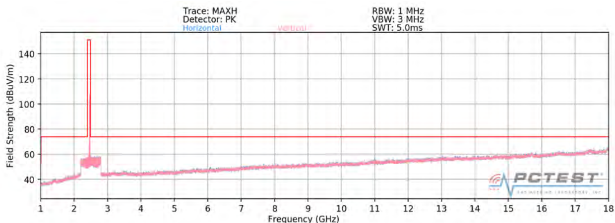
Plot 7-73. Radiated Spurious Plot above 1GHz SISO ANT1 (802.11b – Ch. 11)
