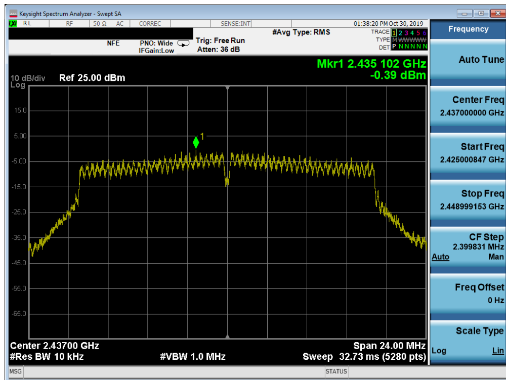
Plot 7-38. Power Spectral Density Plot SISO ANT2 (802.11n (2.4GHz) – Ch. 6)
