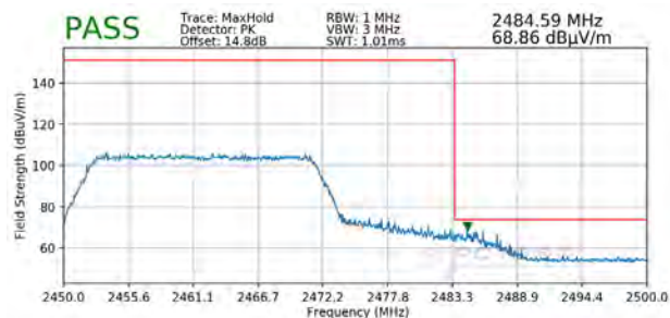
Plot 7-90. Radiated Restricted Upper Band Edge Measurement SISO ANT1 (Peak)
