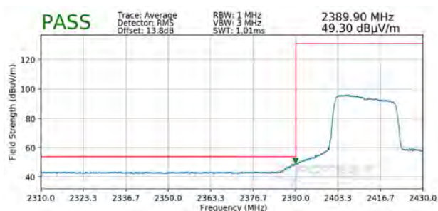
Plot 7-91. Radiated Restricted Lower Band Edge Measurement SISO ANT2 (Average)
