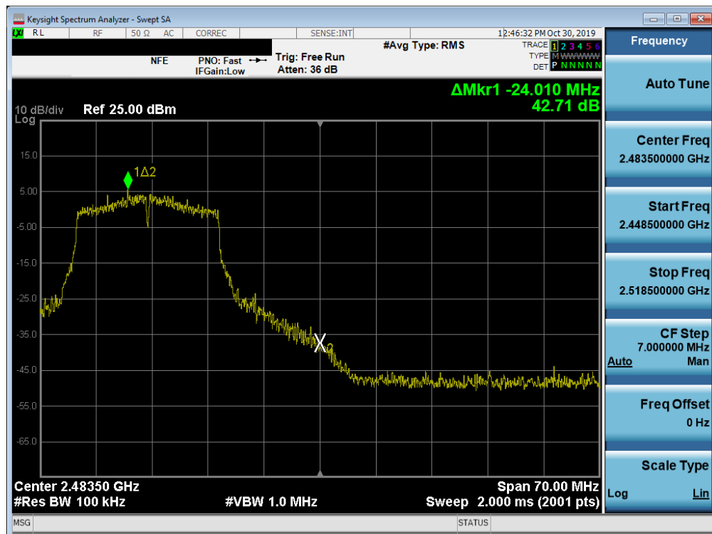
Plot 7-48. Band Edge Plot SISO ANT1 (802.11n (2.4GHz) – Ch. 11)
