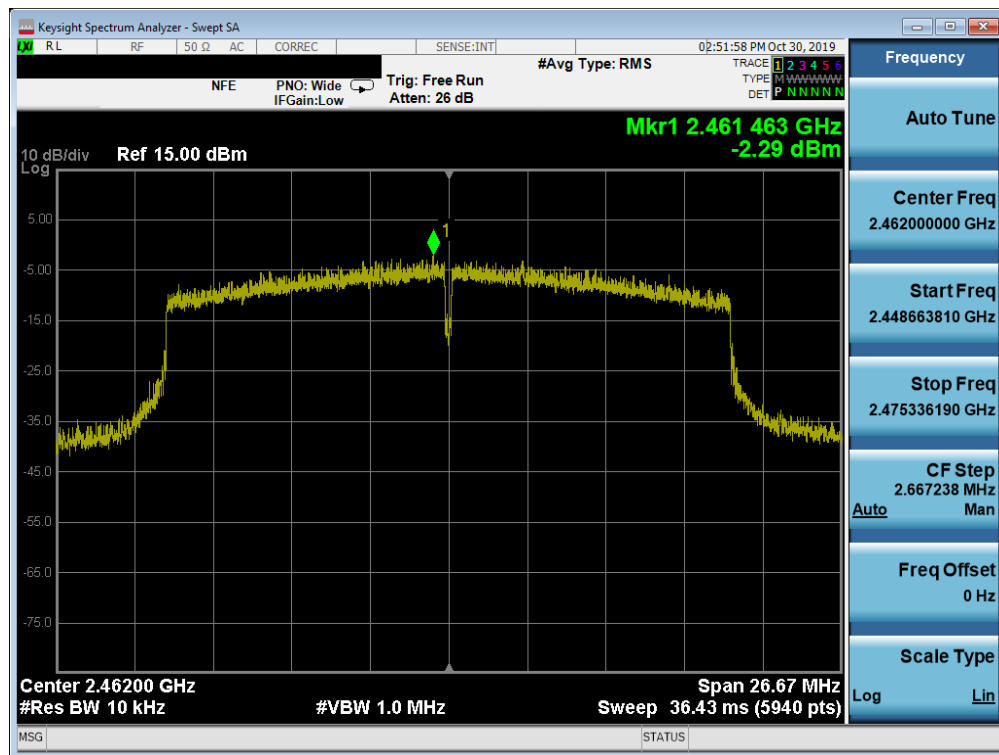
Plot 7-30. Power Spectral Density Plot SISO ANT1 (802.11ax (2.4GHz) – Ch. 11)
