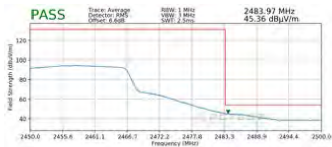
Plot 7-95. Radiated Restricted Upper Band Edge Measurement SISO ANT2 (Average)
