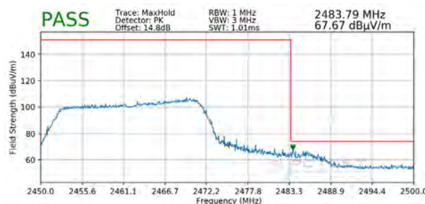
Plot 7-98. Radiated Restricted Upper Band Edge Measurement SISO ANT2 (Peak)
