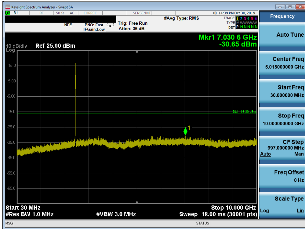
Plot 7-69. Conducted Spurious Plot SISO ANT2 (802.11b – Ch. 11)
