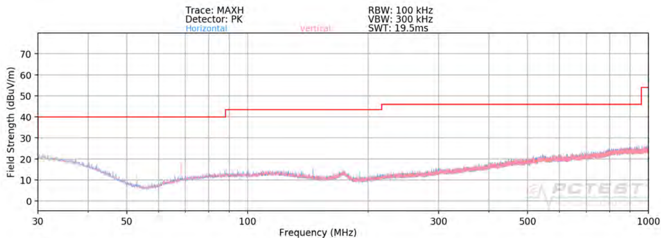
Plot 7-107. Radiated Spurious Plot below 1GHz SISO ANT1
