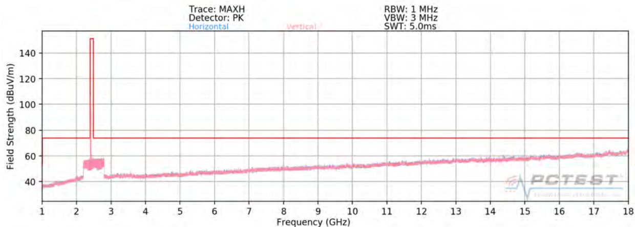
Plot 7-71. Radiated Spurious Plot above 1GHz SISO ANT1 (802.11b – Ch. 1)
