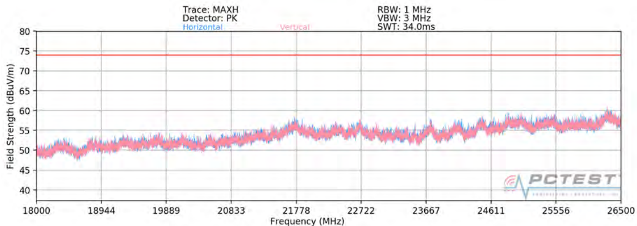
Plot 7-82. Radiated Spurious Plot above 18GHz MIMO/CDD
