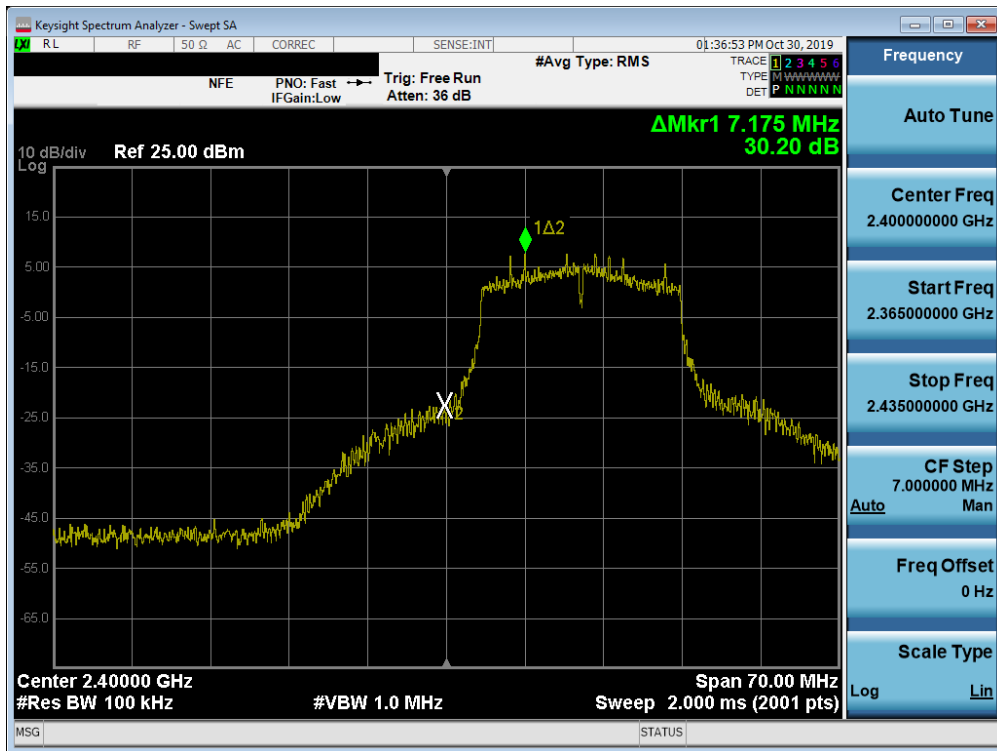
Plot 7-55. Band Edge Plot SISO ANT2 (802.11n (2.4GHz) – Ch. 1)
