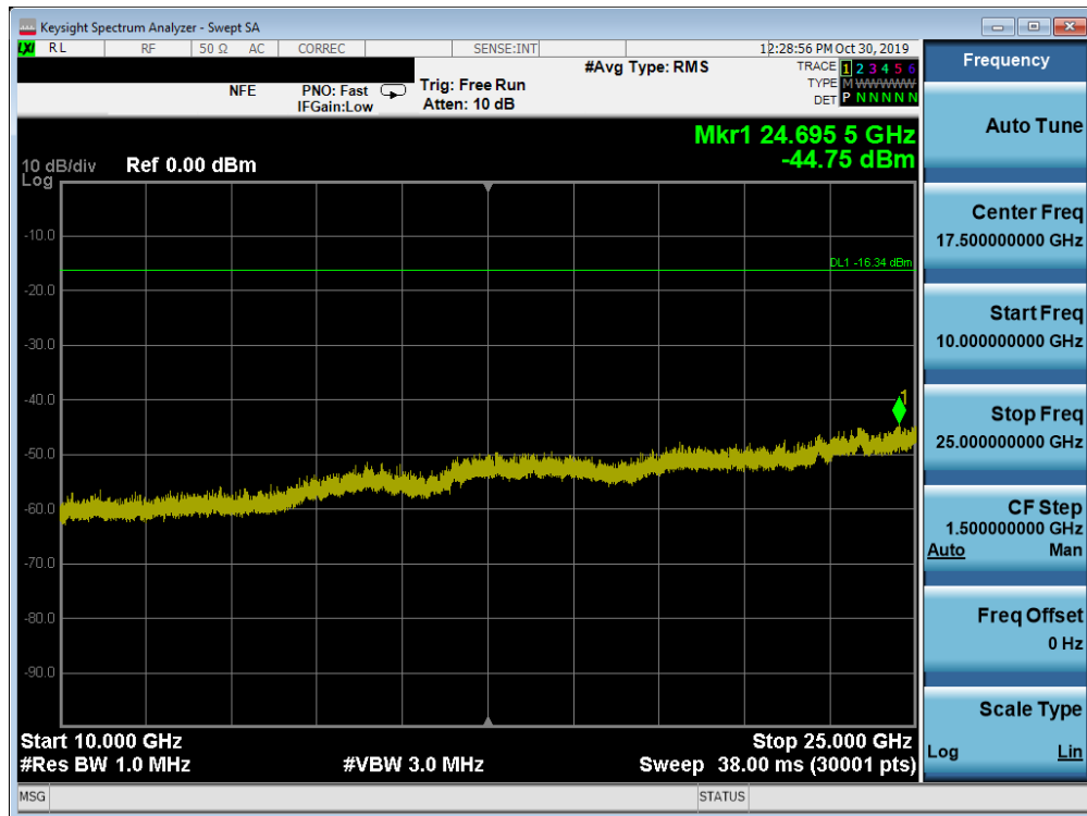
Plot 7-60. Conducted Spurious Plot SISO ANT1 (802.11b – Ch. 1)
