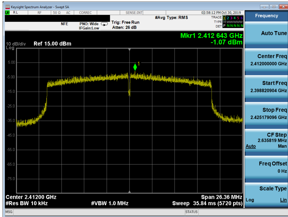
Plot 7-40. Power Spectral Density Plot SISO ANT2 (802.11ax (2.4GHz) – Ch. 1)
