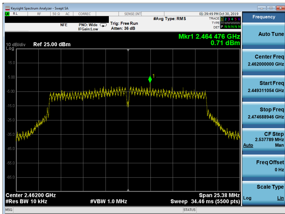
Plot 7-39. Power Spectral Density Plot SISO ANT2 (802.11n (2.4GHz) – Ch. 11)
