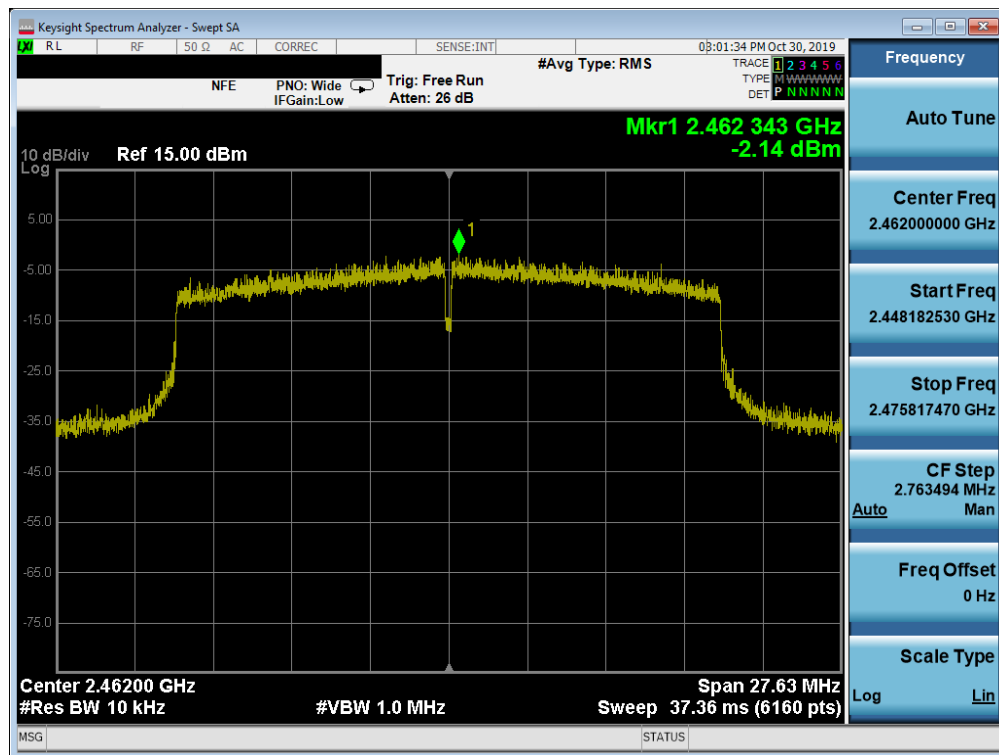
Plot 7-42. Power Spectral Density Plot SISO ANT2 (802.11ax (2.4GHz) – Ch. 11)
