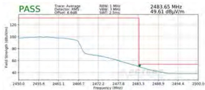
Plot 7-103. Radiated Restricted Upper Band Edge Measurement MIMO (Average)
