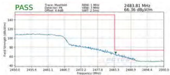
Plot 7-104. Radiated Restricted Upper Band Edge Measurement MIMO (Peak)
