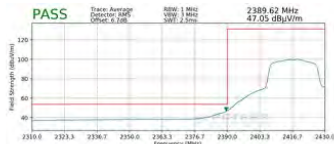
Plot 7-101. Radiated Restricted Lower Band Edge Measurement MIMO (Average)
