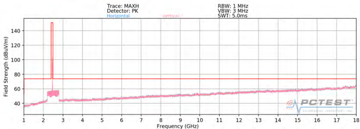
Plot 7-81. Radiated Spurious Plot above 1GHz MIMO/CDD (802.11g – Ch. 11)
