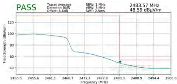
Plot 7-87. Radiated Restricted Upper Band Edge Measurement SISO ANT1 (Average)
