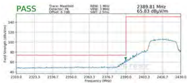
Plot 7-94. Radiated Restricted Lower Band Edge Measurement SISO ANT2 (Peak)
