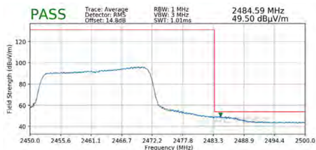
Plot 7-97. Radiated Restricted Upper Band Edge Measurement SISO ANT2 (Average)
