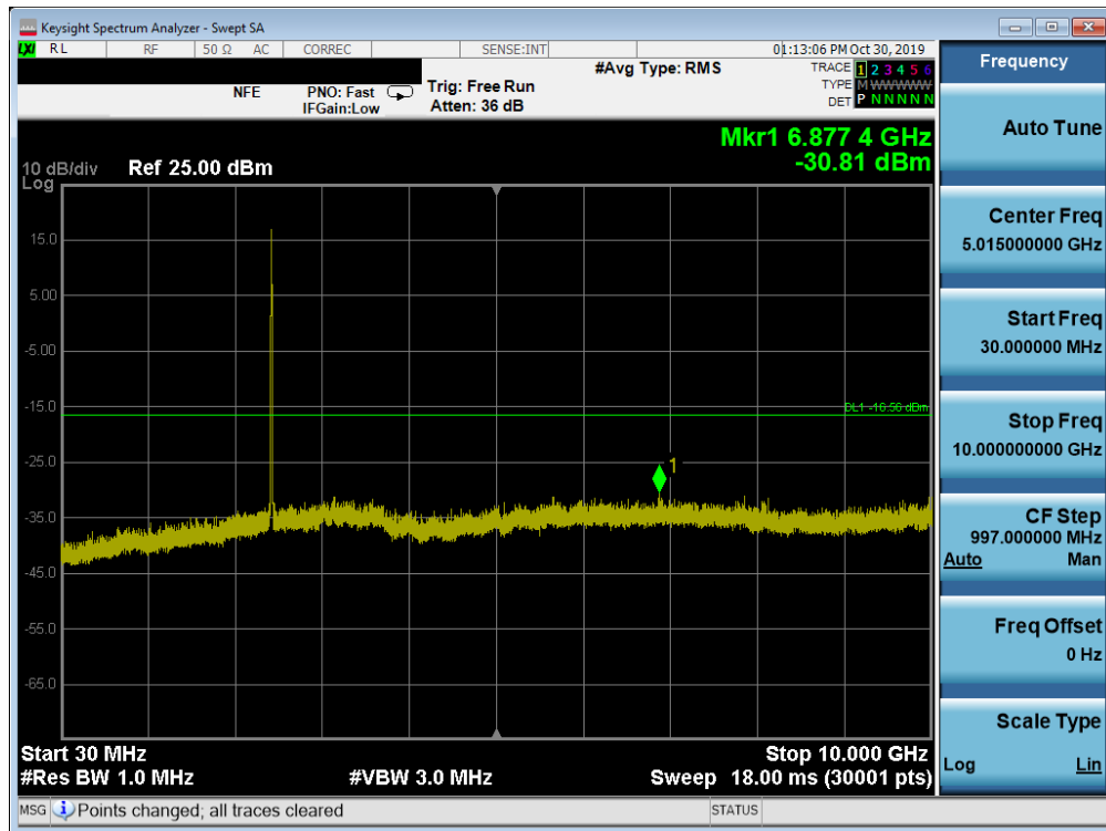
Plot 7-67. Conducted Spurious Plot SISO ANT2 (802.11b - Ch. 6)
