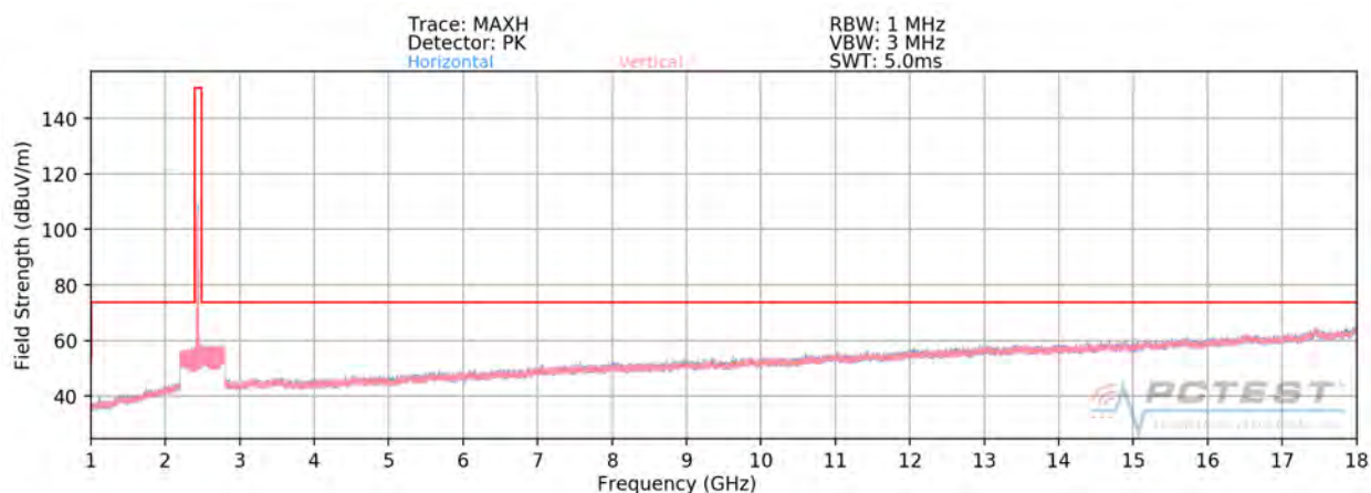
Plot 7-80. Radiated Spurious Plot above 1GHz MIMO/CDD (802.11g – Ch. 6)
