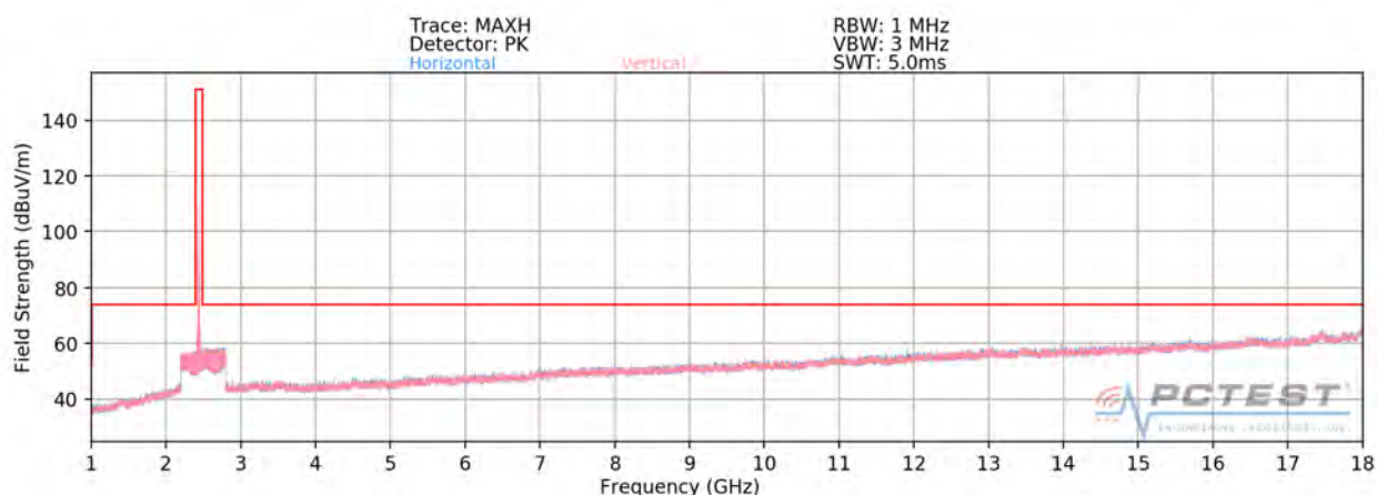
Plot 7-72. Radiated Spurious Plot above 1GHz SISO ANT1 (802.11b – Ch. 6)
