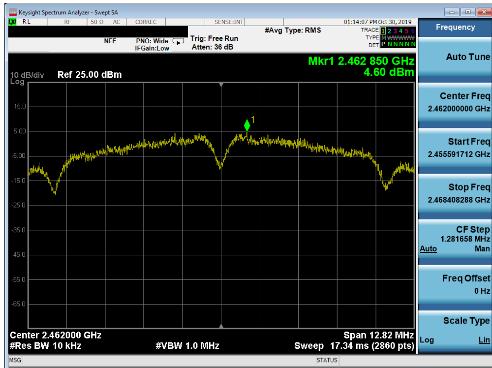
Plot 7-33. Power Spectral Density Plot SISO ANT2 (802.11b – Ch. 11)
