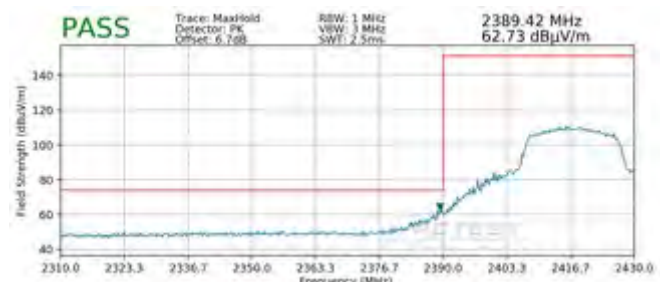
Plot 7-102. Radiated Restricted Lower Band Edge Measurement MIMO (Peak)
