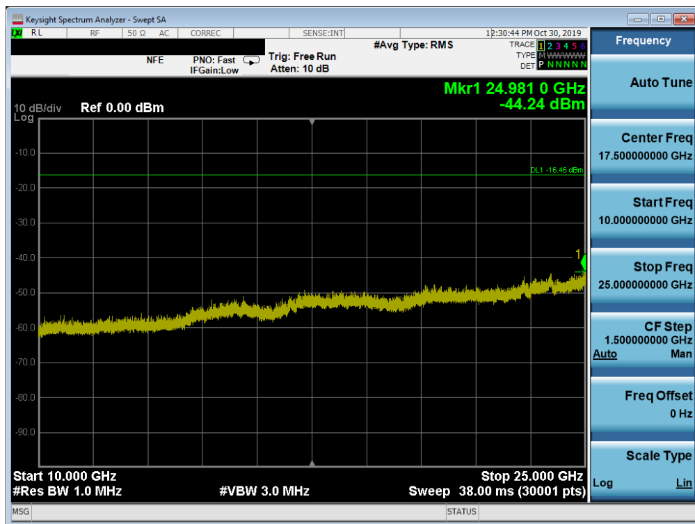
Plot 7-62. Conducted Spurious Plot SISO ANT1 (802.11b – Ch. 6)
