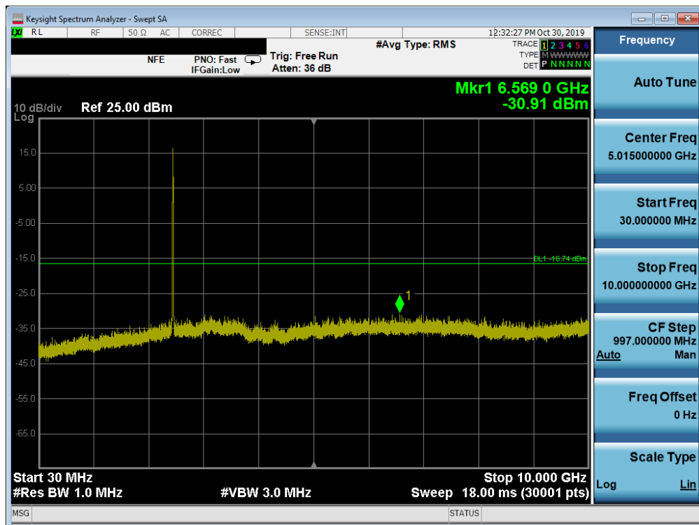
Plot 7-63. Conducted Spurious Plot SISO ANT1 (802.11b – Ch. 11)
