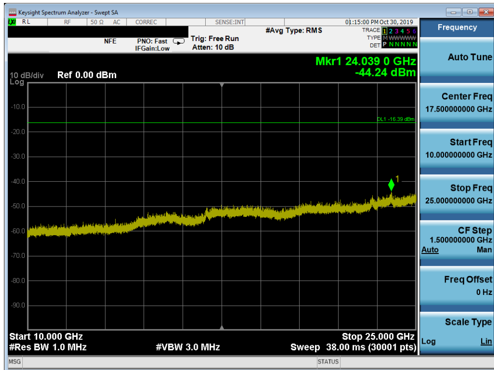
Plot 7-70. Conducted Spurious Plot SISO ANT2 (802.11b – Ch. 11)
