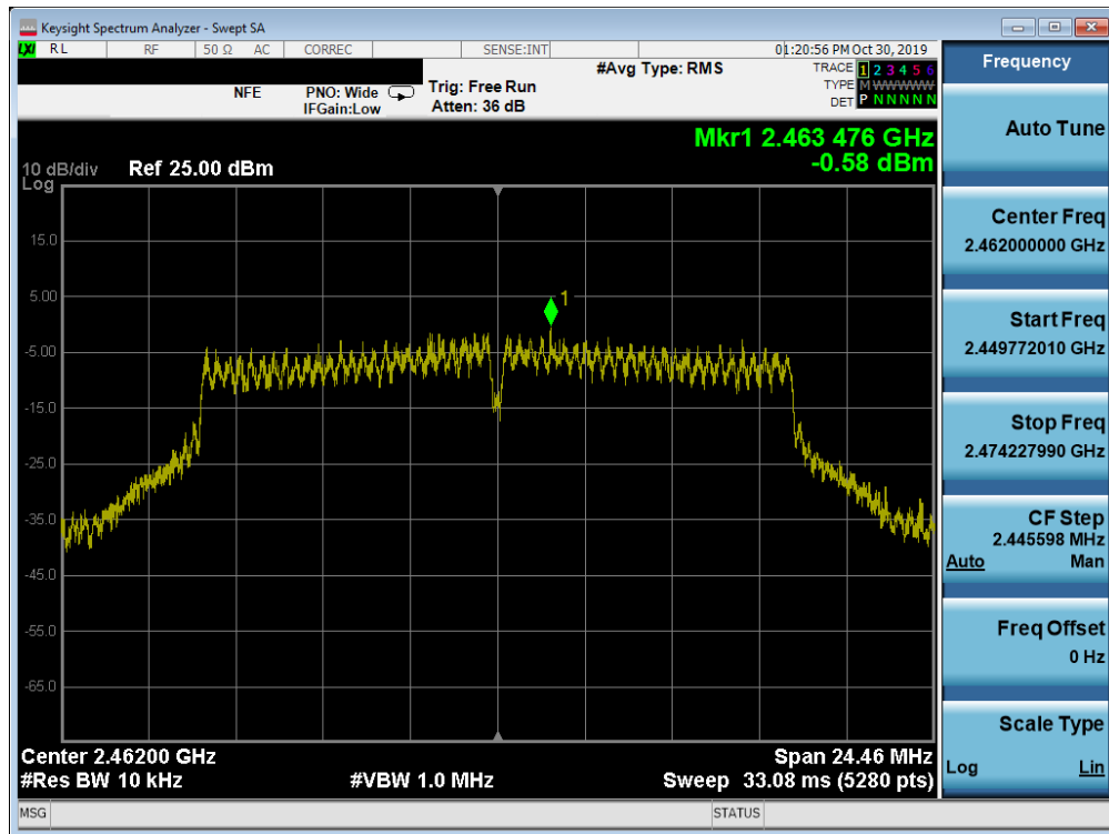
Plot 7-36. Power Spectral Density Plot SISO ANT2 (802.11g – Ch. 11)
