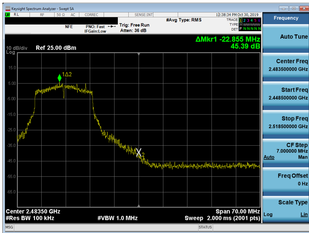
Plot 7-46. Band Edge Plot SISO ANT1 (802.11g - Ch. 11)
