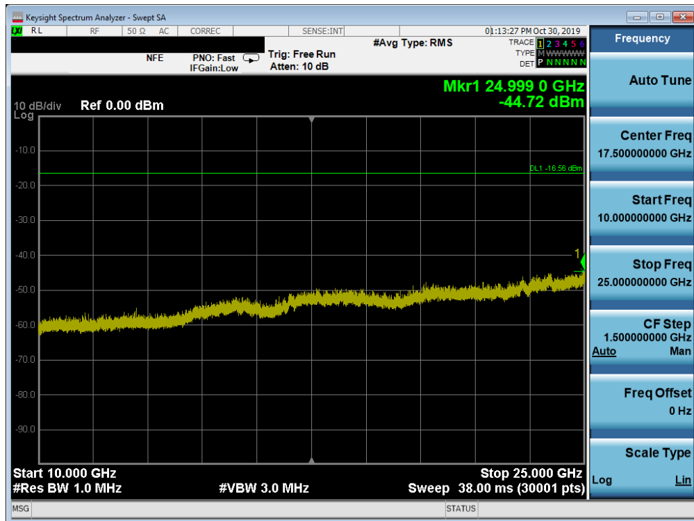
Plot 7-68. Conducted Spurious Plot SISO ANT2 (802.11b - Ch. 6)
