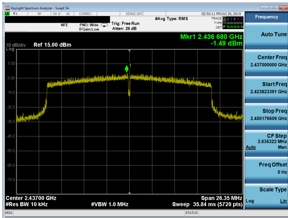
Plot 7-29. Power Spectral Density Plot SISO ANT1 (802.11ax (2.4GHz) – Ch. 6)
