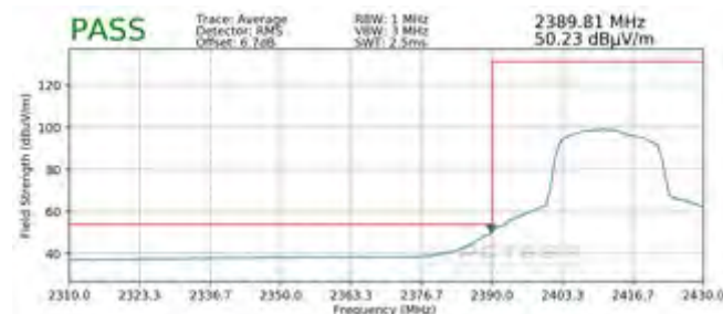
Plot 7-99. Radiated Restricted Lower Band Edge Measurement MIMO (Average)
