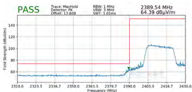
Plot 7-92. Radiated Restricted Lower Band Edge Measurement SISO ANT2 (Peak)
