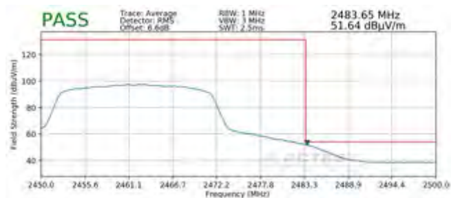
Plot 7-105. Radiated Restricted Upper Band Edge Measurement MIMO (Average)
