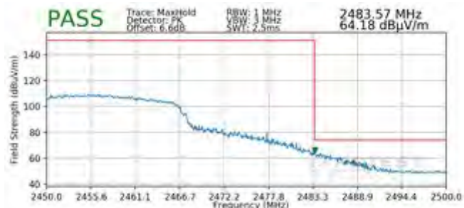
Plot 7-88. Radiated Restricted Upper Band Edge Measurement SISO ANT1 (Peak)
