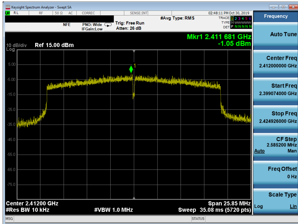
Plot 7-28. Power Spectral Density Plot SISO ANT1 (802.11ax (2.4GHz) – Ch. 1)
