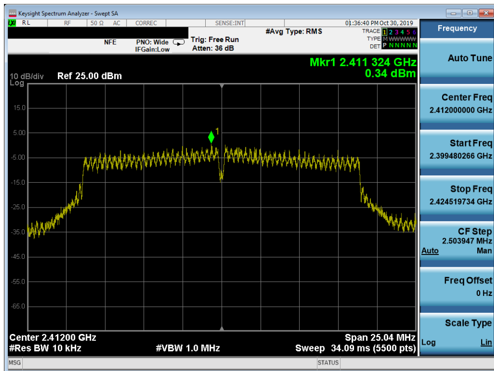
Plot 7-37. Power Spectral Density Plot SISO ANT2 (802.11n (2.4GHz) – Ch. 1)
