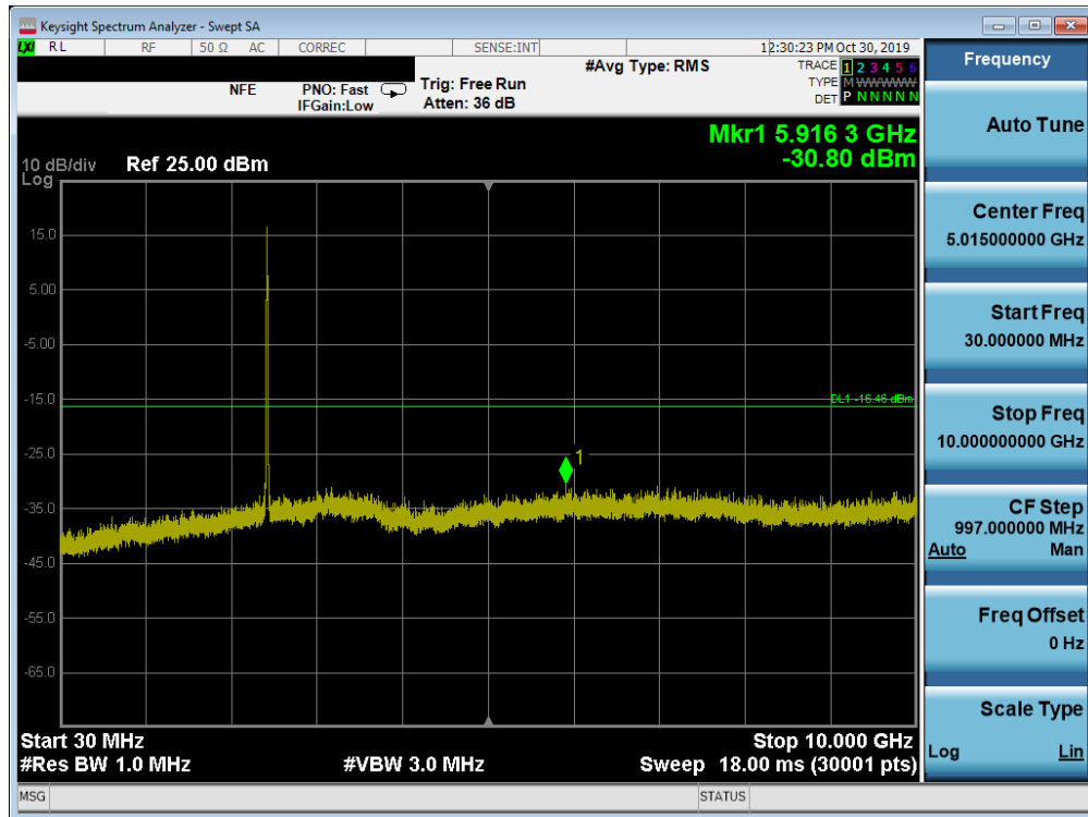
Plot 7-61. Conducted Spurious Plot SISO ANT1 (802.11b – Ch. 6)
