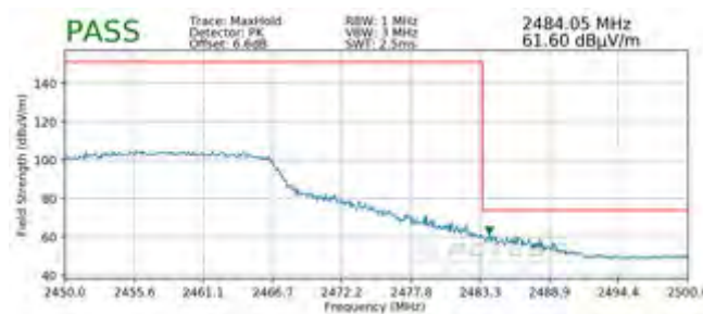
Plot 7-96. Radiated Restricted Upper Band Edge Measurement SISO ANT2 (Peak)
