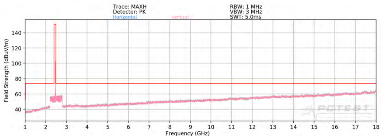
Plot 7-77. Radiated Spurious Plot above 1GHz SISO ANT2 (802.11b – Ch. 11)
