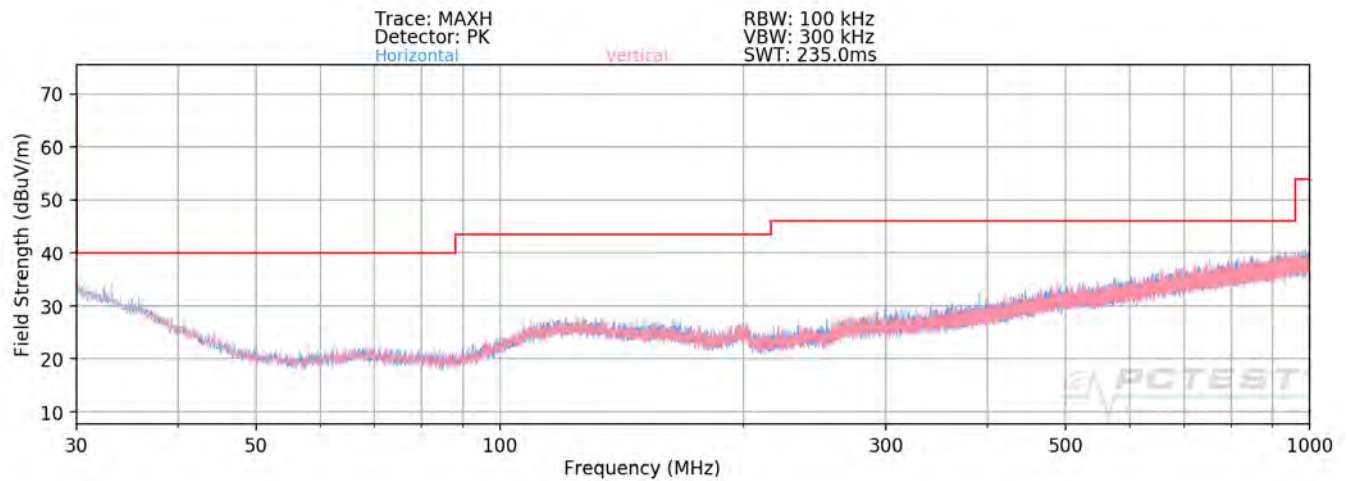
Plot 7-108. Radiated Spurious Plot below 1GHz SISO ANT2
