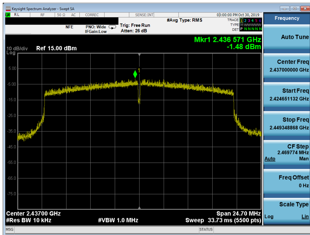
Plot 7-41. Power Spectral Density Plot SISO ANT2 (802.11ax (2.4GHz) – Ch. 6)
