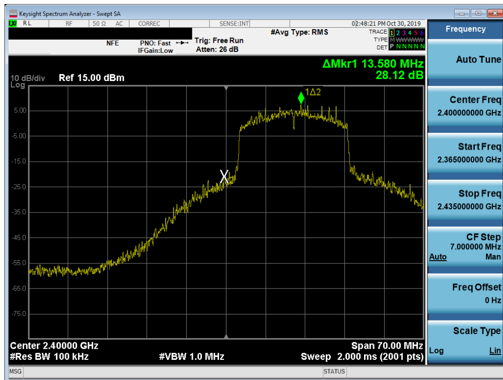
Plot 7-49. Band Edge Plot SISO ANT1 (802.11ax (2.4GHz) – Ch. 1)
