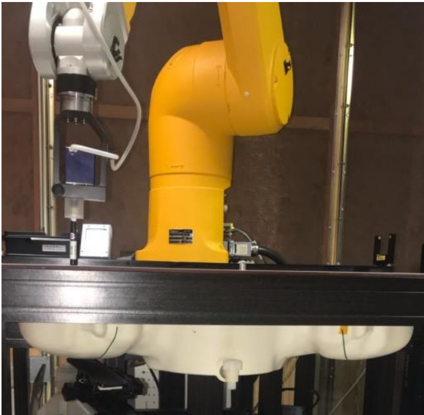
Figure 6-1 SAR measurement setup
