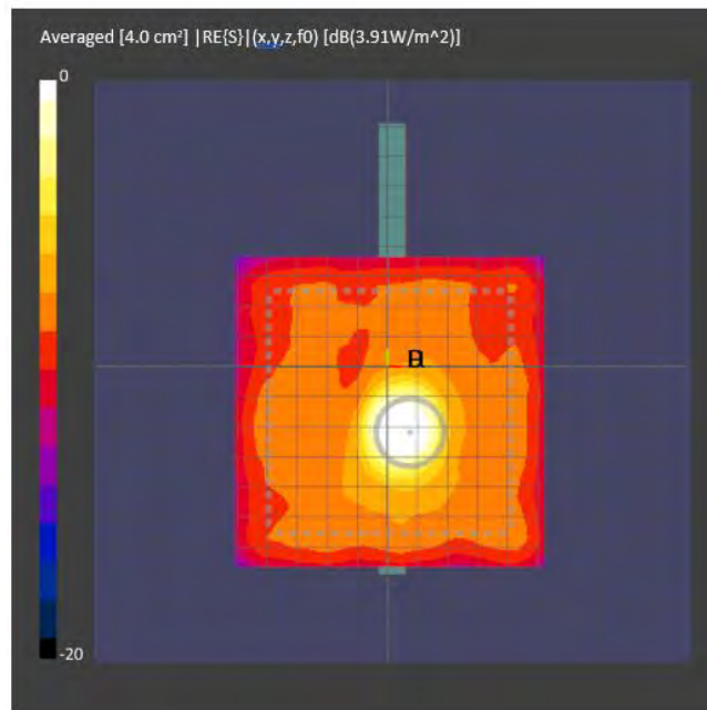
Figure 12-2 4cm 2 psPD distribution measured at input.power.limit of 8 dBm on the back surface for n260 beam 0
