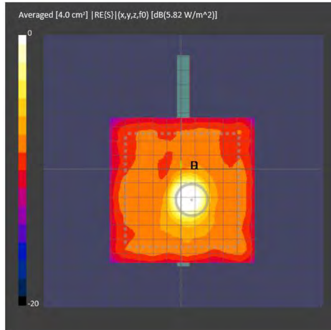
Figure 12-1 4cm 2 psPD distribution measured at input.power.limit of 4.8 dBm on the back surface for n261 beam 12
