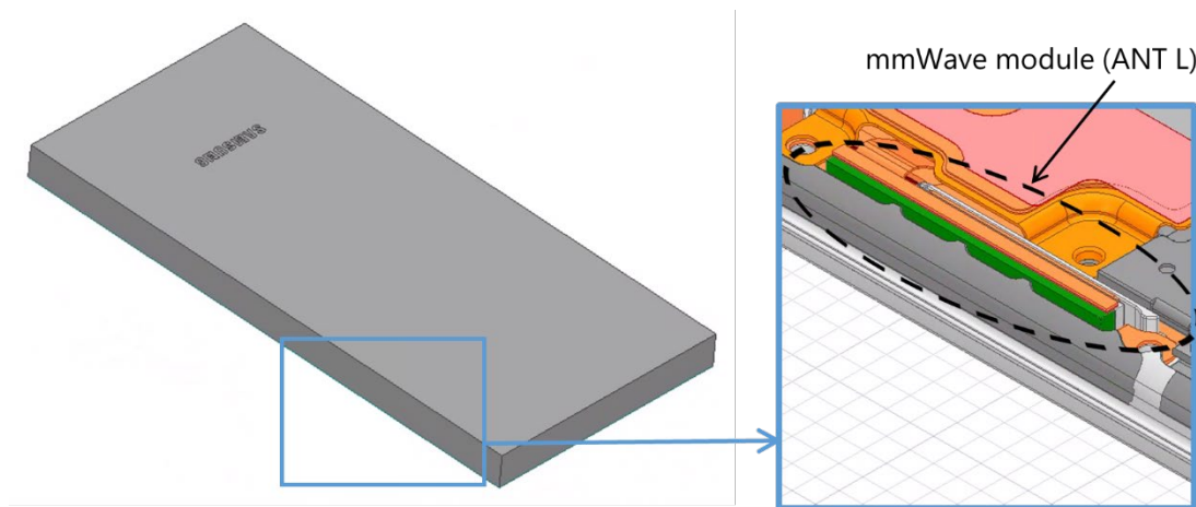
Figure 4. mmWave module (ANT L)
