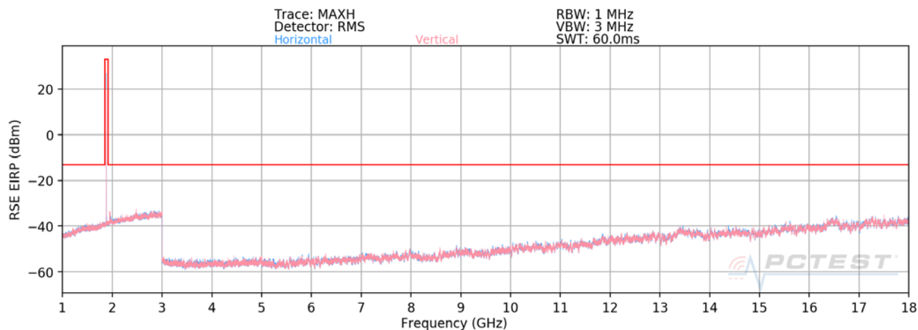
Plot 7-94. Radiated Spurious Plot above 1GHz (PCS GPRS Mode)
