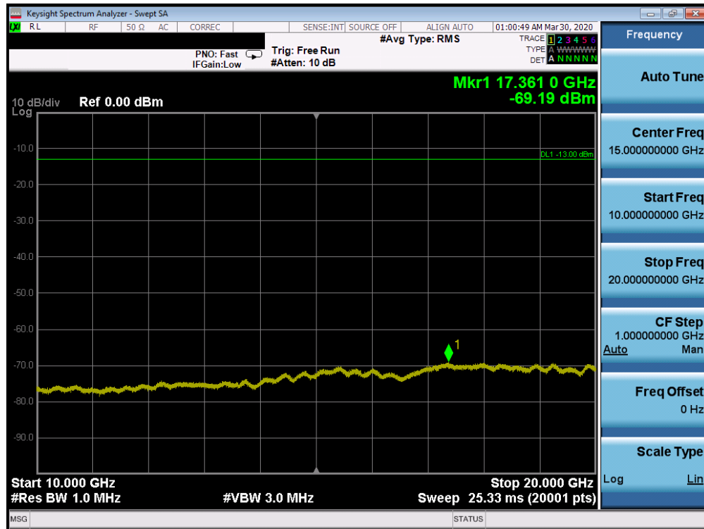
Plot 7-226. Conducted Spurious Plot (n66 - 20.0MHz DFT-s-OFDM BPSK - RB Size 1, RB Offset 0 - Low Channel)
