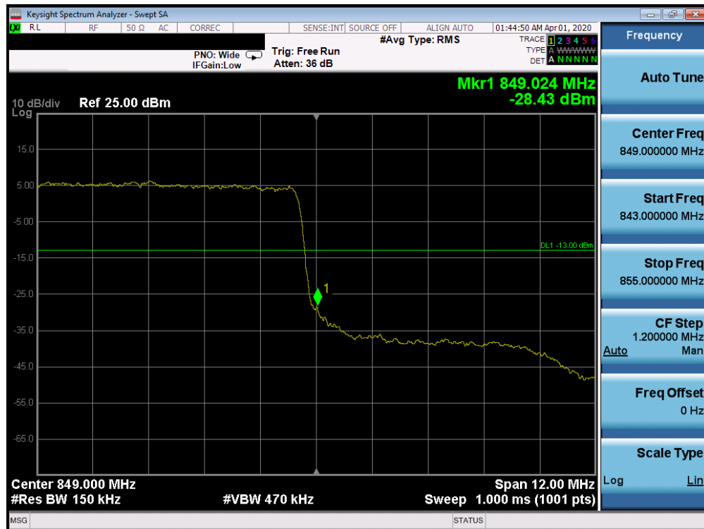
Plot 7-296. Upper Band Edge Plot (n5 – 15.0MHz DFT-s-OFDM BPSK - Full RB Configuration)
