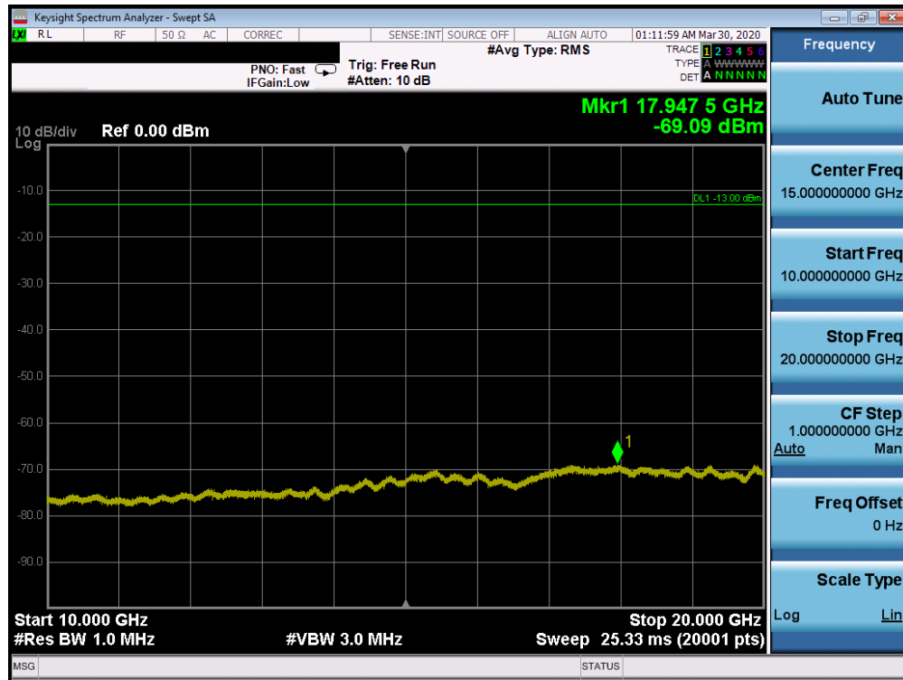
Plot 7-232. Conducted Spurious Plot (n66 - 20.0MHz DFT-s-OFDM BPSK - RB Size 1, RB Offset 0 - High Channel)
